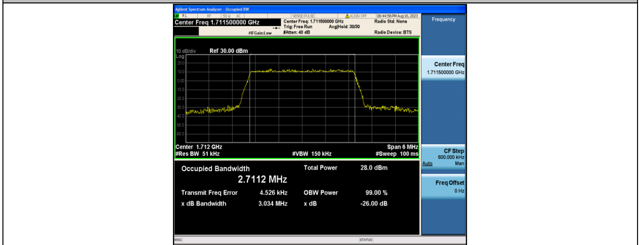
Band4-3MHz-16QAM-19965-15RB#0-PASS
