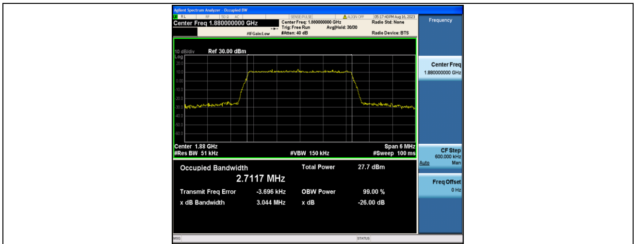
Band2-3MHz-16QAM-18900-15RB#0-PASS
