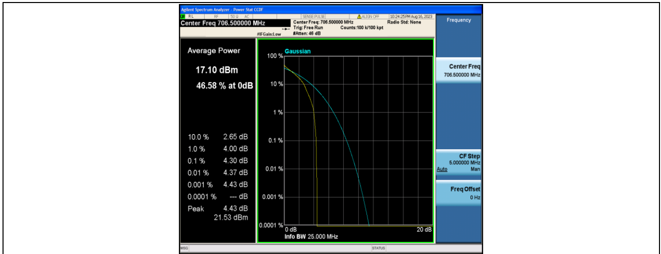
Band17-5MHz-QPSK-23755-1RB#0-PASS
