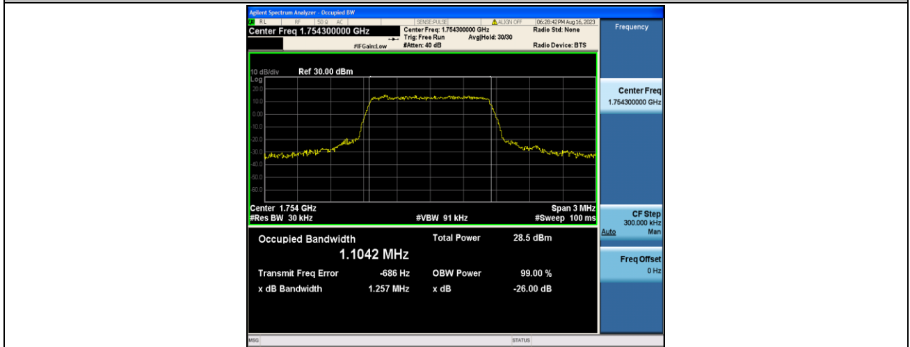
Band4-1.4MHz-16QAM-20393-6RB#0-PASS
