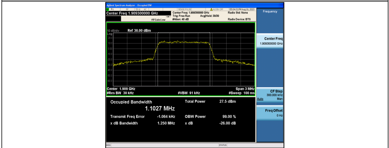
Band2-1.4MHz-16QAM-19193-6RB#0-PASS
