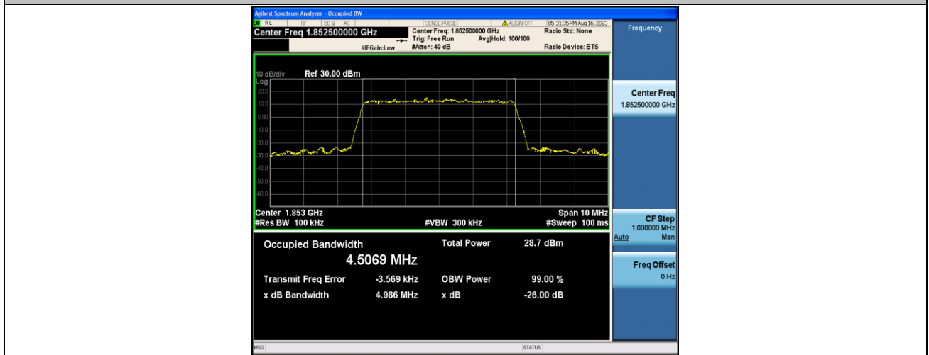
Band2-5MHz-16QAM-18625-25RB#0-PASS
