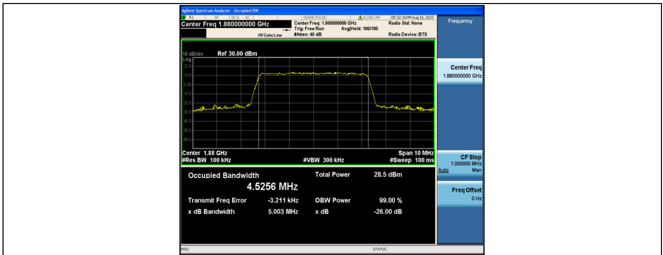
Band2-5MHz-16QAM-18900-25RB#0-PASS
