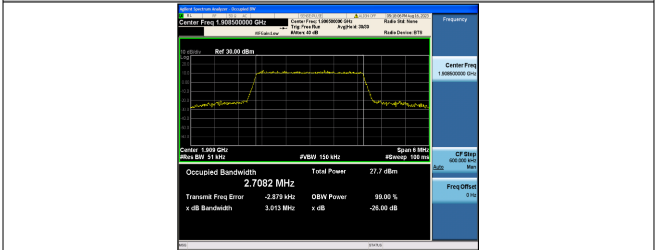
Band2-3MHz-16QAM-19185-15RB#0-PASS
