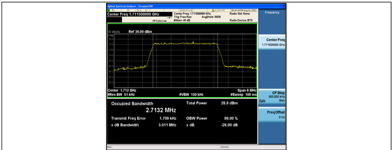
Band4-3MHz-QPSK-19965-15RB#0-PASS
