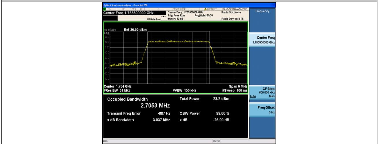
Band4-3MHz-16QAM-20385-15RB#0-PASS
