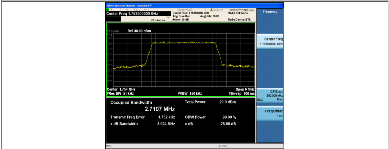
Band4-3MHz-QPSK-20385-15RB#0-PASS
