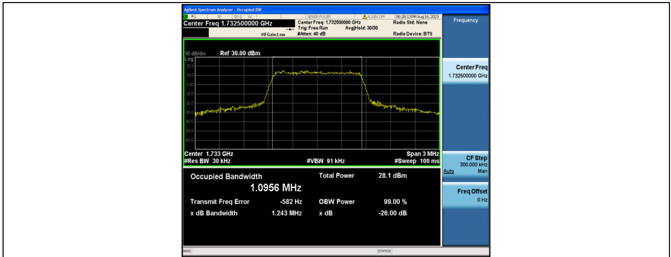
Band4-1.4MHz-16QAM-20175-6RB#0-PASS
