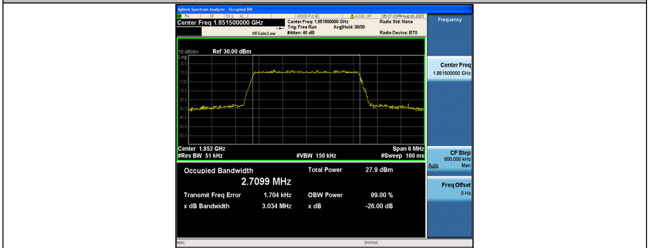
Band2-3MHz-16QAM-18615-15RB#0-PASS
