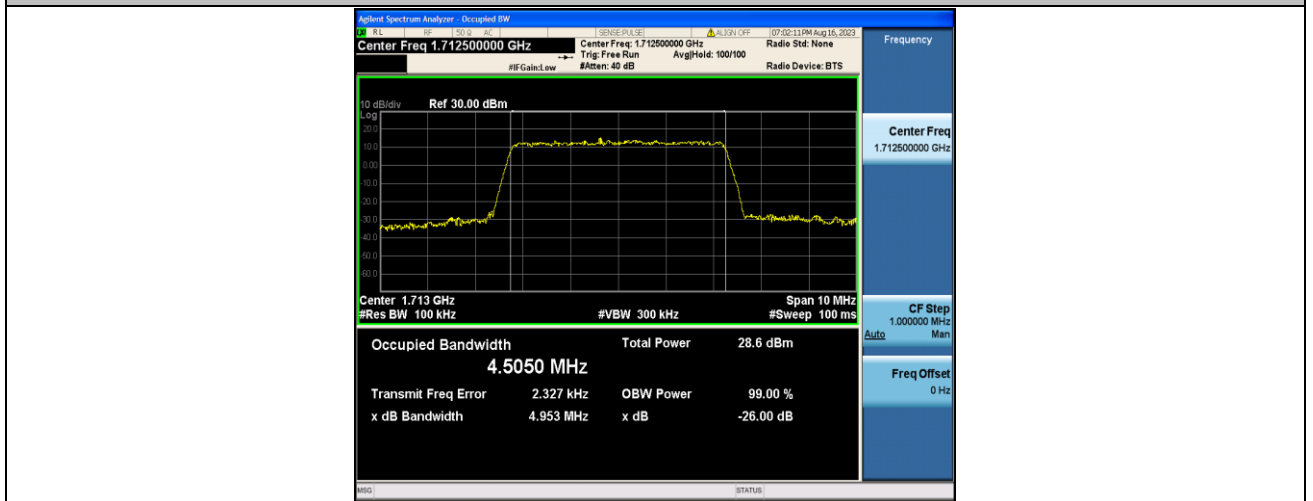
Band4-5MHz-16QAM-19975-25RB#0-PASS
