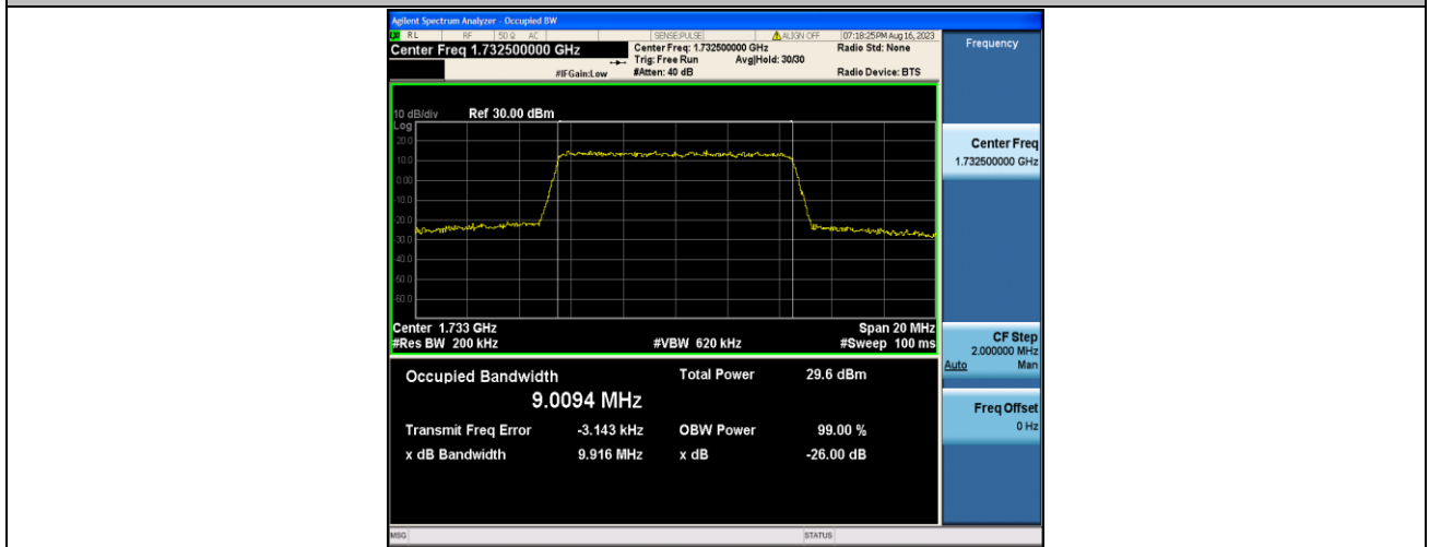
Band4-10MHz-QPSK-20175-50RB#0-PASS
