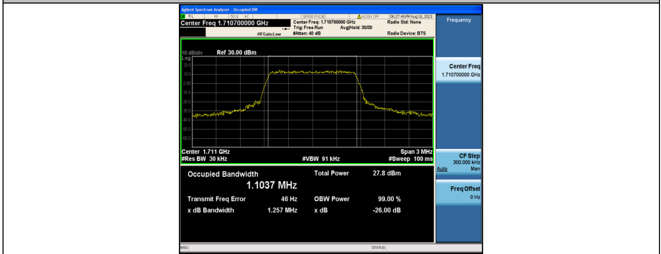
Band4-1.4MHz-16QAM-19957-6RB#0-PASS
