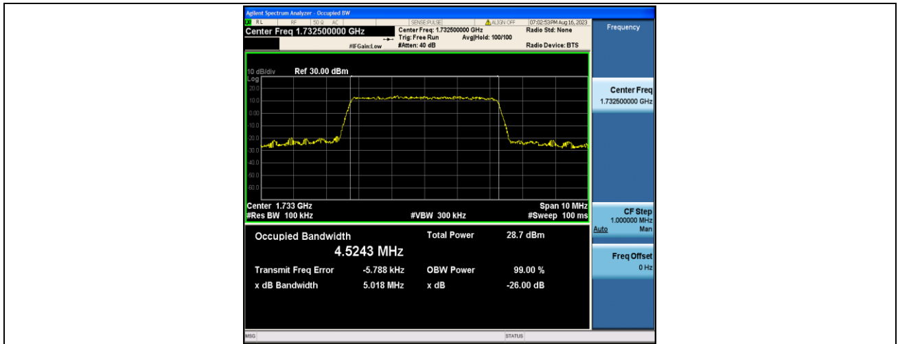
Band4-5MHz-16QAM-20175-25RB#0-PASS
