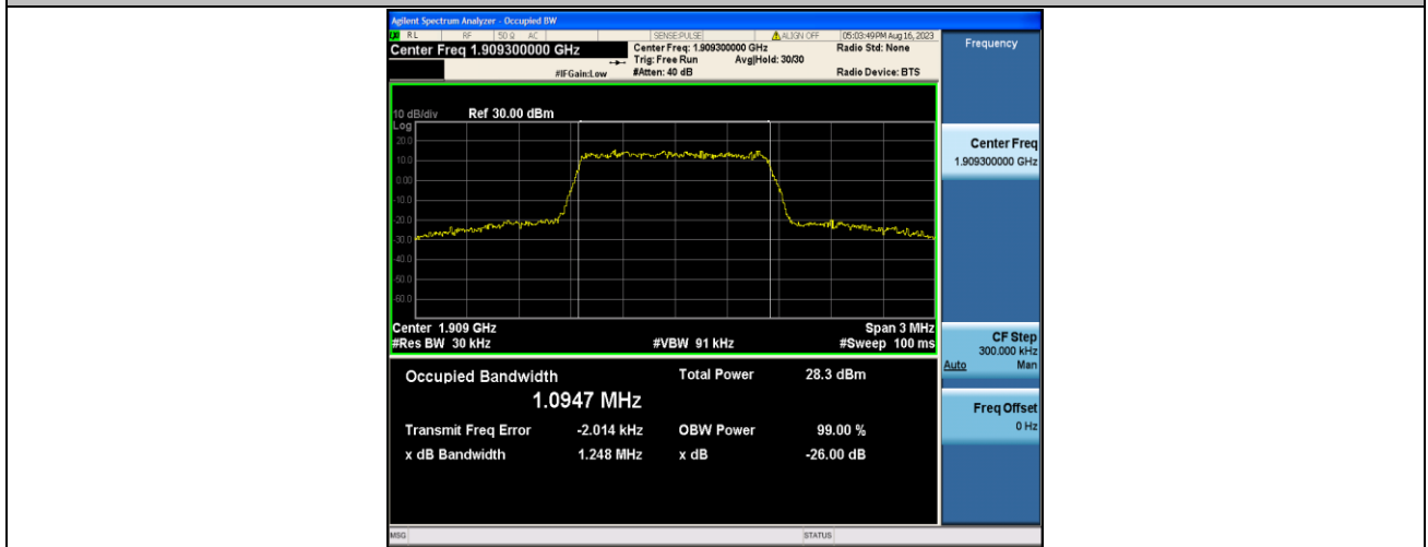
Band2-1.4MHz-QPSK-19193-6RB#0-PASS
