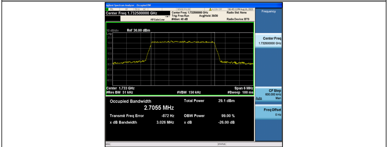
Band4-3MHz-QPSK-20175-15RB#0-PASS
