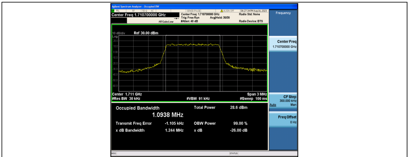
Band4-1.4MHz-QPSK-19957-6RB#0-PASS
