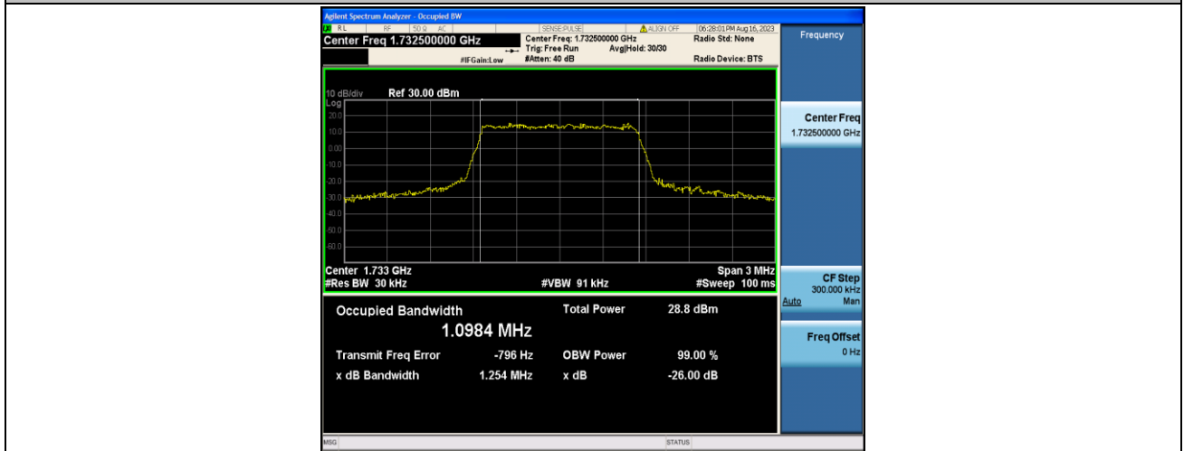
Band4-1.4MHz-QPSK-20175-6RB#0-PASS
