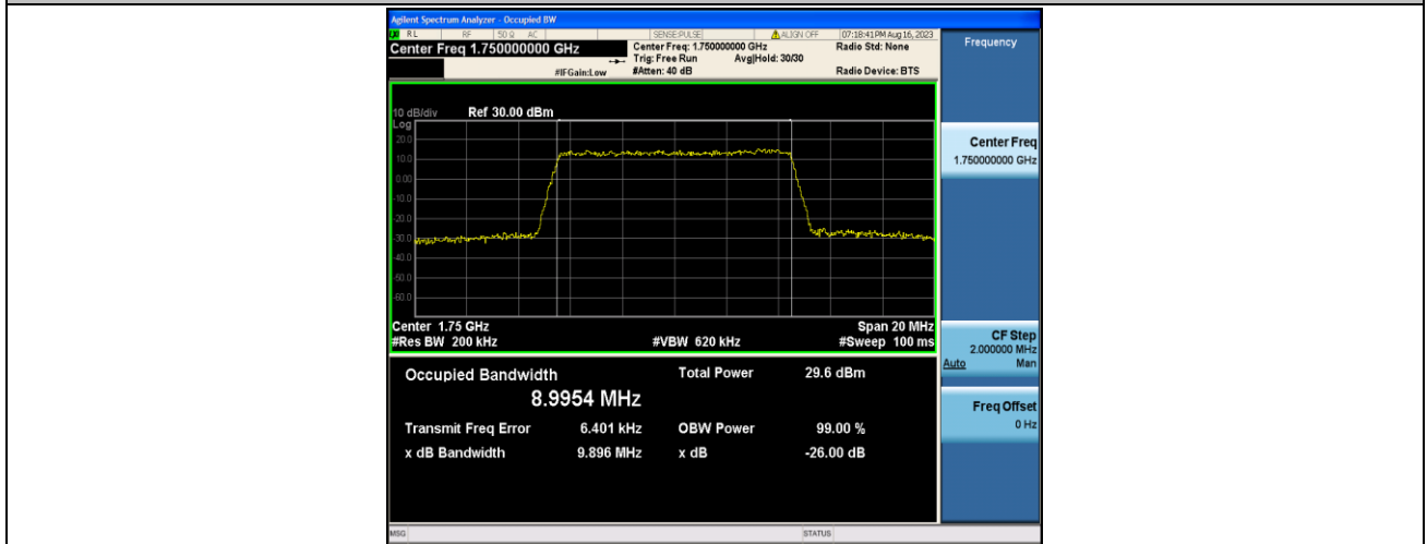
Band4-10MHz-QPSK-20350-50RB#0-PASS
