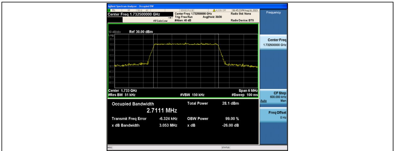
Band4-3MHz-16QAM-20175-15RB#0-PASS
