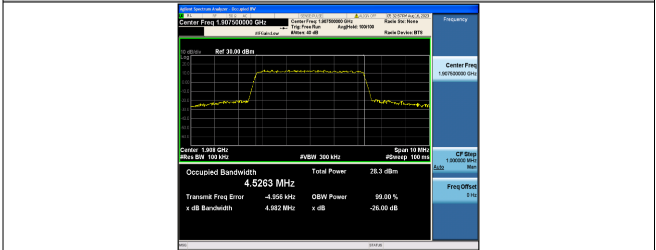
Band2-5MHz-16QAM-19175-25RB#0-PASS
