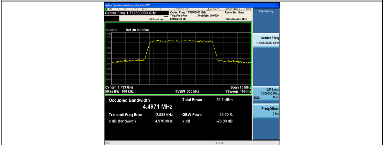
Band4-5MHz-QPSK-20175-25RB#0-PASS
