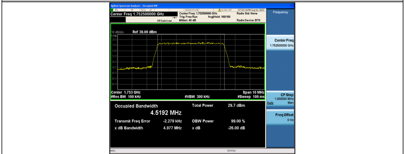
Band4-5MHz-QPSK-20375-25RB#0-PASS
