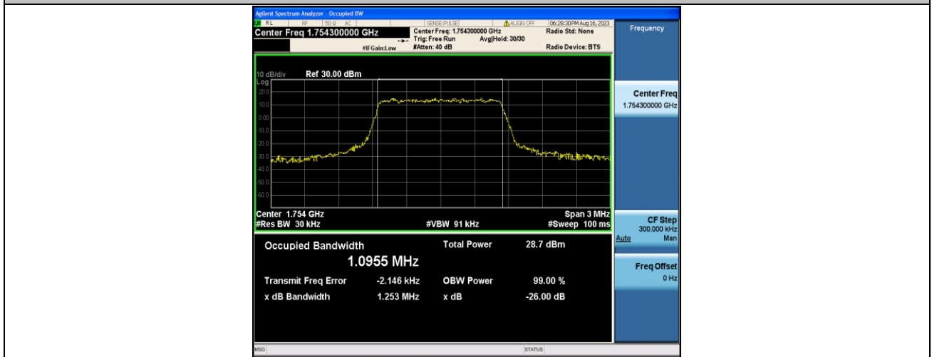
Band4-1.4MHz-QPSK-20393-6RB#0-PASS
