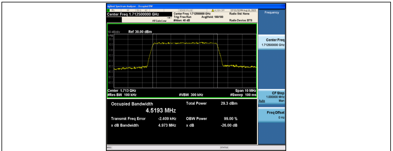
Band4-5MHz-QPSK-19975-25RB#0-PASS
