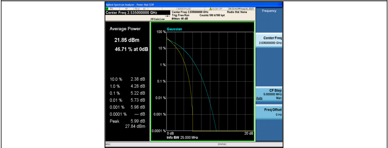
Band7-10MHz-QPSK-21100-50RB#0-PASS
