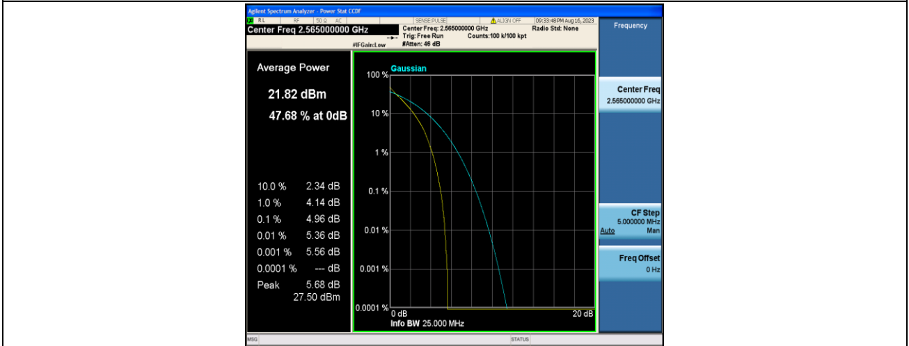
Band7-10MHz-QPSK-21400-50RB#0-PASS
