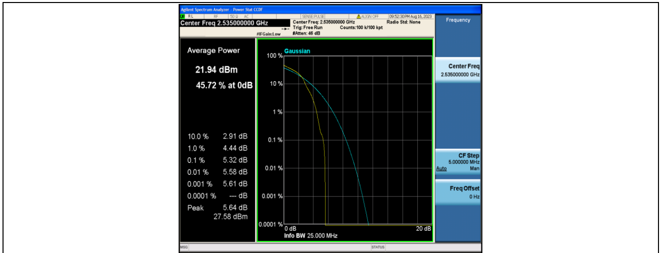
Band7-15MHz-16QAM-21100-1RB#0-PASS
