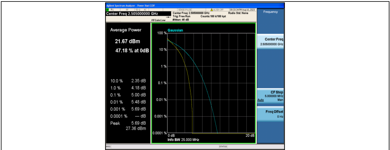
Band7-10MHz-QPSK-20800-50RB#0-PASS
