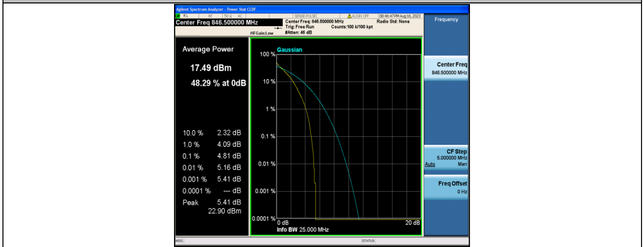
Band5-5MHz-QPSK-20625-25RB#0-PASS
