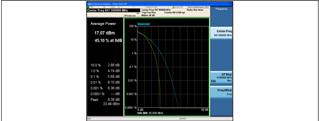
Band5-3MHz-16QAM-20635-15RB#0-PASS
