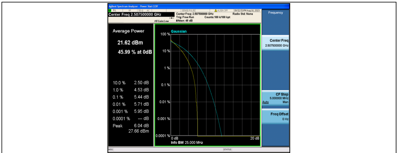
Band7-15MHz-QPSK-20825-75RB#0-PASS
