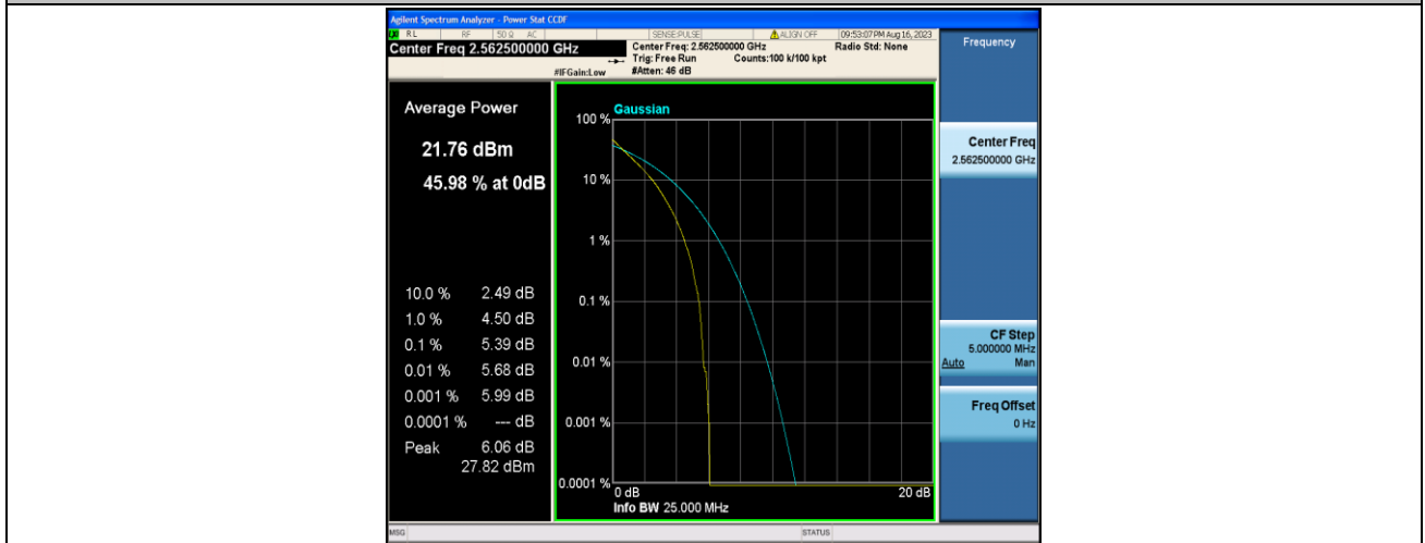
Band7-15MHz-QPSK-21375-75RB#0-PASS
