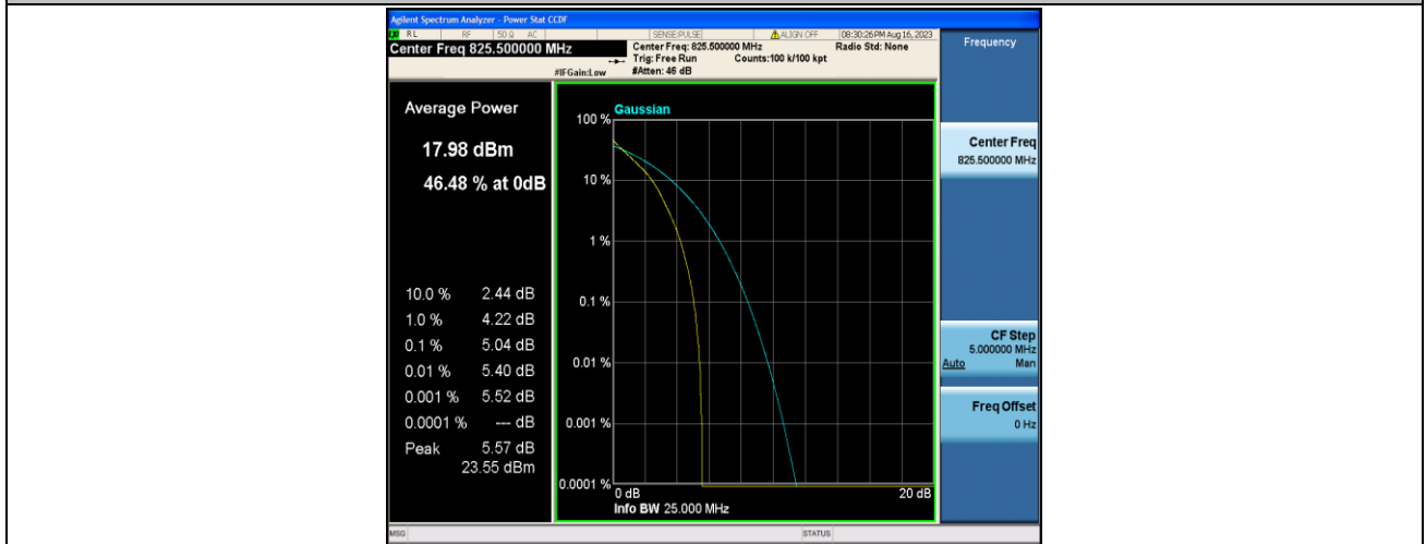
Band5-3MHz-QPSK-20415-15RB#0-PASS
