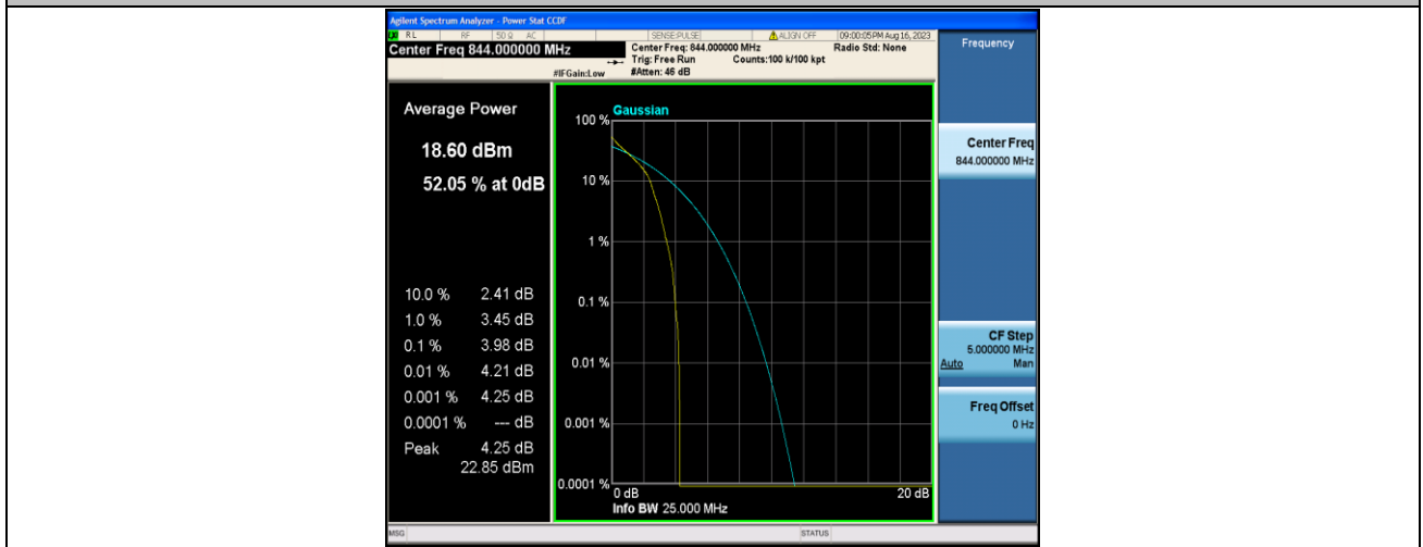
Band5-10MHz-QPSK-20600-1RB#0-PASS
