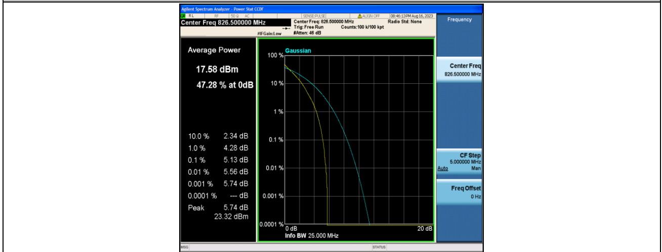
Band5-5MHz-QPSK-20425-25RB#0-PASS
