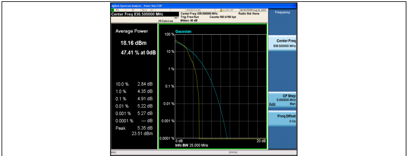
Band5-10MHz-16QAM-20525-1RB#0-PASS
