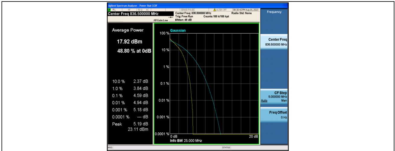
Band5-3MHz-QPSK-20525-15RB#0-PASS
