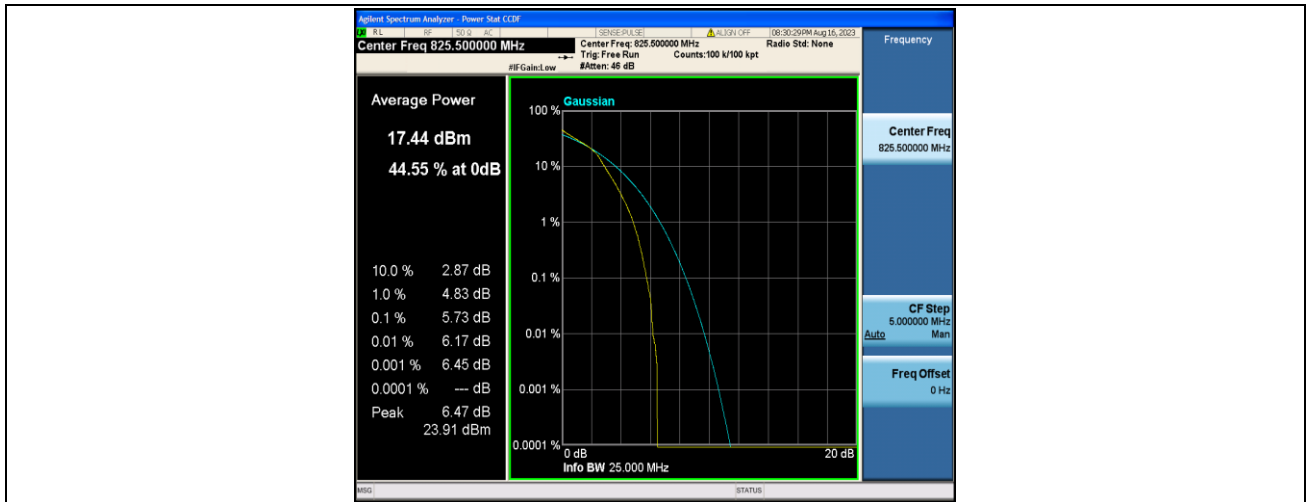
Band5-3MHz-16QAM-20415-15RB#0-PASS
