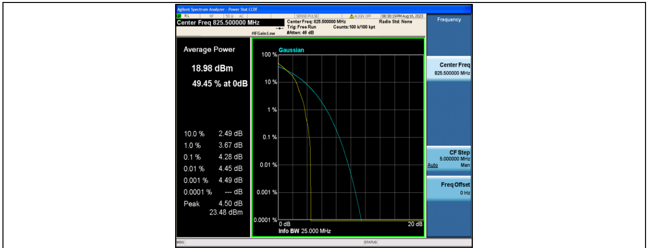
Band5-3MHz-QPSK-20415-1RB#0-PASS
