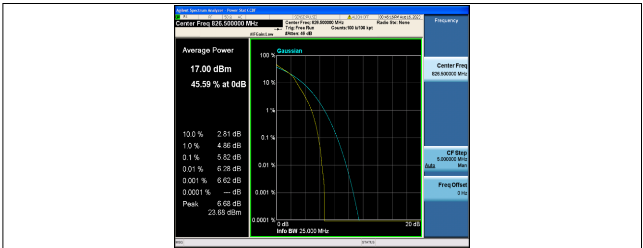
Band5-5MHz-16QAM-20425-25RB#0-PASS
