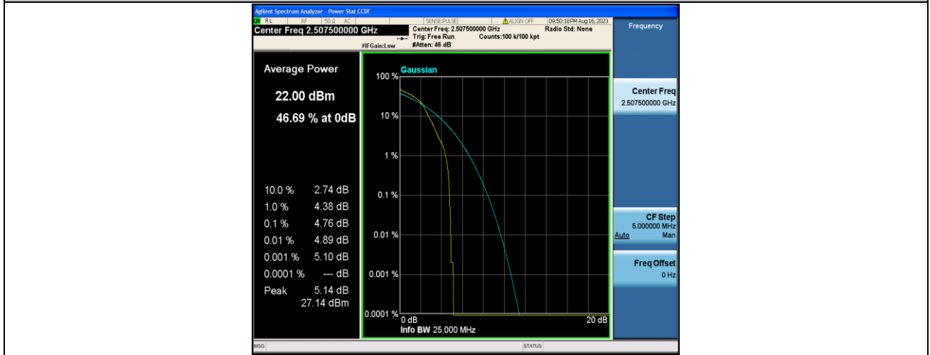
Band7-15MHz-16QAM-20825-1RB#0-PASS
