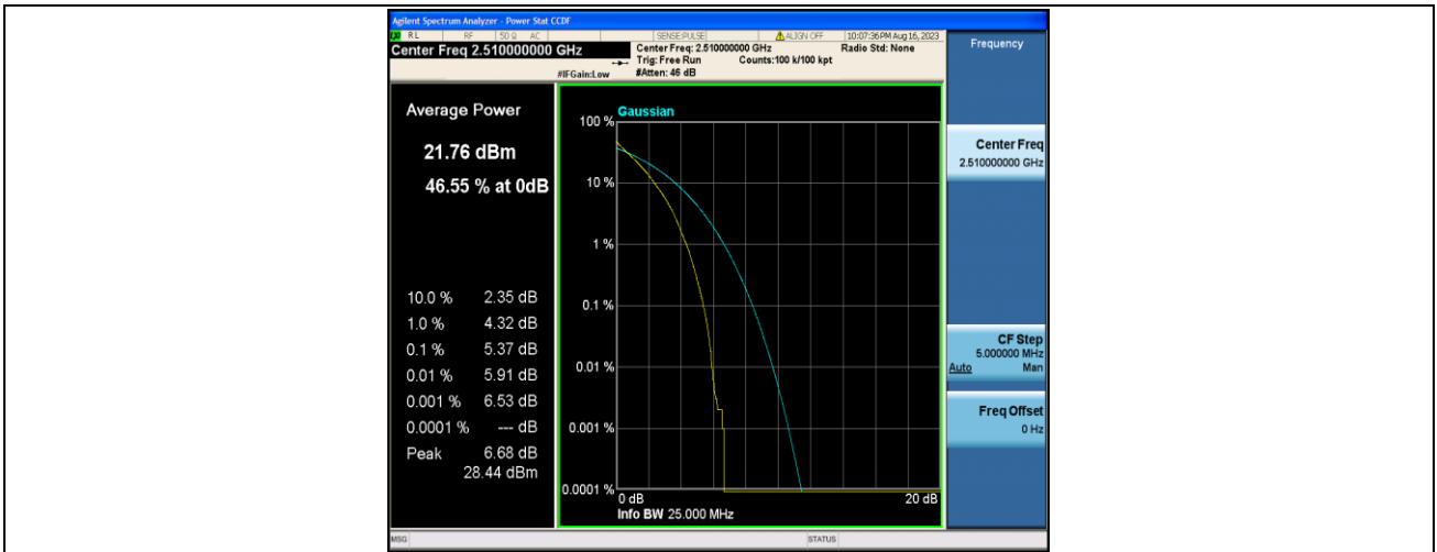
Band7-20MHz-QPSK-20850-100RB#0-PASS
