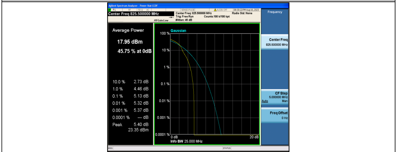
Band5-3MHz-16QAM-20415-1RB#0-PASS
