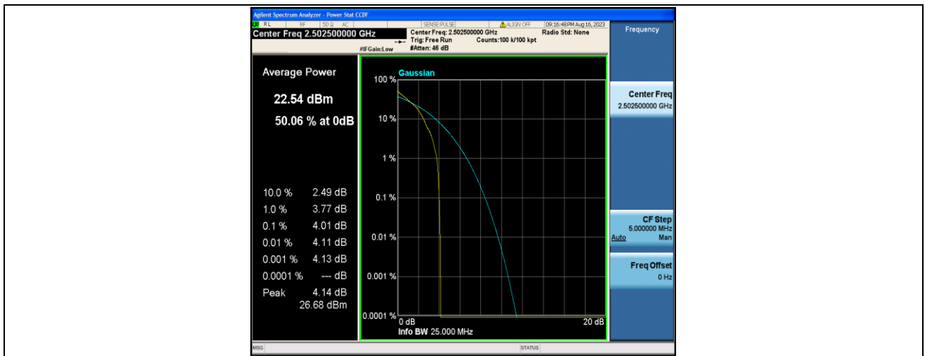
Band7-5MHz-QPSK-20775-1RB#0-PASS
