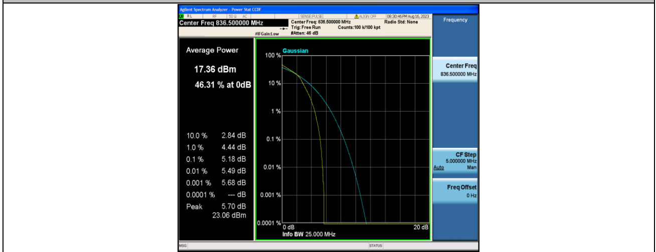
Band5-3MHz-16QAM-20525-15RB#0-PASS
