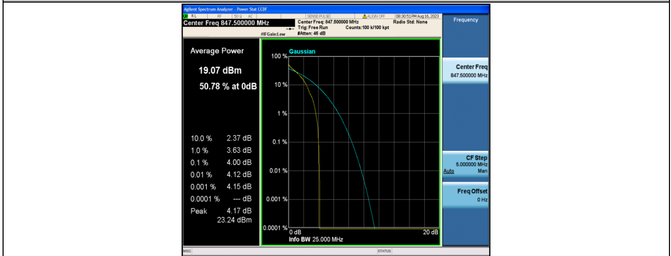
Band5-3MHz-QPSK-20635-1RB#0-PASS
