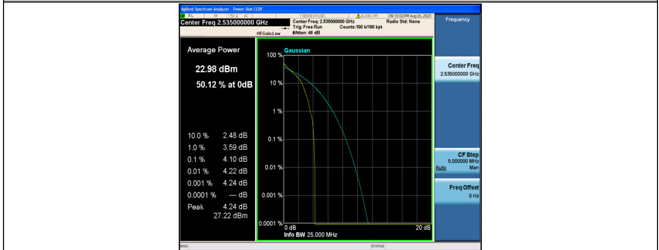
Band7-10MHz-QPSK-21100-1RB#0-PASS
