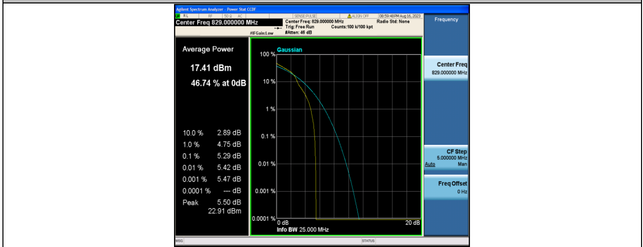
Band5-10MHz-16QAM-20450-1RB#0-PASS
