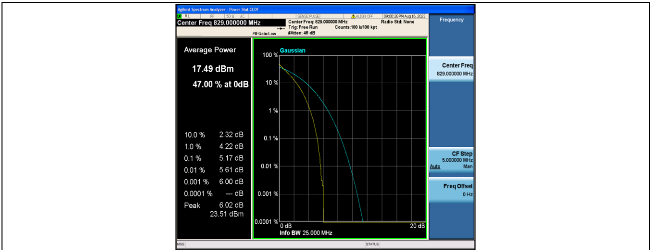
Band5-10MHz-QPSK-20450-50RB#0-PASS
