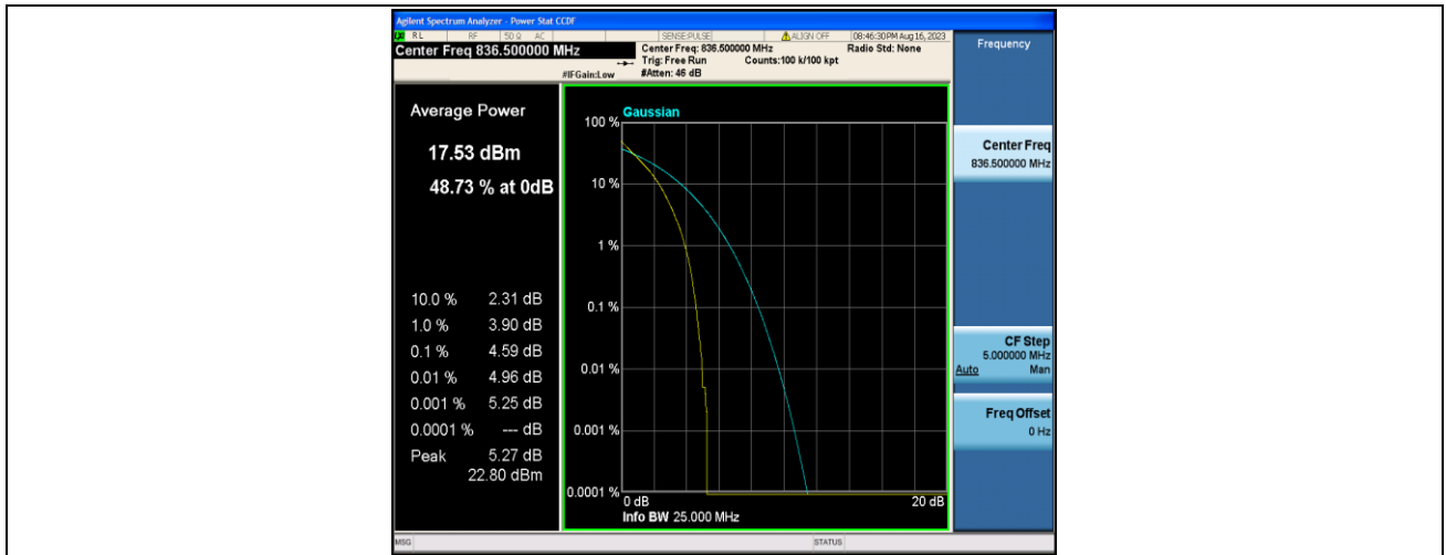
Band5-5MHz-QPSK-20525-25RB#0-PASS
