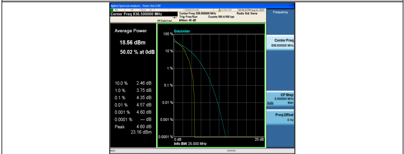
Band5-5MHz-QPSK-20525-1RB#0-PASS
