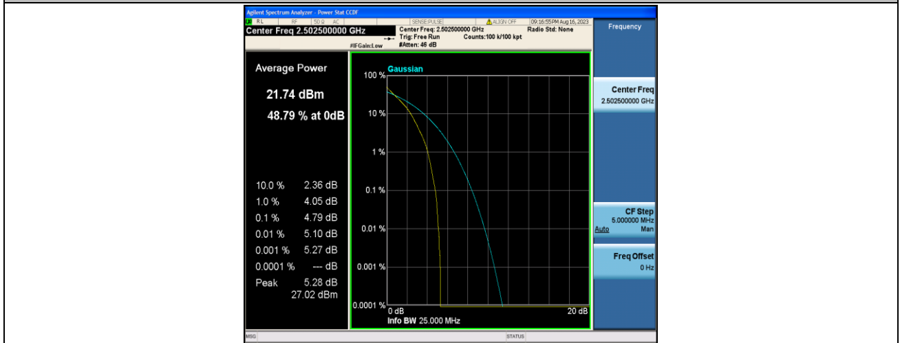
Band7-5MHz-QPSK-20775-25RB#0-PASS
