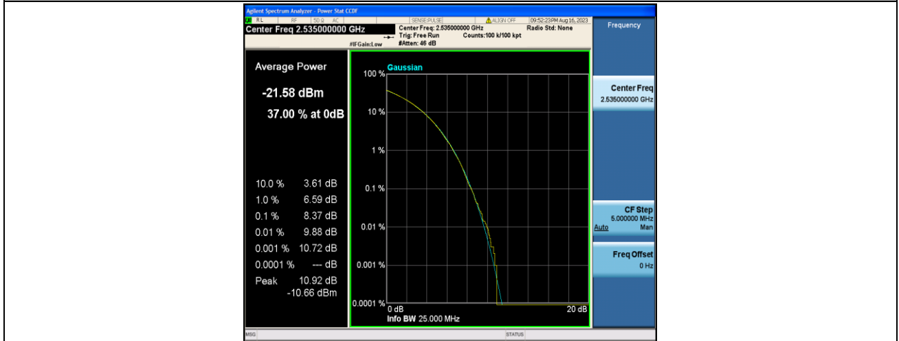
Band7-15MHz-QPSK-21100-1RB#0-PASS
