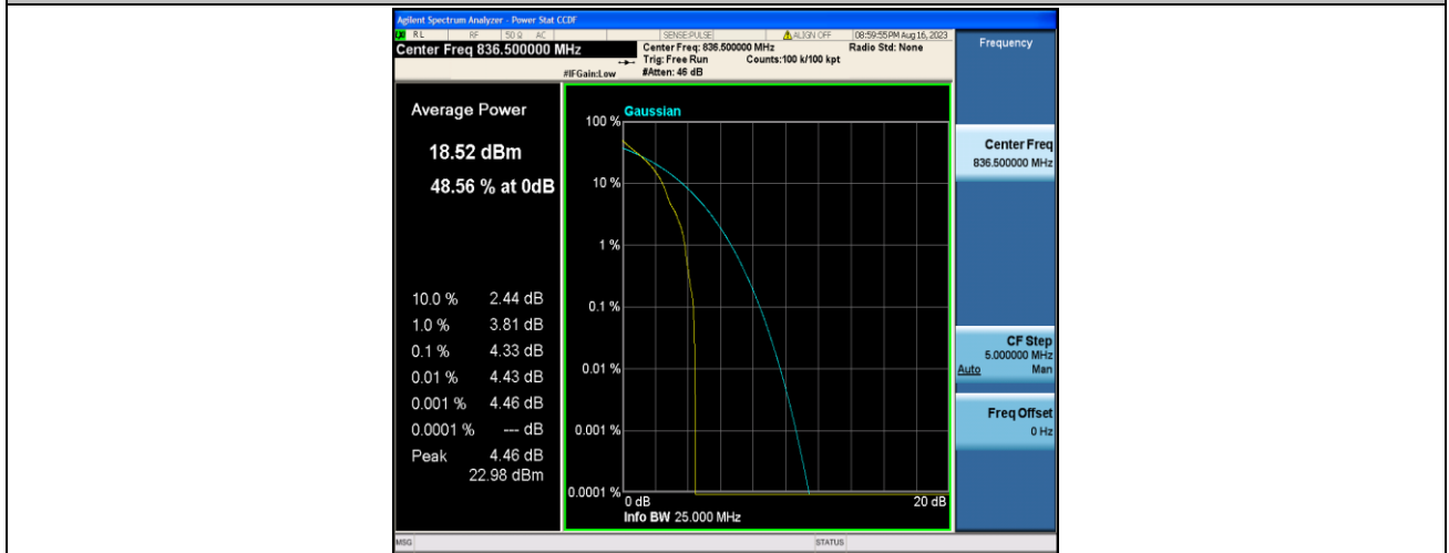
Band5-10MHz-QPSK-20525-1RB#0-PASS
