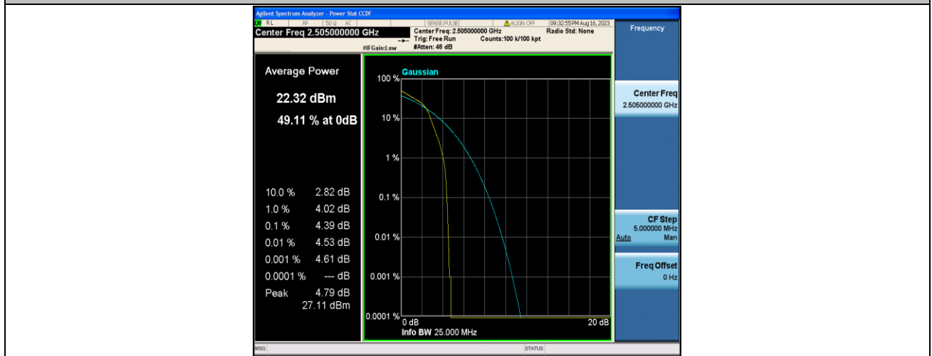
Band7-10MHz-16QAM-20800-1RB#0-PASS
