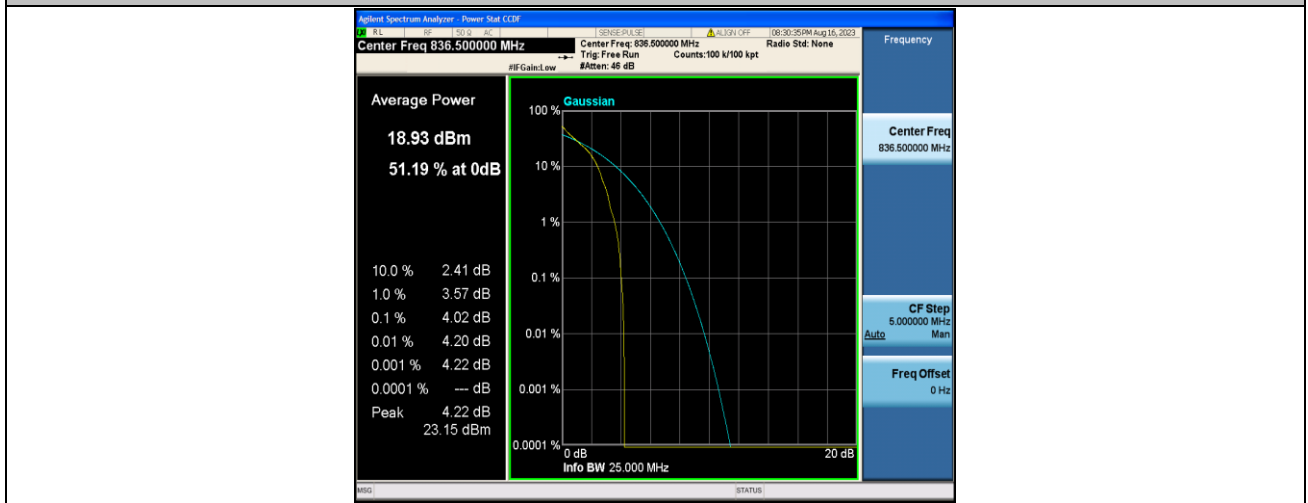
Band5-3MHz-QPSK-20525-1RB#0-PASS
