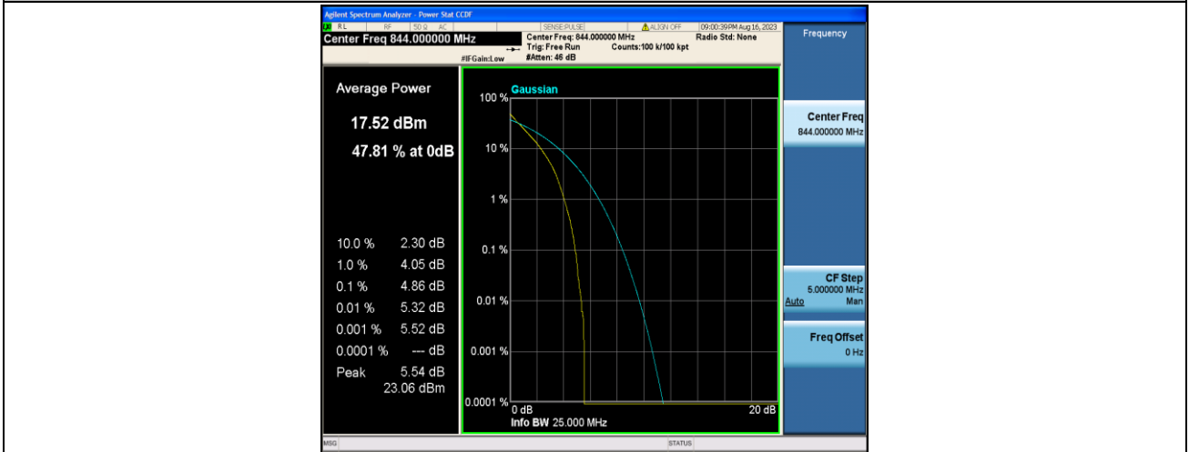
Band5-10MHz-QPSK-20600-50RB#0-PASS
