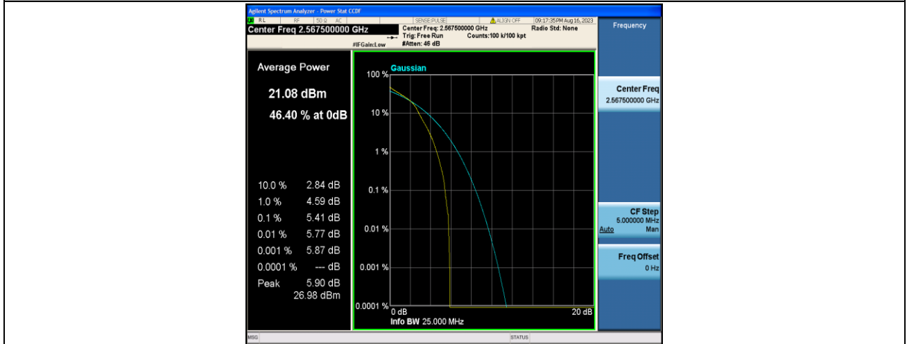
Band7-5MHz-16QAM-21425-25RB#0-PASS
