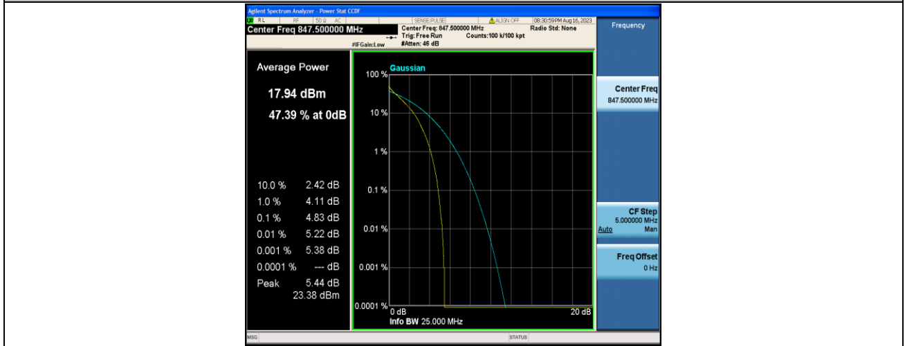
Band5-3MHz-QPSK-20635-15RB#0-PASS
