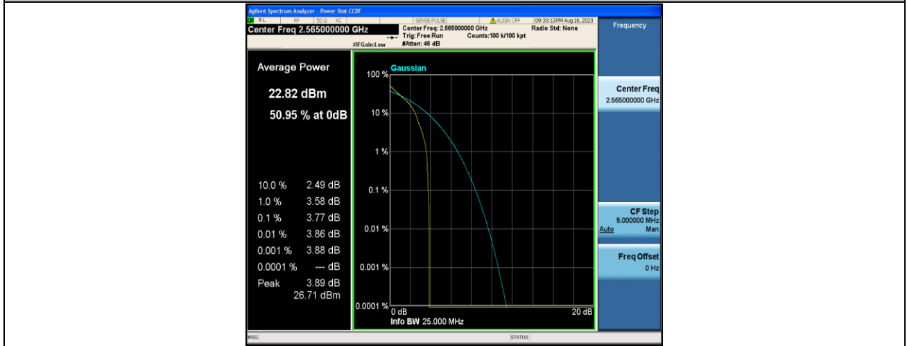
Band7-10MHz-QPSK-21400-1RB#0-PASS
