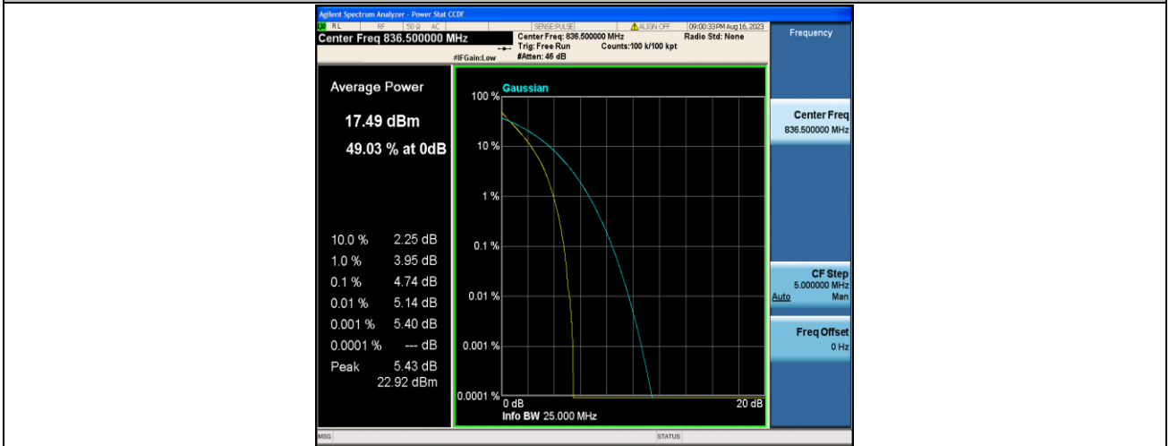
Band5-10MHz-QPSK-20525-50RB#0-PASS
