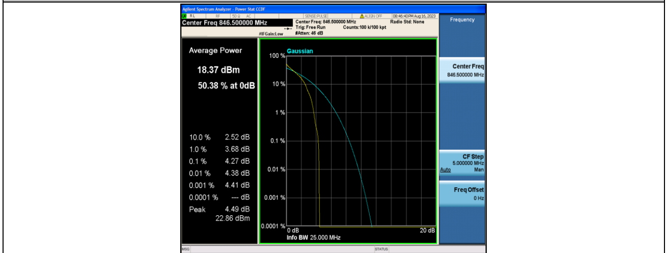
Band5-5MHz-QPSK-20625-1RB#0-PASS
