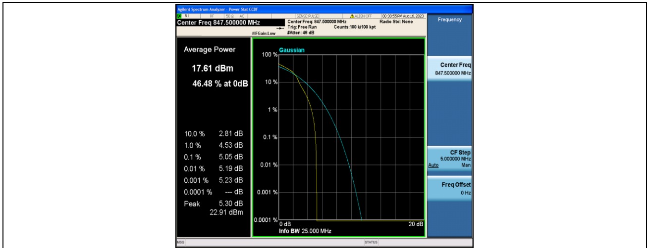
Band5-3MHz-16QAM-20635-1RB#0-PASS
