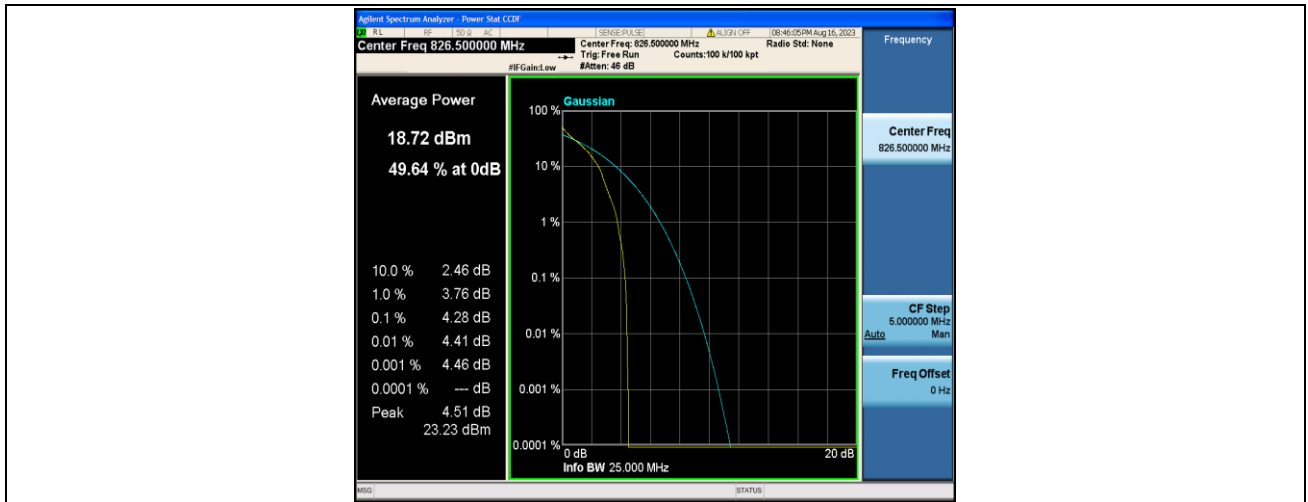
Band5-5MHz-QPSK-20425-1RB#0-PASS
