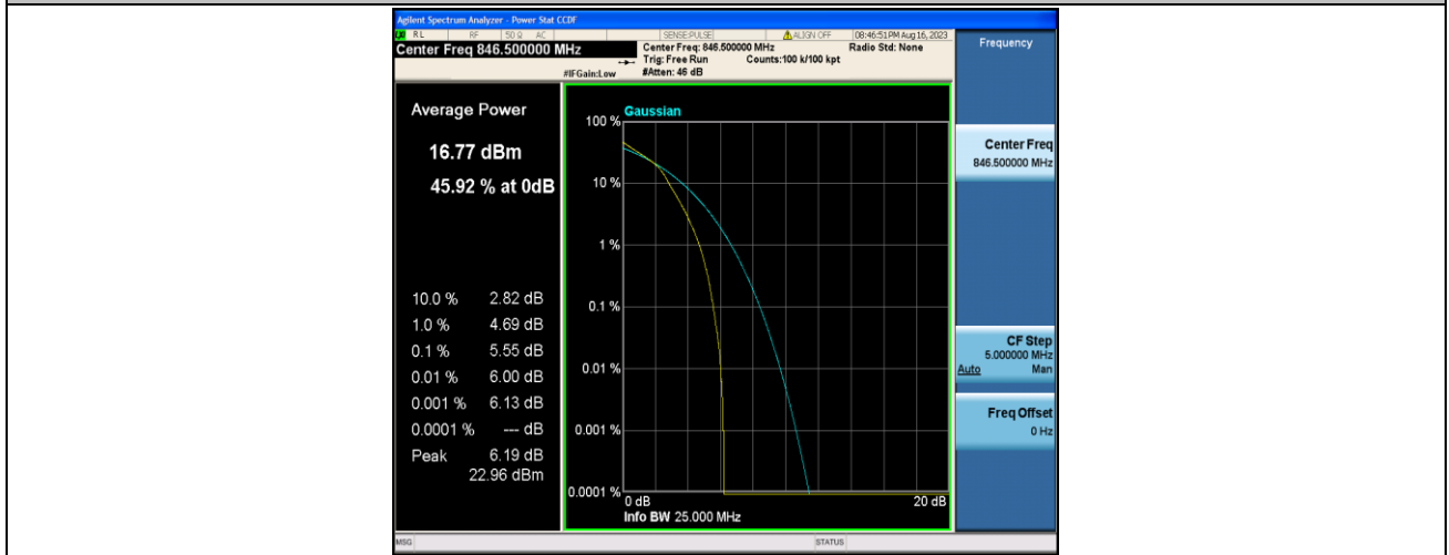
Band5-5MHz-16QAM-20625-25RB#0-PASS
