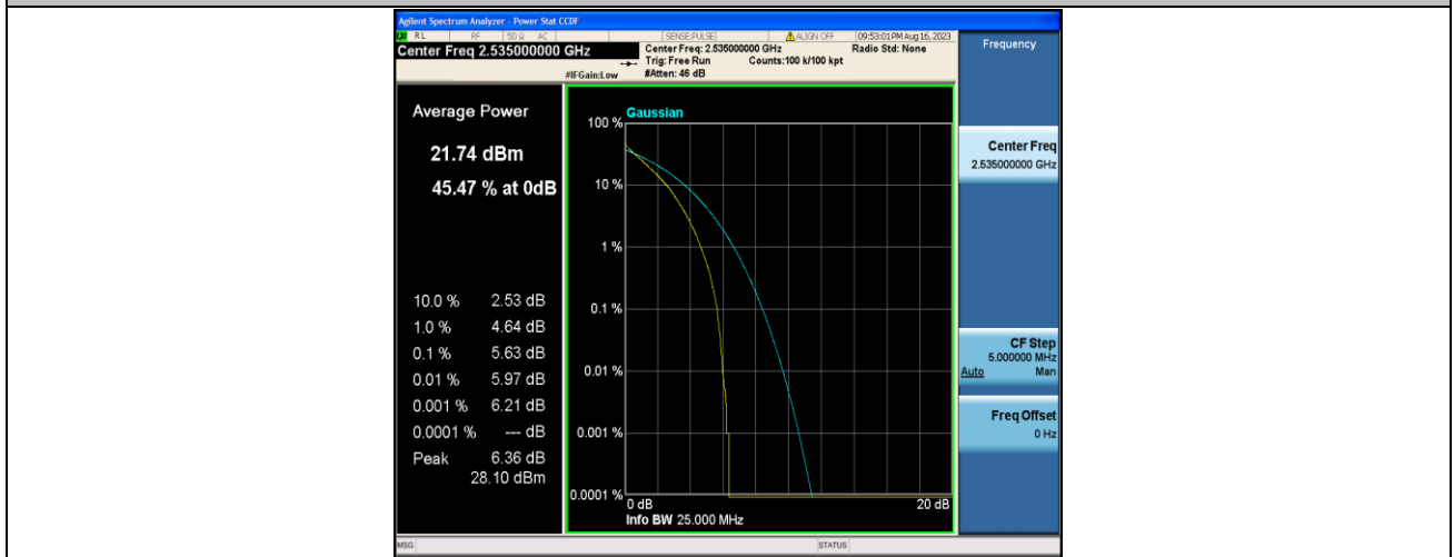
Band7-15MHz-QPSK-21100-75RB#0-PASS
