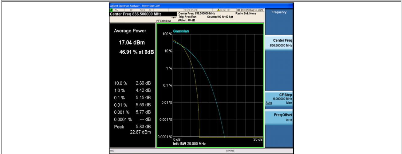
Band5-5MHz-16QAM-20525-25RB#0-PASS
