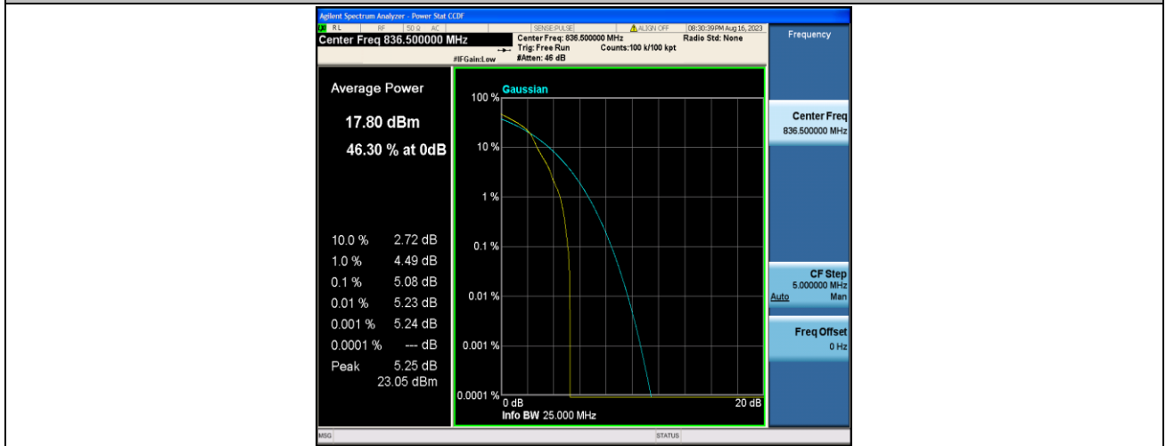
Band5-3MHz-16QAM-20525-1RB#0-PASS
