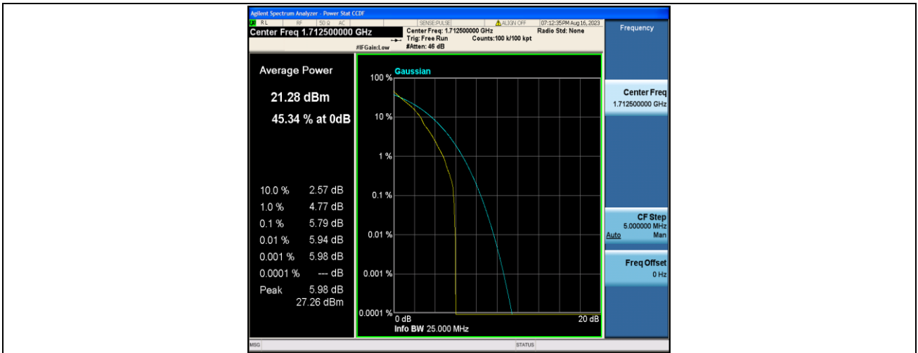
Band4-5MHz-QPSK-19975-1RB#0-PASS
