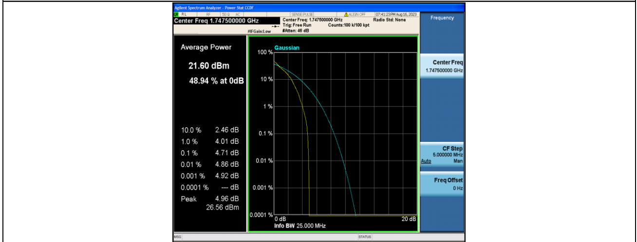
Band4-15MHz-QPSK-20325-1RB#0-PASS
