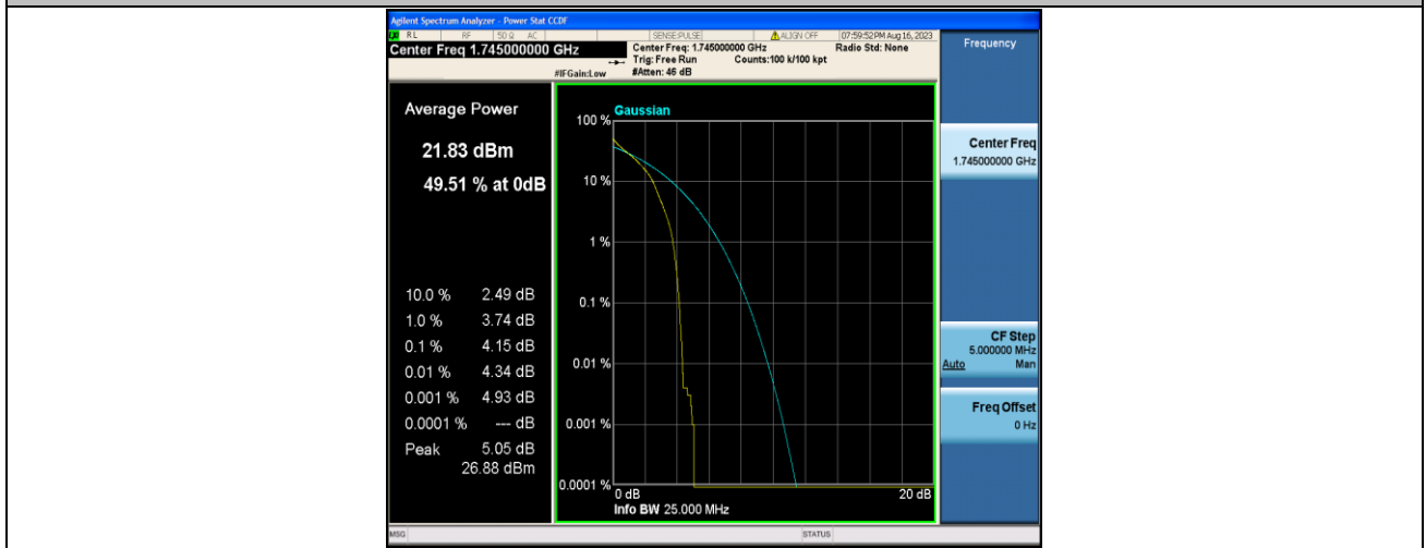
Band4-20MHz-QPSK-20300-1RB#0-PASS
