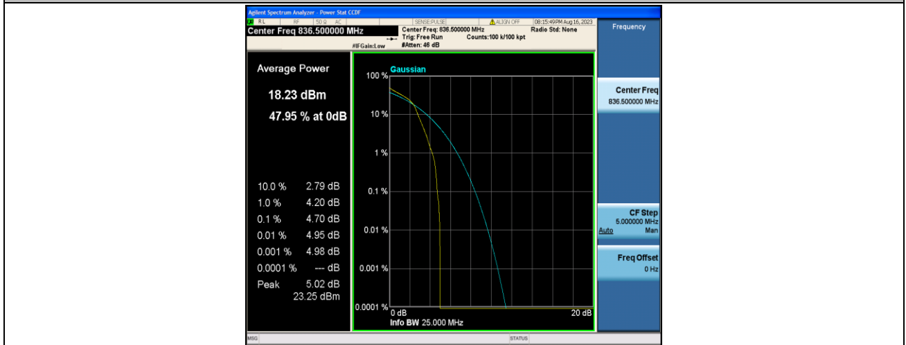
Band5-1.4MHz-16QAM-20525-1RB#0-PASS
