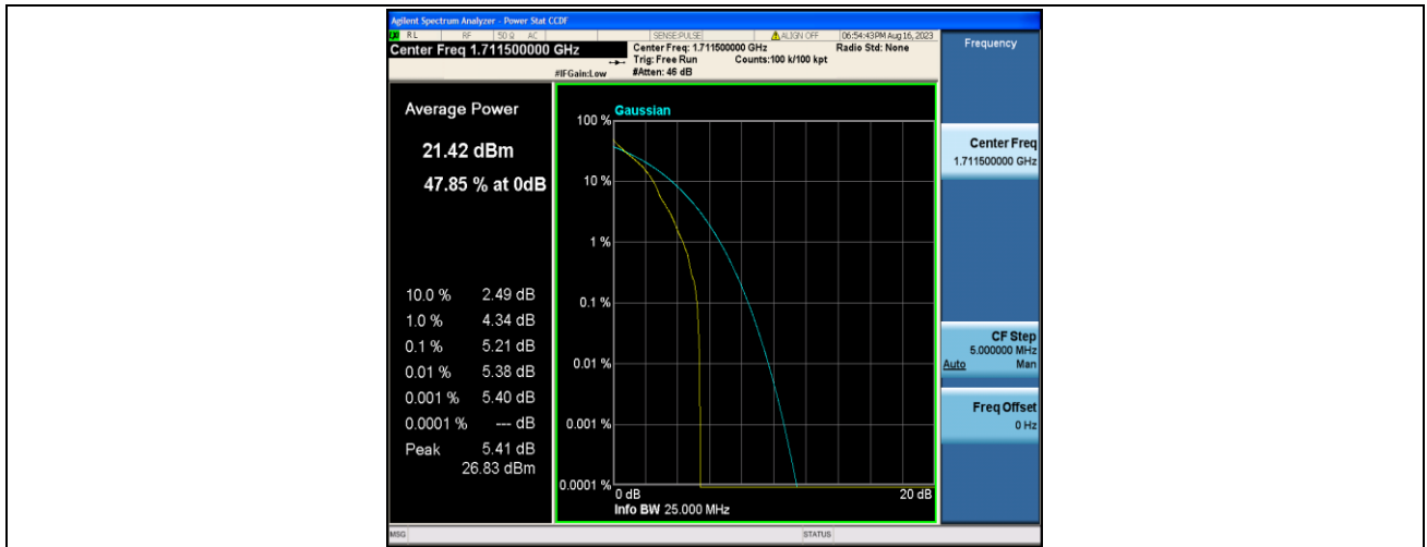
Band4-3MHz-QPSK-19965-1RB#0-PASS
