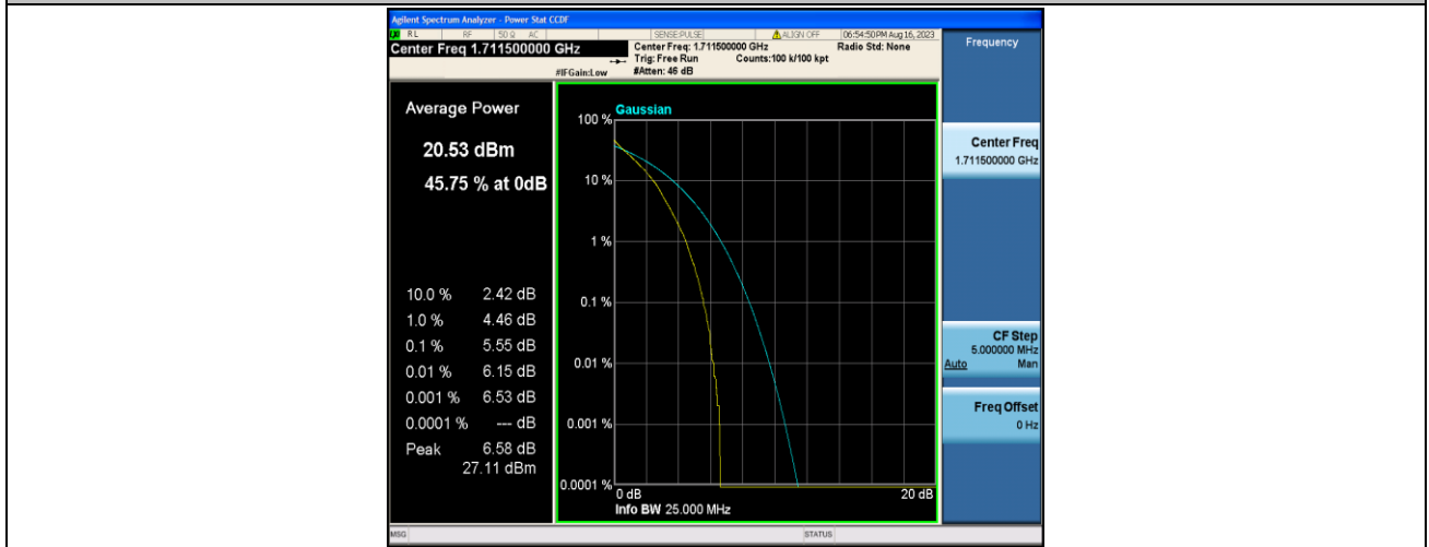
Band4-3MHz-QPSK-19965-15RB#0-PASS
