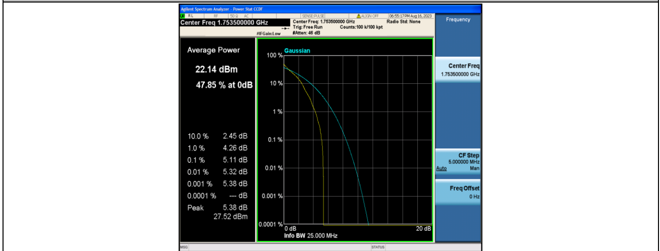
Band4-3MHz-QPSK-20385-1RB#0-PASS
