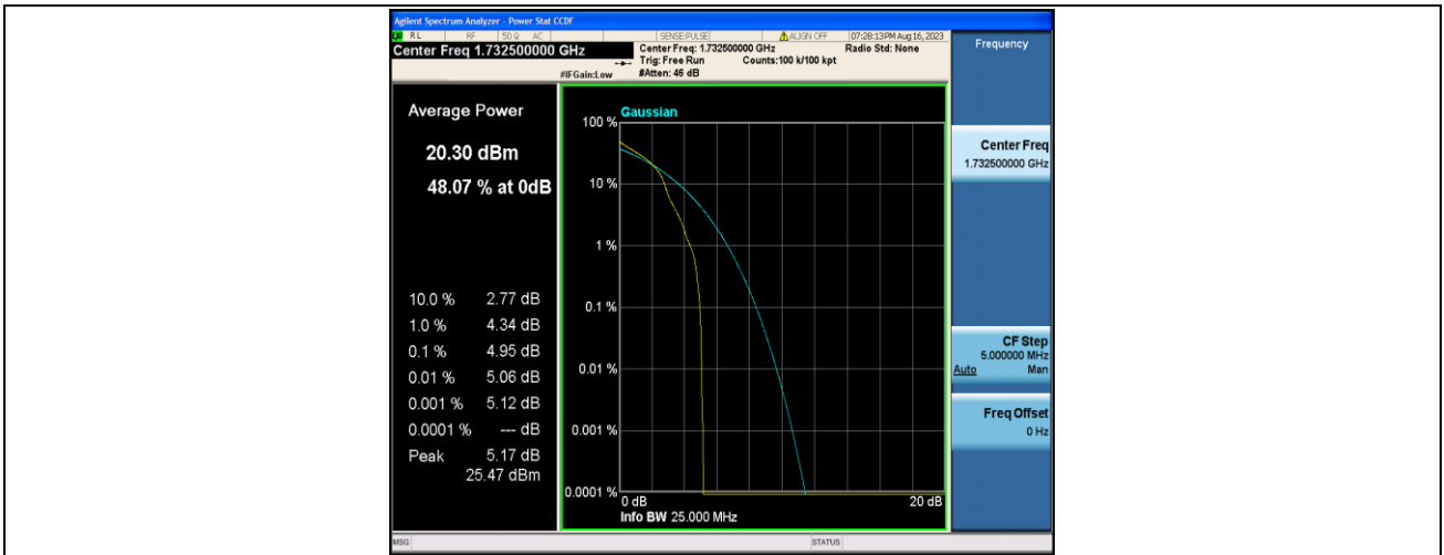
Band4-10MHz-16QAM-20175-1RB#0-PASS
