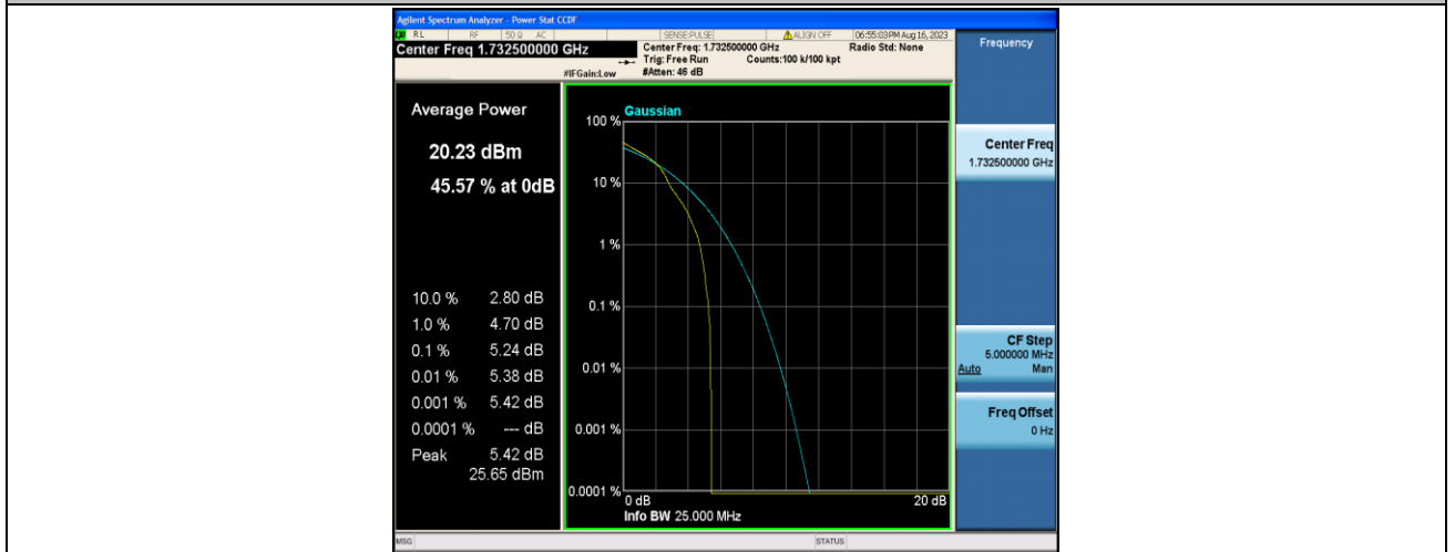
Band4-3MHz-16QAM-20175-1RB#0-PASS
