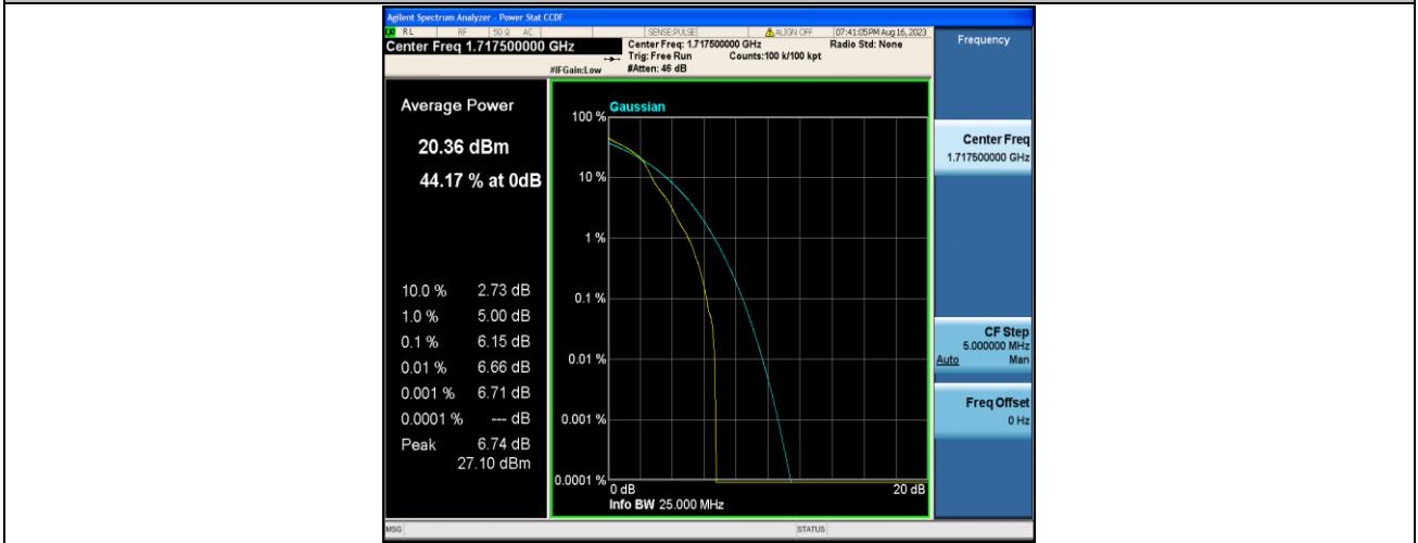
Band4-15MHz-16QAM-20025-1RB#0-PASS
