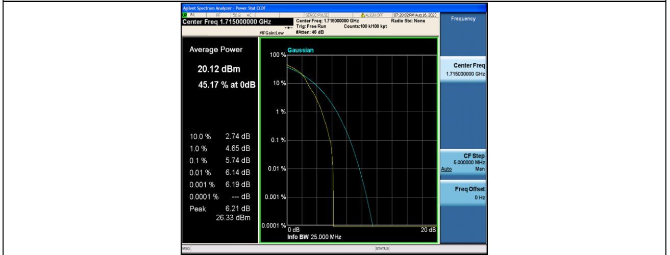
Band4-10MHz-16QAM-20000-1RB#0-PASS
