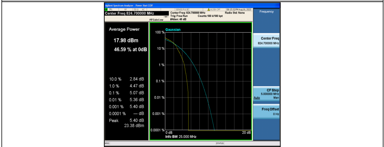
Band5-1.4MHz-16QAM-20407-1RB#0-PASS
