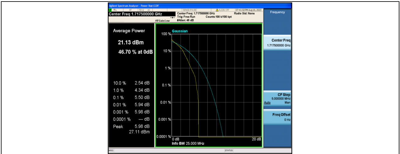
Band4-15MHz-QPSK-20025-1RB#0-PASS
