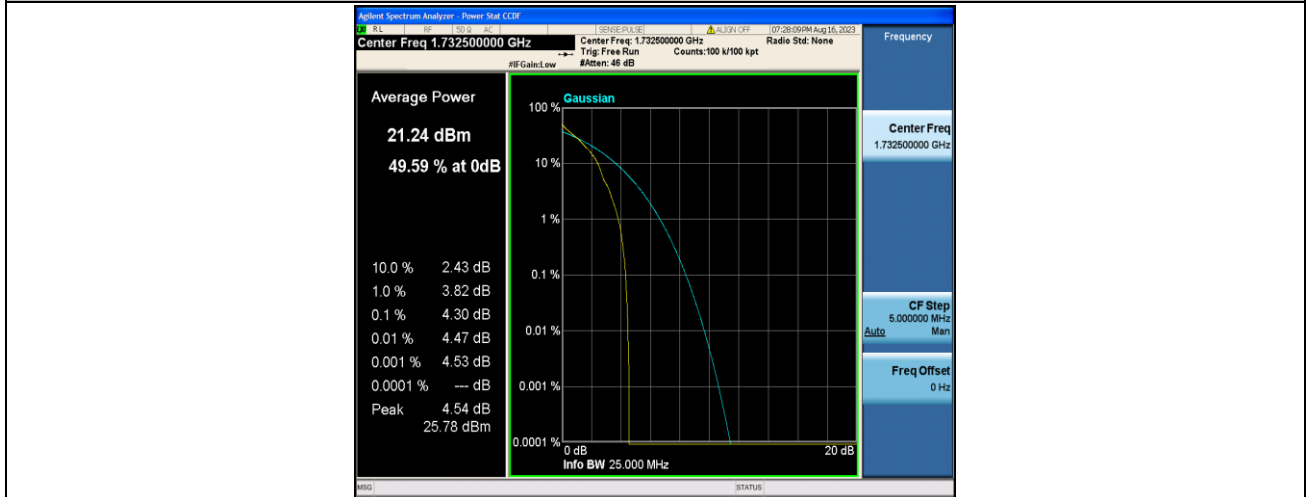
Band4-10MHz-QPSK-20175-1RB#0-PASS
