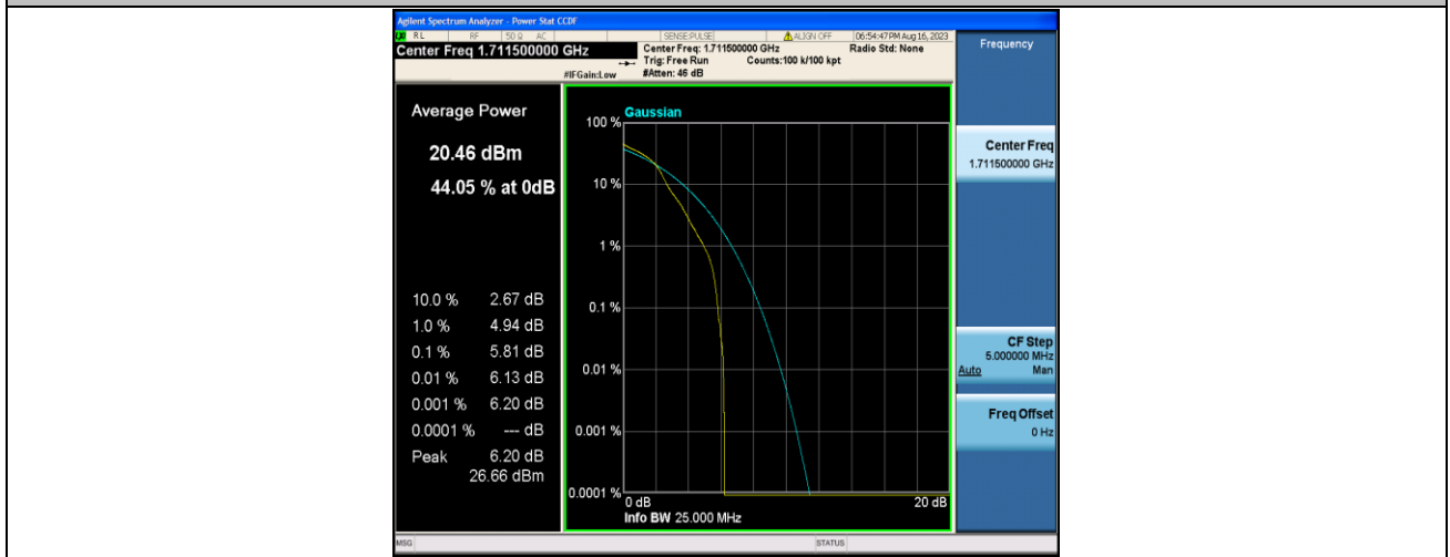
Band4-3MHz-16QAM-19965-1RB#0-PASS
