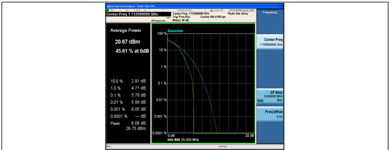
Band4-20MHz-16QAM-20175-1RB#0-PASS
