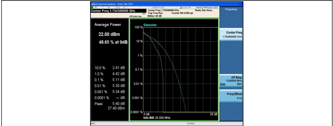
Band4-1.4MHz-QPSK-20393-1RB#0-PASS
