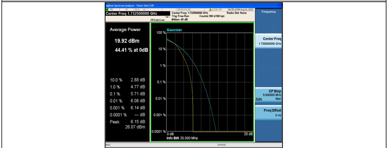
Band4-3MHz-16QAM-20175-15RB#0-PASS
