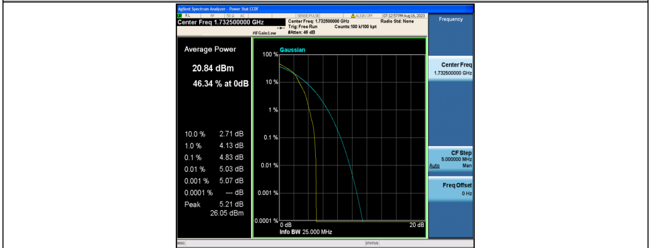
Band4-5MHz-16QAM-20175-1RB#0-PASS
