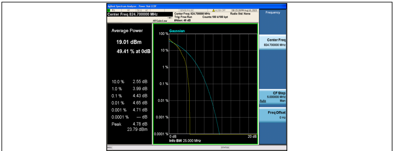
Band5-1.4MHz-QPSK-20407-1RB#0-PASS
