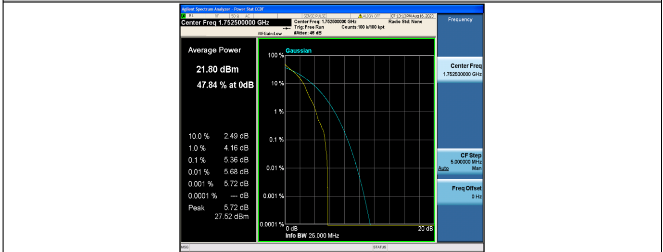
Band4-5MHz-QPSK-20375-1RB#0-PASS
