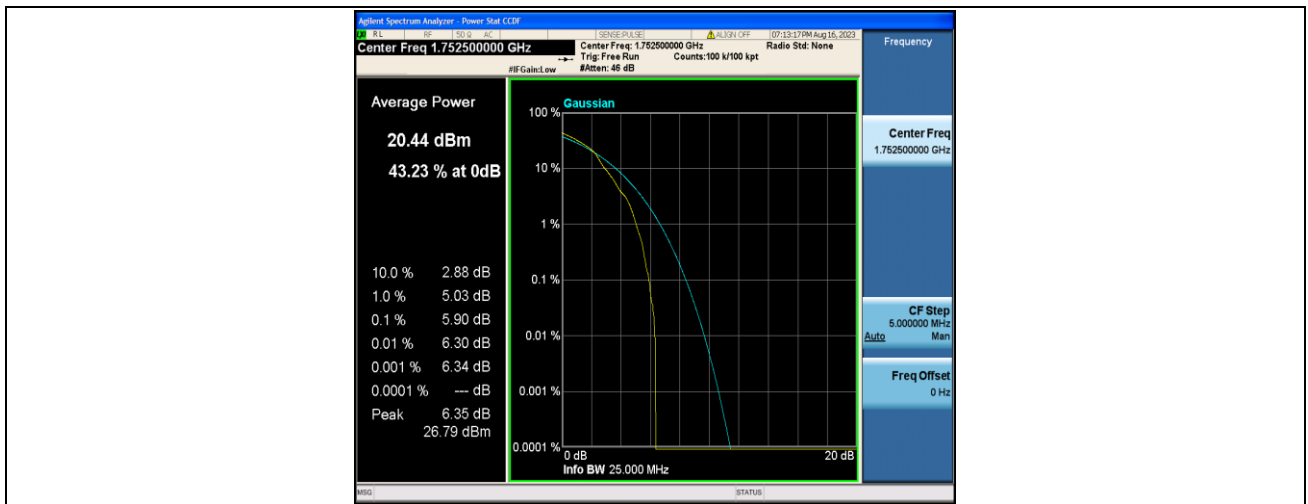
Band4-5MHz-16QAM-20375-1RB#0-PASS
