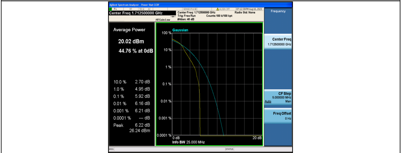
Band4-5MHz-16QAM-19975-1RB#0-PASS
