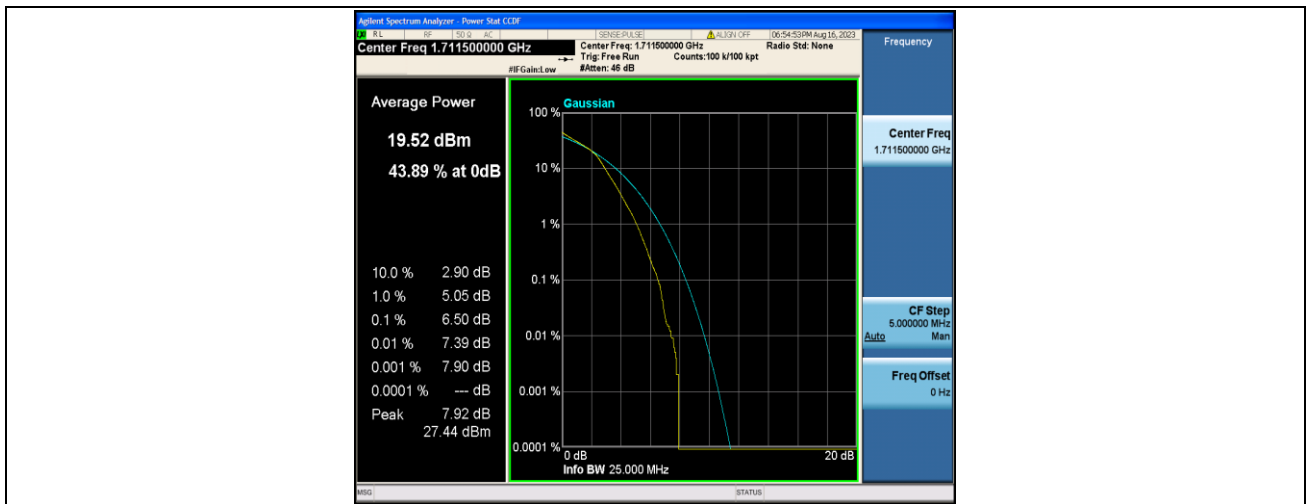
Band4-3MHz-16QAM-19965-15RB#0-PASS
