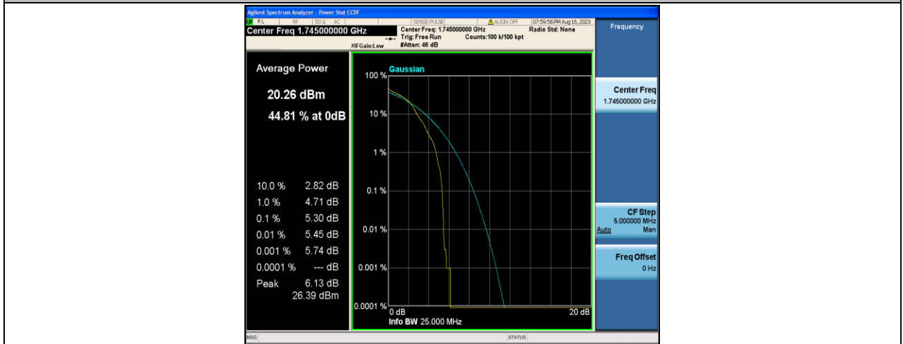
Band4-20MHz-16QAM-20300-1RB#0-PASS
