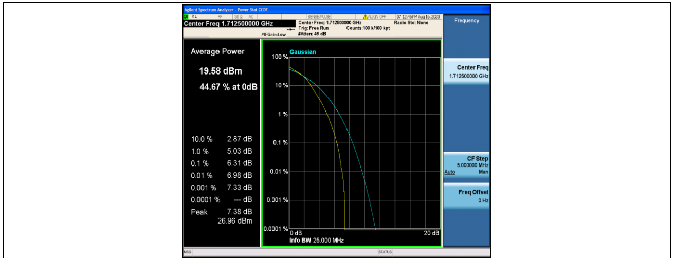
Band4-5MHz-16QAM-19975-25RB#0-PASS
