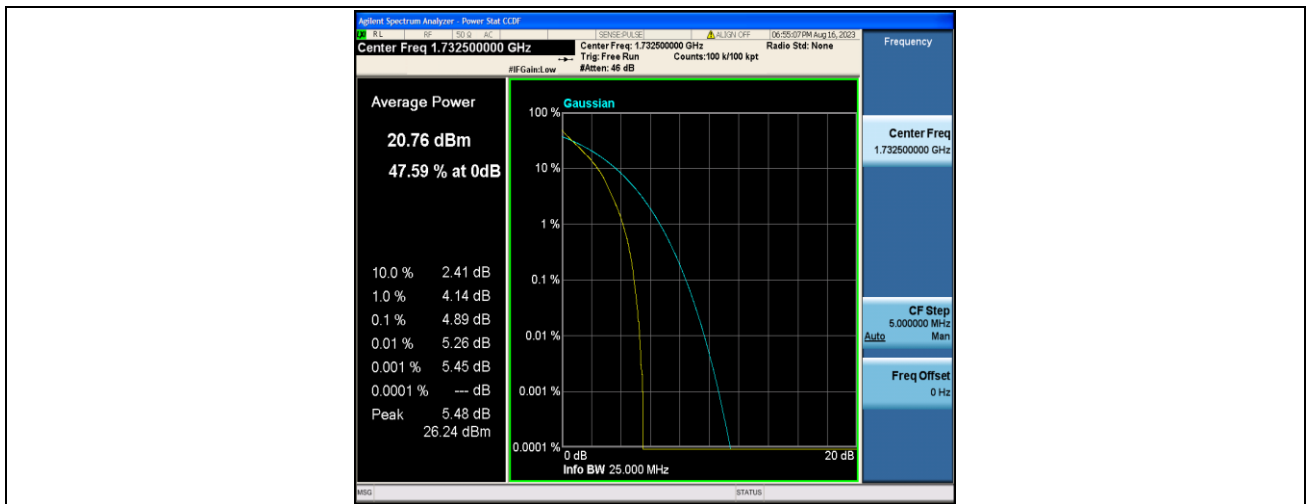
Band4-3MHz-QPSK-20175-15RB#0-PASS
