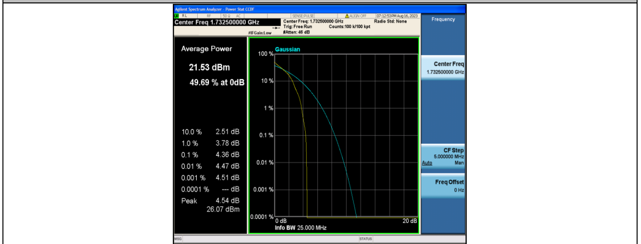
Band4-5MHz-QPSK-20175-1RB#0-PASS
