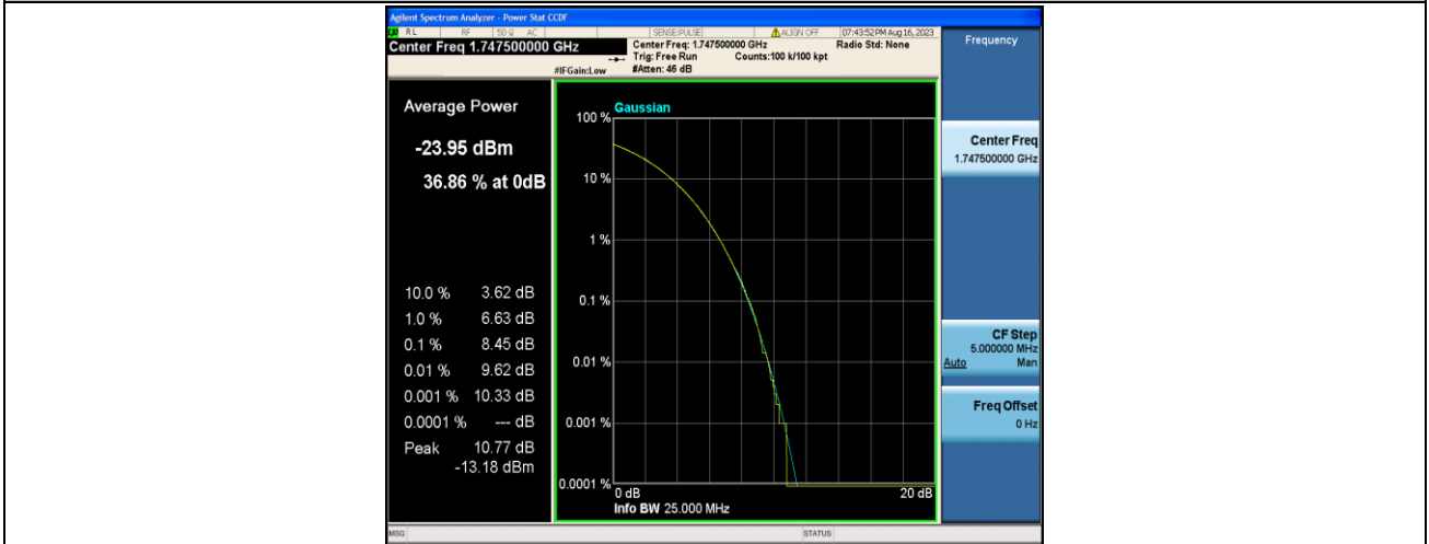
Band4-15MHz-QPSK-20325-75RB#0-PASS
