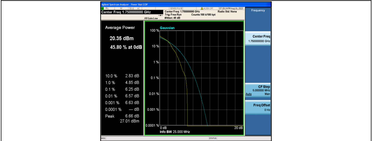
Band4-10MHz-16QAM-20350-1RB#0-PASS
