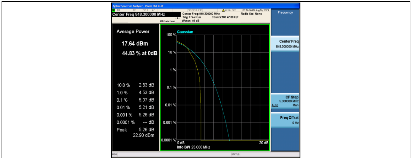
Band5-1.4MHz-16QAM-20643-1RB#0-PASS
