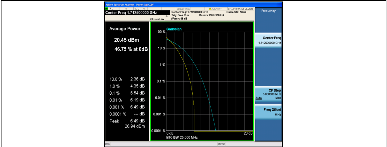
Band4-5MHz-QPSK-19975-25RB#0-PASS
