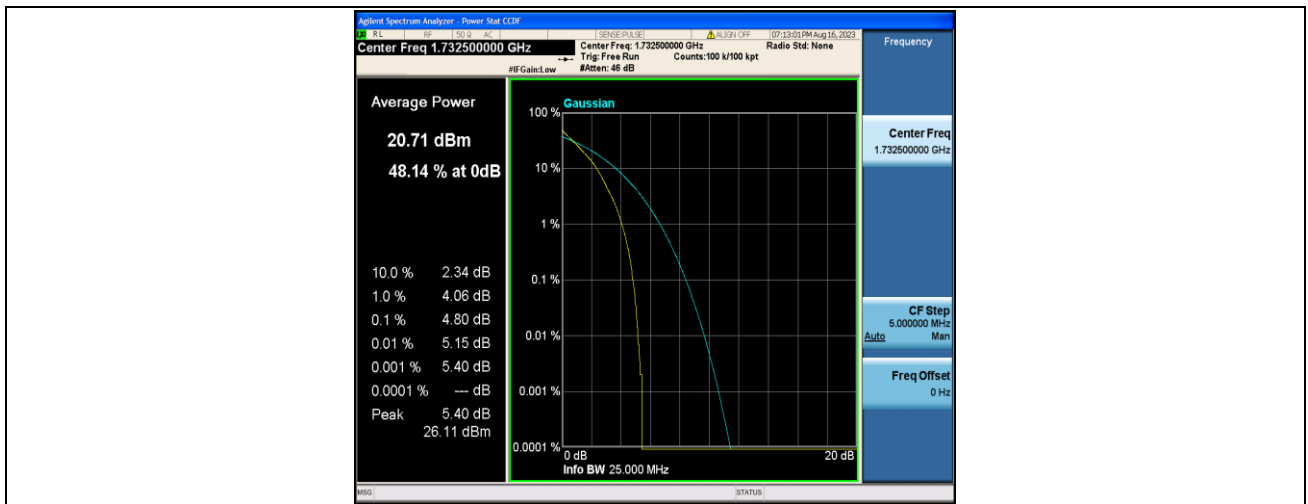
Band4-5MHz-QPSK-20175-25RB#0-PASS
