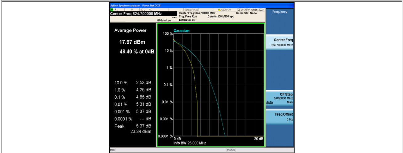
Band5-1.4MHz-QPSK-20407-6RB#0-PASS
