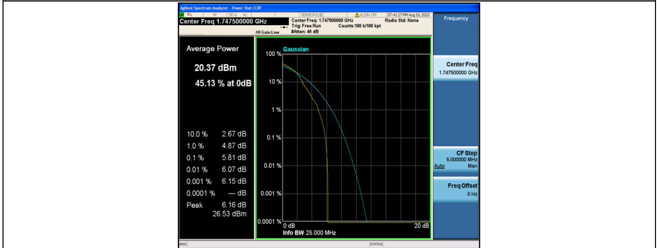
Band4-15MHz-16QAM-20325-1RB#0-PASS
