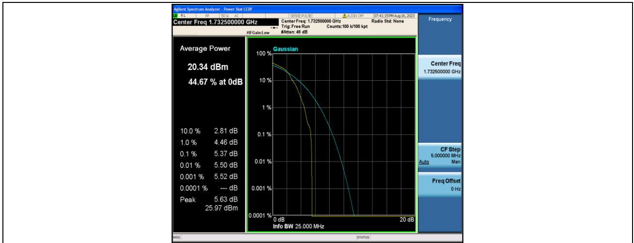
Band4-15MHz-16QAM-20175-1RB#0-PASS
