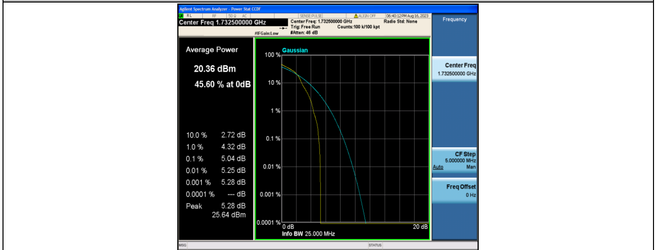
Band4-1.4MHz-16QAM-20175-1RB#0-PASS
