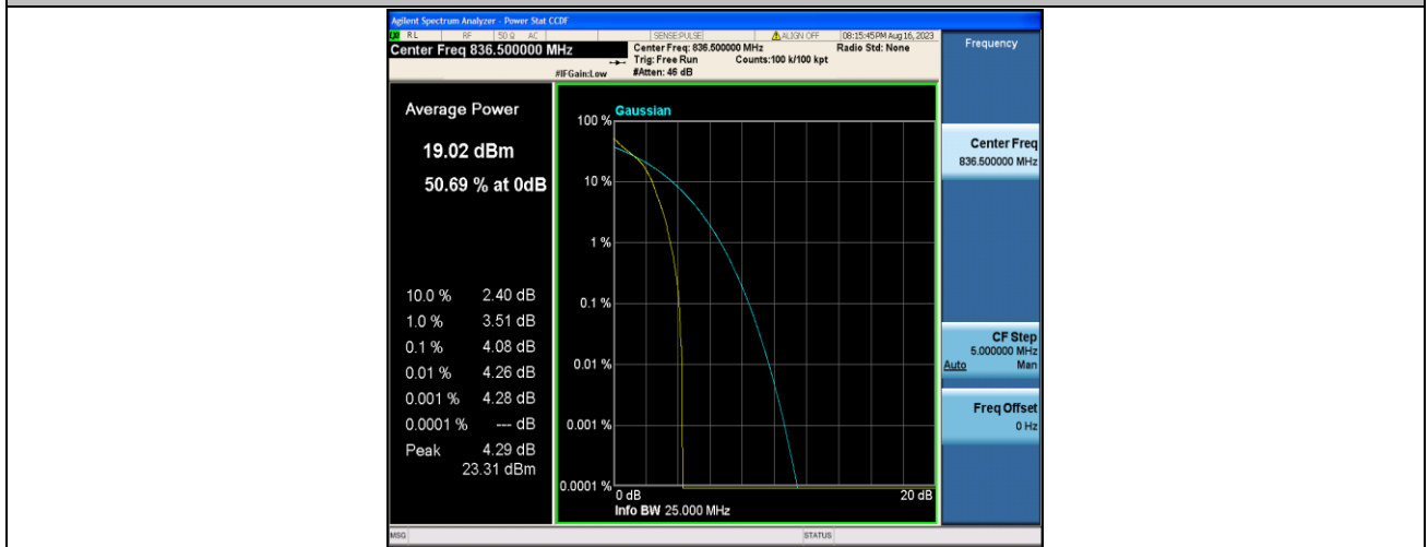
Band5-1.4MHz-QPSK-20525-1RB#0-PASS
