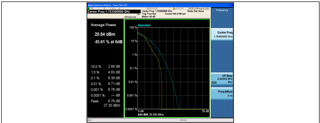
Band4-3MHz-16QAM-20385-1RB#0-PASS
