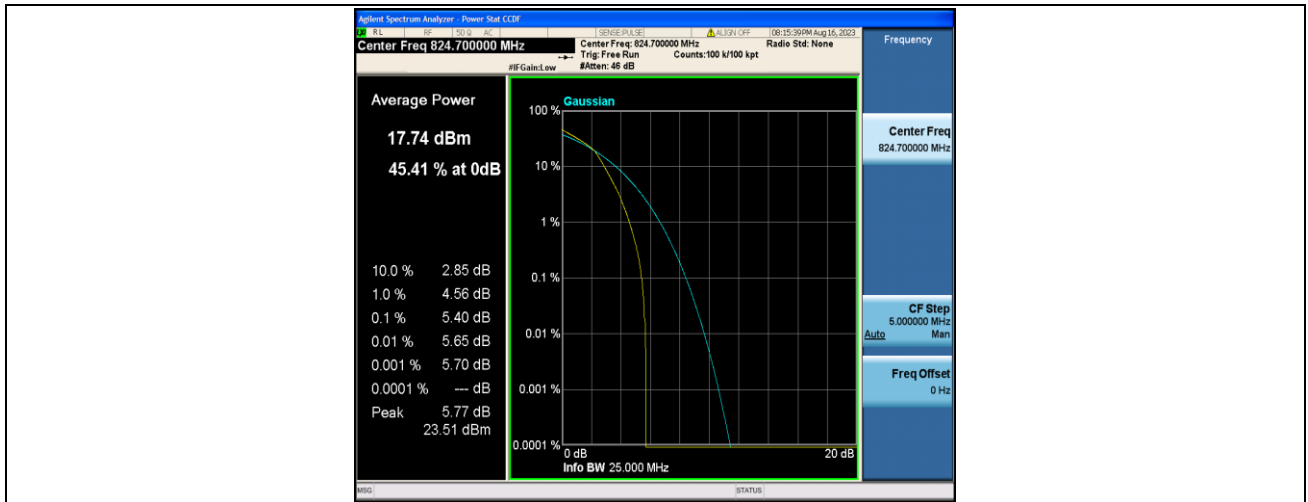
Band5-1.4MHz-16QAM-20407-6RB#0-PASS
