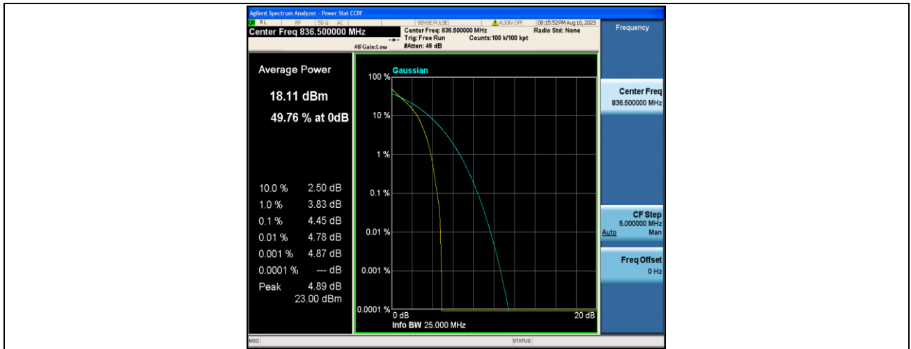
Band5-1.4MHz-QPSK-20525-6RB#0-PASS
