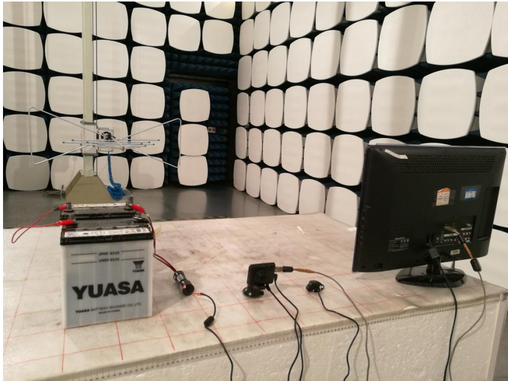
Radiated Emission (For DC 24V) Below 1GHz
