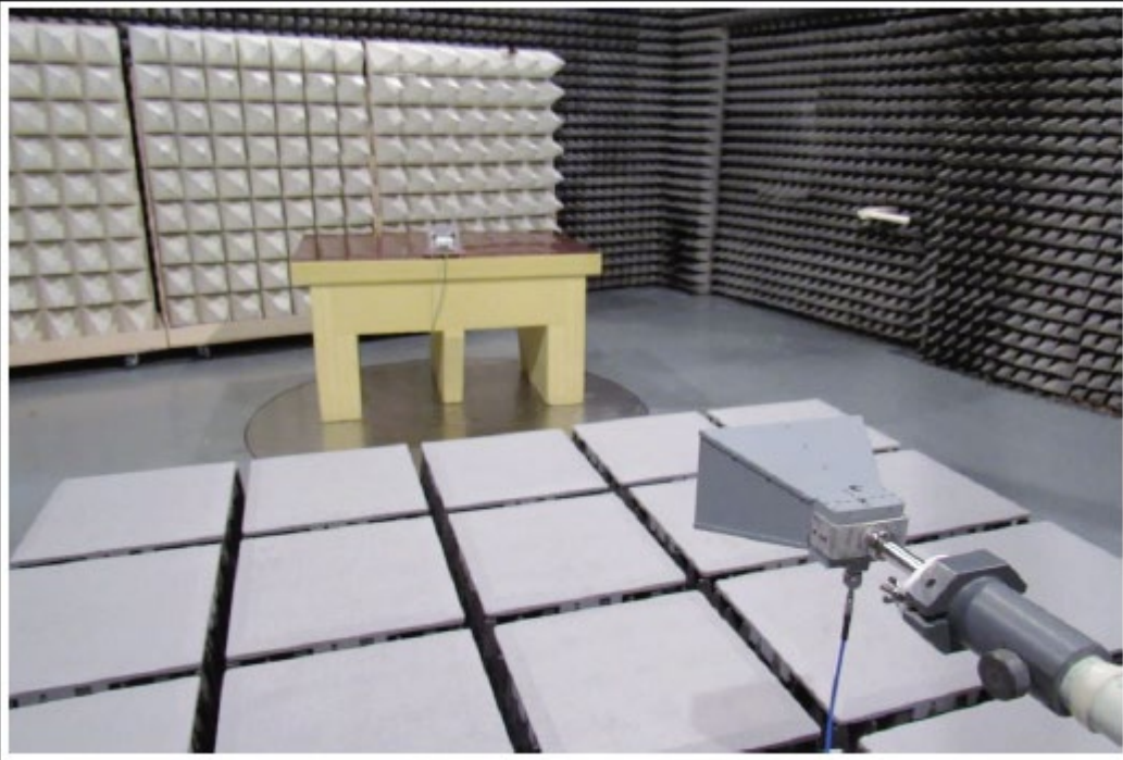
TEST SETUP 3 RADIATED EMISSION
