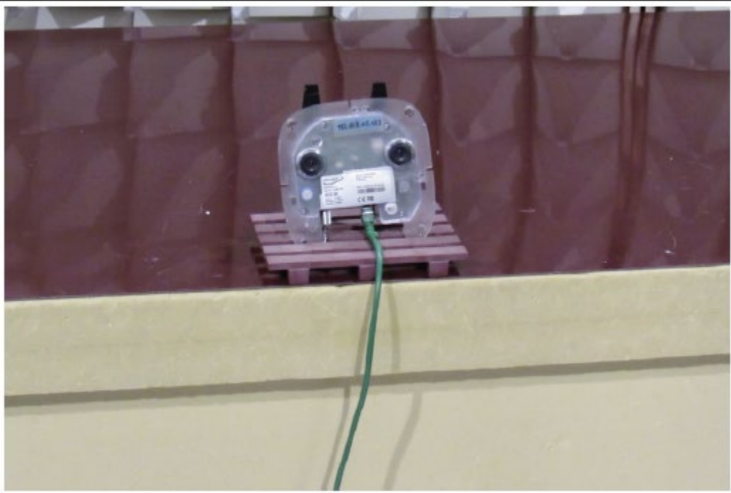
TEST SETUP FOCUS RADIATED EMISSION
