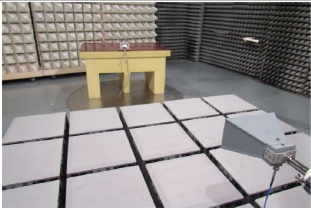
TEST SETUP-3 EUT CONFIGURATION-1 RE
