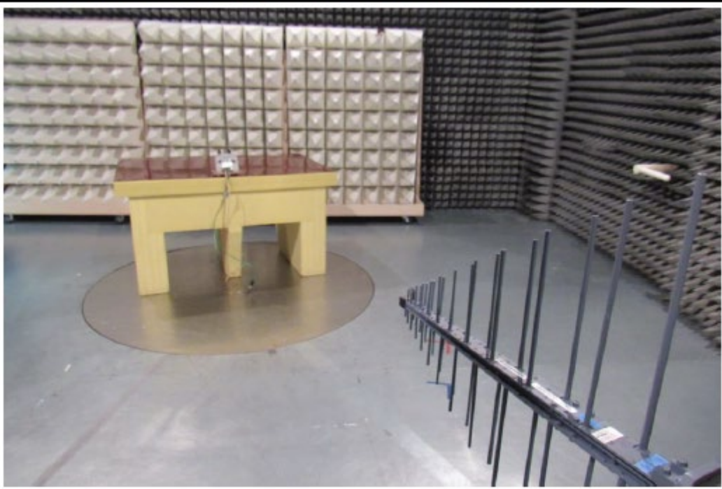
TEST SETUP-2 EUT CONFIGURATION-2 RADIATED EMISSION
