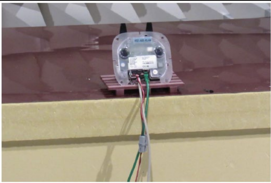
TEST SETUP FOCUS EUT CONFIGURATION-2 RE
