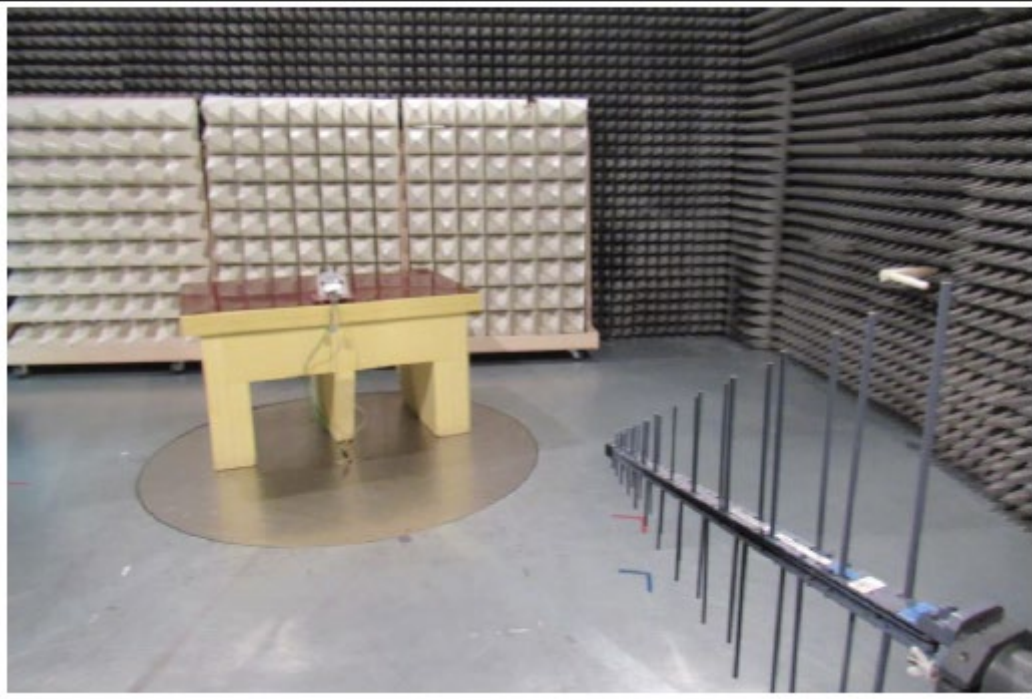
TEST SETUP-2 EUT CONFIGURATION-1 RE
