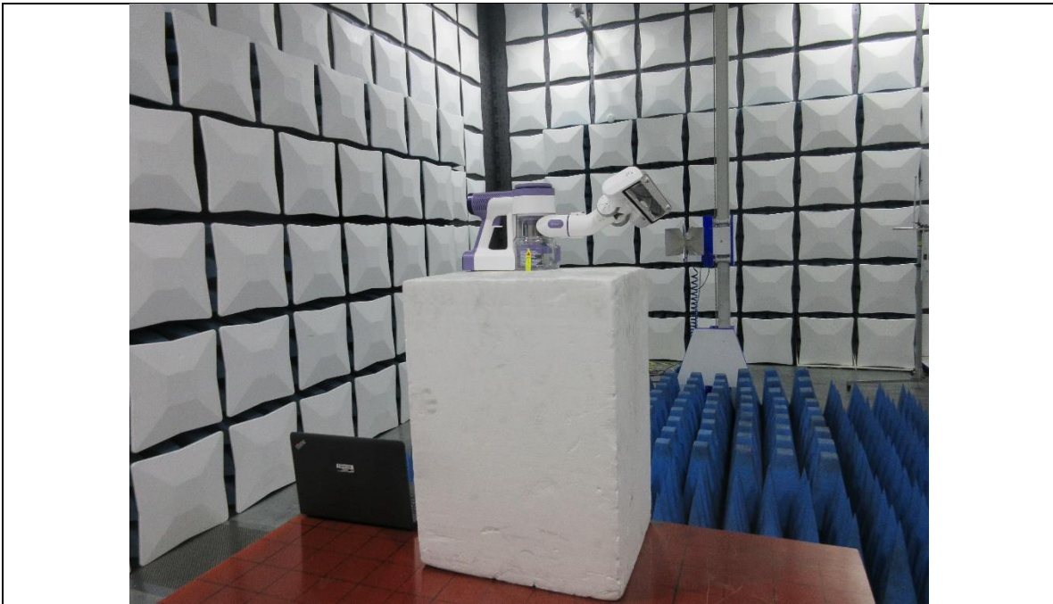
RADIATED RF MEASUREMENT SETUP (ABOVE 1 GHz- Y axis)
