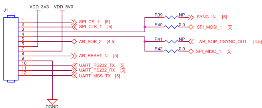
Figure 3. 12-Pin Header
