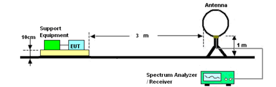
Below 30MHz
