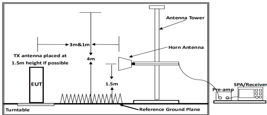
Above 1GHz
