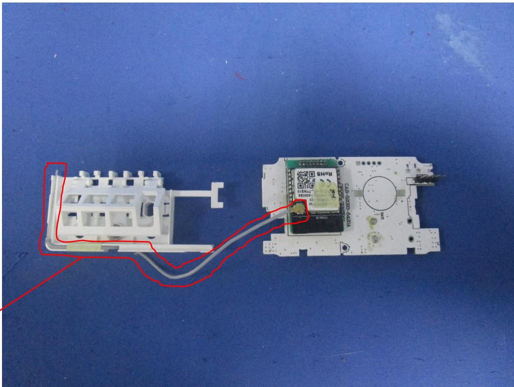
2.4G Wi-Fi Antenna
