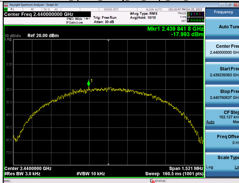
Power_Spectral_Density_BLE_1Mbps_2440_00
