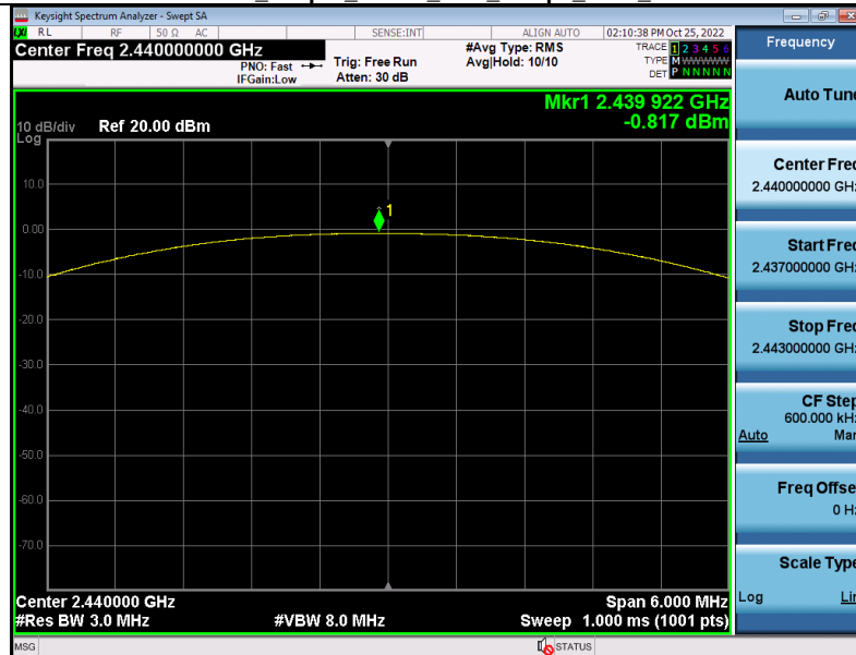
Peak_Output_Power_BLE_1Mbps_2440_00
