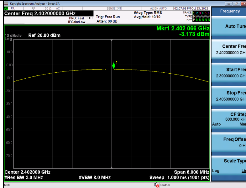
Peak_Output_Power_BLE_1Mbps_2402
