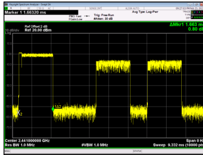
2441MHzDH3
