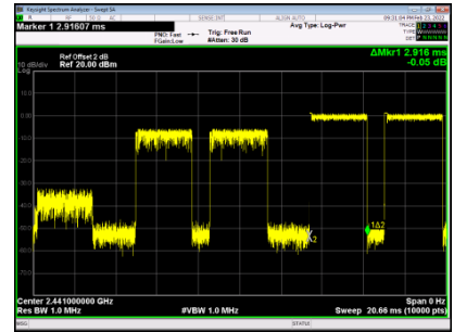
2441MHzDH5
