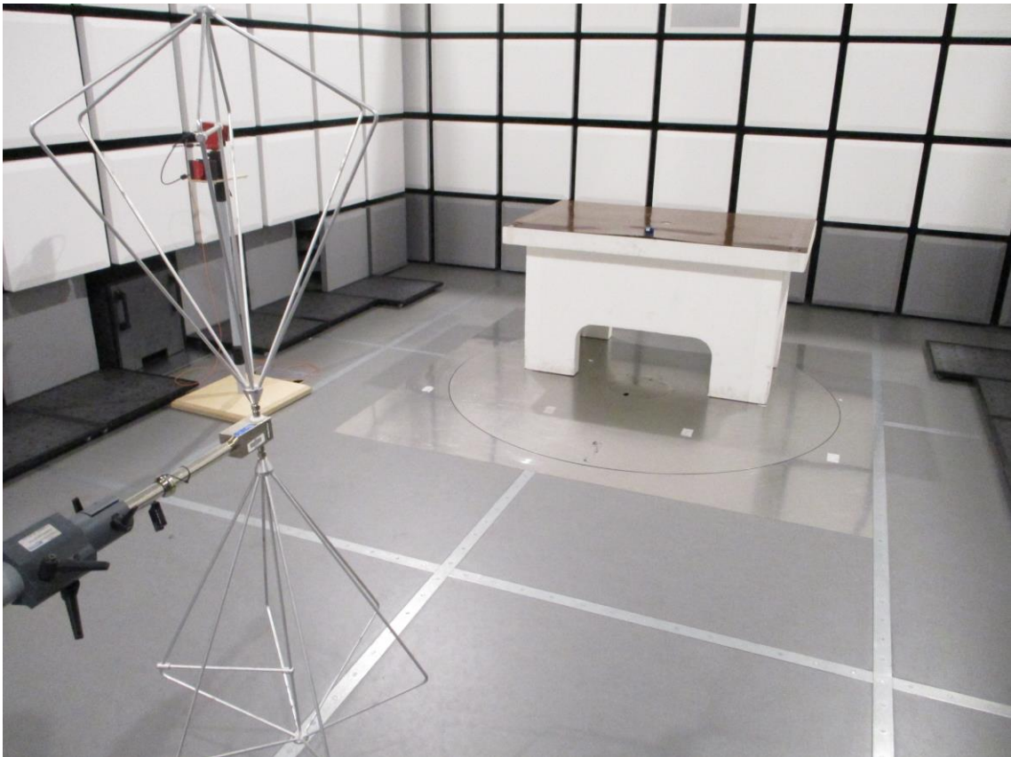
Figure 1: Spurious emission 30 MHz-200 MHz
