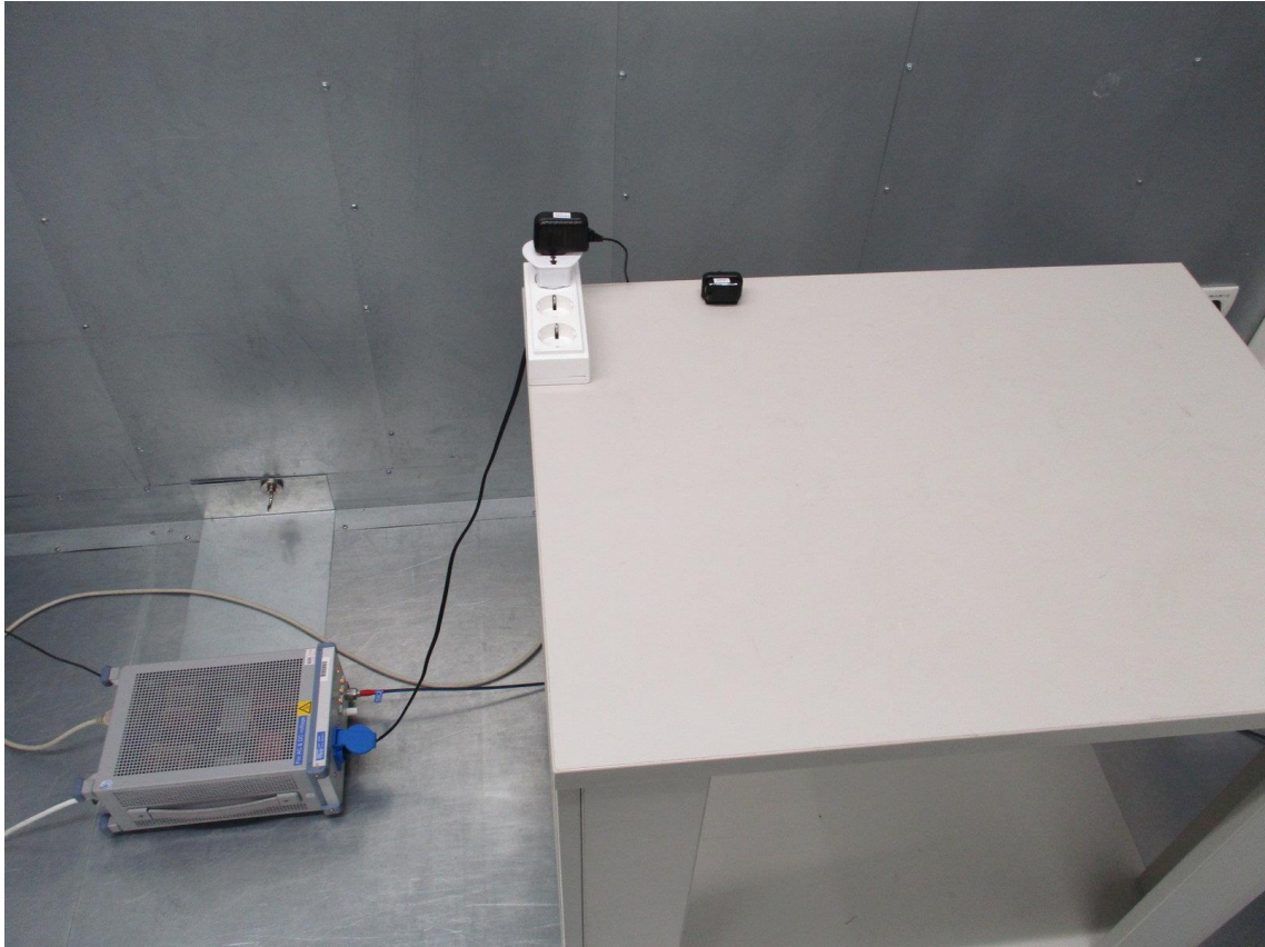
Figure 5: AC Conducted emission test setup
