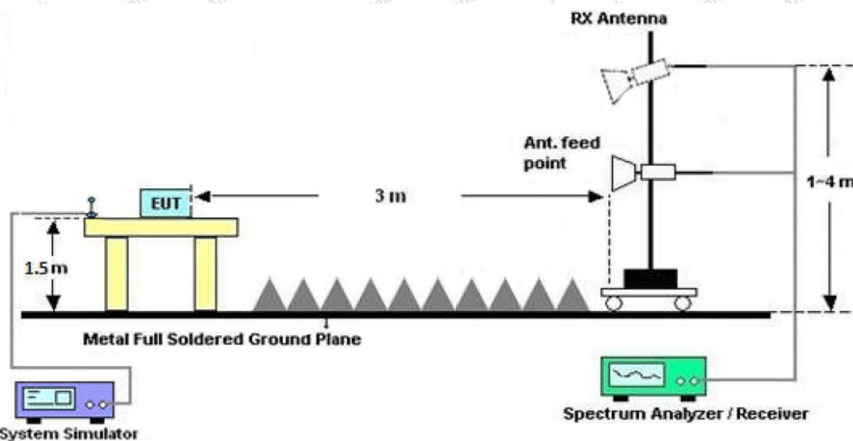
Figure 3. Above 1 GHz
