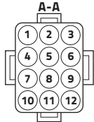
12 pin Harness pin out
