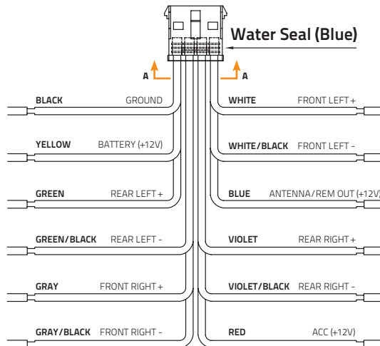
12 pin Harness pin out
