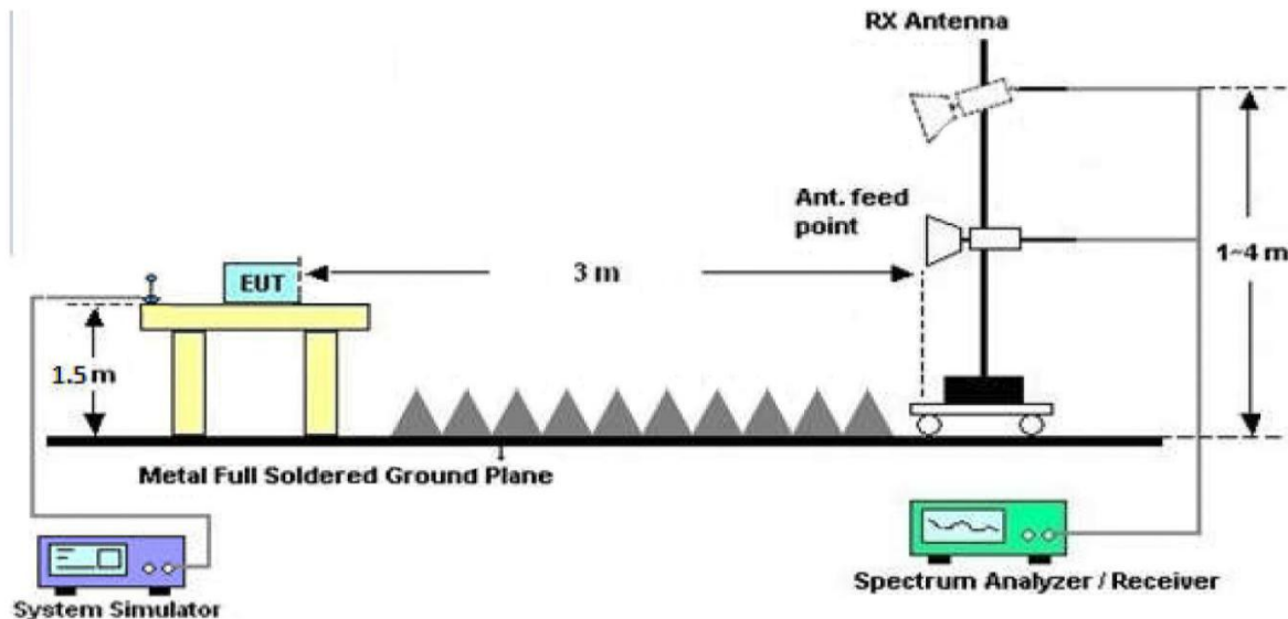
Figure 3. Above 1 GHz
