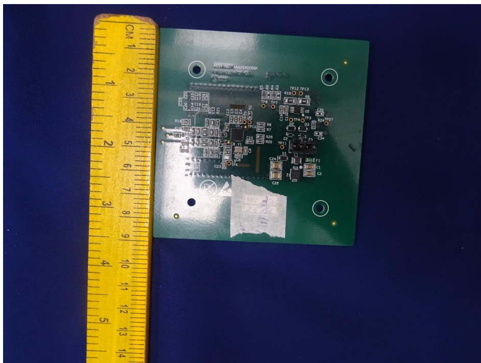
Photo 4:PCB Dimensional view( Width)
