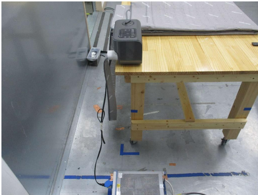
Disturbance Voltage Test
