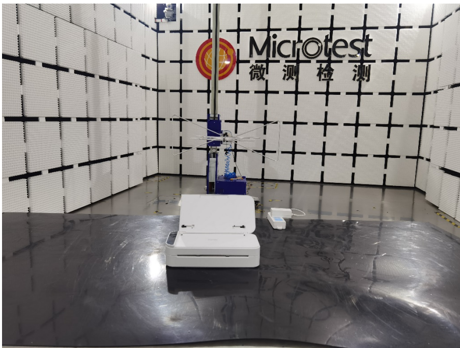
Emissions (above 1GHz)
