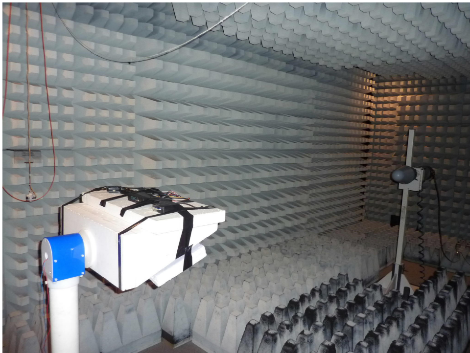
181948_4.JPG : Test setup final measurement from 1 to 14 GHz
