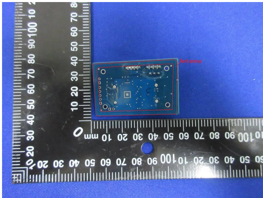
Antenna Location
