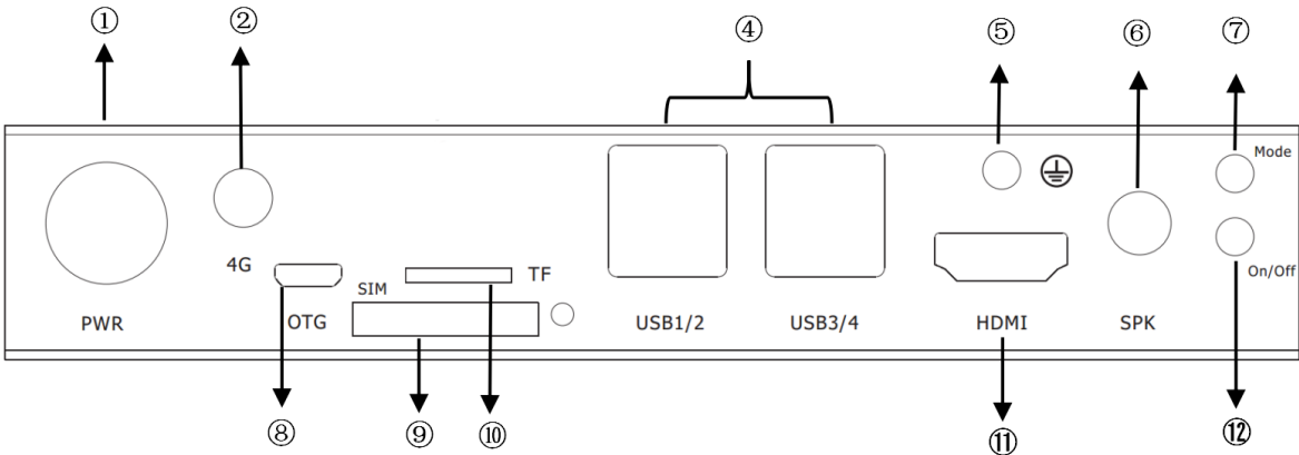
Figure 3-2-1 Front panel interface diagram
