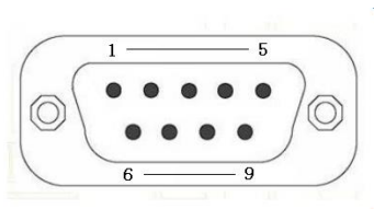
Figure 3-3-1 DB9 Interface Diagram
