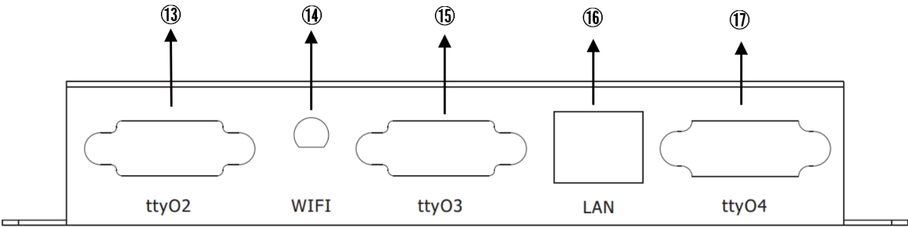
Figure 3-2-2 Rear panel interface diagram
