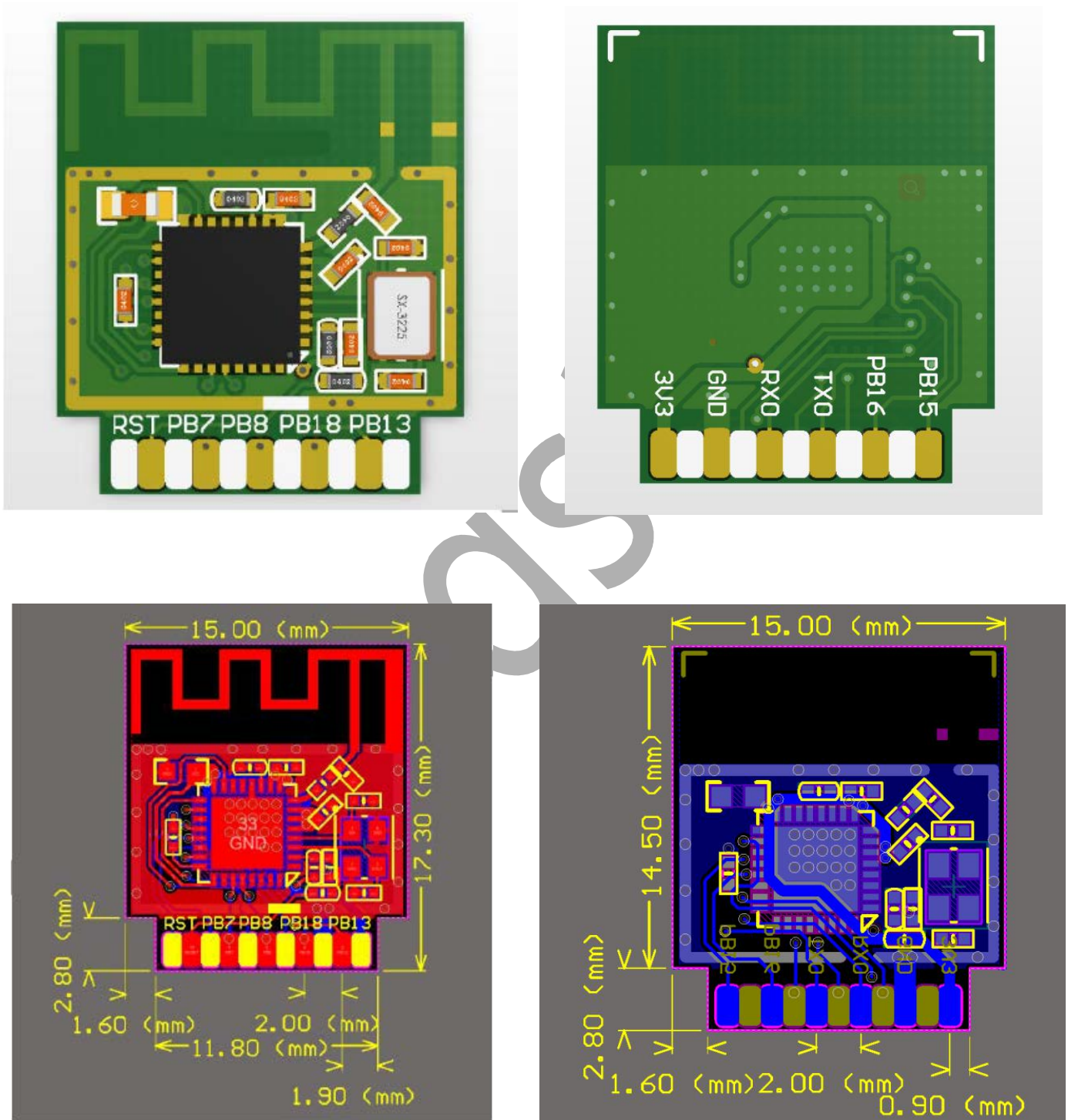
Figure 1.1 tw-02 pin dimensions
