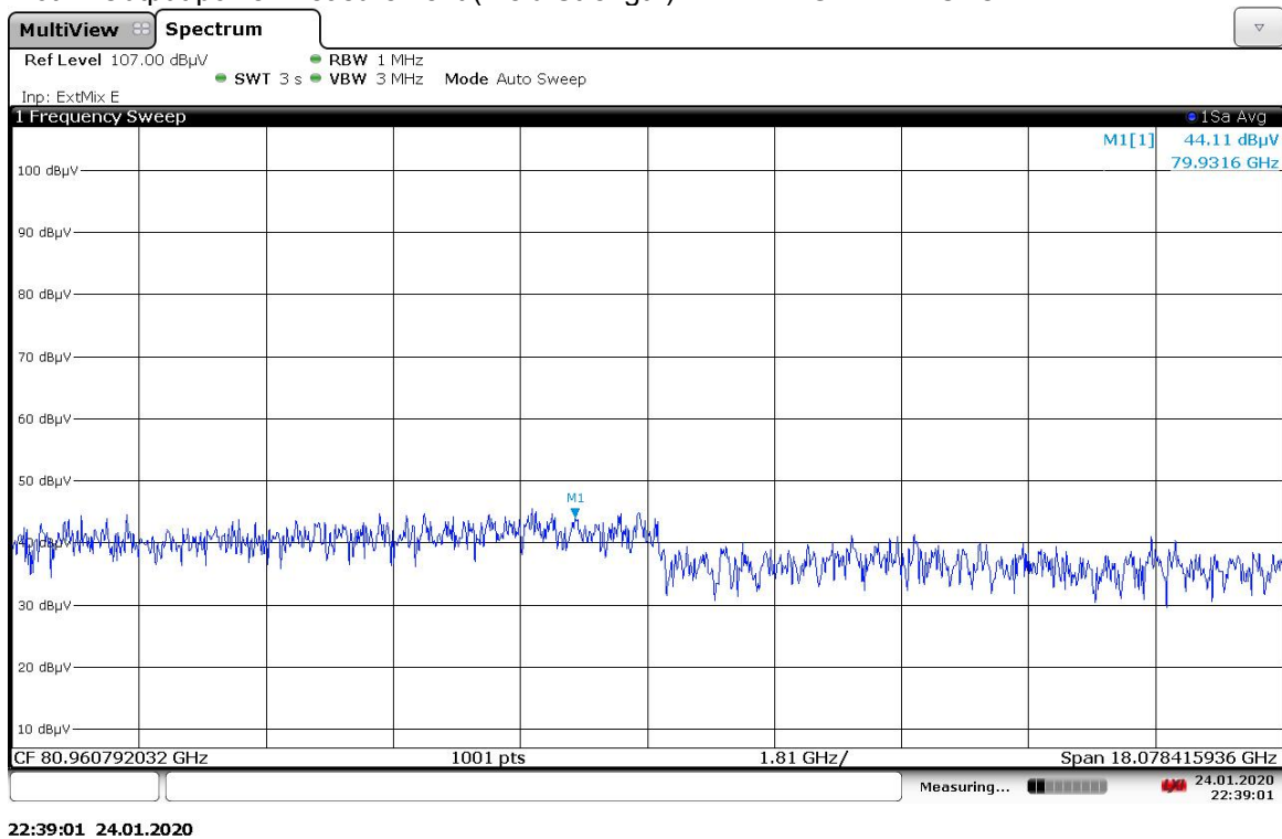
Plot 2: Output power measurement (Field Strength) – AVERAGE DETECTOR
