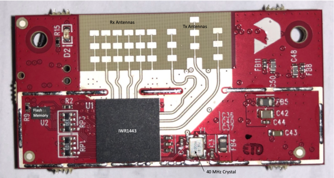
Figure 1. Key Module Component Placement (Front w/shield removed)
