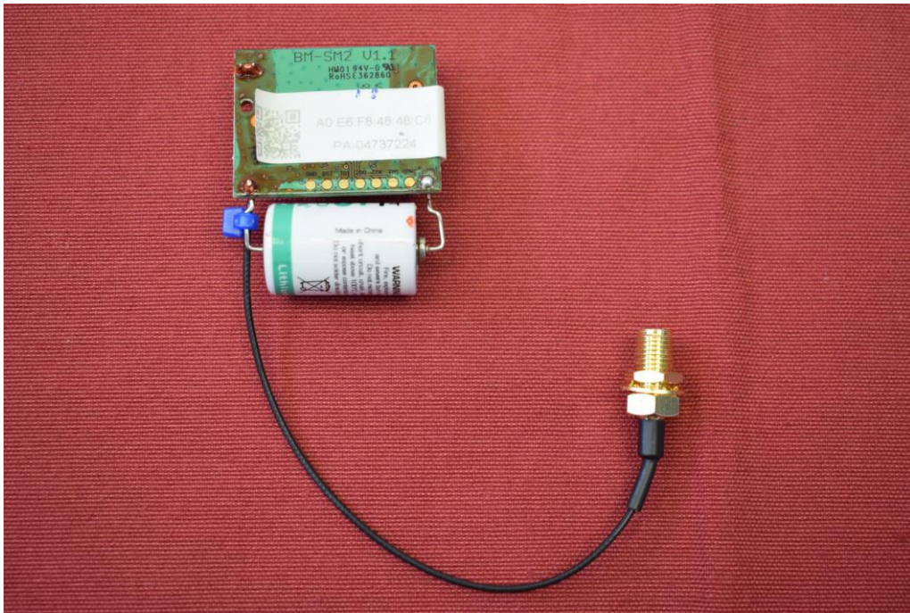
Picture 13: Module with antenna cable – bottom view
