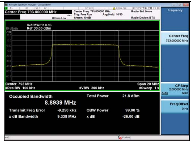
LTE band 14 - Middle CH 16QAM-10
