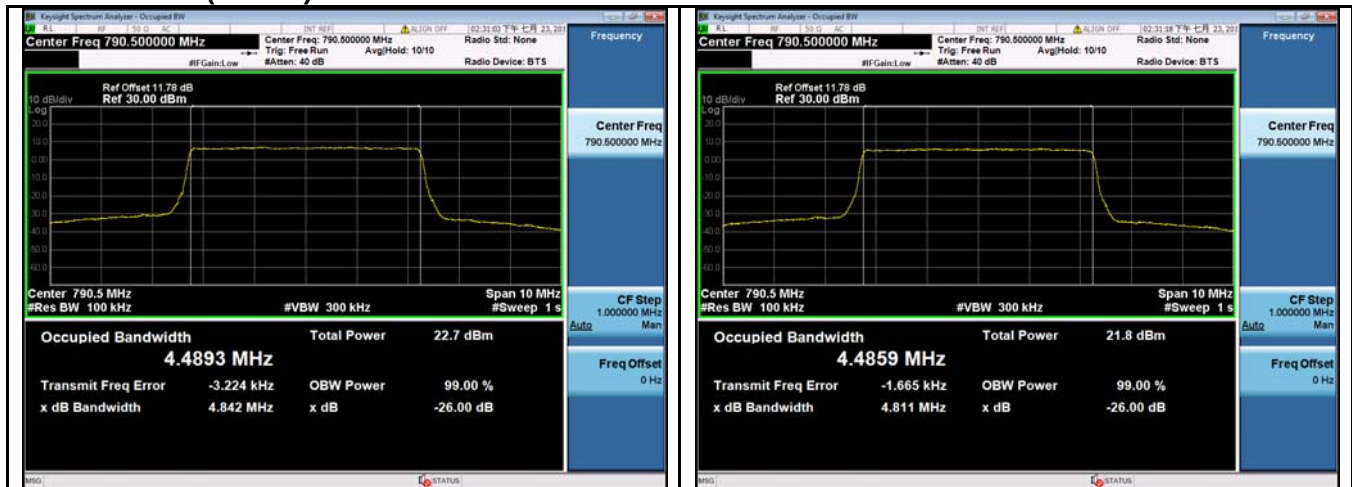
LTE band 14 - Low CH QPSK-5
