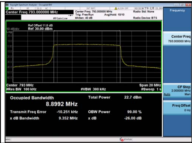
LTE band 14 - Middle CH QPSK-10
