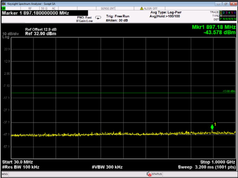
30MHz-1GHz
