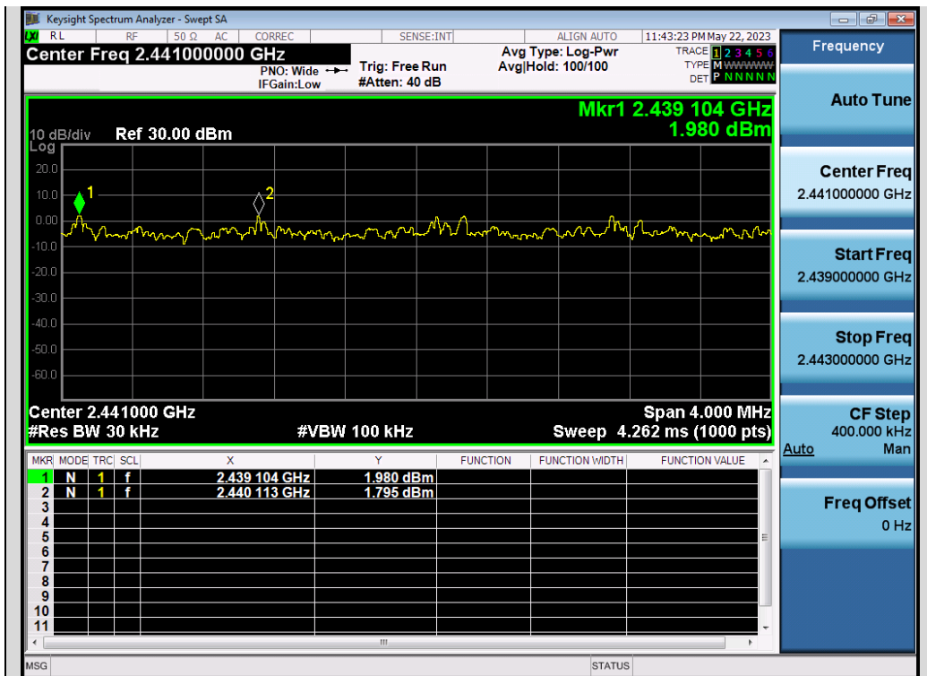
Test_Graph_BR_HOP_ANT1_NA_2Mbps_Hopping Separation
