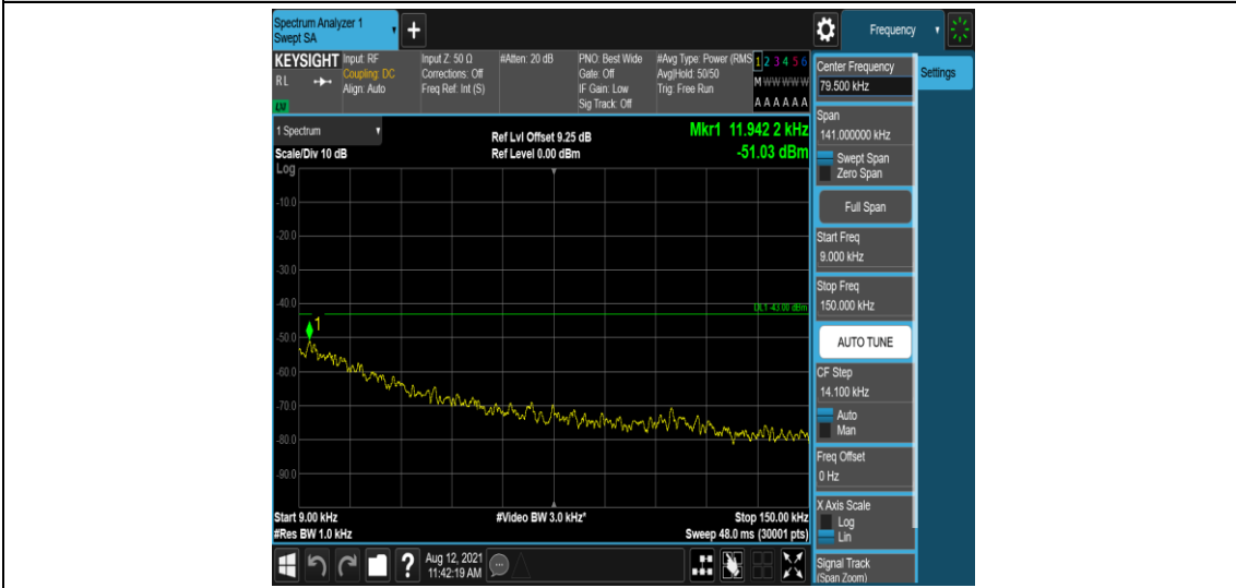
Band66-20MHz-QPSK-132322-1-0-Low-0.009-0.15--51.03-PASS
