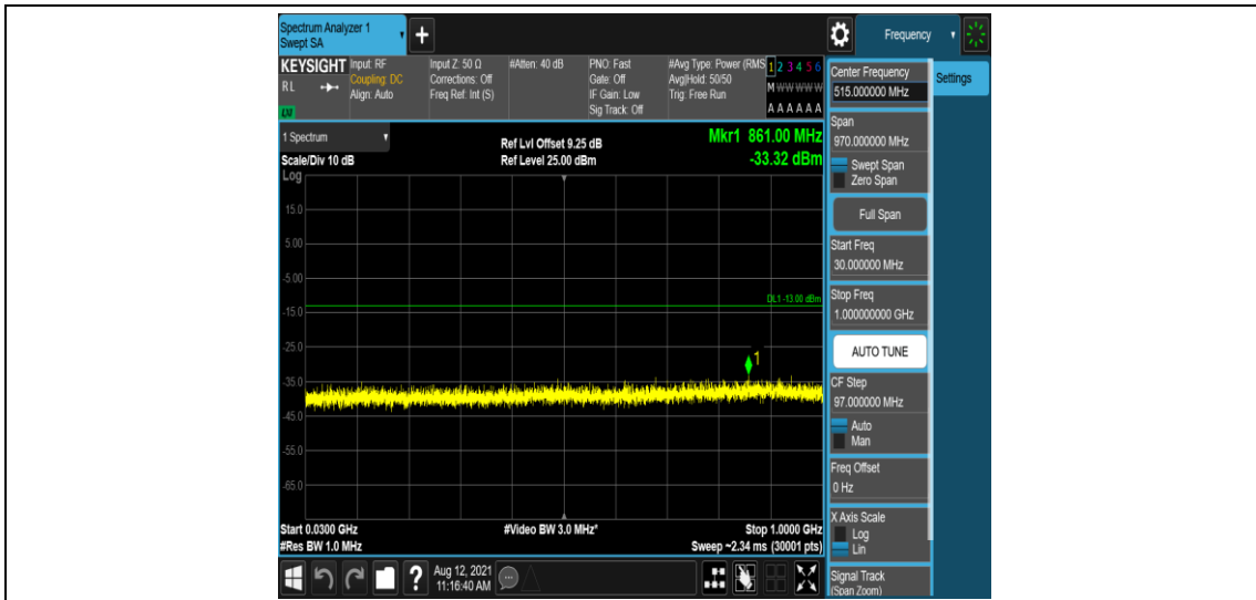
Band66-15MHz-QPSK-132322-1-0-Low-30-1000--33.32-PASS
