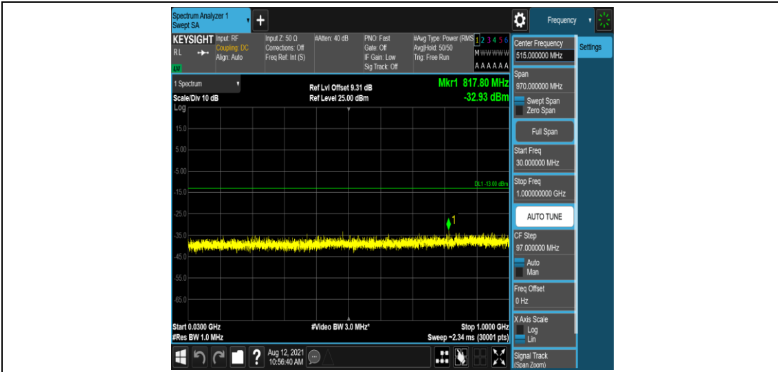
Band66-10MHz-16QAM-132622-1-0-High-30-1000--32.93-PASS
