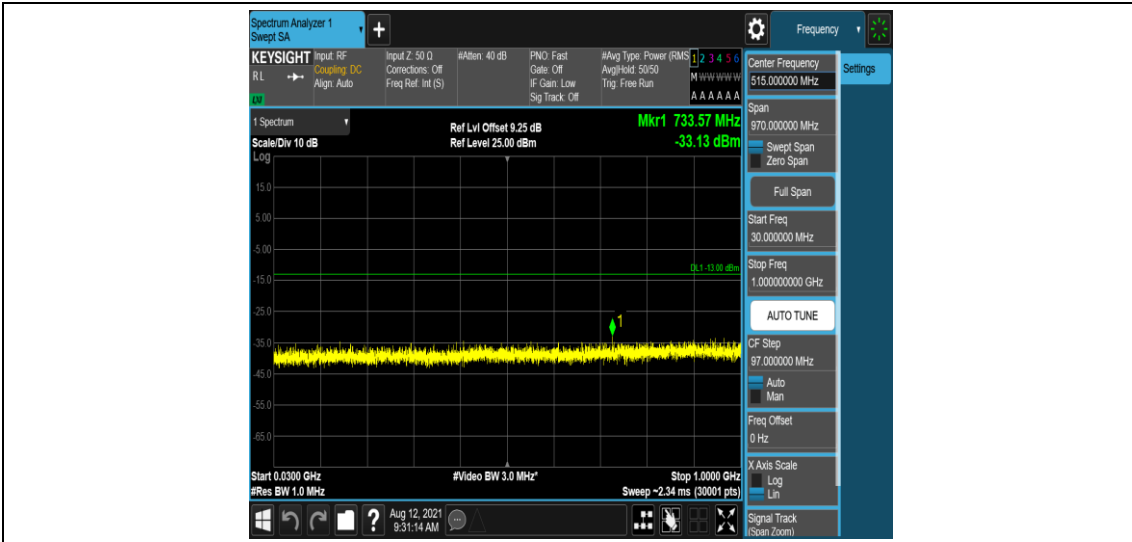
Band66-5MHz-QPSK-132322-1-0-Low-30-1000--33.13-PASS
