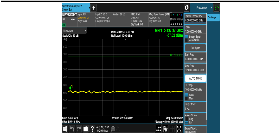
Band66-5MHz-QPSK-131997-1-0-Low-5000-12000--57.02-PASS
