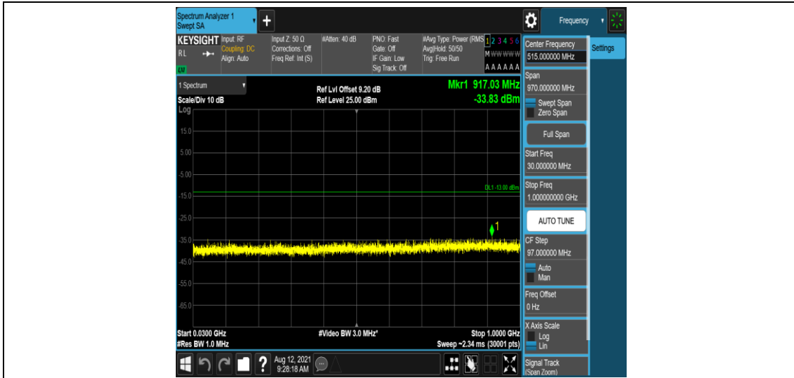
Band66-5MHz-QPSK-131997-1-0-Low-30-1000--33.83-PASS
