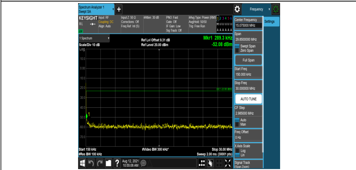
Band66-10MHz-QPSK-132622-1-0-High-0.15-30--52.08-PASS
