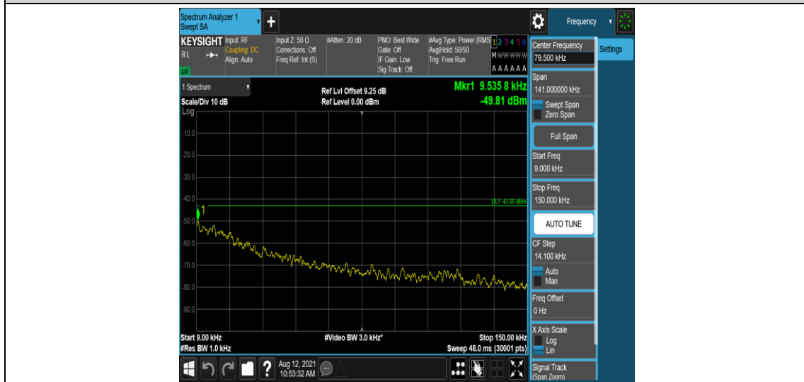
Band66-10MHz-16QAM-132322-1-0-Low-0.009-0.15--49.81-PASS
