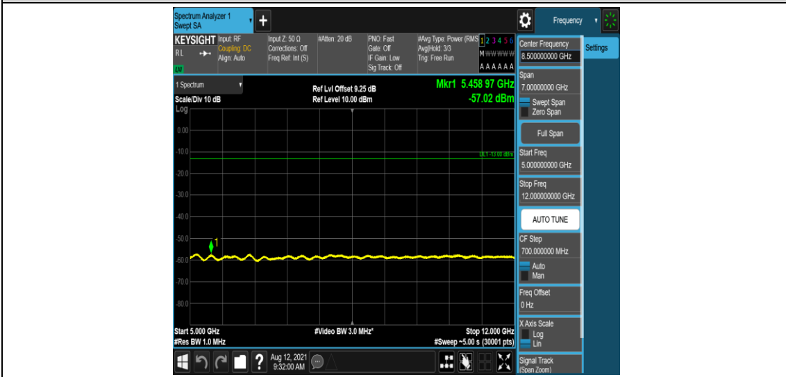
Band66-5MHz-QPSK-132322-1-0-Low-5000-12000--57.02-PASS
