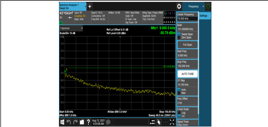
Band66-5MHz-QPSK-132647-1-0-High-0.009-0.15--50.79-PASS
