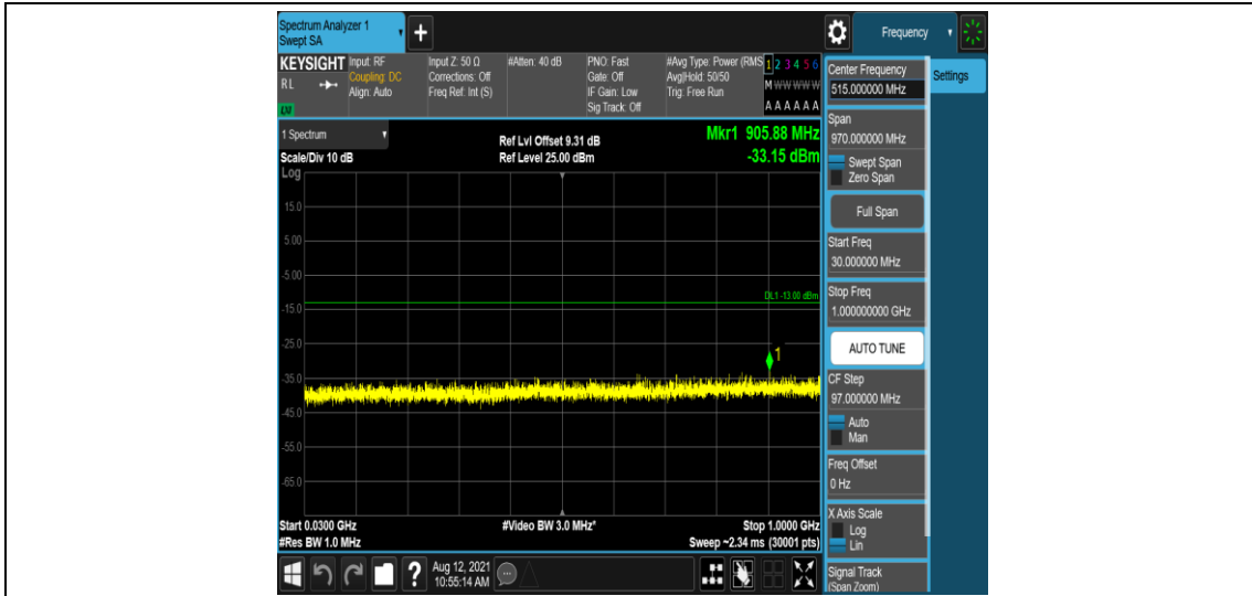
Band66-10MHz-QPSK-132622-1-0-High-30-1000--33.15-PASS
