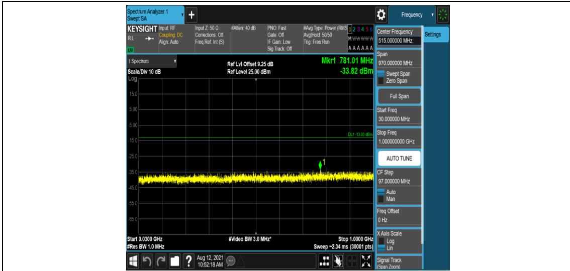
Band66-10MHz-QPSK-132322-1-0-Low-30-1000--33.82-PASS
