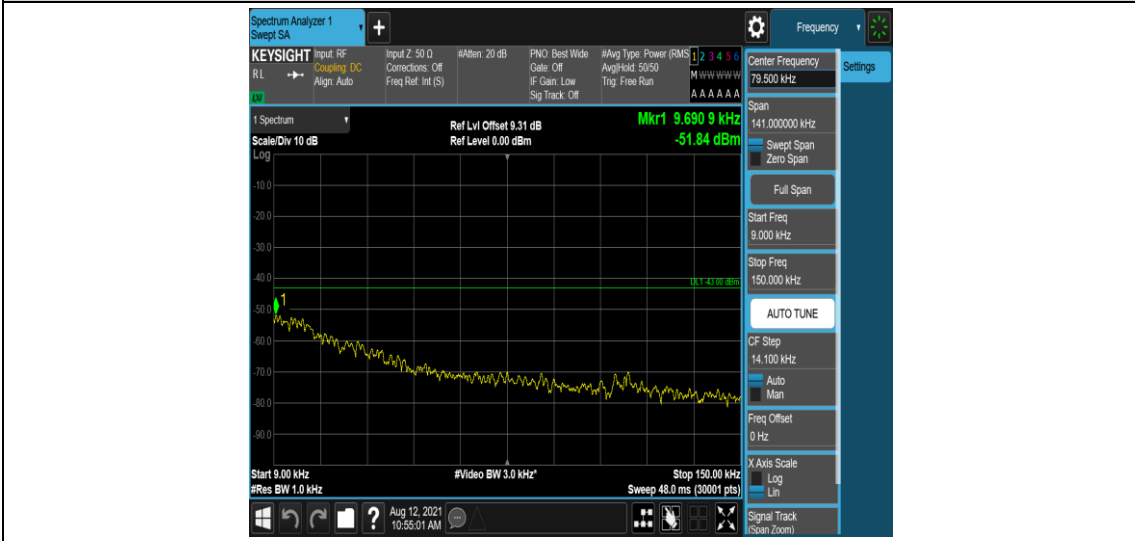
Band66-10MHz-QPSK-132622-1-0-High-0.009-0.15--51.84-PASS
