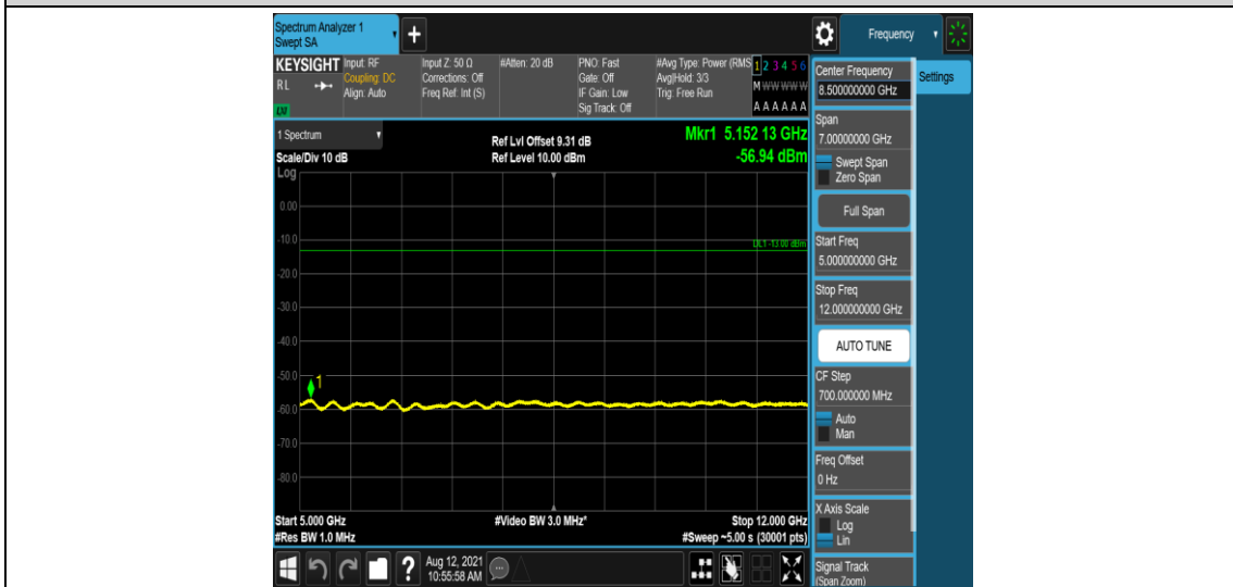
Band66-10MHz-QPSK-132622-1-0-High-5000-12000--56.94-PASS
