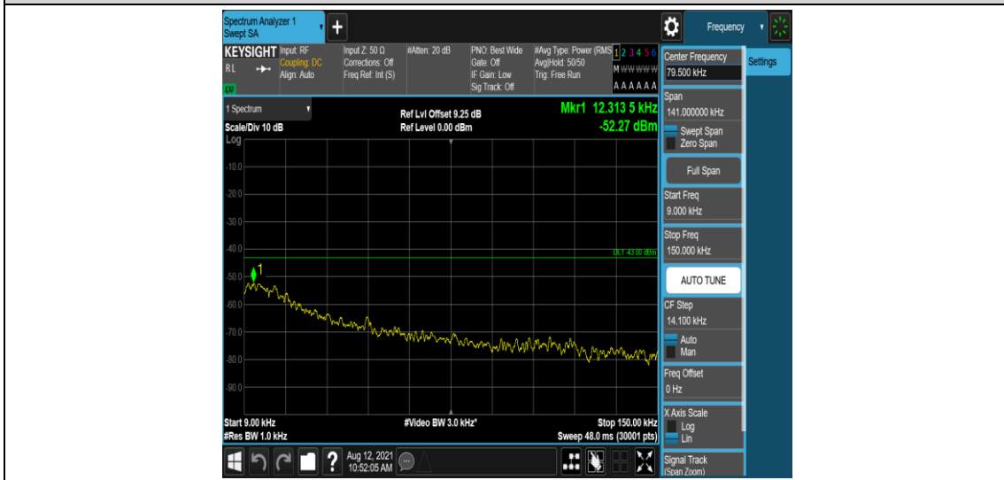
Band66-10MHz-QPSK-132322-1-0-Low-0.009-0.15--52.27-PASS
