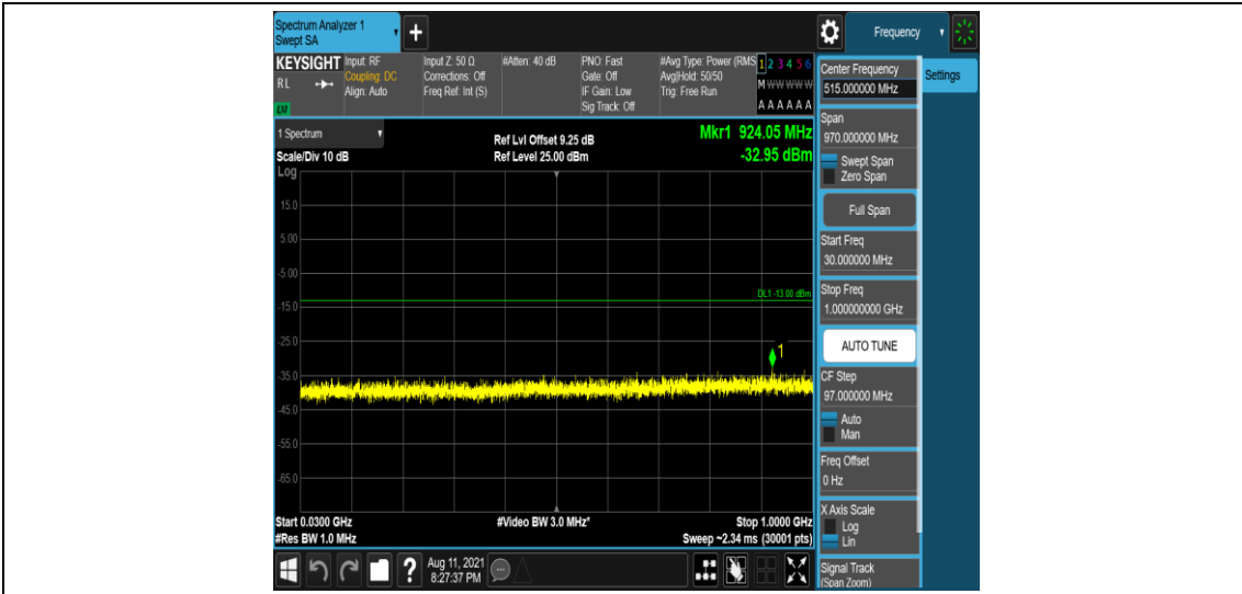
Band66-3MHz-QPSK-132322-1-0-Low-30-1000--32.95-PASS
