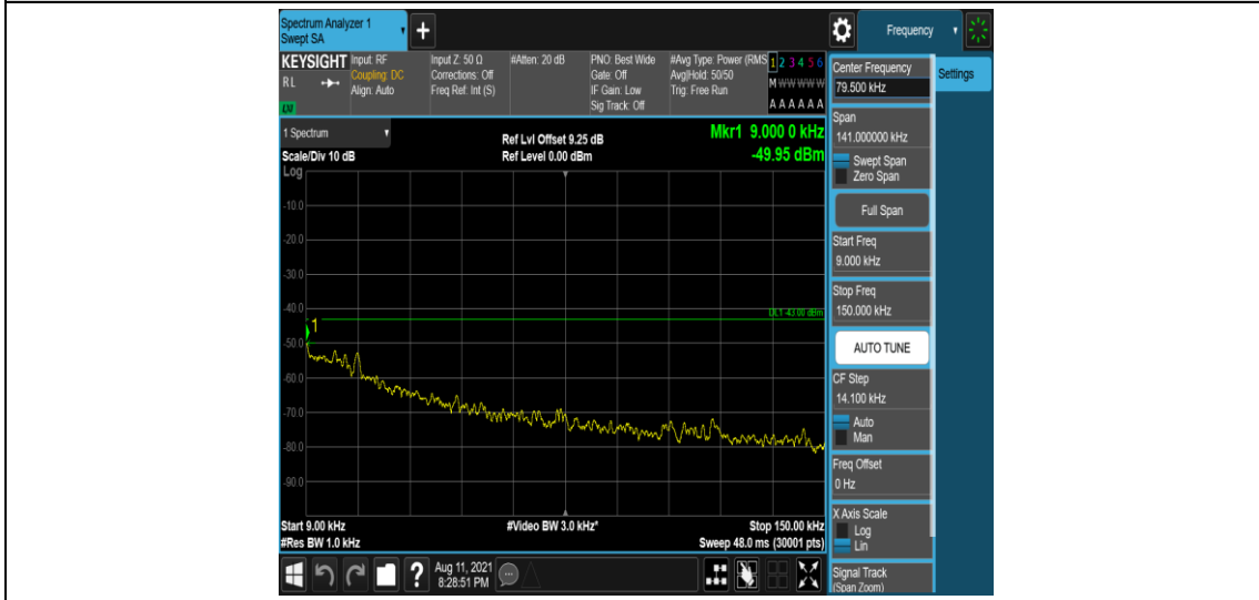
Band66-3MHz-16QAM-132322-1-0-Low-0.009-0.15--49.95-PASS
