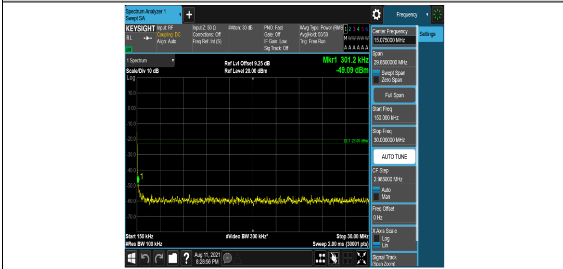
Band66-3MHz-16QAM-132322-1-0-Low-0.15-30--49.09-PASS
