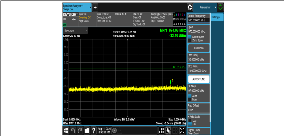
Band66-3MHz-QPSK-132657-1-0-High-30-1000--33.1-PASS
