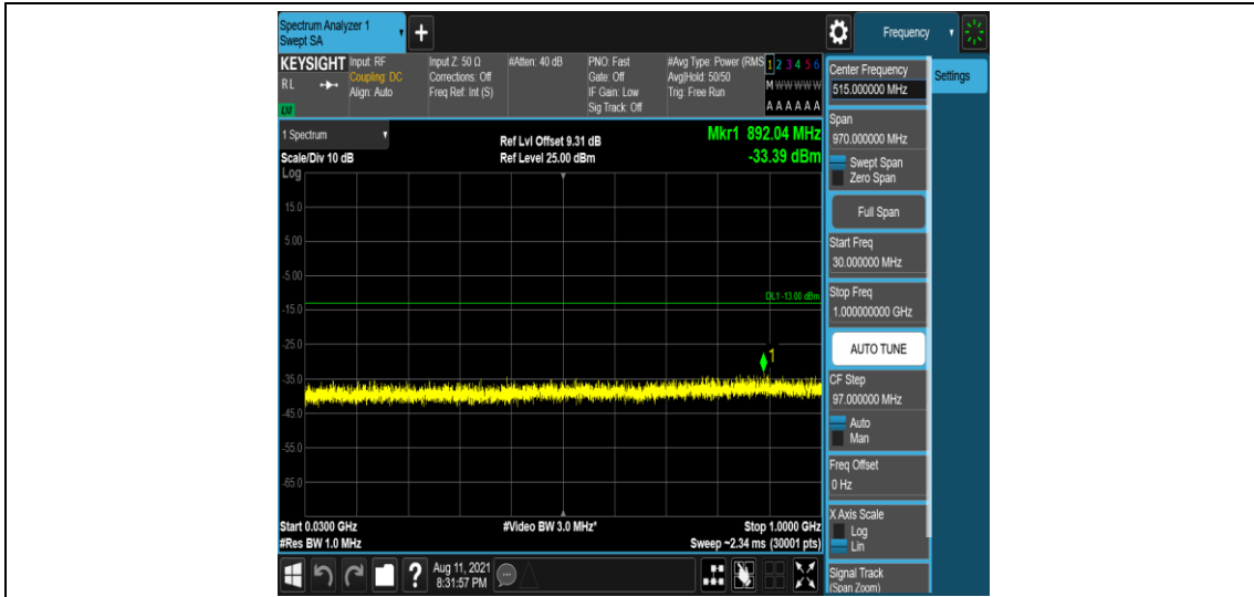
Band66-3MHz-16QAM-132657-1-0-High-30-1000--33.39-PASS
