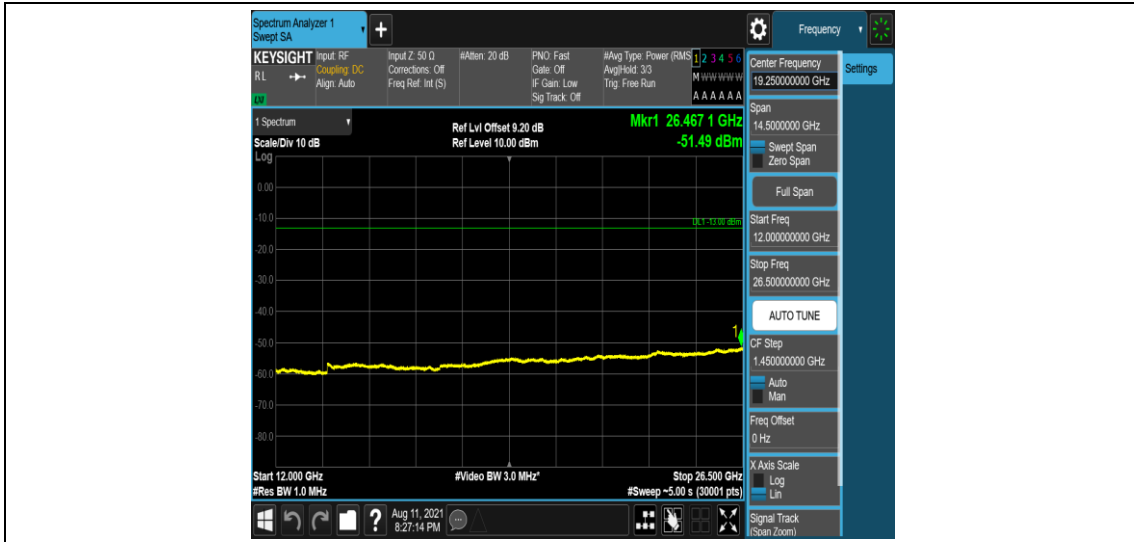
Band66-3MHz-16QAM-131987-1-0-Low-12000-26500--51.49-PASS
