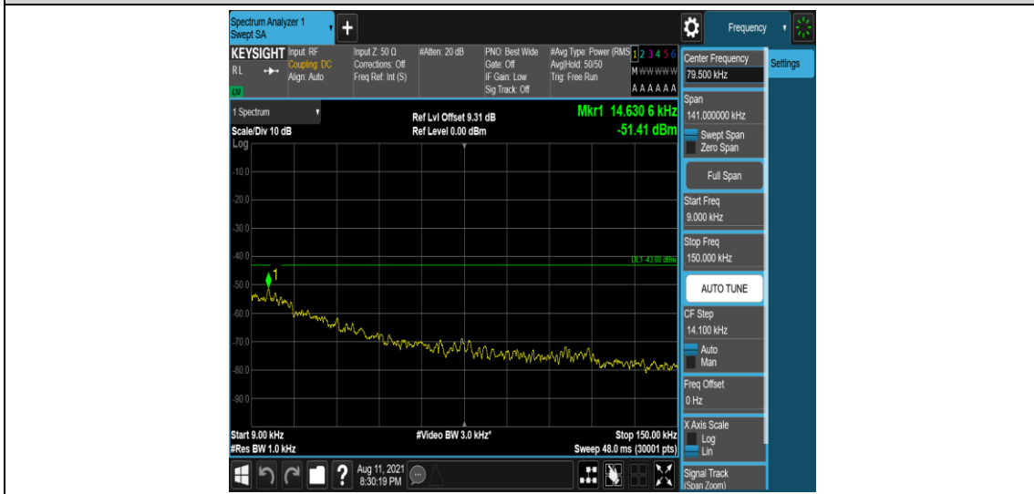
Band66-3MHz-QPSK-132657-1-0-High-0.009-0.15--51.41-PASS
