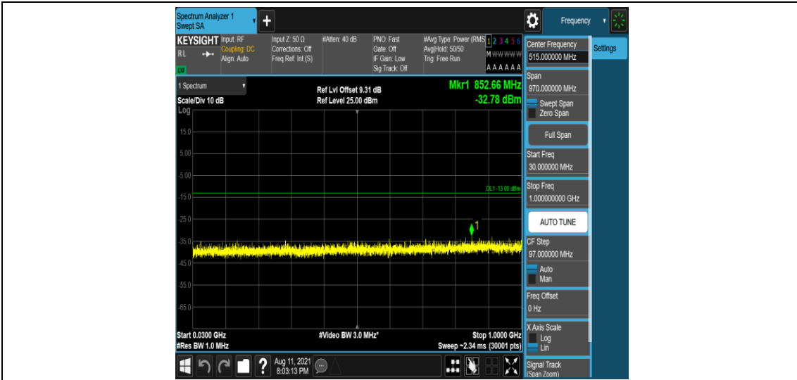
Band66-1.4MHz-QPSK-132665-1-0-High-30-1000--32.78-PASS
