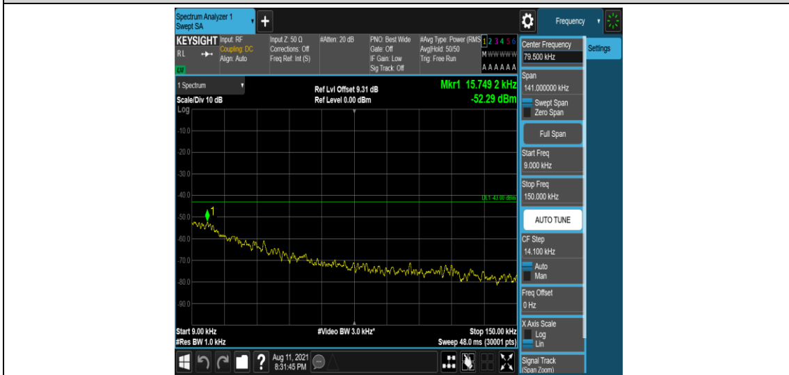
Band66-3MHz-16QAM-132657-1-0-High-0.009-0.15--52.29-PASS
