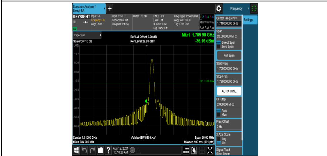
Band66-10MHz-16QAM-132022-1-0-Low--36.16-PASS
