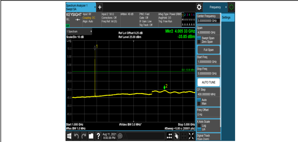
Band66-1.4MHz-QPSK-132322-1-0-Low-1000-5000--35.85-PASS
