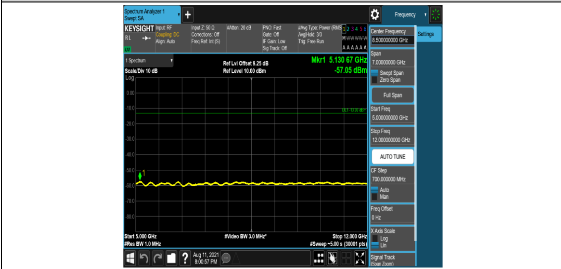
Band66-1.4MHz-QPSK-132322-1-0-Low-5000-12000--57.05-PASS
