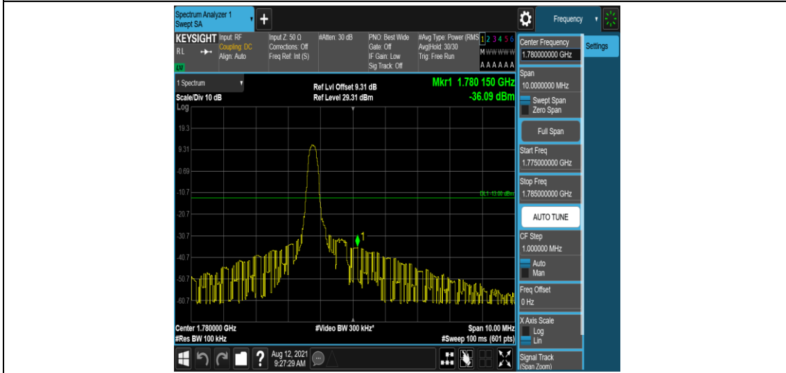
Band66-5MHz-QPSK-132647-1-0-High--36.09-PASS
