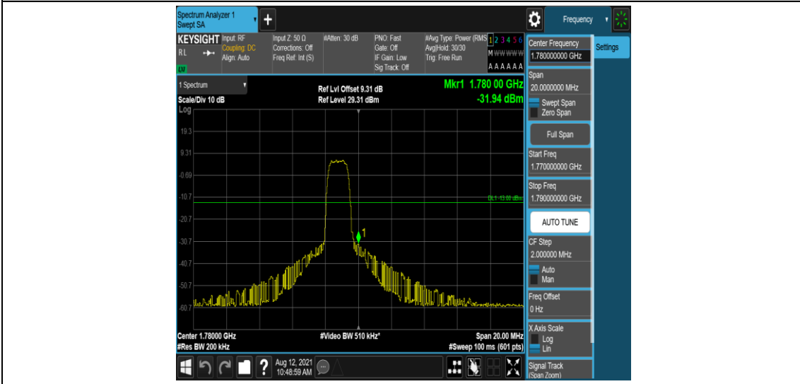
Band66-10MHz-16QAM-132622-6-0-High--31.94-PASS
