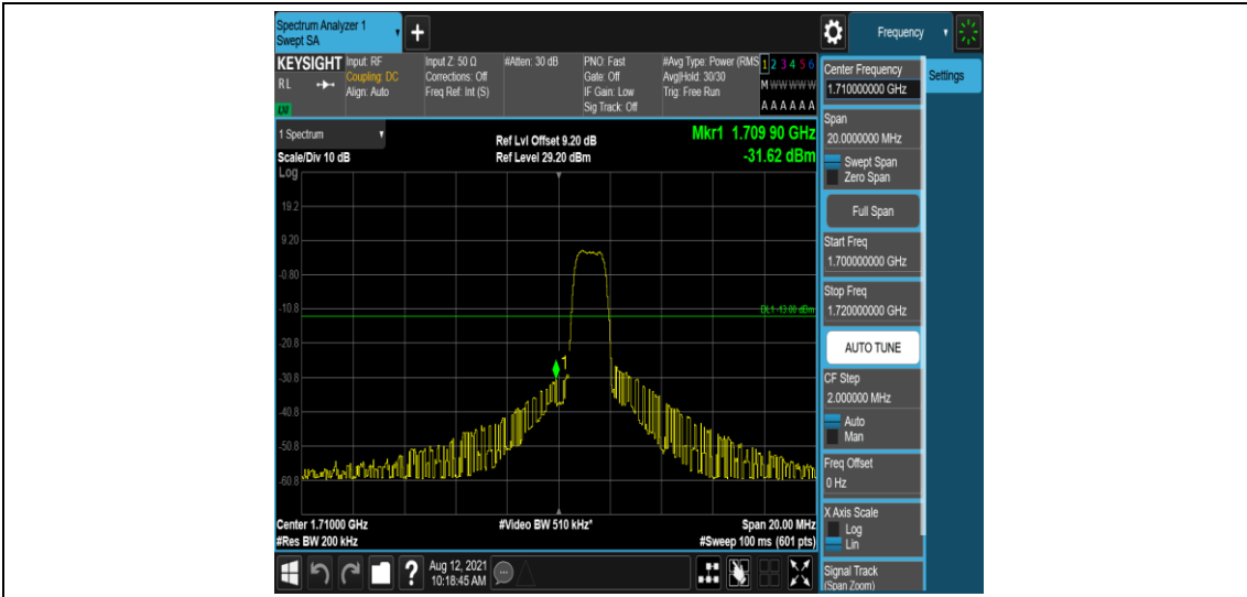
Band66-10MHz-16QAM-132022-6-0-Low--31.62-PASS
