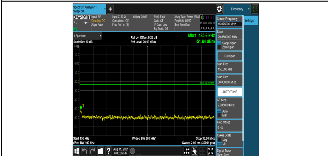
Band66-1.4MHz-QPSK-132322-1-0-Low-0.15-30--51.64-PASS
