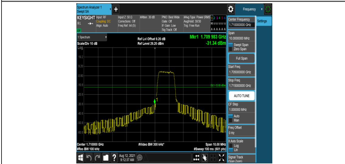
Band66-5MHz-16QAM-131997-6-0-Low--31.34-PASS
