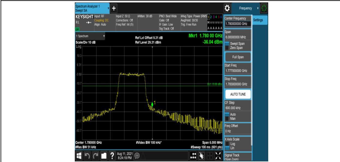
Band66-3MHz-16QAM-132657-6-0-High--36.04-PASS
