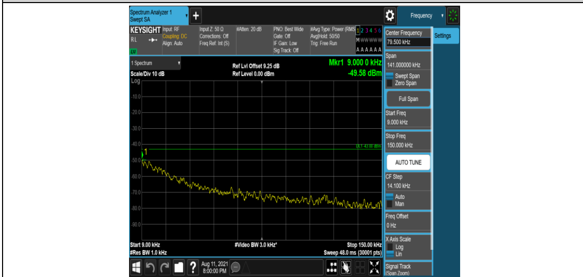
Band66-1.4MHz-QPSK-132322-1-0-Low-0.009-0.15--49.58-PASS
