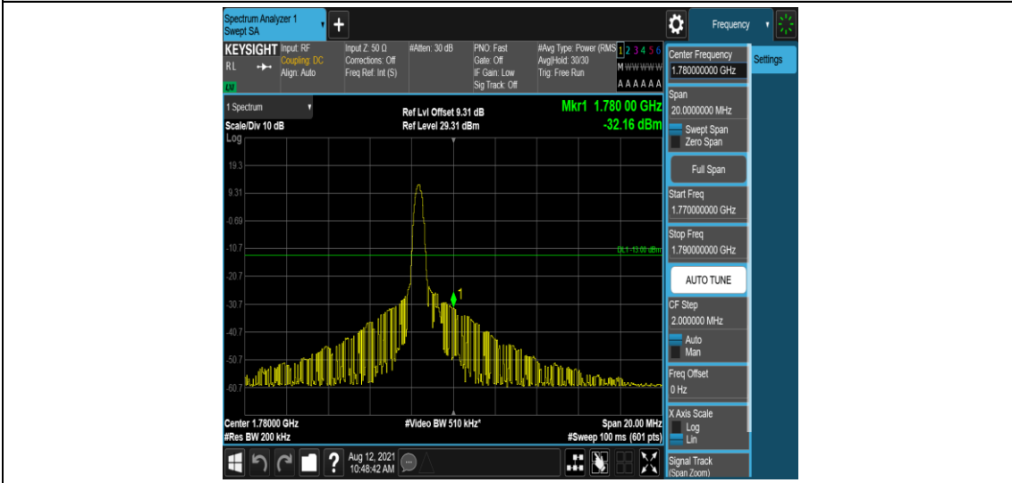
Band66-10MHz-16QAM-132622-1-0-High--32.16-PASS
