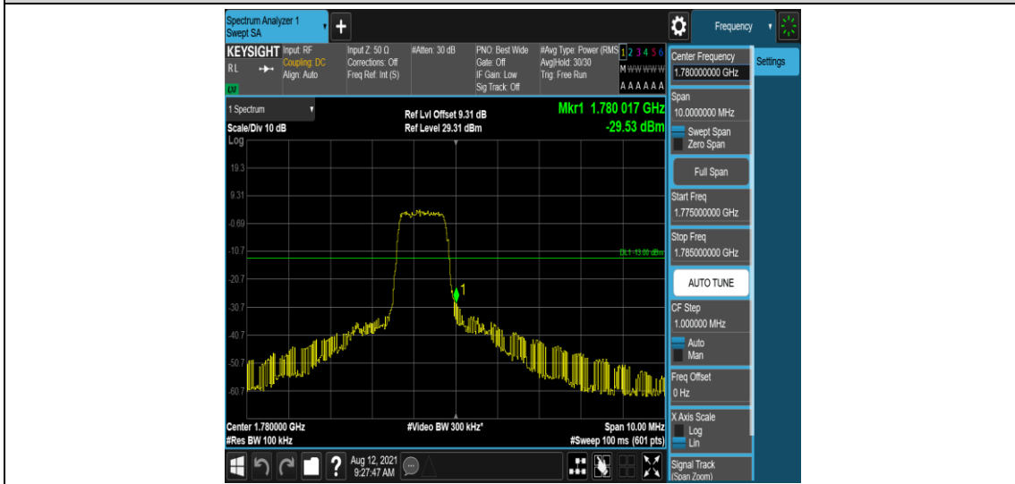
Band66-5MHz-QPSK-132647-6-0-High--29.53-PASS
