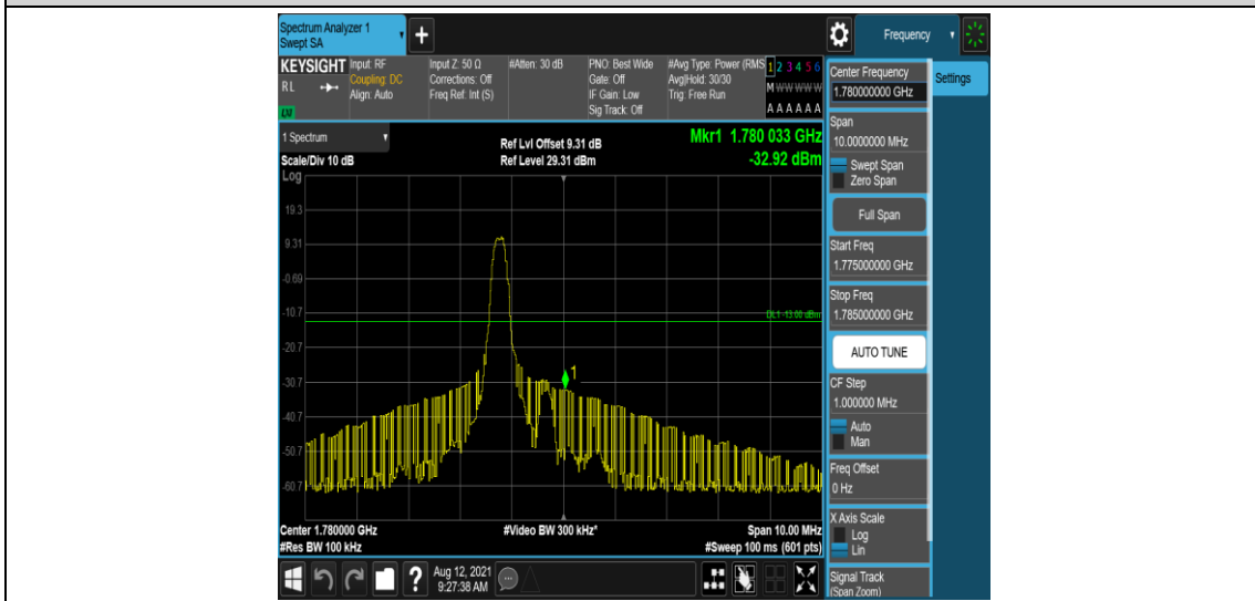
Band66-5MHz-16QAM-132647-1-0-High--32.92-PASS
