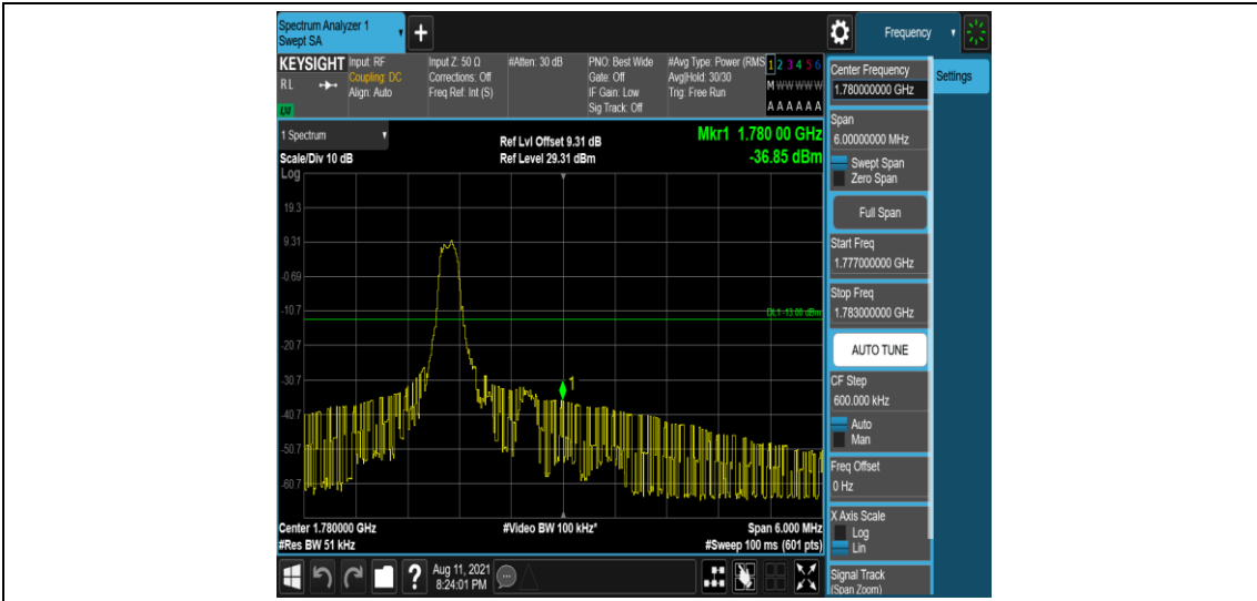
Band66-3MHz-16QAM-132657-1-0-High--36.85-PASS
