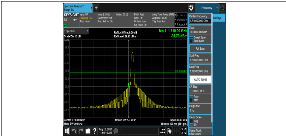
Band66-15MHz-QPSK-132047-1-0-Low--31.73-PASS
