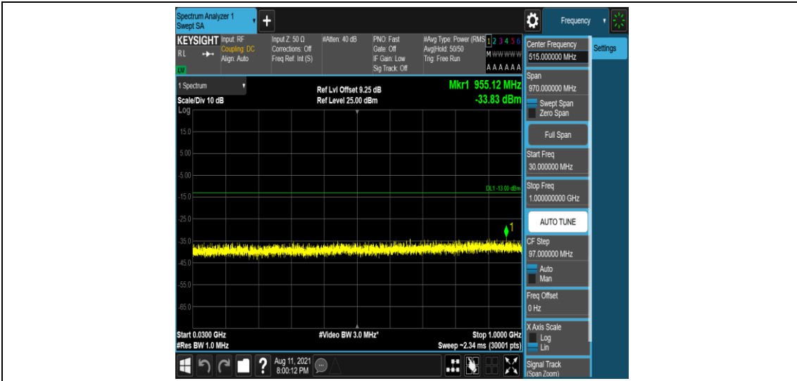
Band66-1.4MHz-QPSK-132322-1-0-Low-30-1000--33.83-PASS
