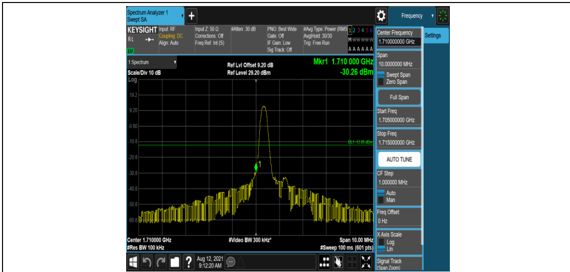
Band66-5MHz-16QAM-131997-1-0-Low--30.26-PASS
