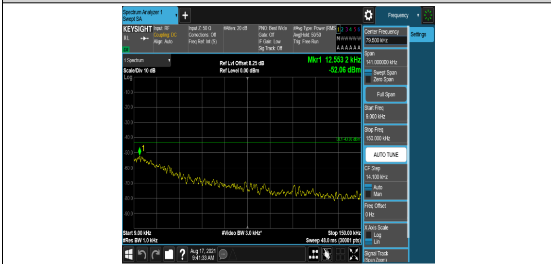
Band26-10MHz-16QAM-26840-1-0-Low-0.009-0.15--52.06-PASS
