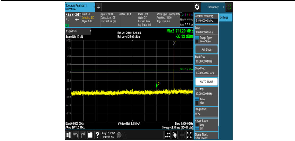
Band26-10MHz-QPSK-26990-1-0-High-30-1000--34-PASS
