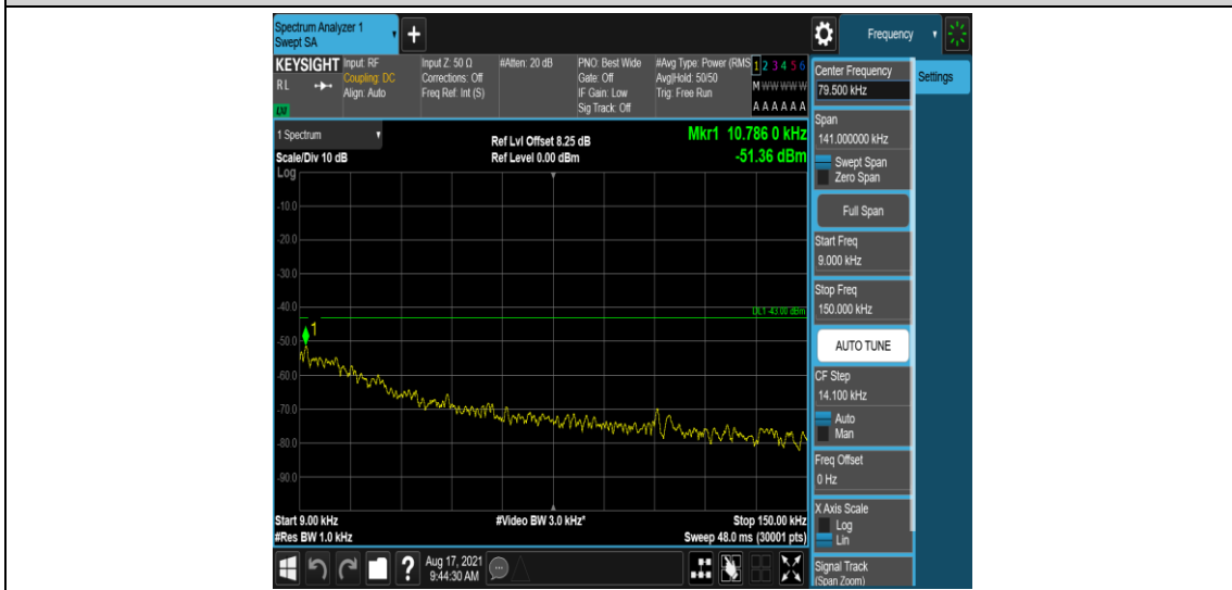
Band26-10MHz-16QAM-26915-1-0-Low-0.009-0.15--51.36-PASS
