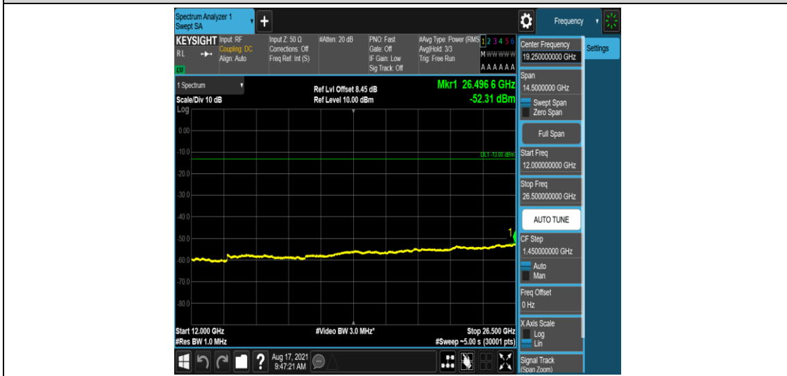
Band26-10MHz-QPSK-26990-1-0-High-12000-26500--52.31-PASS
