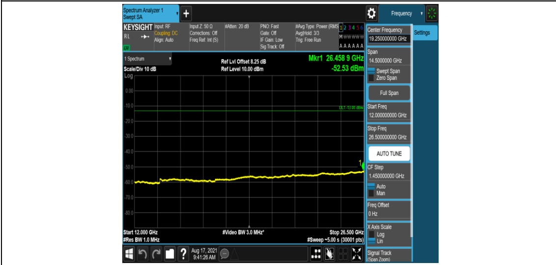
Band26-10MHz-QPSK-26840-1-0-Low-12000-26500--52.53-PASS
