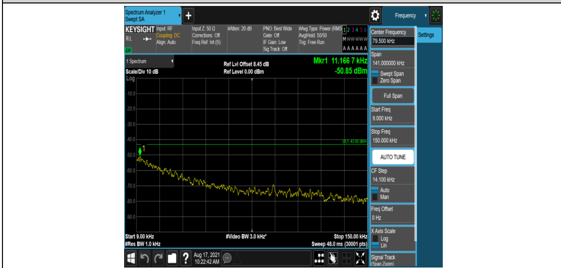
Band26-15MHz-QPSK-26960-1-0-High-0.009-0.15--50.85-PASS
