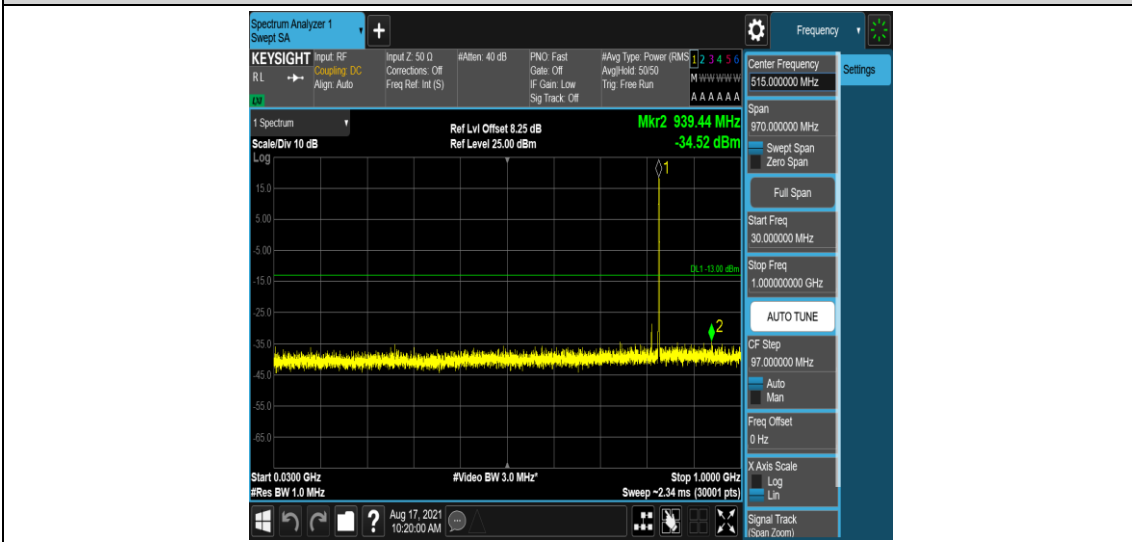
Band26-15MHz-QPSK-26915-1-0-Low-30-1000--34.52-PASS
