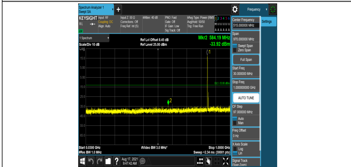
Band26-10MHz-16QAM-26990-1-0-High-30-1000--33.92-PASS
