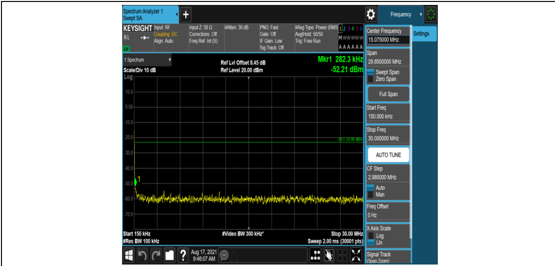
Band26-10MHz-QPSK-26990-1-0-High-0.15-30--52.21-PASS
