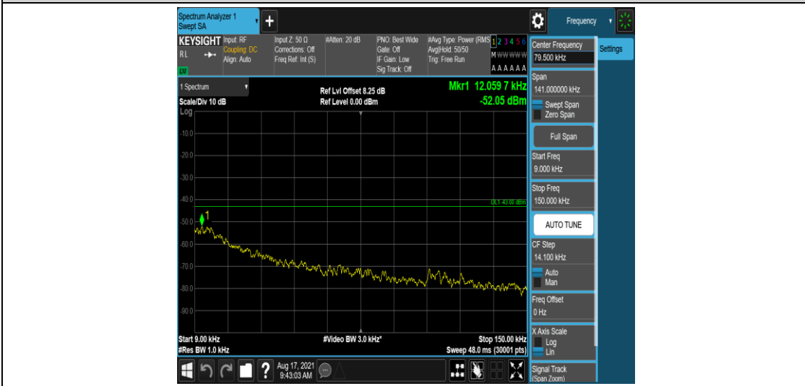
Band26-10MHz-QPSK-26915-1-0-Low-0.009-0.15--52.05-PASS
