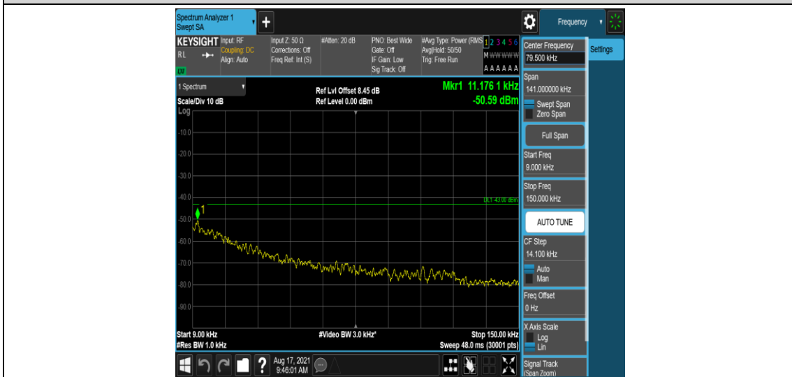
Band26-10MHz-QPSK-26990-1-0-High-0.009-0.15--50.59-PASS
