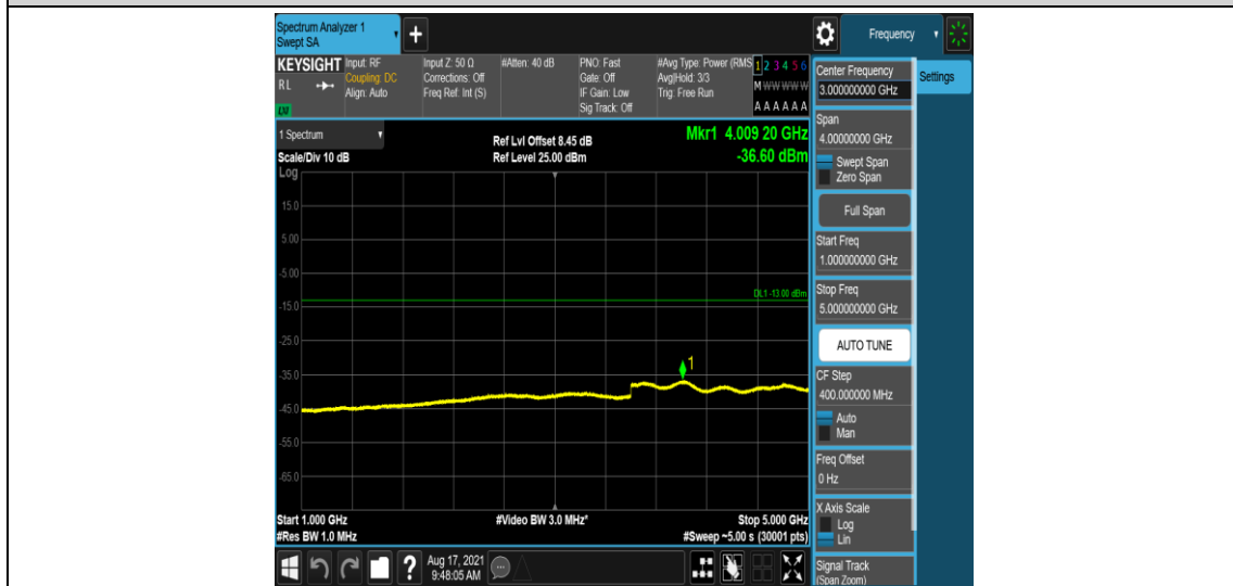
Band26-10MHz-16QAM-26990-1-0-High-1000-5000--36.6-PASS
