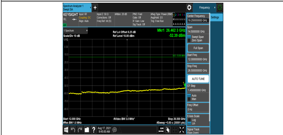
Band26-10MHz-16QAM-26915-1-0-Low-12000-26500--52.39-PASS
