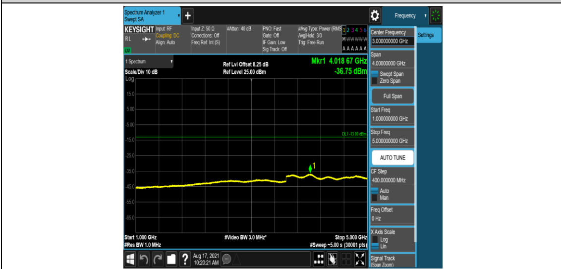
Band26-15MHz-QPSK-26915-1-0-Low-1000-5000--36.75-PASS
