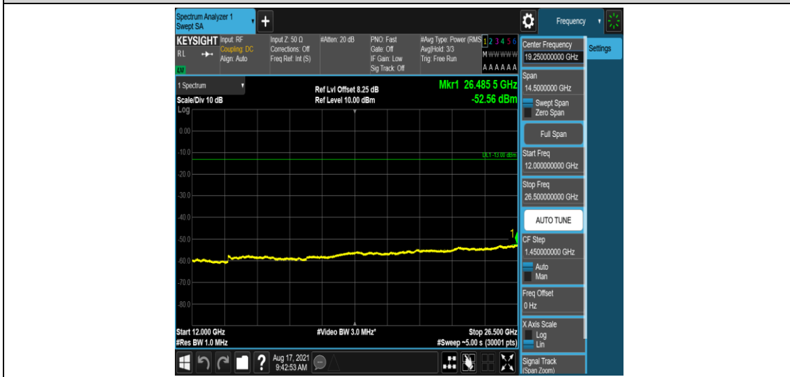
Band26-10MHz-16QAM-26840-1-0-Low-12000-26500--52.56-PASS
