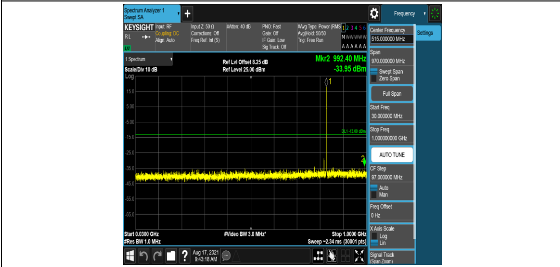
Band26-10MHz-QPSK-26915-1-0-Low-30-1000--33.95-PASS
