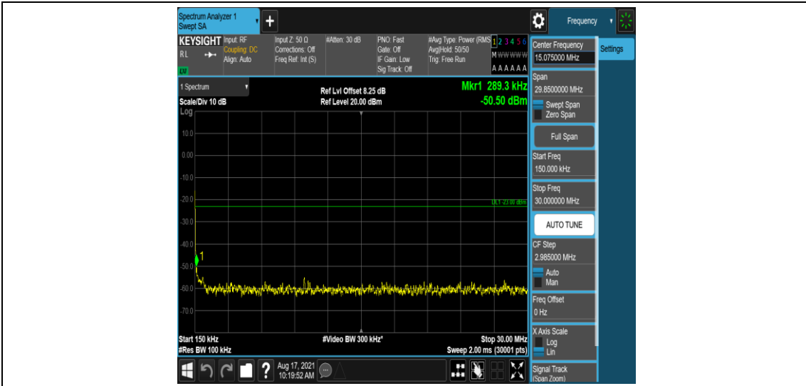
Band26-15MHz-QPSK-26915-1-0-Low-0.15-30--50.5-PASS
