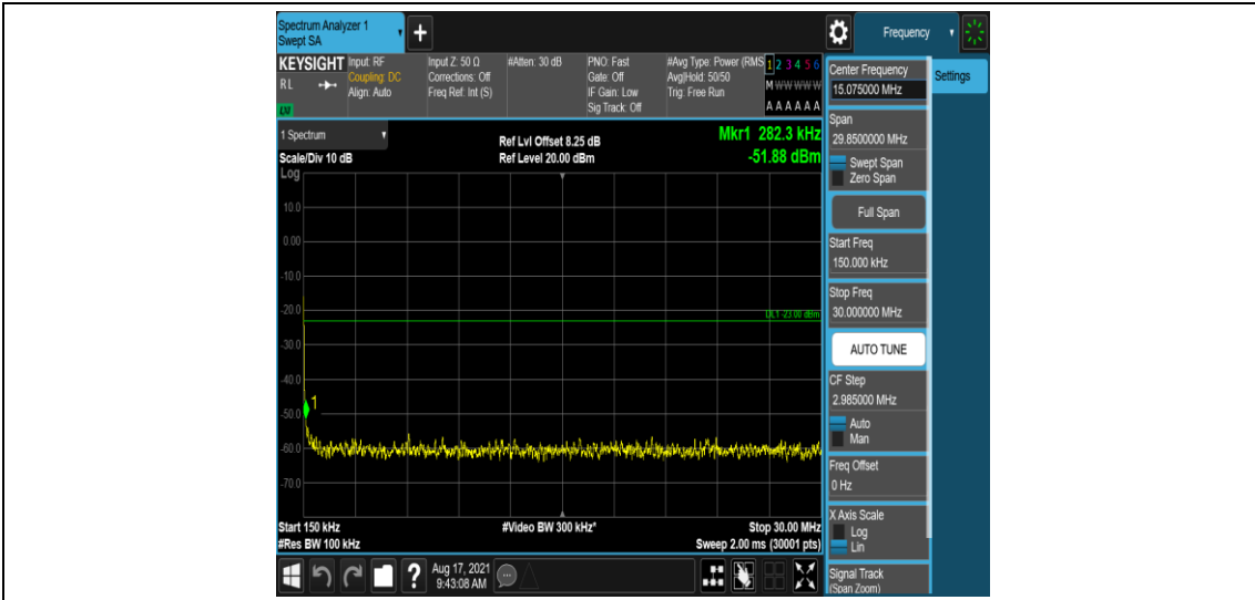
Band26-10MHz-QPSK-26915-1-0-Low-0.15-30--51.88-PASS
