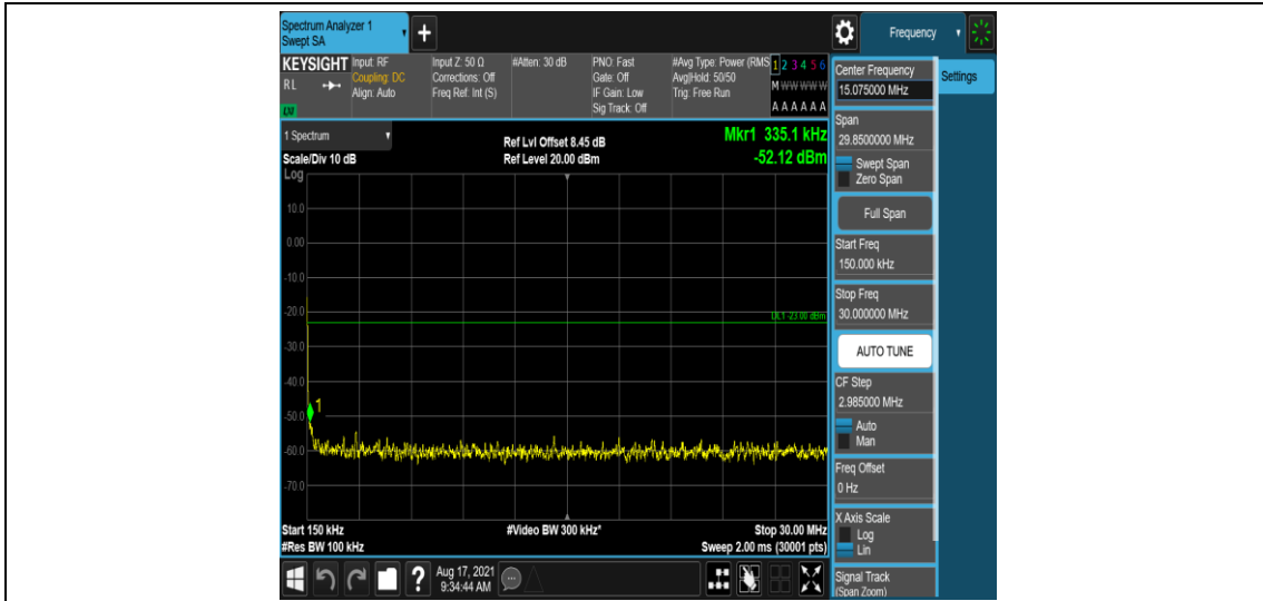
Band26-5MHz-16QAM-27015-1-0-High-0.15-30--52.12-PASS
