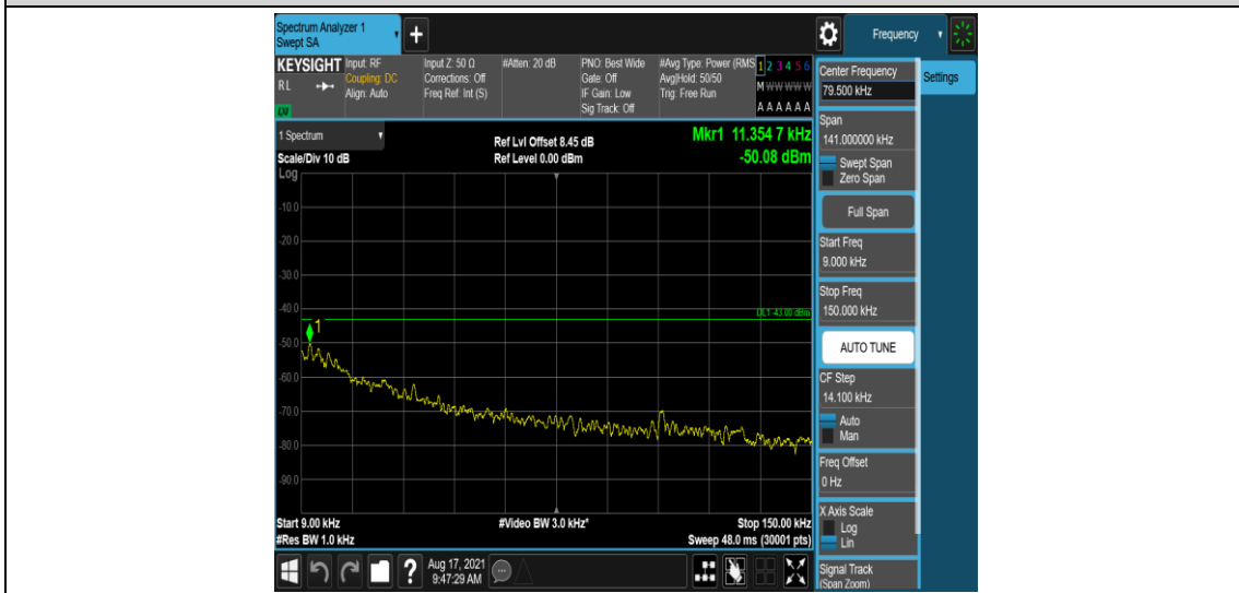
Band26-10MHz-16QAM-26990-1-0-High-0.009-0.15--50.08-PASS
