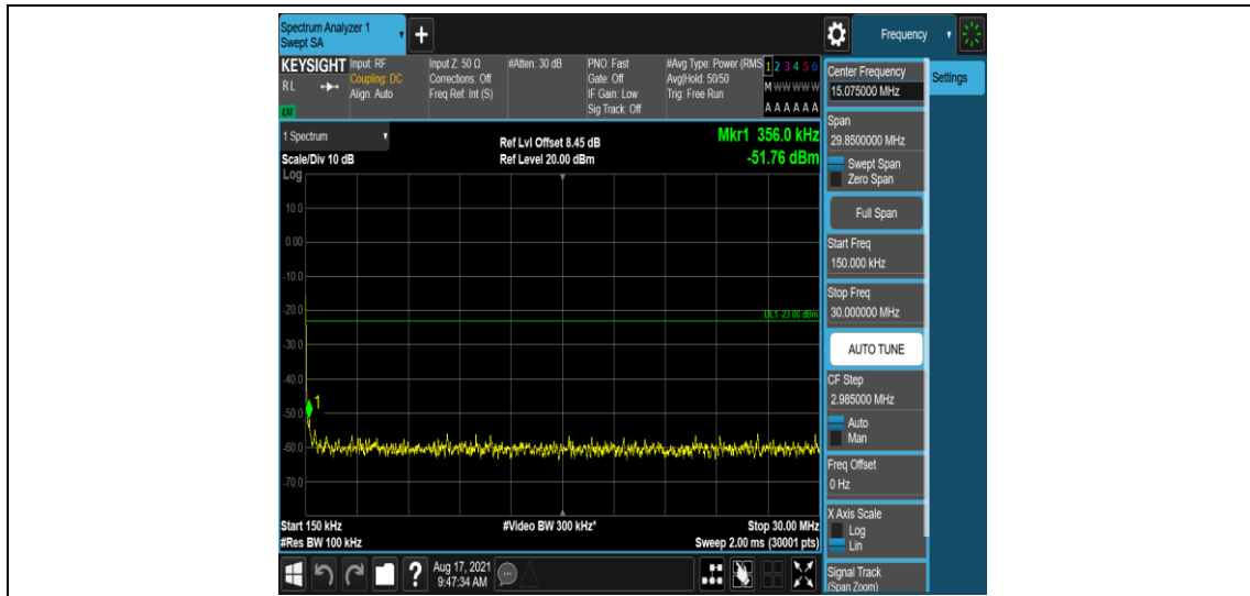
Band26-10MHz-16QAM-26990-1-0-High-0.15-30--51.76-PASS
