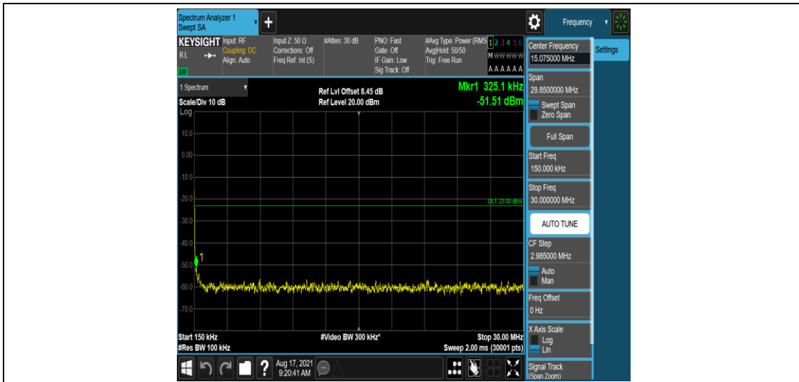
Band26-3MHz-QPSK-27025-1-0-High-0.15-30--51.51-PASS
