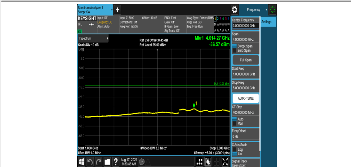
Band26-5MHz-QPSK-27015-1-0-High-1000-5000--36.57-PASS
