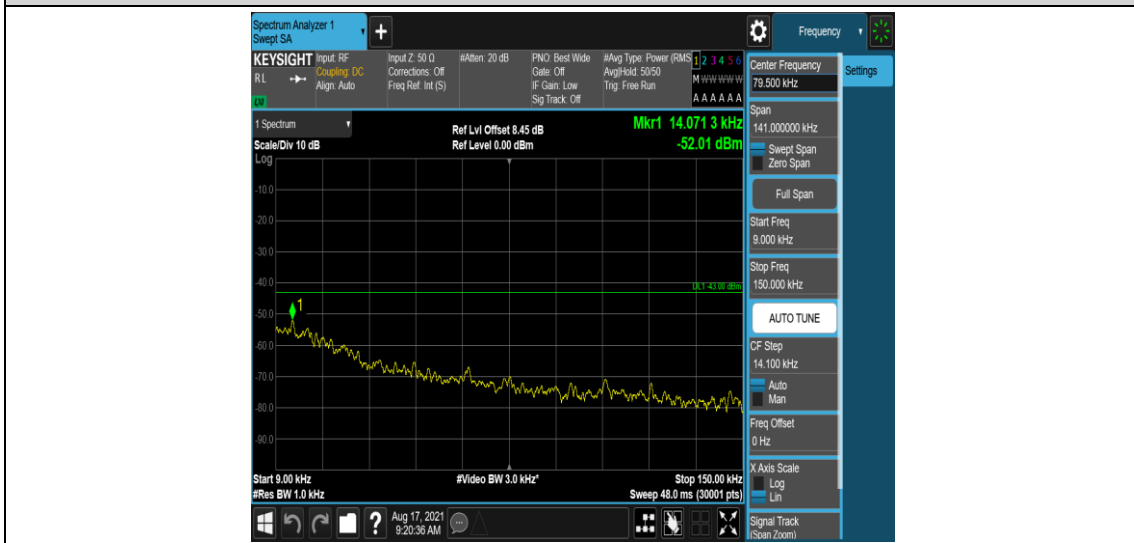
Band26-3MHz-QPSK-27025-1-0-High-0.009-0.15--52.01-PASS
