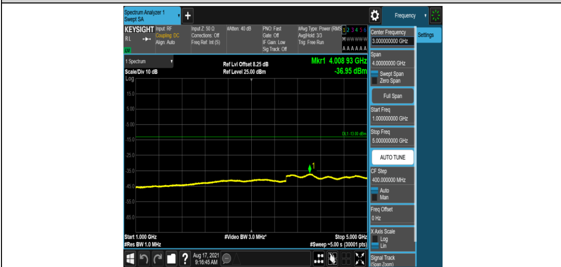
Band26-3MHz-16QAM-26805-1-0-Low-1000-5000--36.95-PASS
