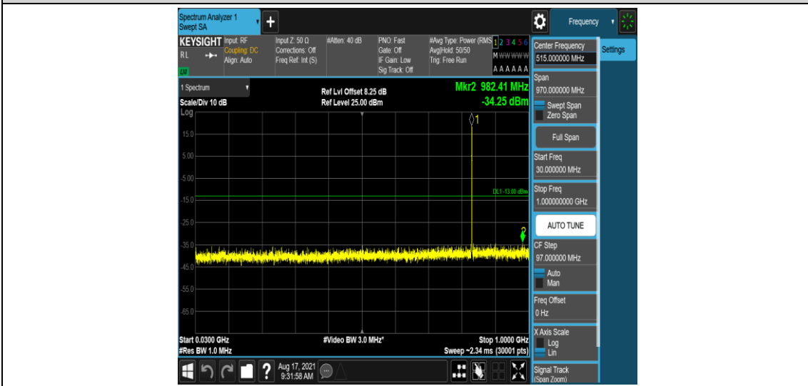
Band26-5MHz-16QAM-26915-1-0-Low-30-1000--34.25-PASS
