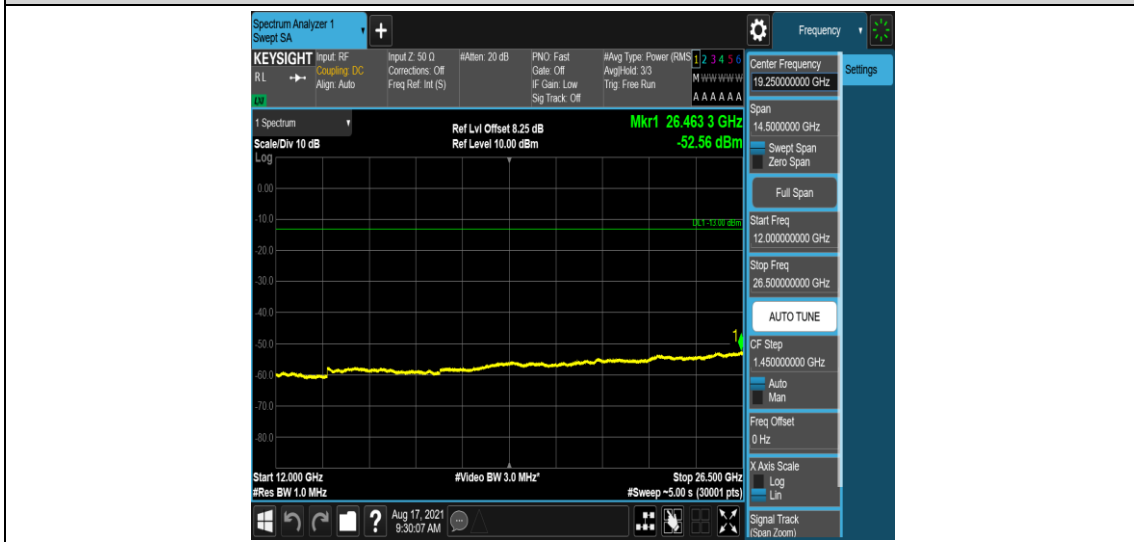
Band26-5MHz-16QAM-26815-1-0-Low-12000-26500--52.56-PASS
