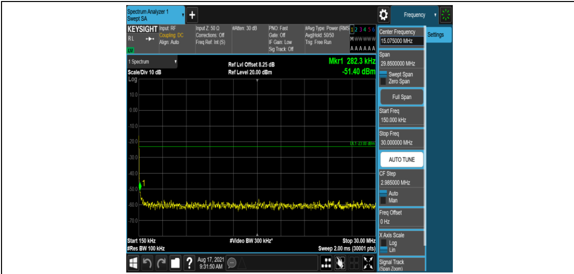
Band26-5MHz-16QAM-26915-1-0-Low-0.15-30--51.4-PASS
