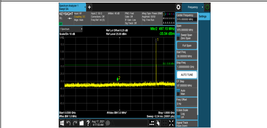
Band26-3MHz-QPSK-26915-1-0-Low-30-1000--35.54-PASS
