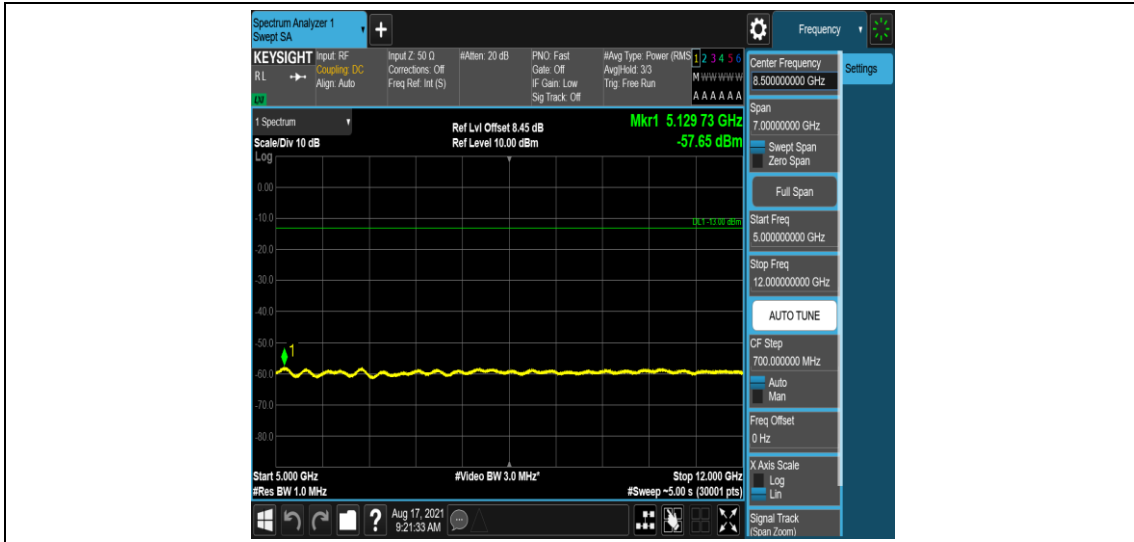
Band26-3MHz-QPSK-27025-1-0-High-5000-12000--57.65-PASS
