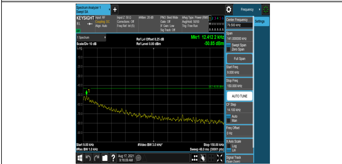
Band26-3MHz-16QAM-26805-1-0-Low-0.009-0.15--50.85-PASS
