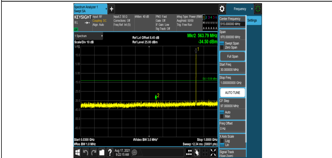
Band26-3MHz-16QAM-27025-1-0-High-30-1000--34.5-PASS
