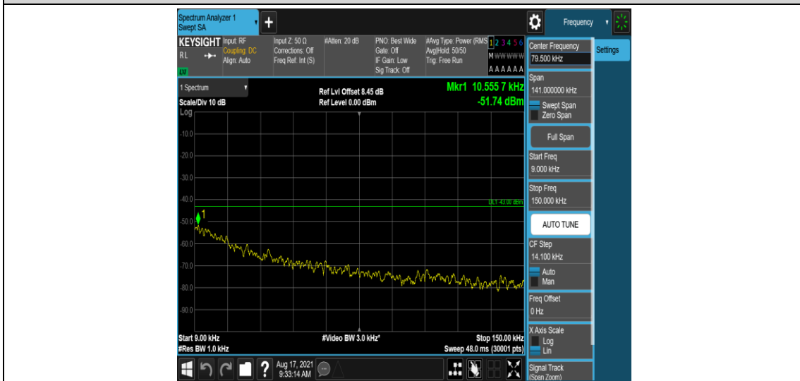
Band26-5MHz-QPSK-27015-1-0-High-0.009-0.15--51.75-PASS
