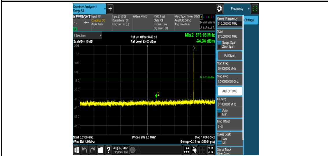
Band26-3MHz-QPSK-27025-1-0-High-30-1000--34.34-PASS
