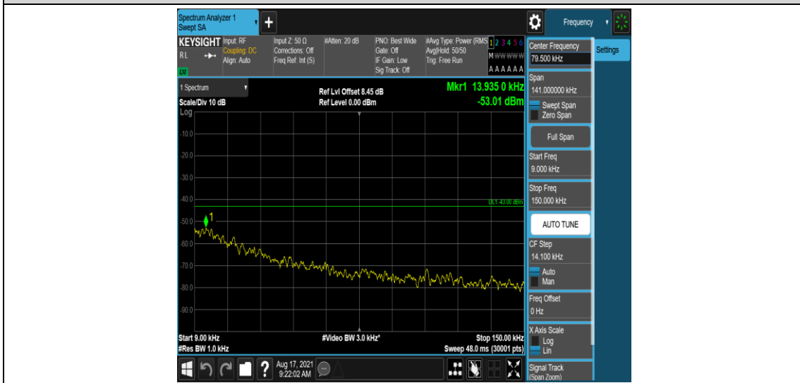
Band26-3MHz-16QAM-27025-1-0-High-0.009-0.15--53.01-PASS
