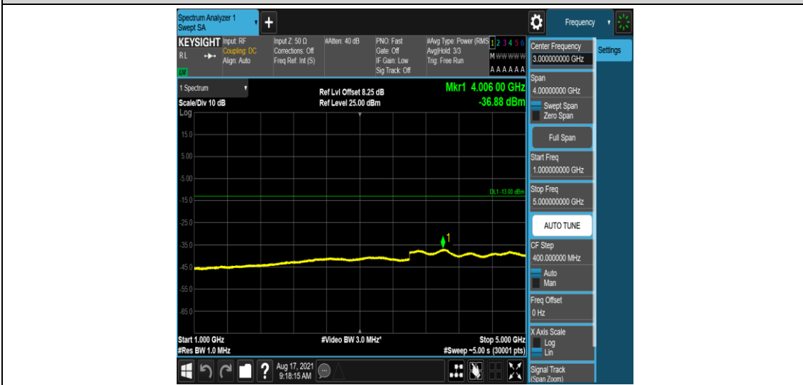
Band26-3MHz-QPSK-26915-1-0-Low-1000-5000--36.88-PASS
