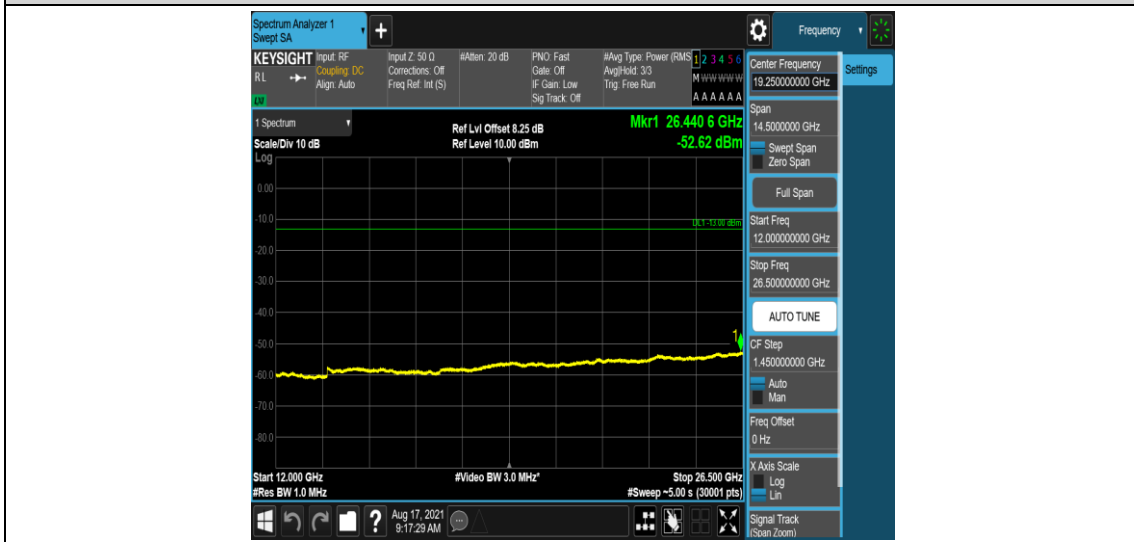
Band26-3MHz-16QAM-26805-1-0-Low-12000-26500--52.63-PASS
