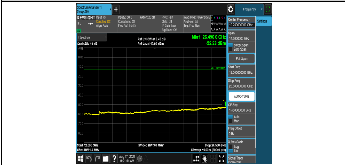
Band26-3MHz-QPSK-27025-1-0-High-12000-26500--52.23-PASS
