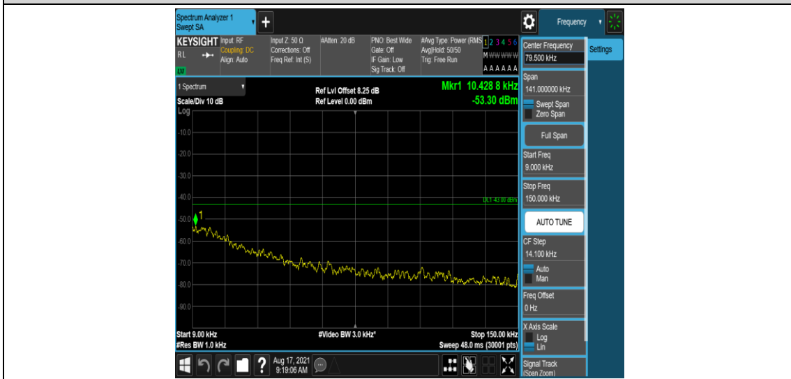
Band26-3MHz-16QAM-26915-1-0-Low-0.009-0.15--53.3-PASS
