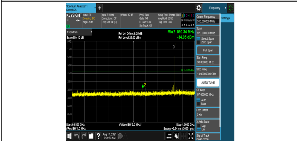
Band26-1.4MHz-16QAM-26915-1-0-Low-30-1000--34.05-PASS
