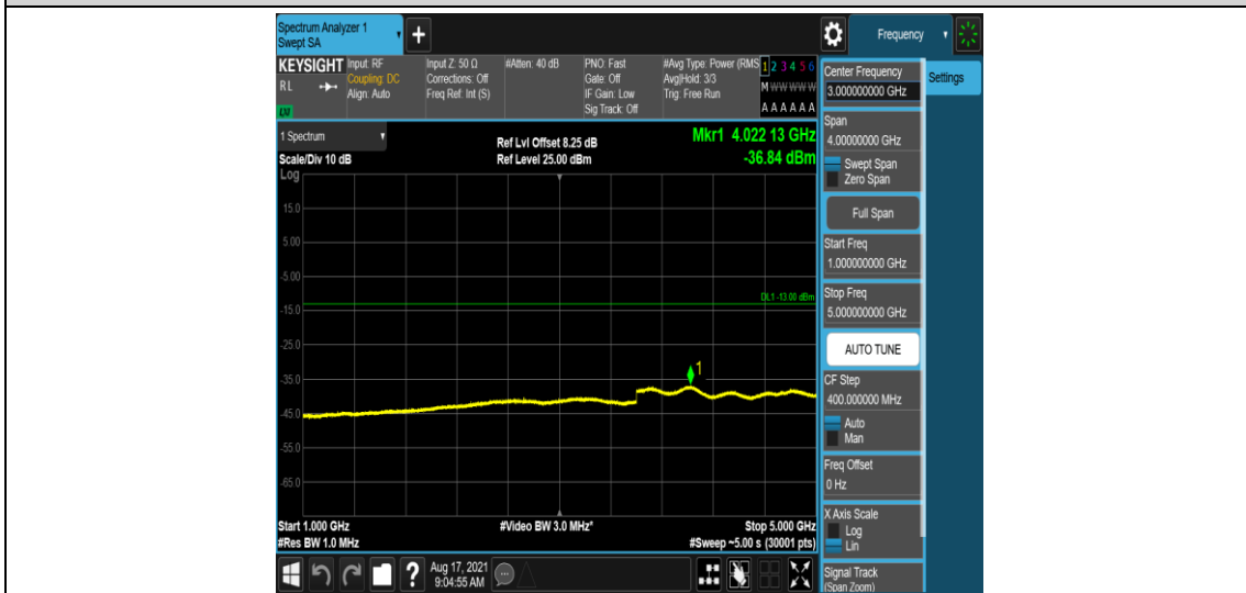
Band26-1.4MHz-16QAM-26915-1-0-Low-1000-5000--36.84-PASS
