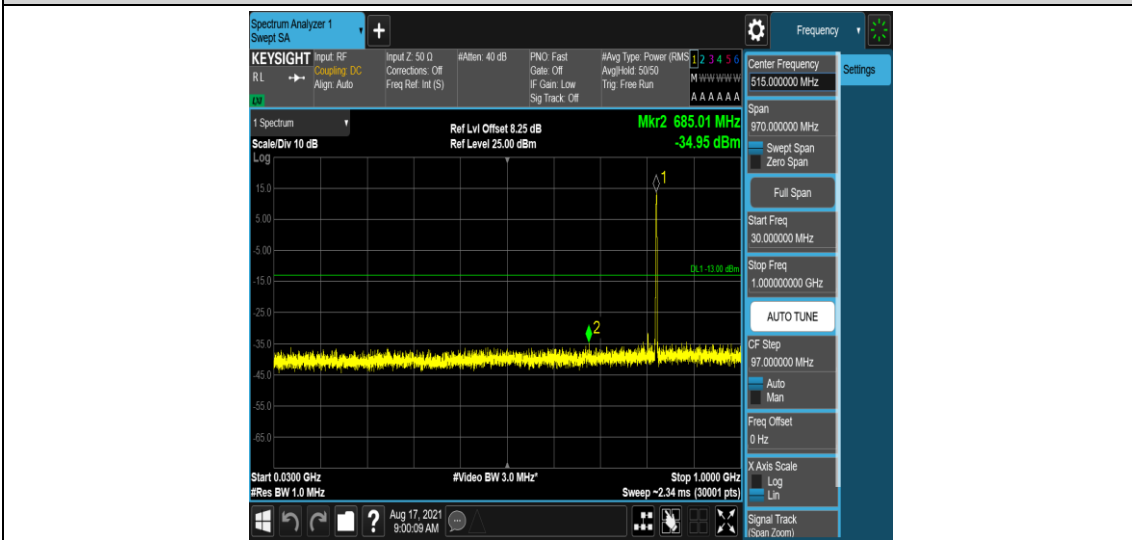
Band26-1.4MHz-QPSK-26797-1-0-Low-30-1000--34.95-PASS
