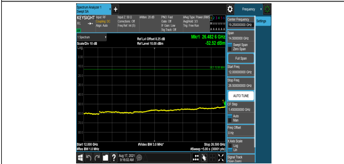
Band26-3MHz-QPSK-26805-1-0-Low-12000-26500--52.52-PASS
