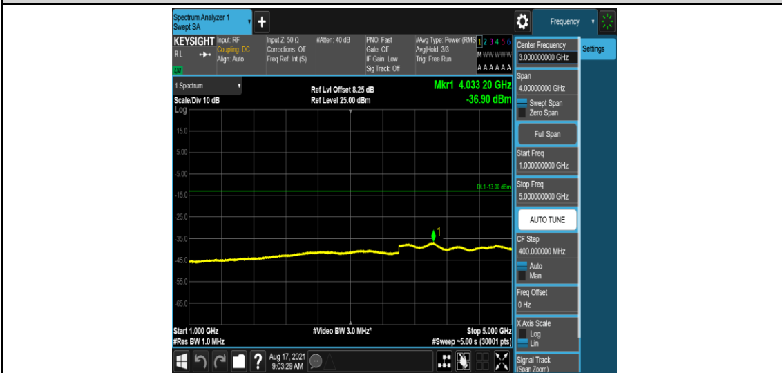
Band26-1.4MHz-QPSK-26915-1-0-Low-1000-5000--36.9-PASS
