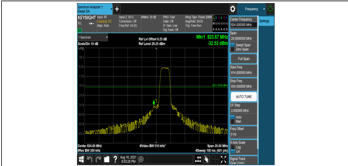
Band26-10MHz-16QAM-26840-6-0-Low--32.53-PASS
