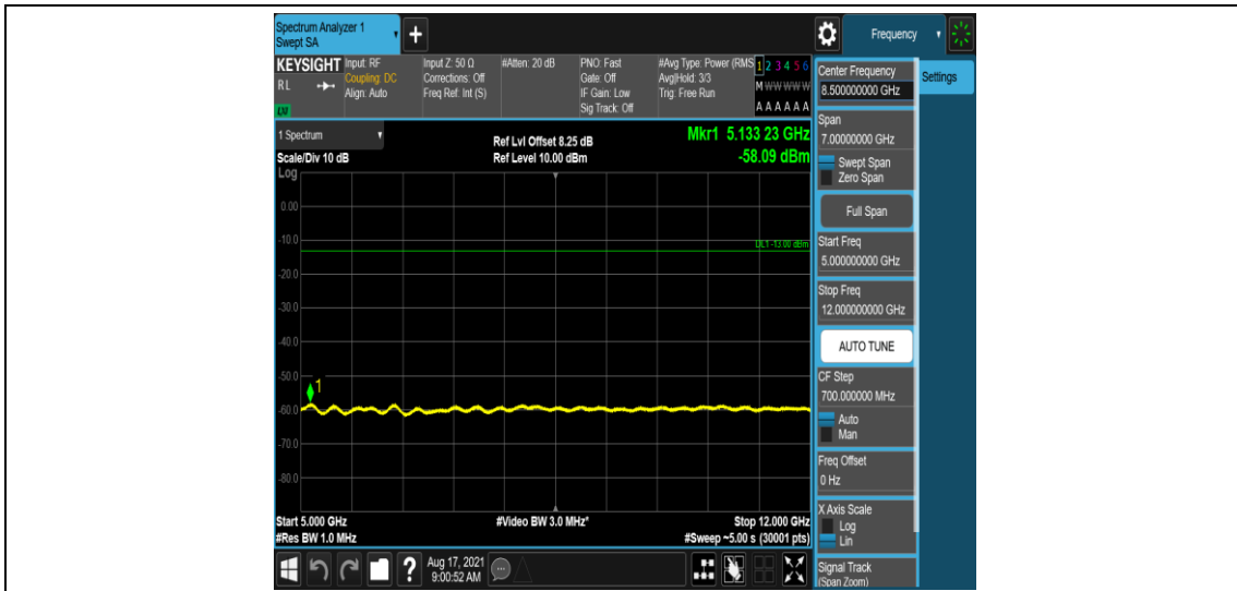
Band26-1.4MHz-QPSK-26797-1-0-Low-5000-12000--58.09-PASS
