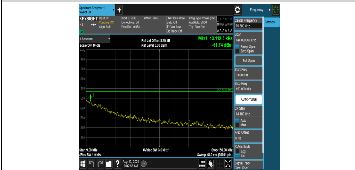
Band26-1.4MHz-QPSK-26915-1-0-Low-0.009-0.15--51.74-PASS
