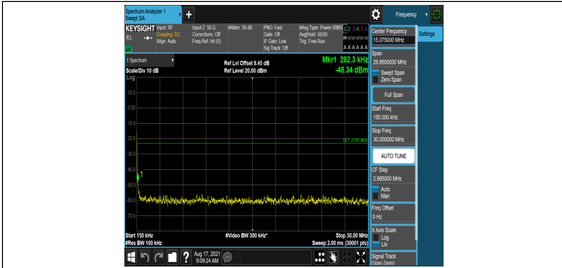
Band26-1.4MHz-16QAM-27033-1-0-High-0.15-30--48.34-PASS
