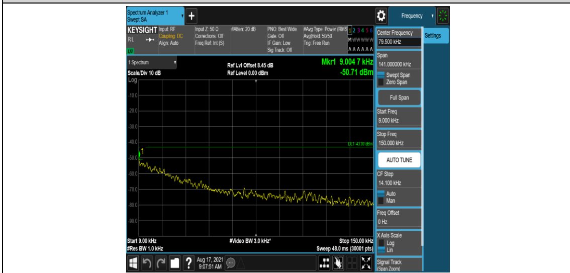
Band26-1.4MHz-QPSK-27033-1-0-High-0.009-0.15--50.71-PASS
