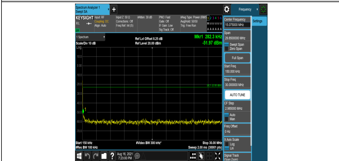
Band26-3MHz-16QAM-26775-1-0-High-0.15-30--51.97-PASS
