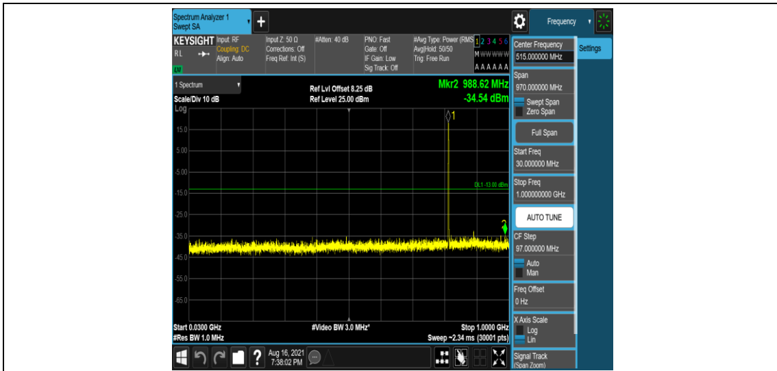
Band26-5MHz-QPSK-26740-1-0-Low-30-1000--34.54-PASS
