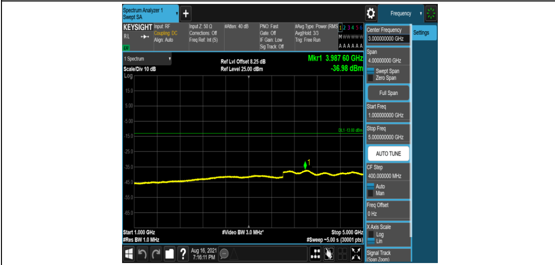
Band26-3MHz-QPSK-26705-1-0-Low-1000-5000--36.98-PASS
