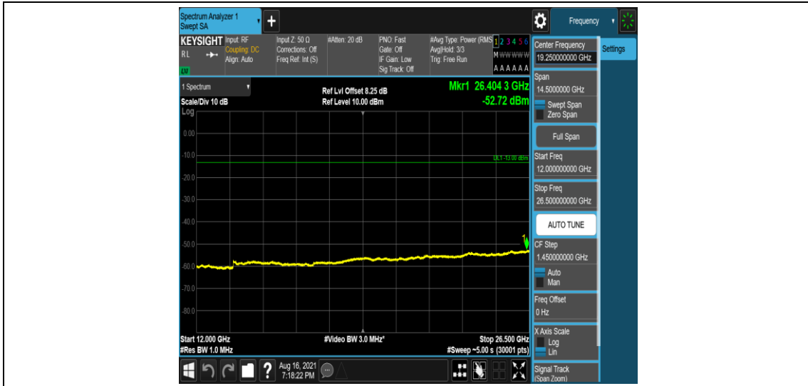
Band26-3MHz-16QAM-26705-1-0-Low-12000-26500--52.72-PASS
