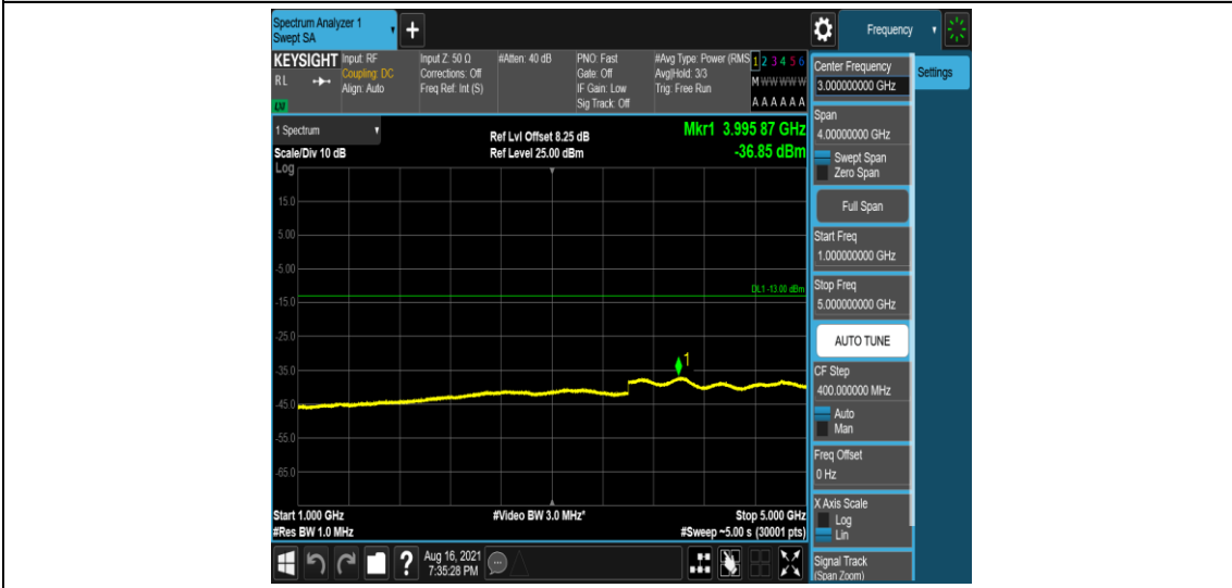
Band26-5MHz-QPSK-26715-1-0-Low-1000-5000--36.85-PASS
