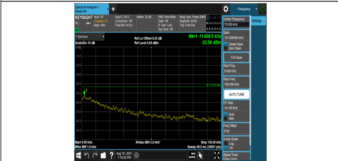
Band26-3MHz-QPSK-26740-1-0-Low-0.009-0.15--52.59-PASS
