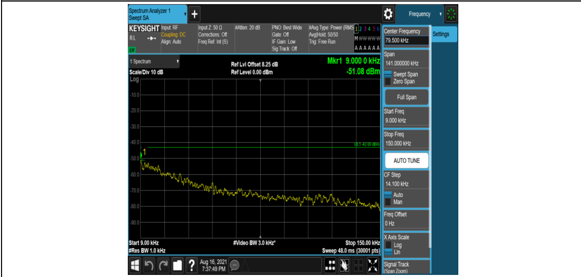
Band26-5MHz-QPSK-26740-1-0-Low-0.009-0.15--51.08-PASS
