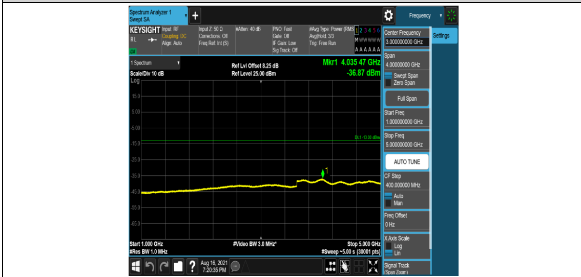
Band26-3MHz-16QAM-26740-1-0-Low-1000-5000--36.87-PASS
