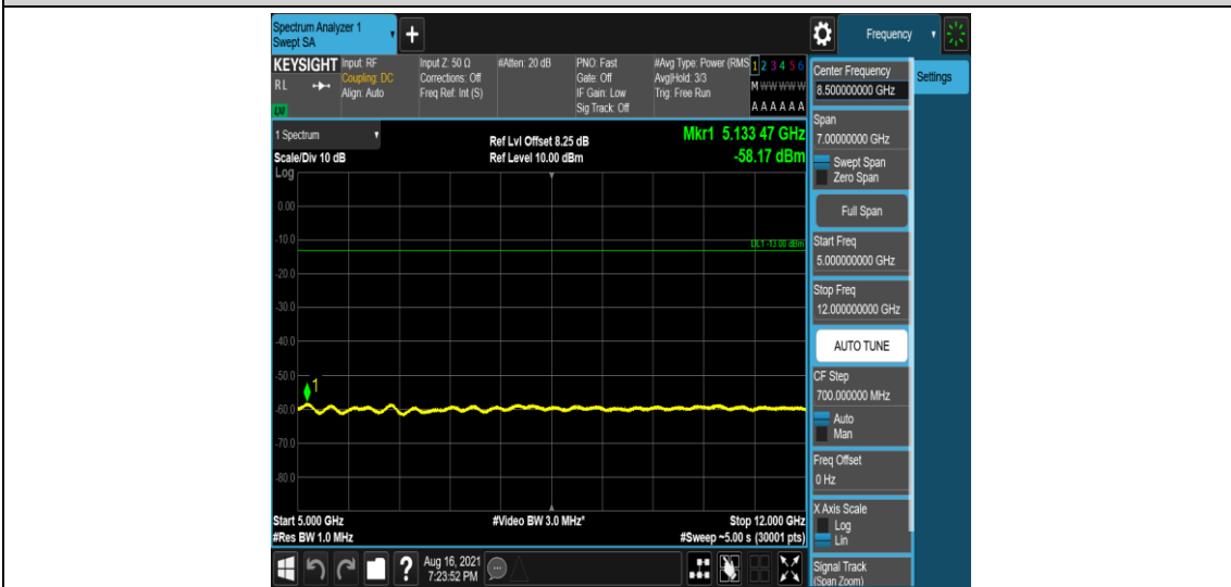
Band26-3MHz-16QAM-26775-1-0-High-5000-12000--58.17-PASS
