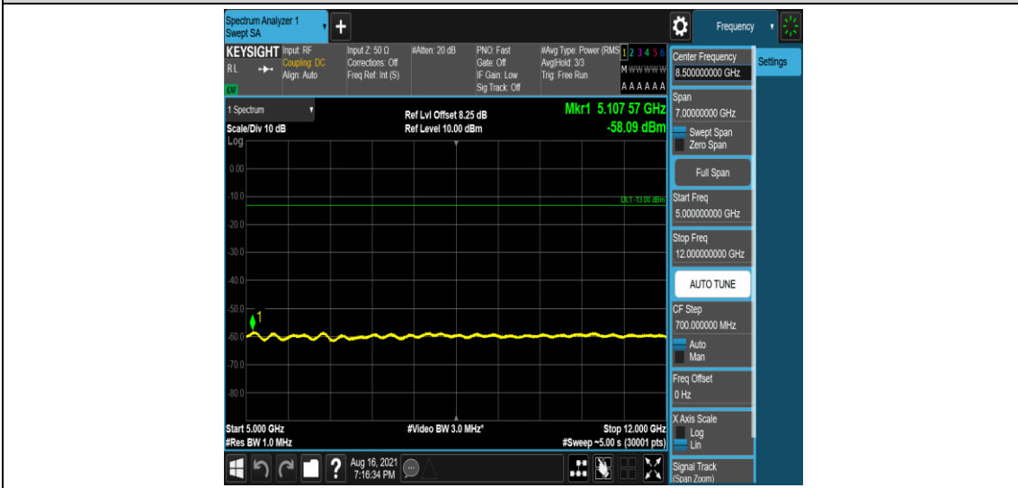
Band26-3MHz-QPSK-26705-1-0-Low-5000-12000--58.09-PASS
