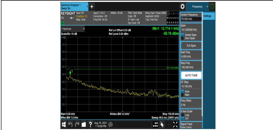
Band26-3MHz-16QAM-26740-1-0-Low-0.009-0.15--50.76-PASS
