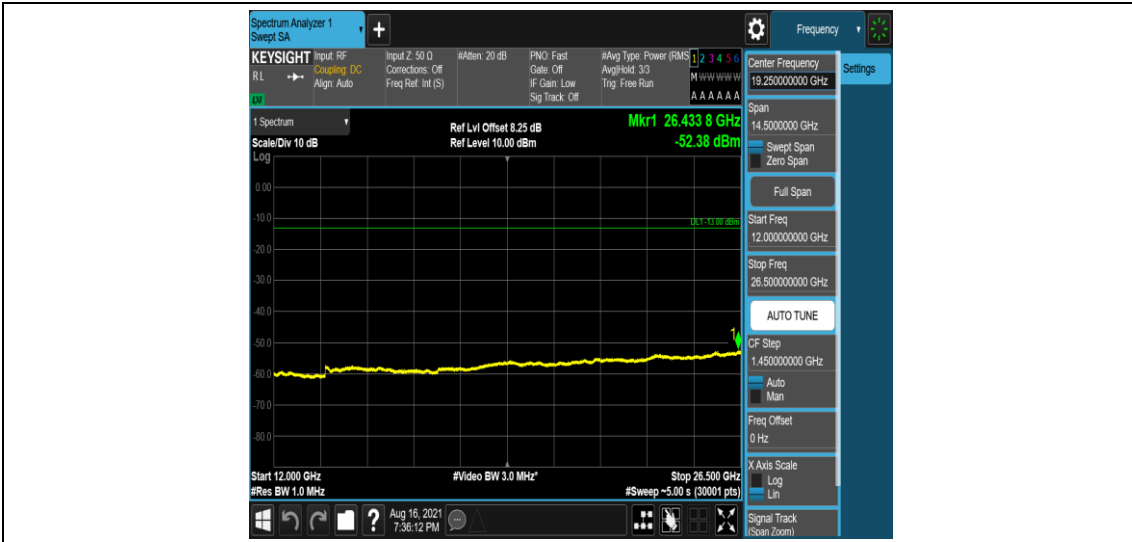
Band26-5MHz-QPSK-26715-1-0-Low-12000-26500--52.38-PASS
