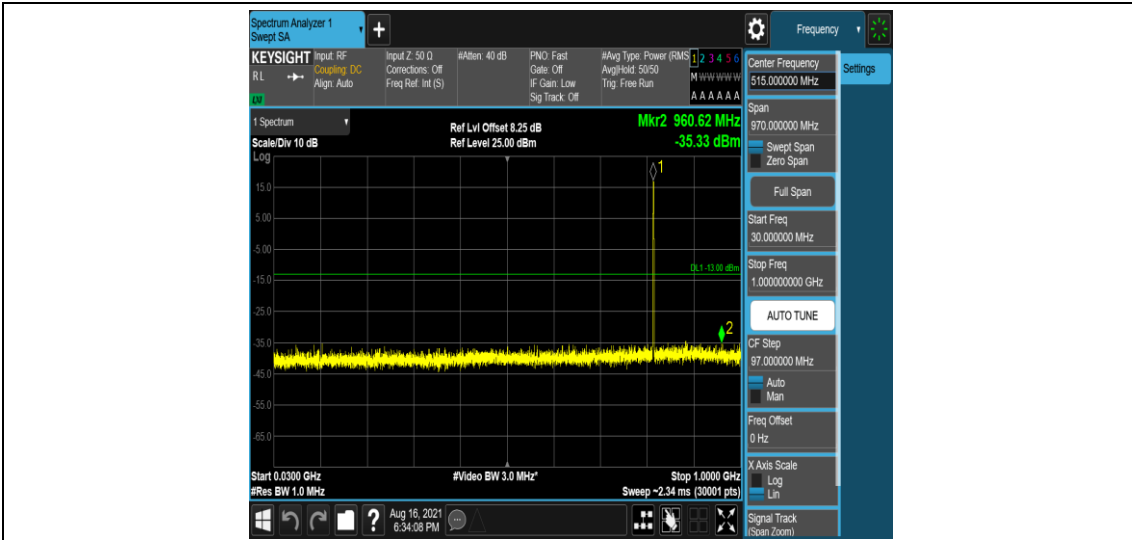
Band26-1.4MHz-16QAM-26740-1-0-Low-30-1000--35.33-PASS
