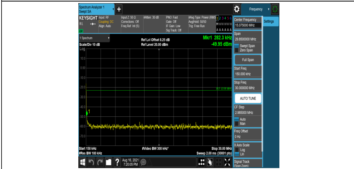
Band26-3MHz-16QAM-26740-1-0-Low-0.15-30--49.95-PASS
