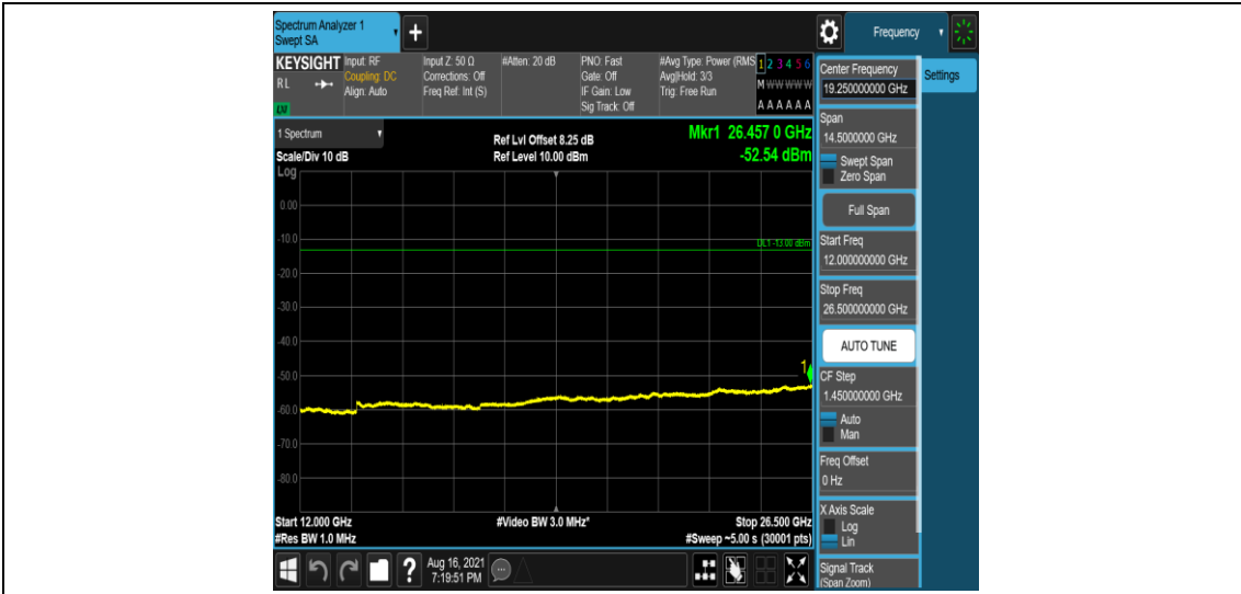
Band26-3MHz-QPSK-26740-1-0-Low-12000-26500--52.54-PASS
