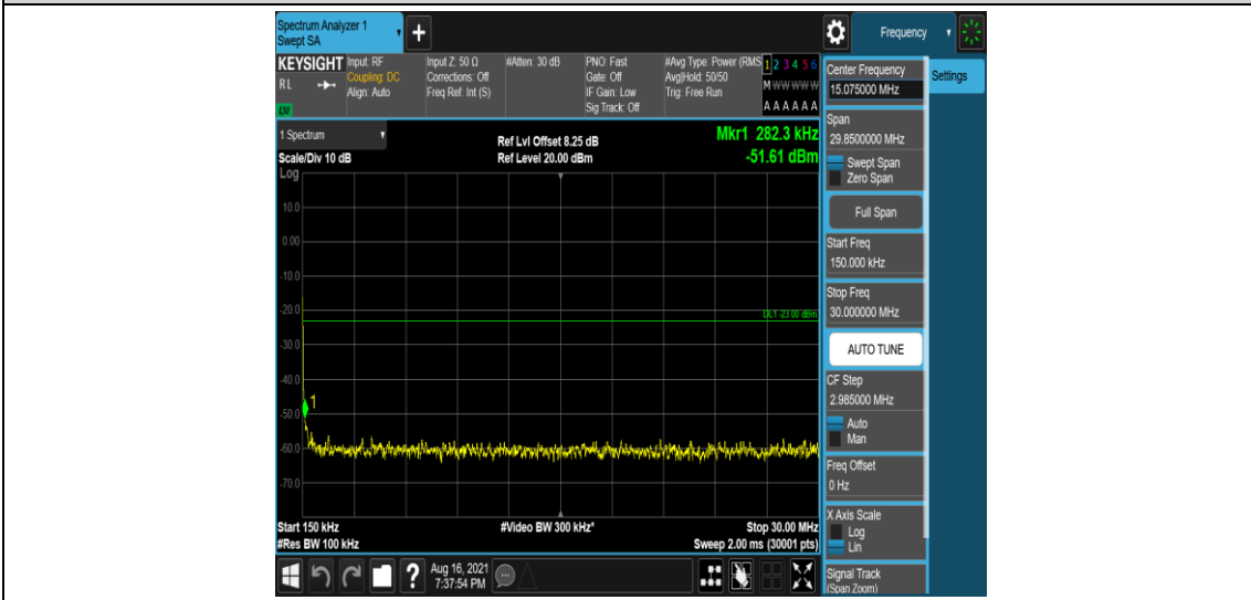
Band26-5MHz-QPSK-26740-1-0-Low-0.15-30--51.61-PASS
