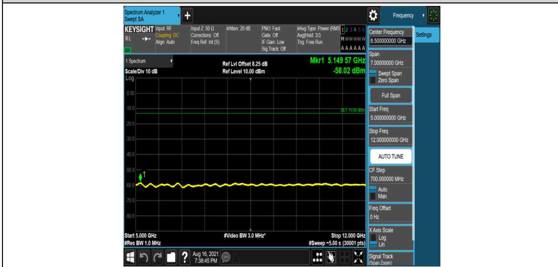
Band26-5MHz-QPSK-26740-1-0-Low-5000-12000--58.02-PASS
