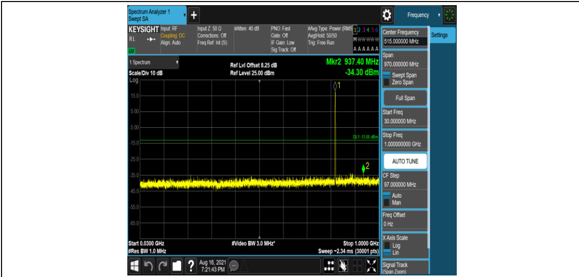
Band26-3MHz-QPSK-26775-1-0-High-30-1000--34.3-PASS
