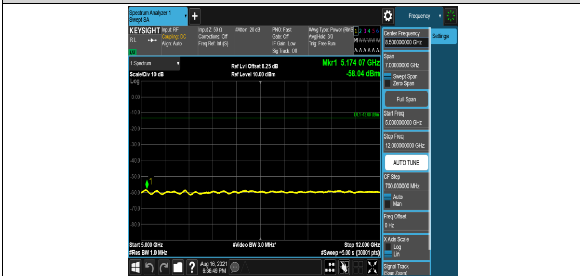
Band26-1.4MHz-QPSK-26783-1-0-High-5000-12000--58.04-PASS
