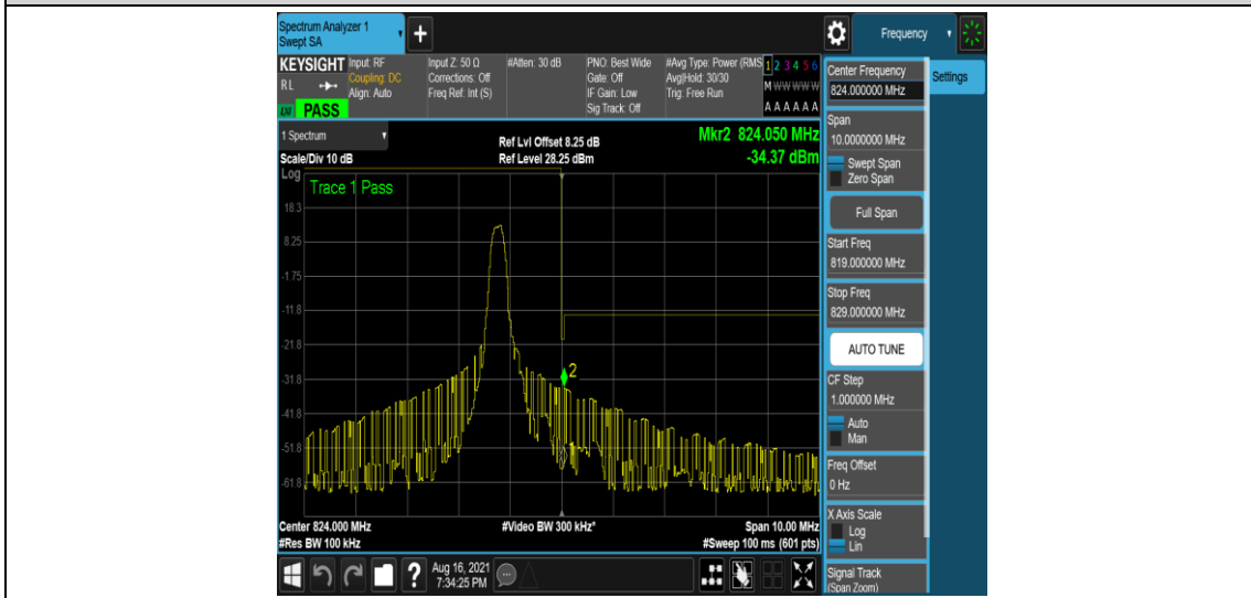
Band26-5MHz-16QAM-26765-1-0-High--57.13,-34.37-PASS
