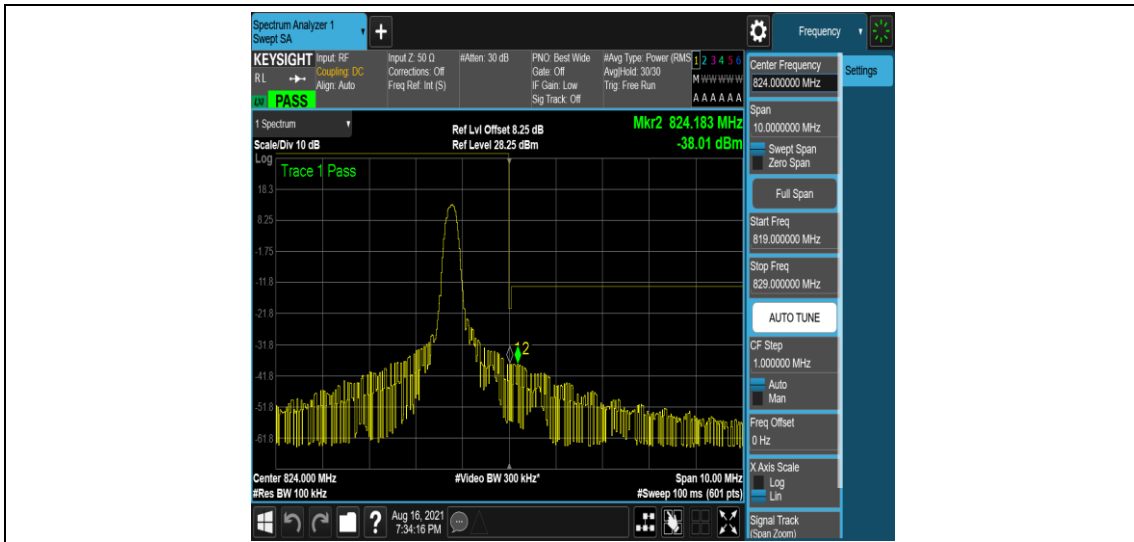
Band26-5MHz-QPSK-26765-1-0-High--37.98,-38.01-PASS
