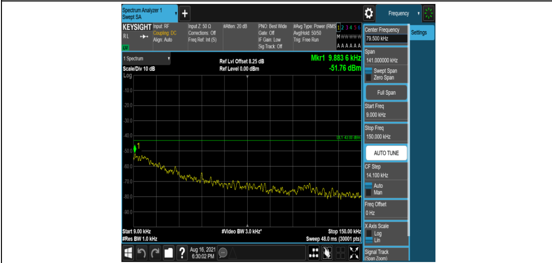
Band26-1.4MHz-16QAM-26697-1-0-Low-0.009-0.15--51.76-PASS
