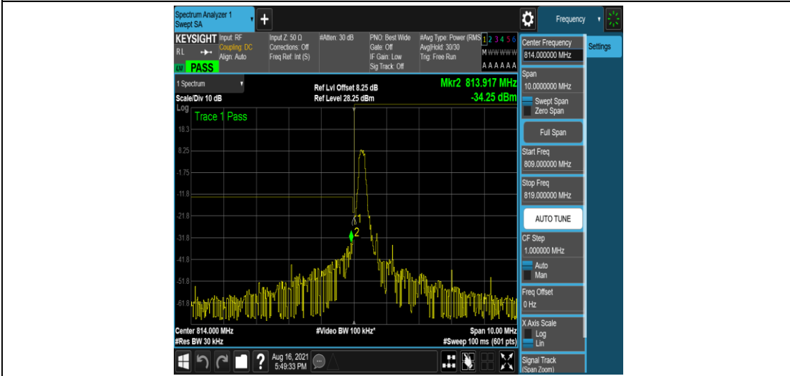
Band26-1.4MHz-16QAM-26697-1-0-Low--28.16,-34.25-PASS
