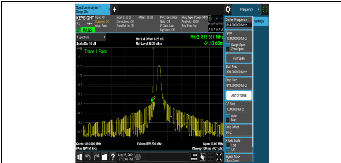
Band26-3MHz-16QAM-26705-1-0-Low--29.83,-31.13-PASS
