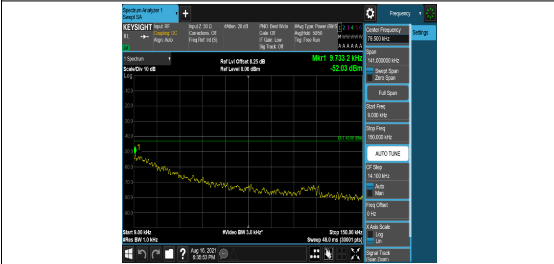
Band26-1.4MHz-QPSK-26783-1-0-High-0.009-0.15--52.03-PASS
