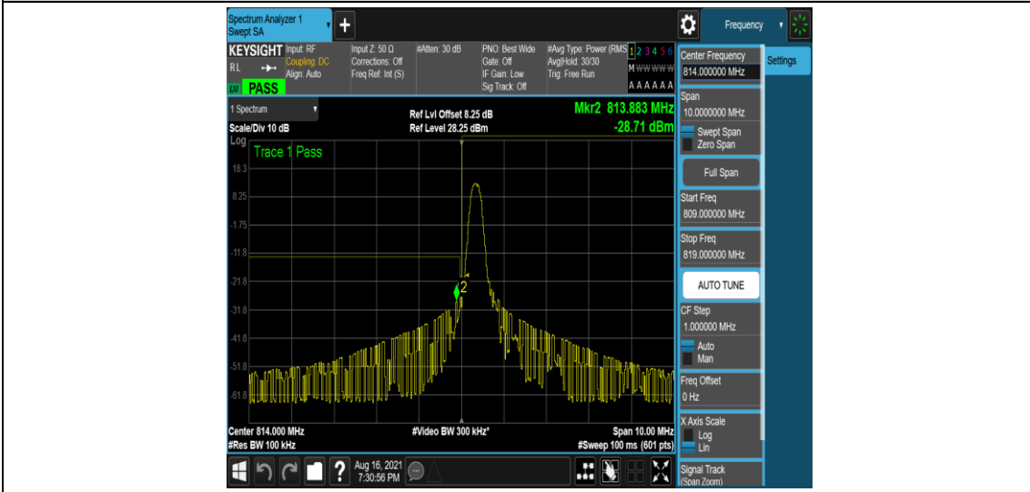
Band26-5MHz-QPSK-26715-1-0-Low--25.84,-28.71-PASS
