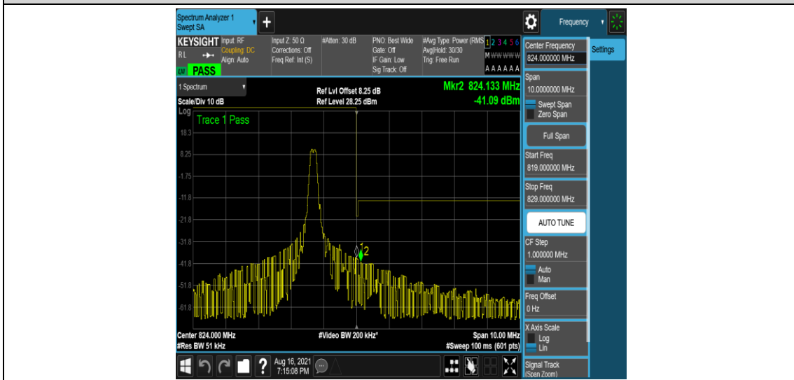
Band26-3MHz-16QAM-26775-1-0-High--39.44,-41.09-PASS
