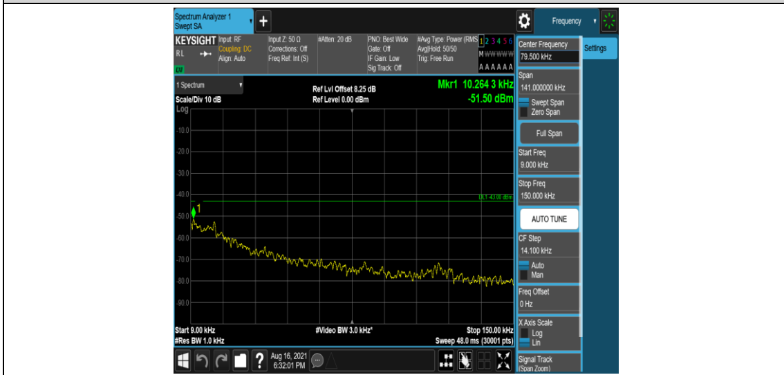
Band26-1.4MHz-QPSK-26740-1-0-Low-0.009-0.15--51.5-PASS
