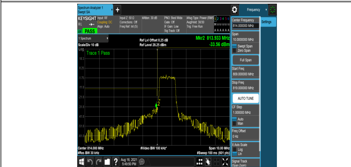
Band26-1.4MHz-16QAM-26697-6-0-Low--31.06,-33.56-PASS
