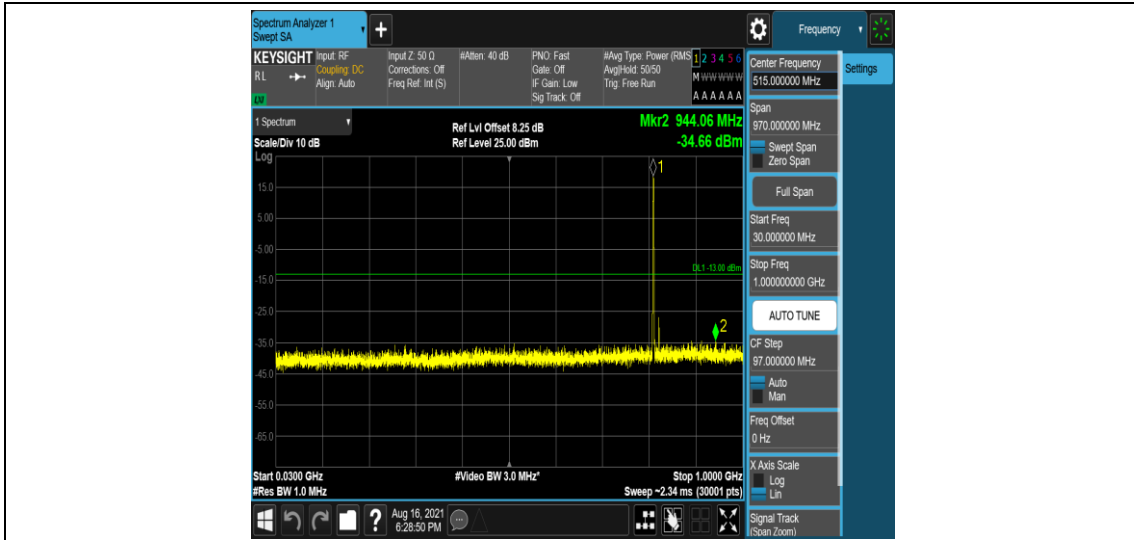
Band26-1.4MHz-QPSK-26697-1-0-Low-30-1000--34.66-PASS
