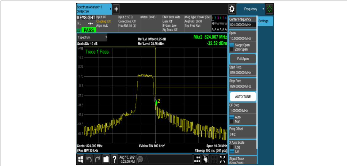
Band26-1.4MHz-QPSK-26783-6-0-High--31.22,-32.52-PASS
