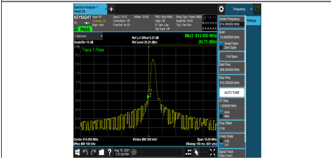
Band26-5MHz-16QAM-26715-1-0-Low--25.87,-30.71-PASS
