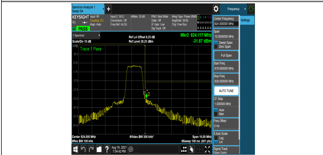
Band26-5MHz-16QAM-26765-6-0-High--29.02,-31.87-PASS
