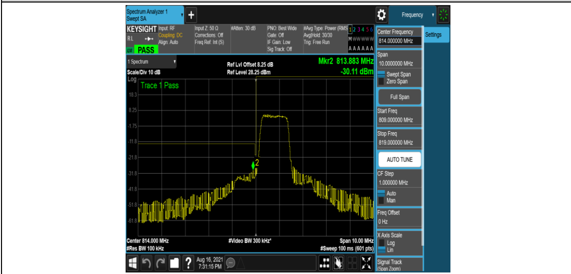
Band26-5MHz-QPSK-26715-6-0-Low--28.36,-30.11-PASS
