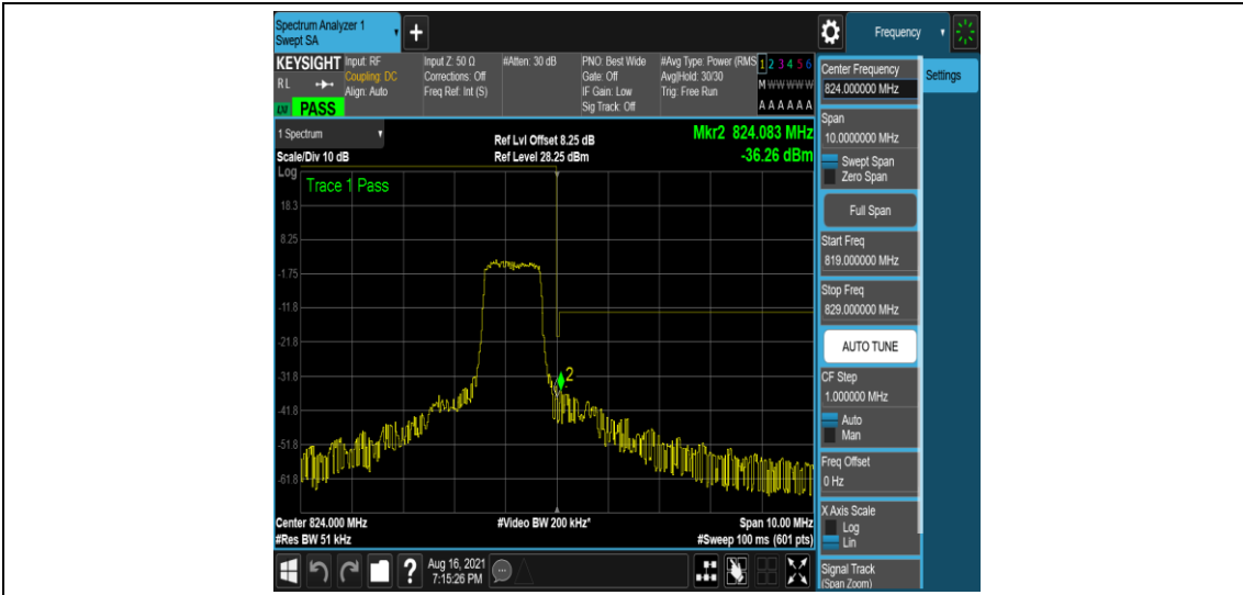
Band26-3MHz-16QAM-26775-6-0-High--38.31,-36.26-PASS
