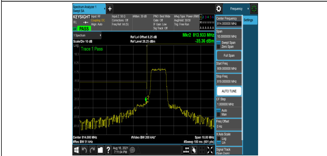
Band26-3MHz-16QAM-26705-6-0-Low--33.84,-35.36-PASS
