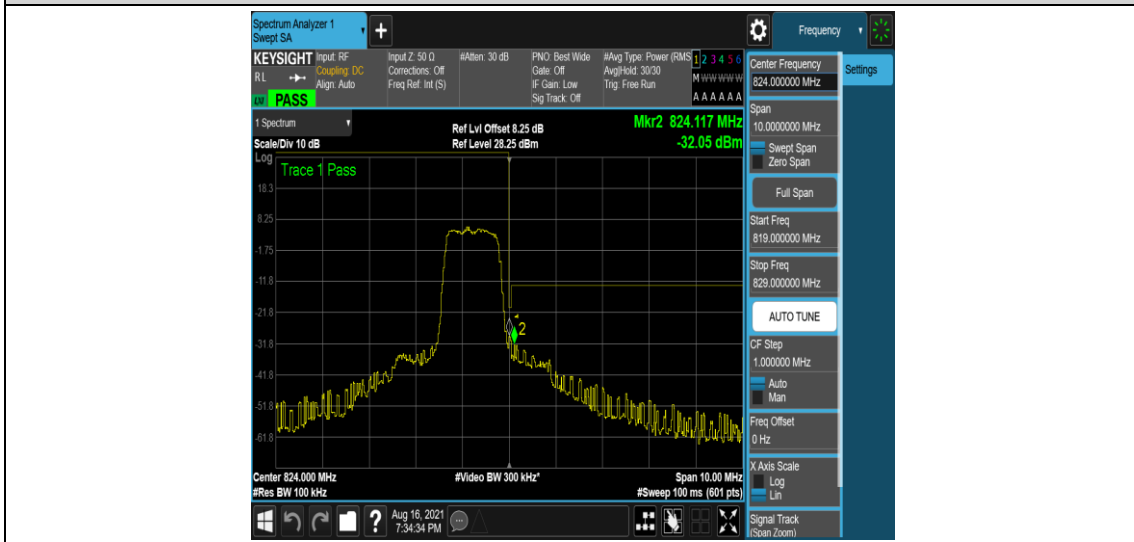
Band26-5MHz-QPSK-26765-6-0-High--29.36,-32.05-PASS
