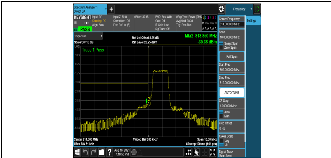
Band26-3MHz-QPSK-26705-6-0-Low--33.99,-35.38-PASS
