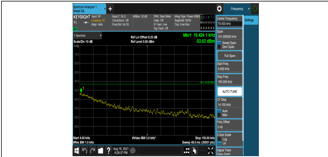
Band26-1.4MHz-QPSK-26697-1-0-Low-0.009-0.15--53.02-PASS
