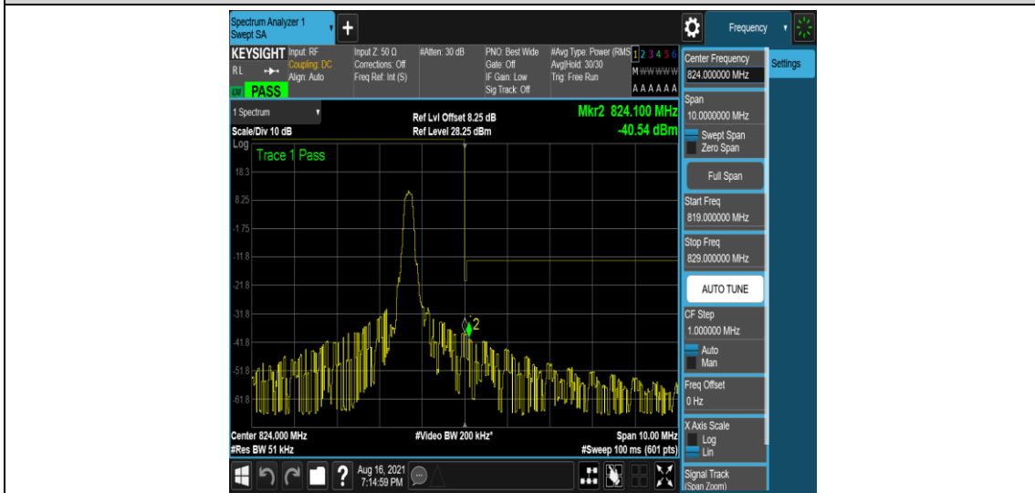
Band26-3MHz-QPSK-26775-1-0-High--38.93,-40.54-PASS
