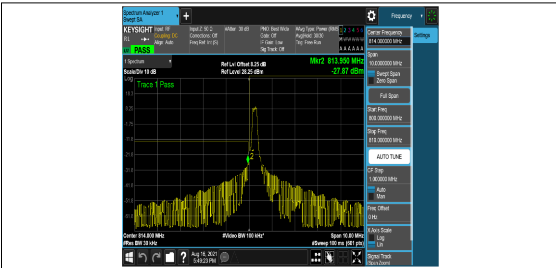
Band26-1.4MHz-QPSK-26697-1-0-Low--25.52,-27.87-PASS
