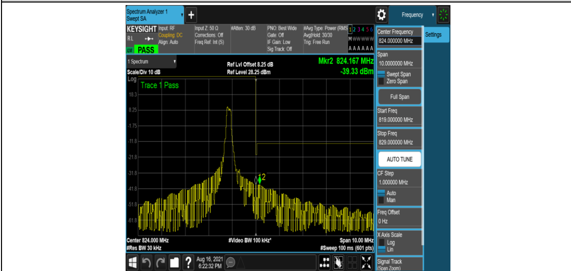
Band26-1.4MHz-QPSK-26783-1-0-High--39.71,-39.33-PASS
