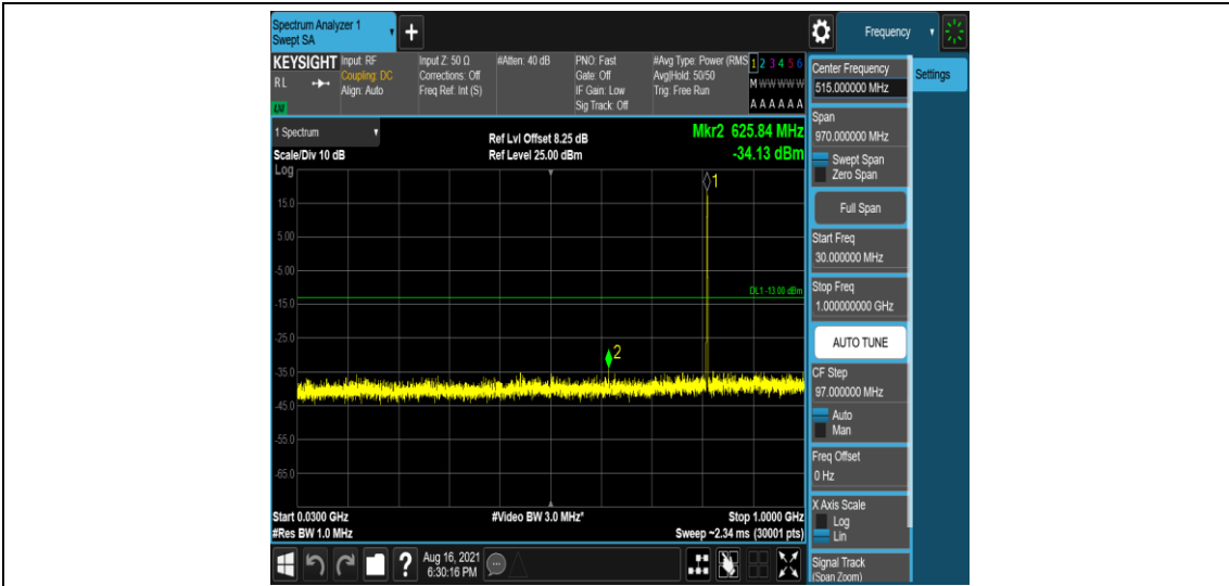
Band26-1.4MHz-16QAM-26697-1-0-Low-30-1000--34.13-PASS
