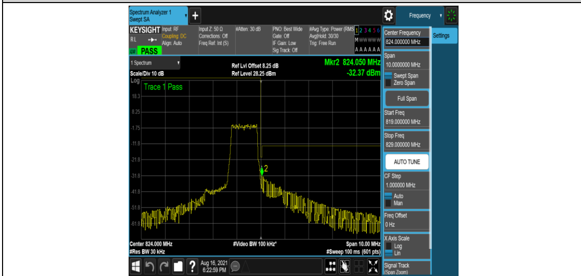
Band26-1.4MHz-16QAM-26783-6-0-High--31.38,-32.37-PASS
