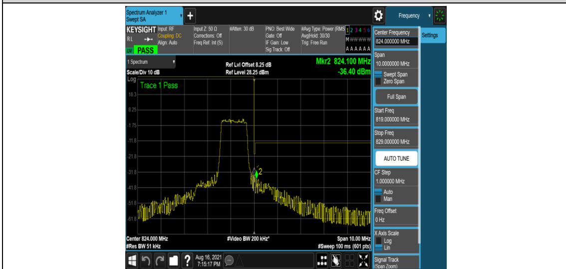
Band26-3MHz-QPSK-26775-6-0-High--34.74,-36.40-PASS
