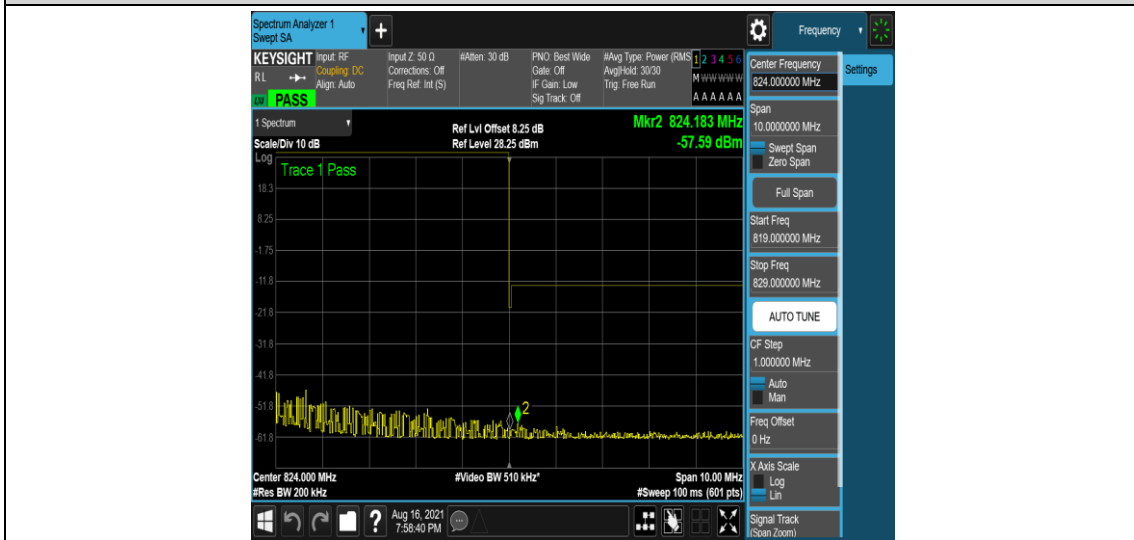
Band26-10MHz-QPSK-26740-6-0-Low--59.68,-57.59-PASS
