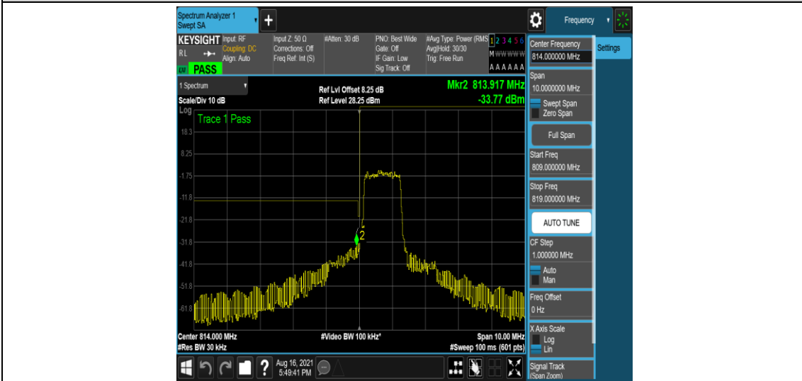
Band26-1.4MHz-QPSK-26697-6-0-Low--31.40,-33.77-PASS
