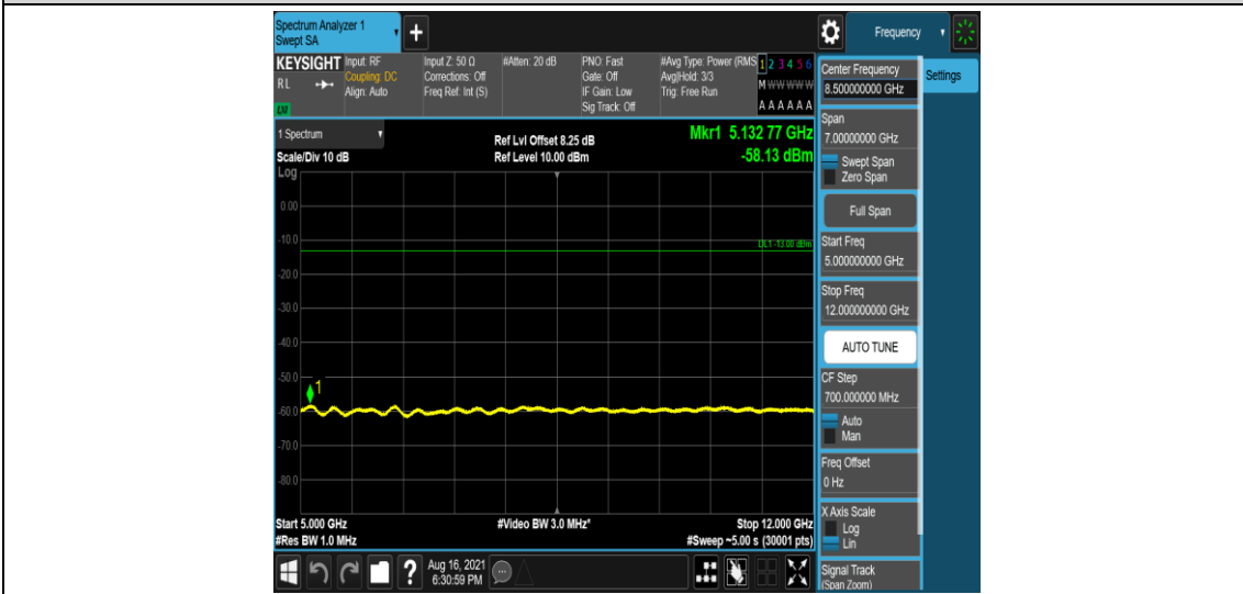
Band26-1.4MHz-16QAM-26697-1-0-Low-5000-12000--58.13-PASS
