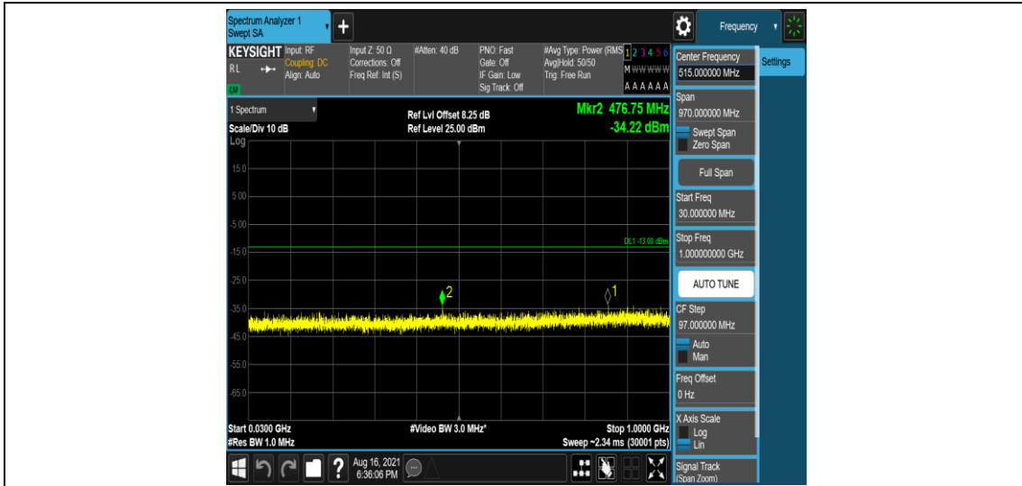
Band26-1.4MHz-QPSK-26783-1-0-High-30-1000--34.22-PASS
