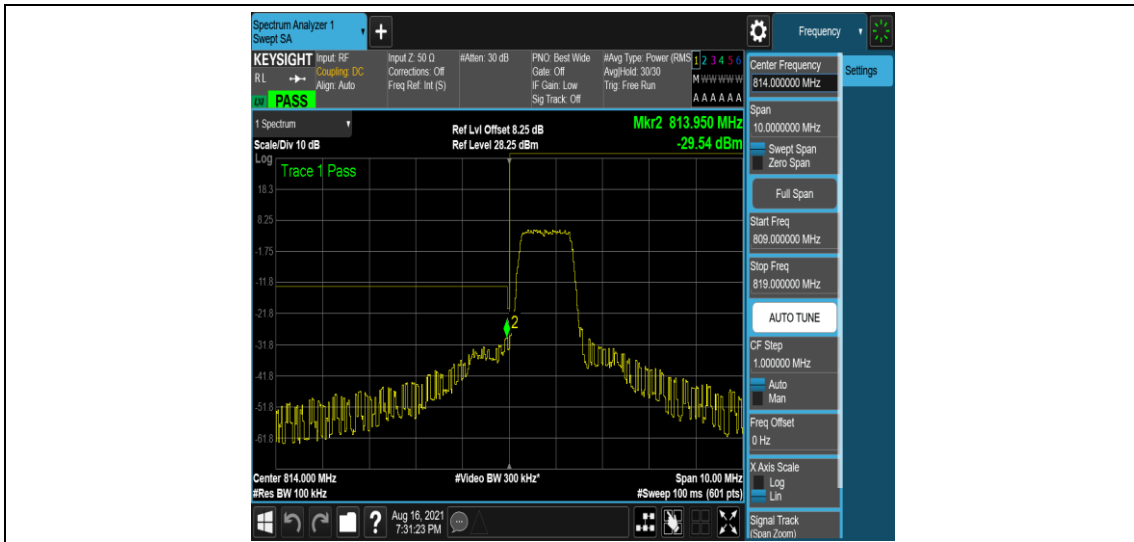
Band26-5MHz-16QAM-26715-6-0-Low--29.15,-29.54-PASS
