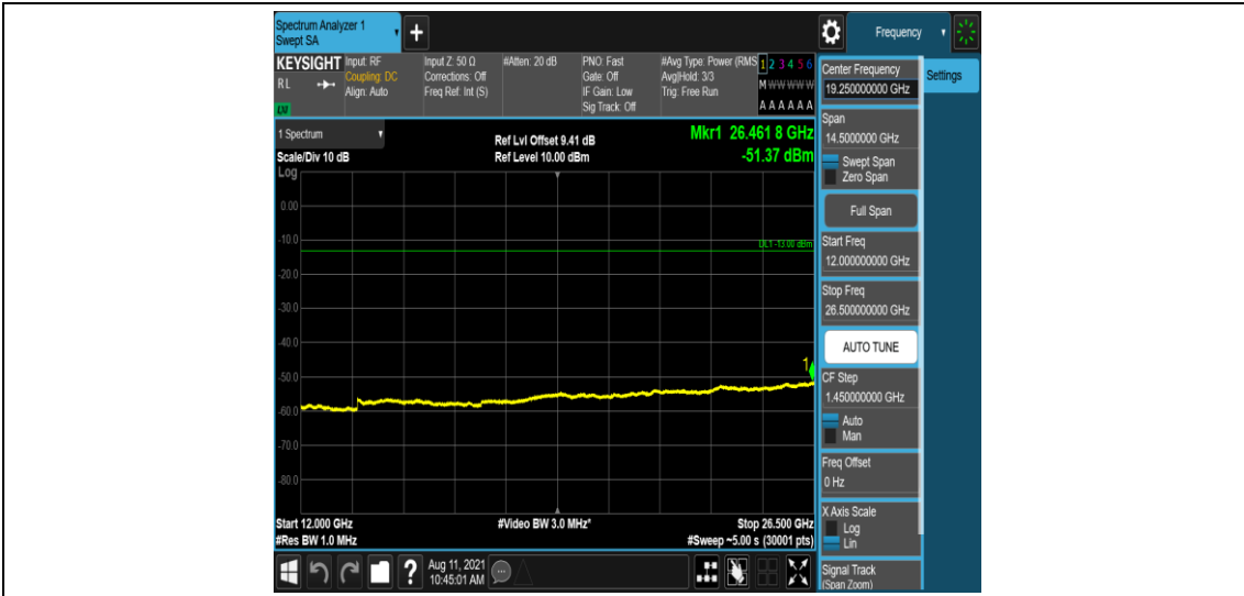
Band25-15MHz-16QAM-26365-1-0-Low-12000-26500--51.37-PASS
