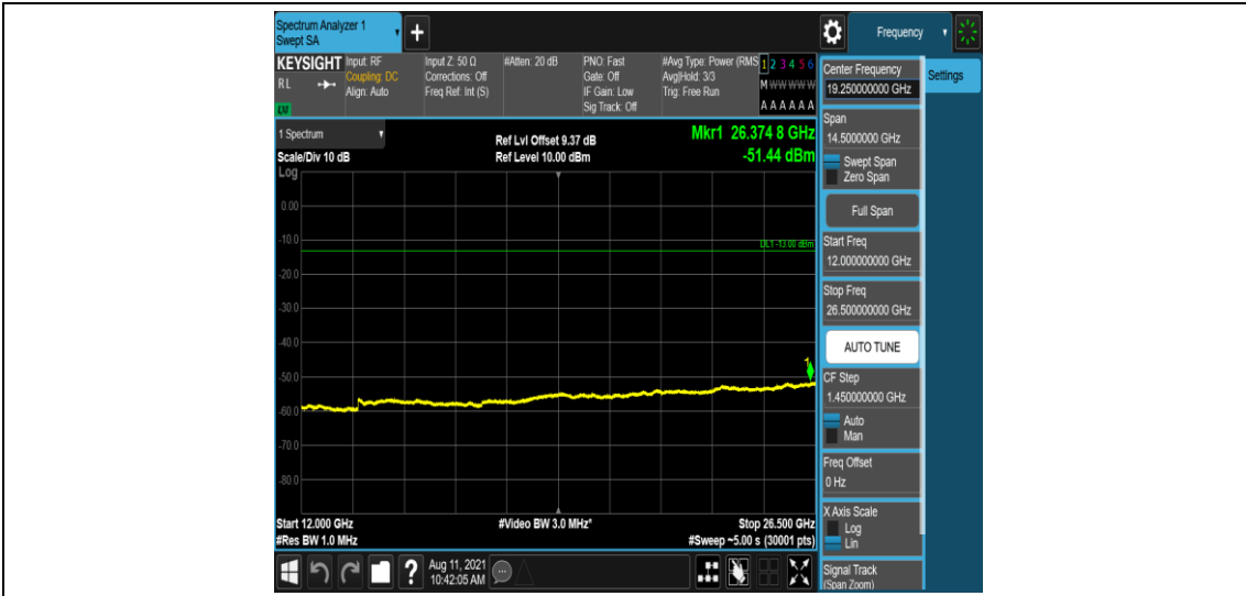
Band25-15MHz-16QAM-26115-1-0-Low-12000-26500--51.44-PASS
