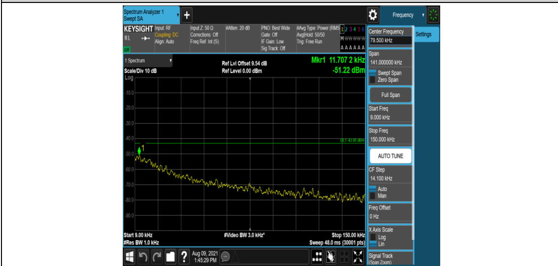
Band25-10MHz-16QAM-26640-1-0-High-0.009-0.15--51.22-PASS
