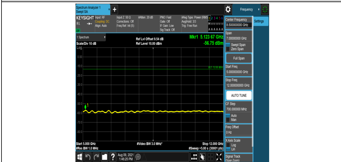
Band25-10MHz-16QAM-26640-1-0-High-5000-12000--56.75-PASS
