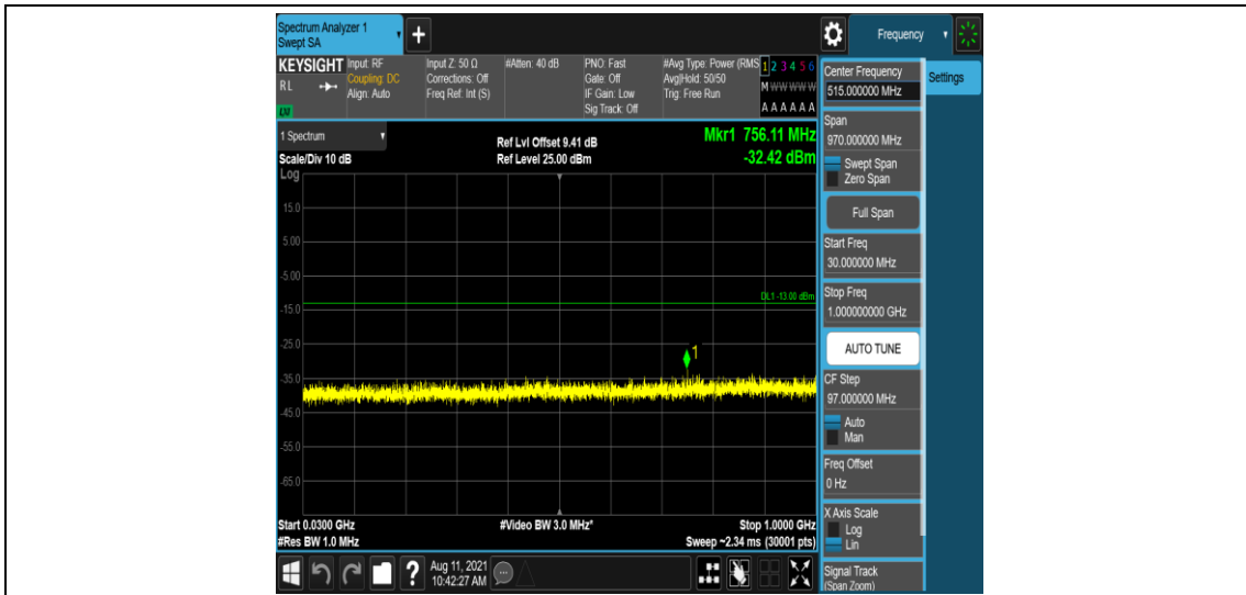
Band25-15MHz-QPSK-26365-1-0-Low-30-1000--32.42-PASS
