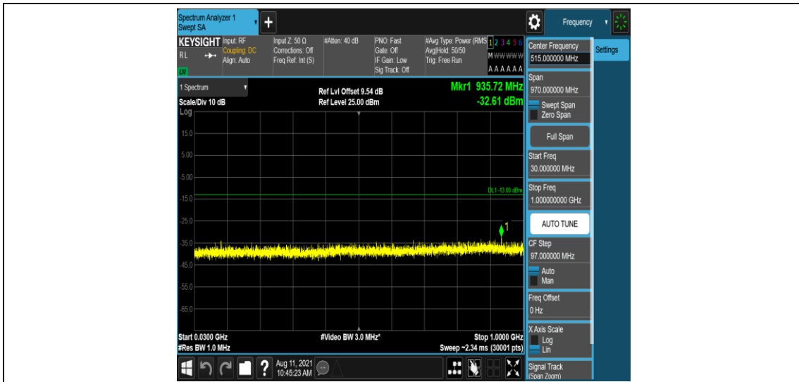
Band25-15MHz-QPSK-26615-1-0-High-30-1000--32.61-PASS
