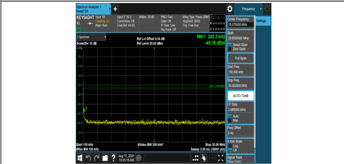
Band25-15MHz-QPSK-26615-1-0-High-0.15-30--49.76-PASS
