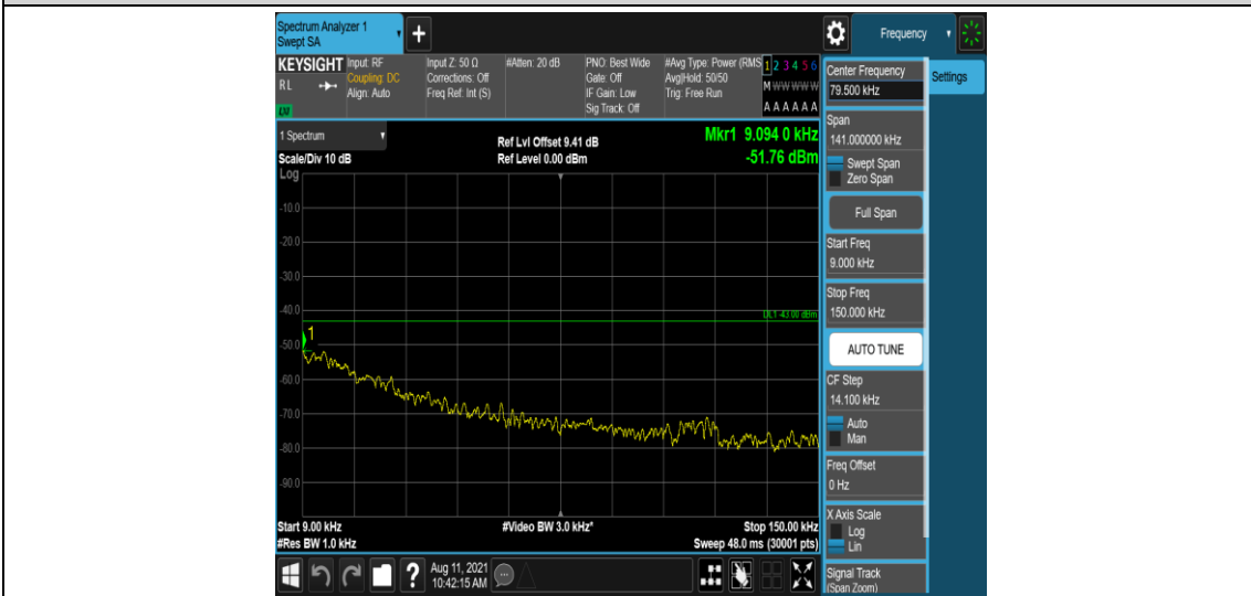
Band25-15MHz-QPSK-26365-1-0-Low-0.009-0.15--51.76-PASS
