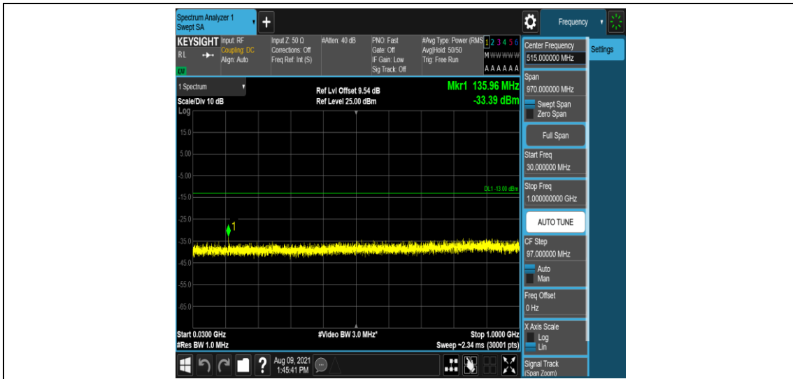
Band25-10MHz-16QAM-26640-1-0-High-30-1000--33.39-PASS
