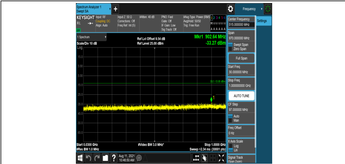
Band25-15MHz-16QAM-26615-1-0-High-30-1000--33.27-PASS
