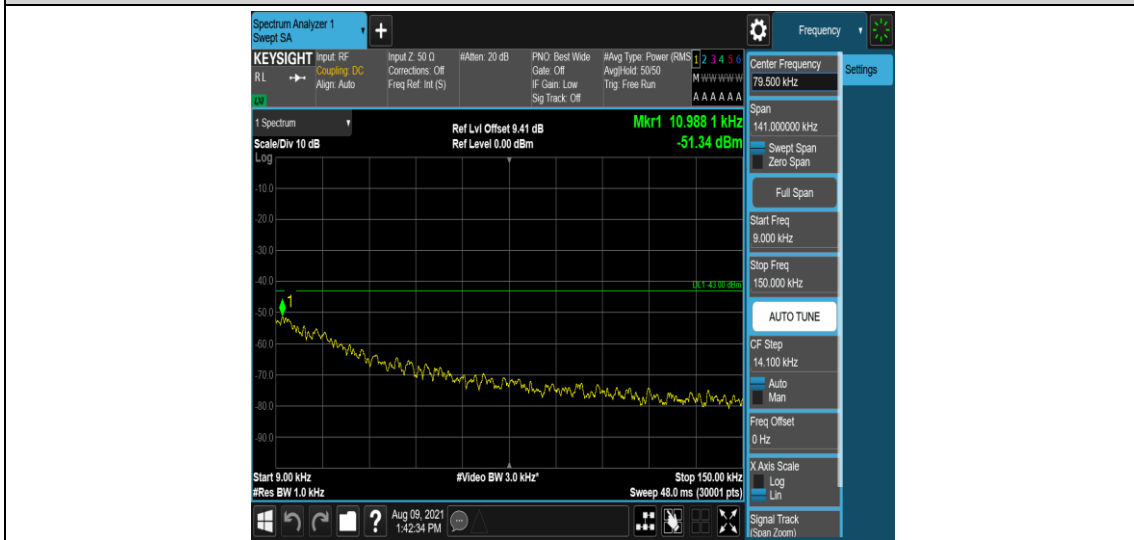
Band25-10MHz-16QAM-26365-1-0-Low-0.009-0.15--51.34-PASS
