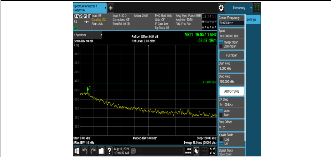
Band25-15MHz-16QAM-26615-1-0-High-0.009-0.15--52.07-PASS
