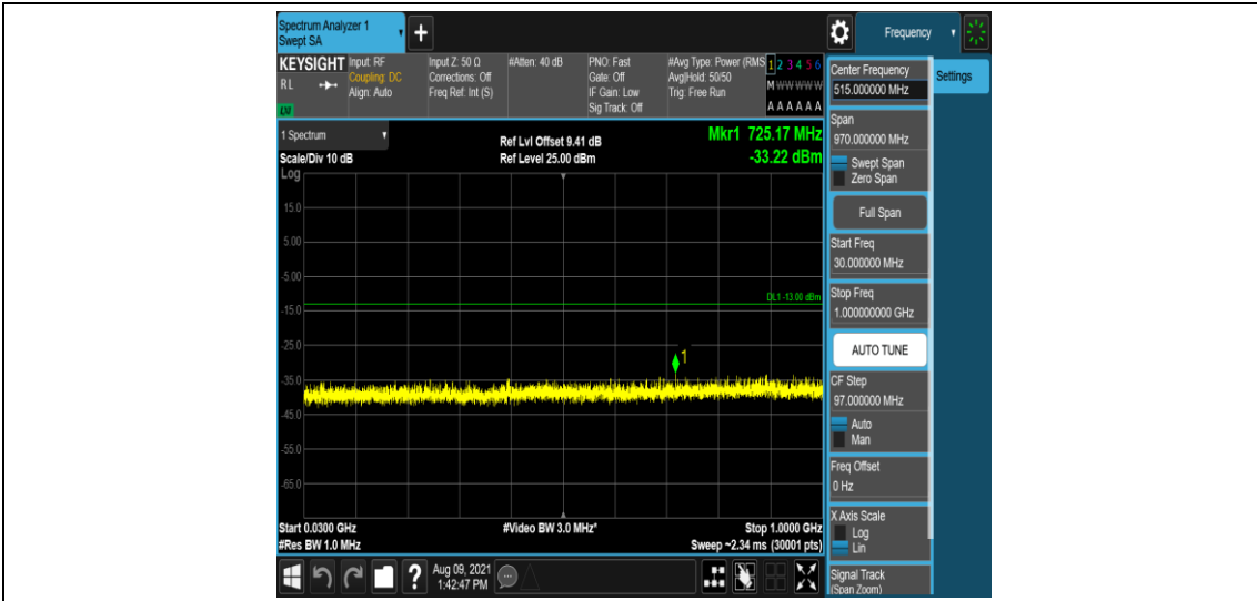
Band25-10MHz-16QAM-26365-1-0-Low-30-1000--33.23-PASS
