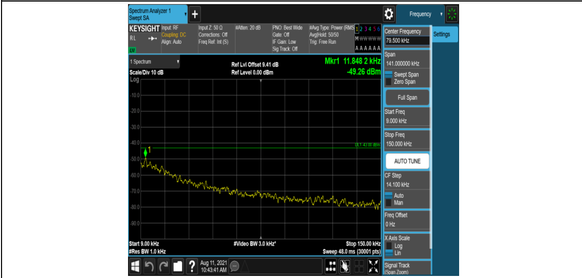
Band25-15MHz-16QAM-26365-1-0-Low-0.009-0.15--49.26-PASS
