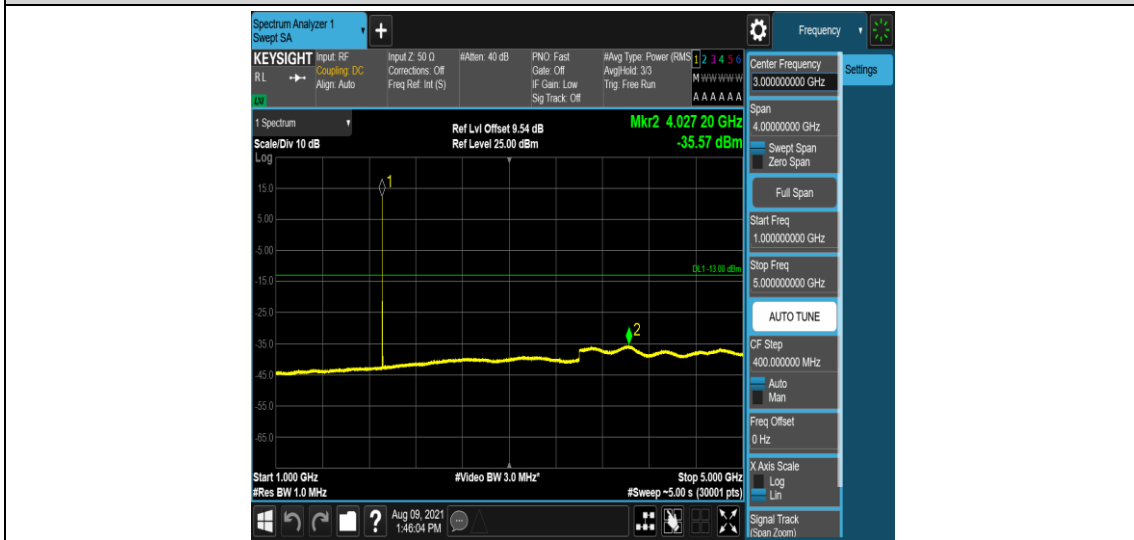
Band25-10MHz-16QAM-26640-1-0-High-1000-5000--35.57-PASS
