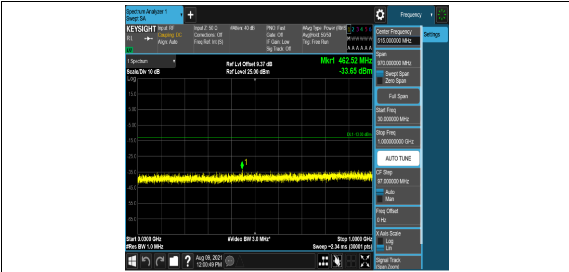
Band25-5MHz-QPSK-26065-1-0-Low-30-1000--33.65-PASS
