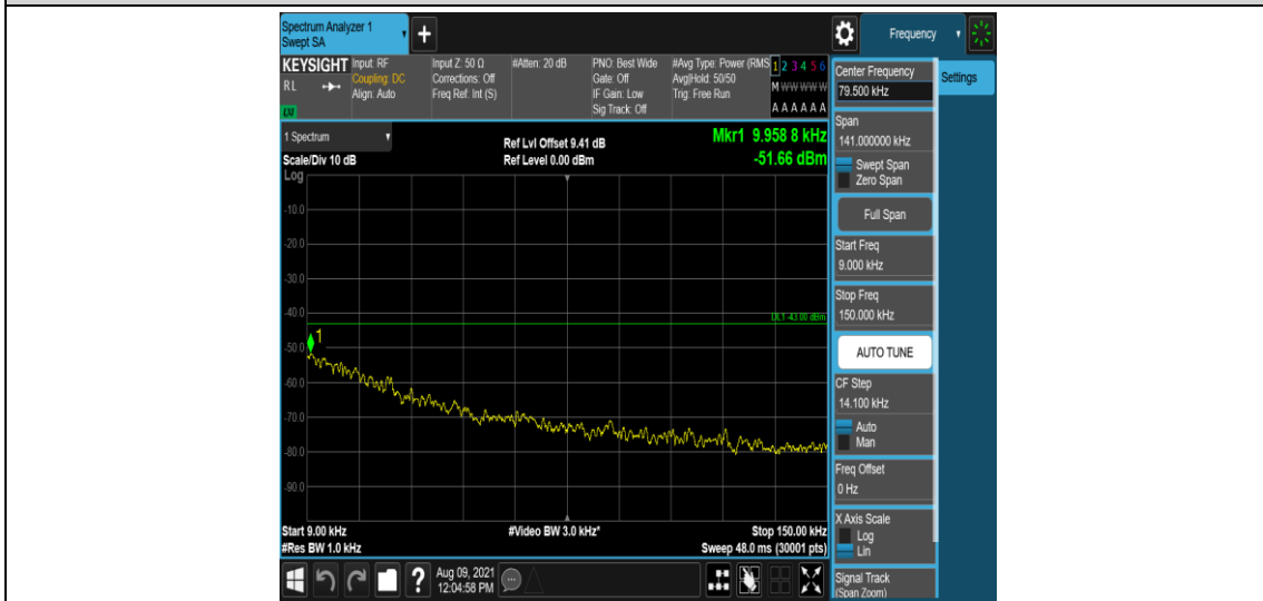
Band25-5MHz-16QAM-26365-1-0-Low-0.009-0.15--51.66-PASS
