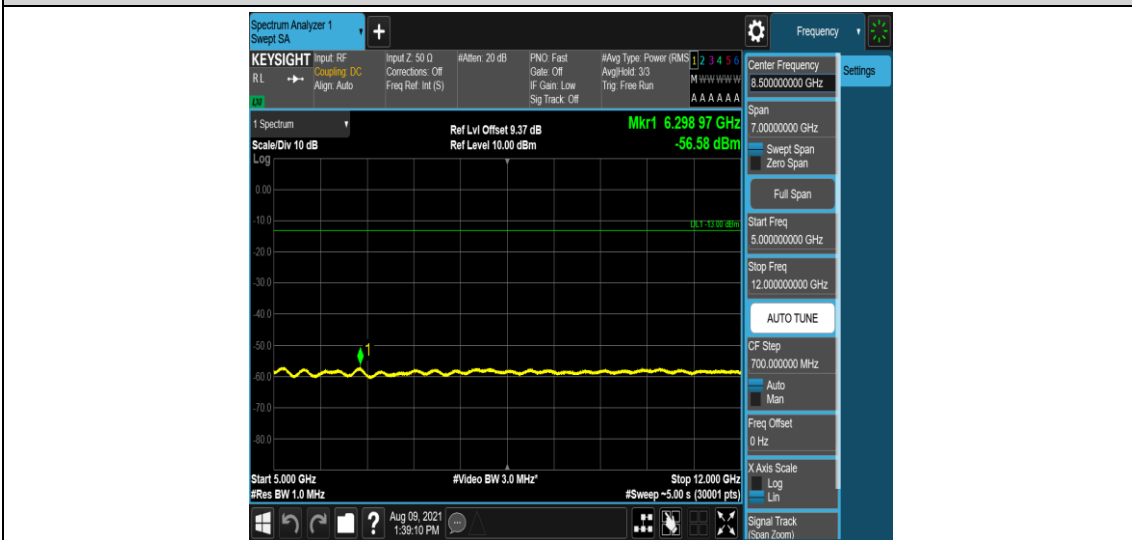
Band25-10MHz-QPSK-26090-1-0-Low-5000-12000--56.58-PASS
