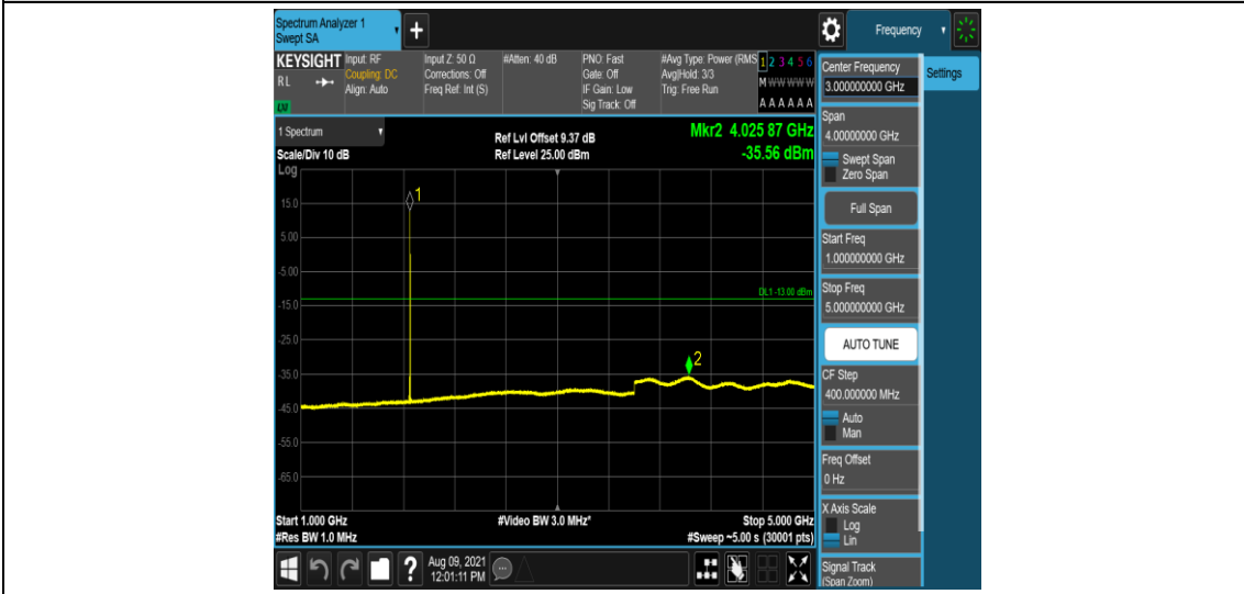
Band25-5MHz-QPSK-26065-1-0-Low-1000-5000--35.56-PASS
