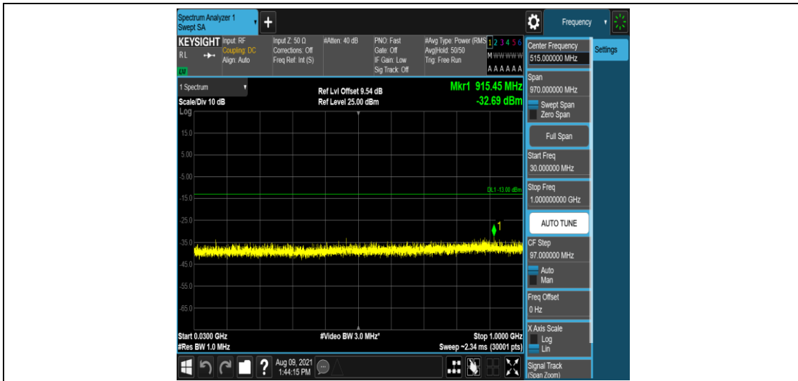
Band25-10MHz-QPSK-26640-1-0-High-30-1000--32.69-PASS
