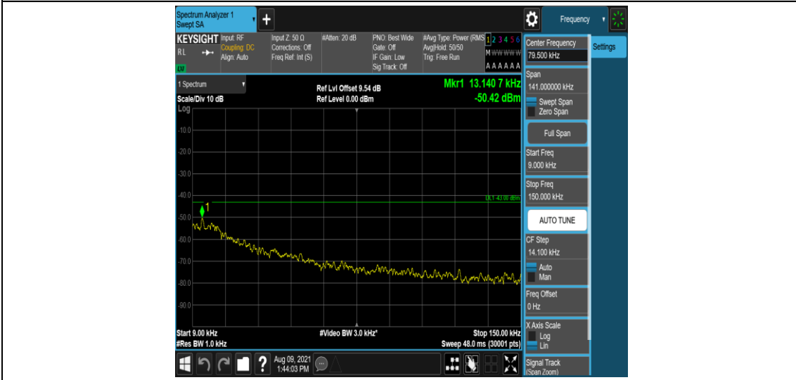
Band25-10MHz-QPSK-26640-1-0-High-0.009-0.15--50.42-PASS
