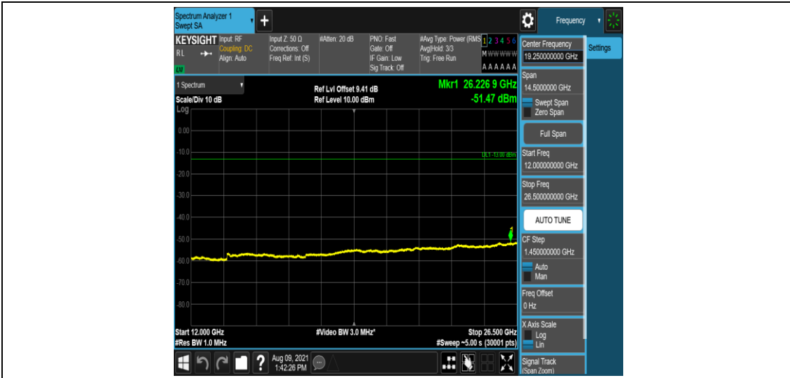
Band25-10MHz-QPSK-26365-1-0-Low-12000-26500--51.47-PASS
