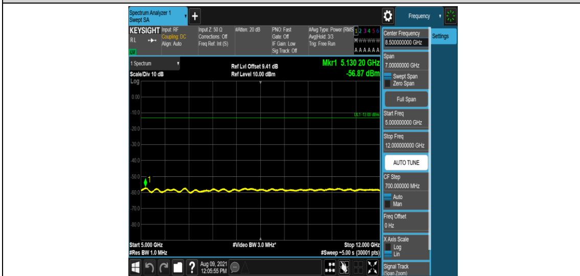
Band25-5MHz-16QAM-26365-1-0-Low-5000-12000--56.87-PASS
