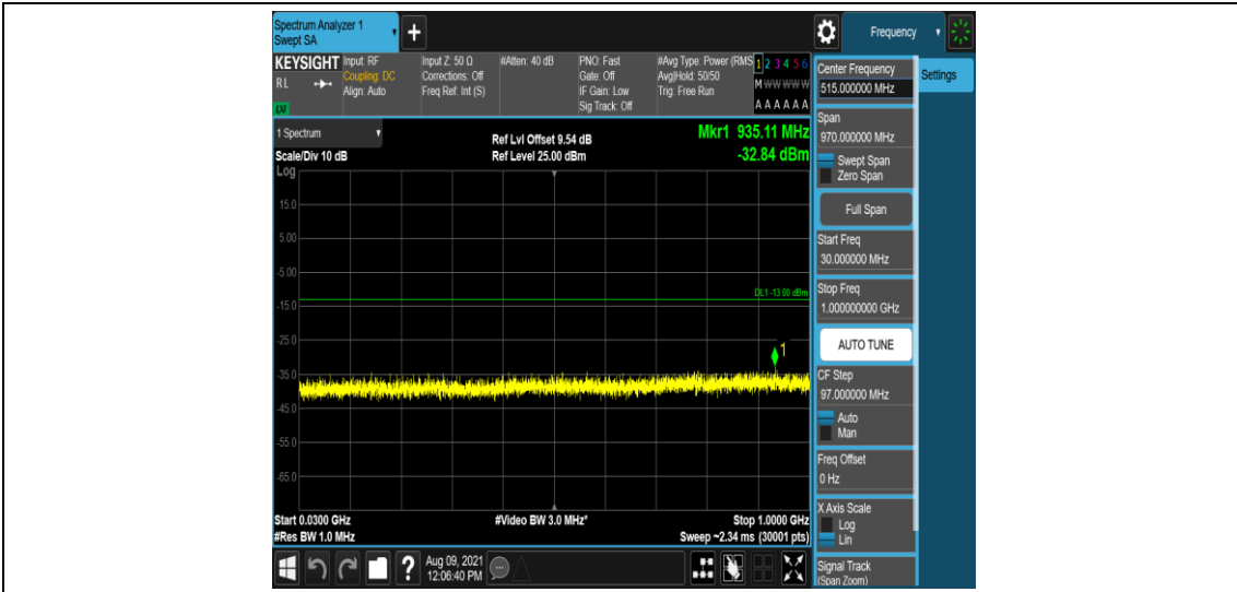
Band25-5MHz-QPSK-26665-1-0-High-30-1000--32.84-PASS
