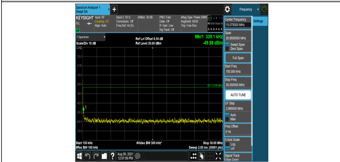
Band25-5MHz-16QAM-26665-1-0-High-0.15-30--49.88-PASS
