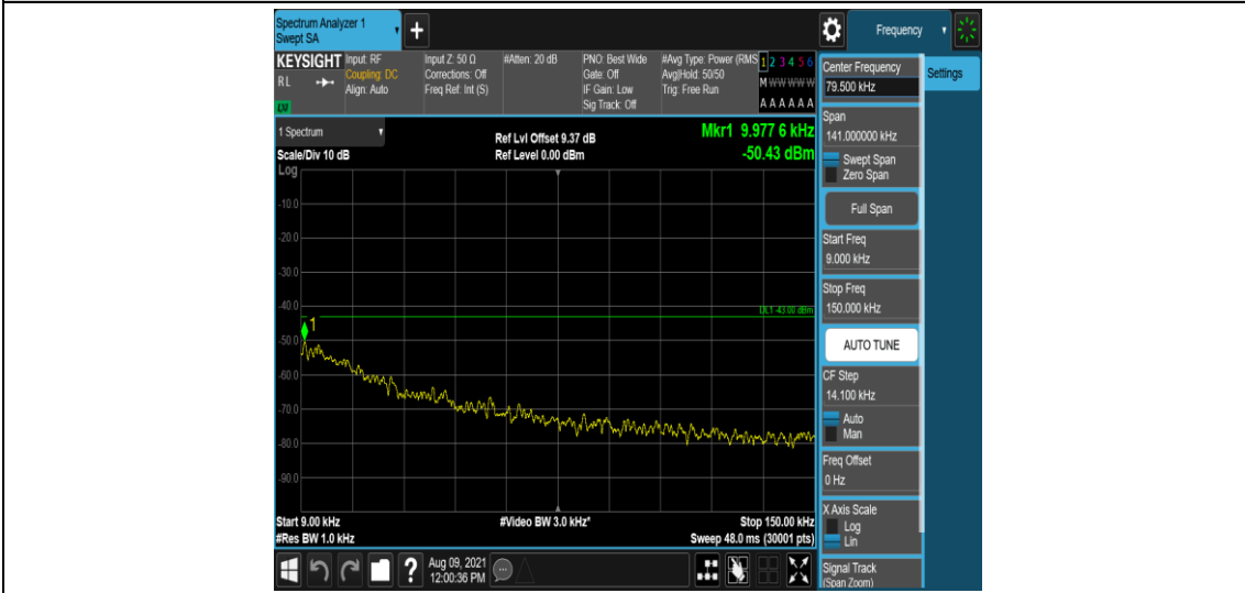
Band25-5MHz-QPSK-26065-1-0-Low-0.009-0.15--50.43-PASS
