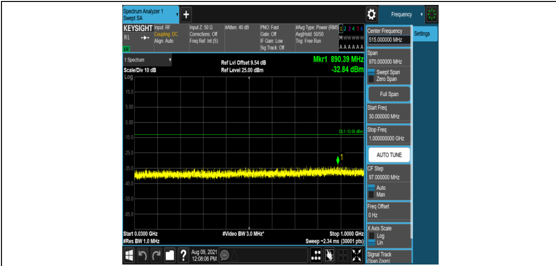
Band25-5MHz-16QAM-26665-1-0-High-30-1000--32.84-PASS
