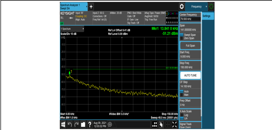
Band25-5MHz-QPSK-26365-1-0-Low-0.009-0.15--51.21-PASS
