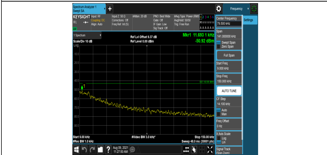
Band25-3MHz-16QAM-26055-1-0-Low-0.009-0.15--50.93-PASS
