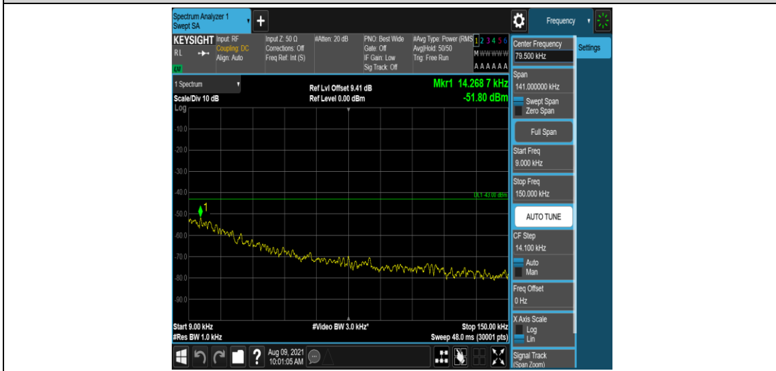
Band25-1.4MHz-16QAM-26365-1-0-Low-0.009-0.15--51.8-PASS
