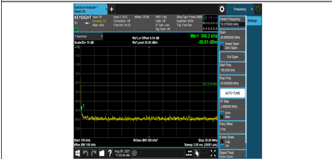
Band25-3MHz-16QAM-26675-1-0-High-0.15-30--50.61-PASS
