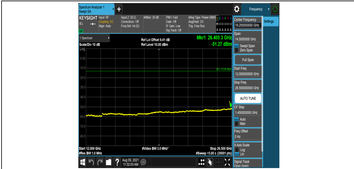
Band25-3MHz-16QAM-26365-1-0-Low-12000-26500--51.27-PASS
