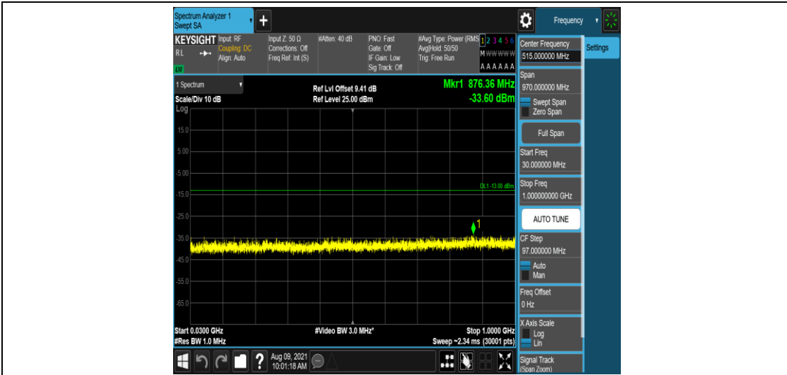
Band25-1.4MHz-16QAM-26365-1-0-Low-30-1000--33.6-PASS
