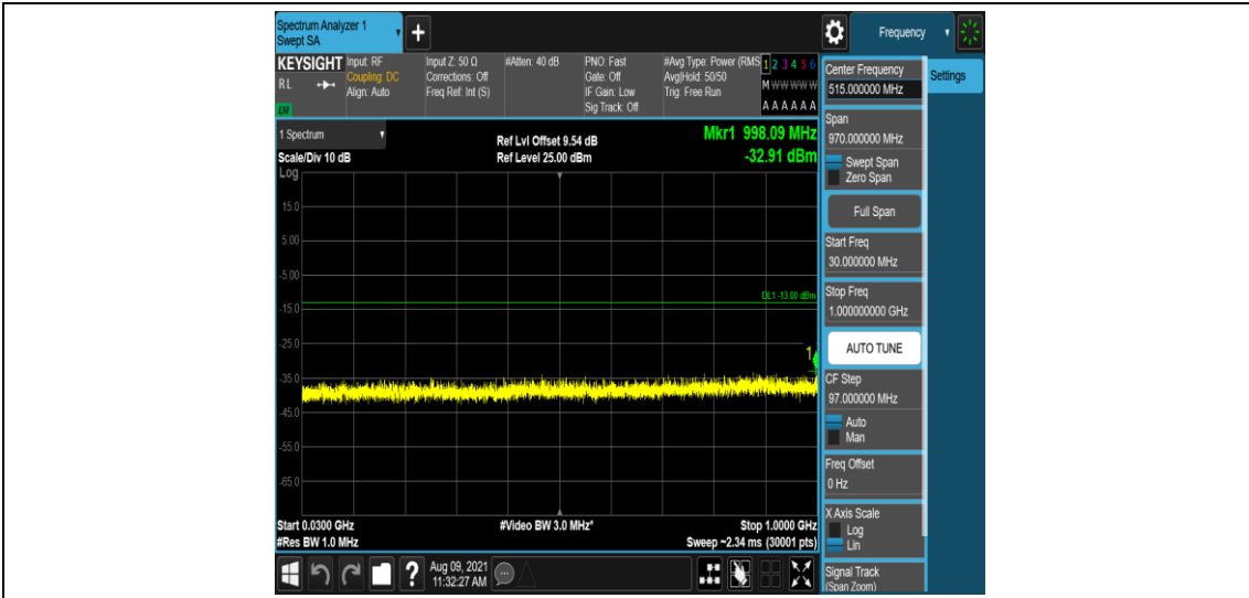
Band25-3MHz-QPSK-26675-1-0-High-30-1000--32.91-PASS
