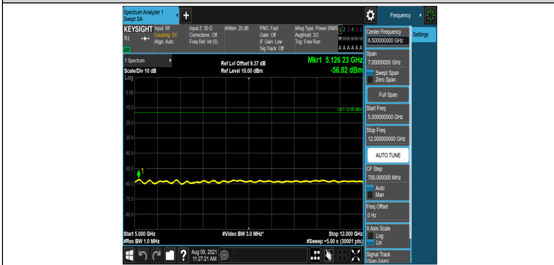
Band25-3MHz-QPSK-26055-1-0-Low-5000-12000--56.82-PASS
