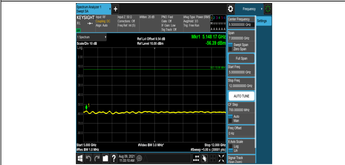
Band25-3MHz-QPSK-26675-1-0-High-5000-12000--56.39-PASS
