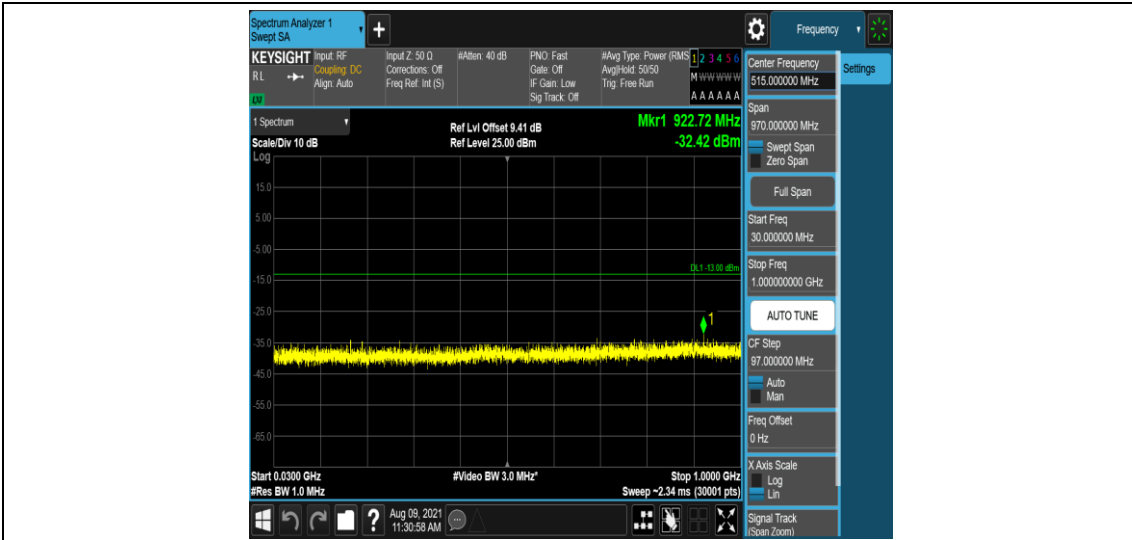
Band25-3MHz-16QAM-26365-1-0-Low-30-1000--32.42-PASS
