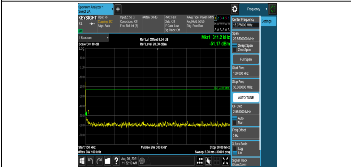
Band25-3MHz-QPSK-26675-1-0-High-0.15-30--51.17-PASS
