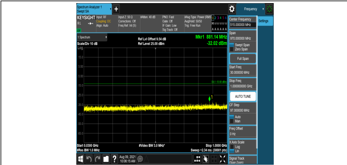
Band25-1.4MHz-16QAM-26683-1-0-High-30-1000--32.02-PASS
