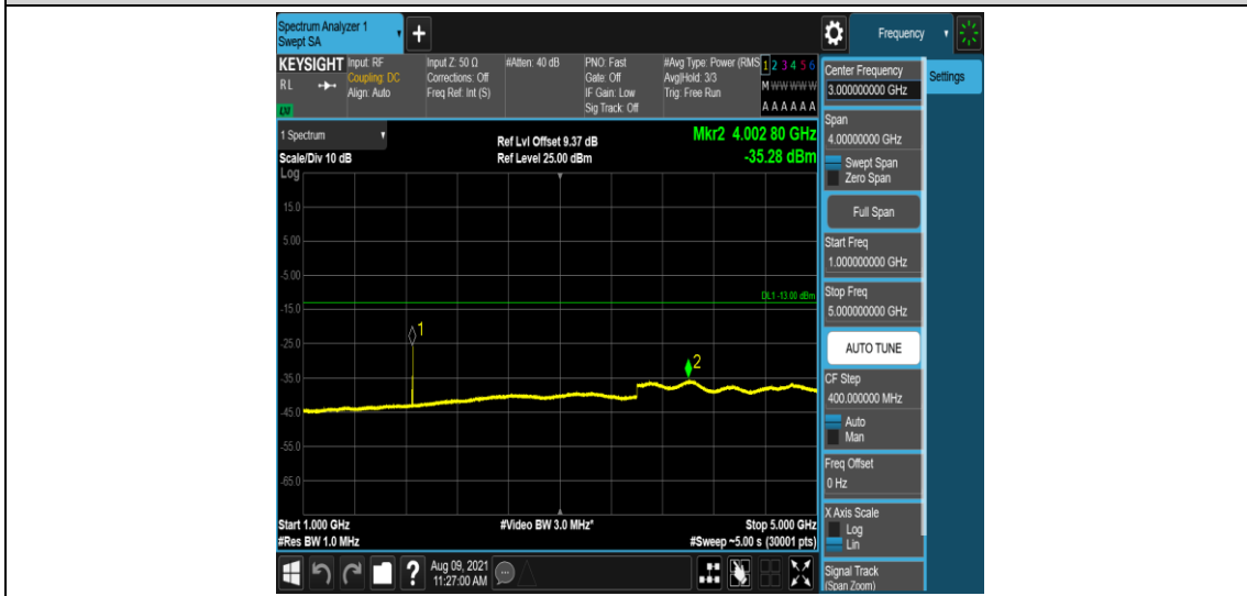
Band25-3MHz-QPSK-26055-1-0-Low-1000-5000--35.28-PASS
