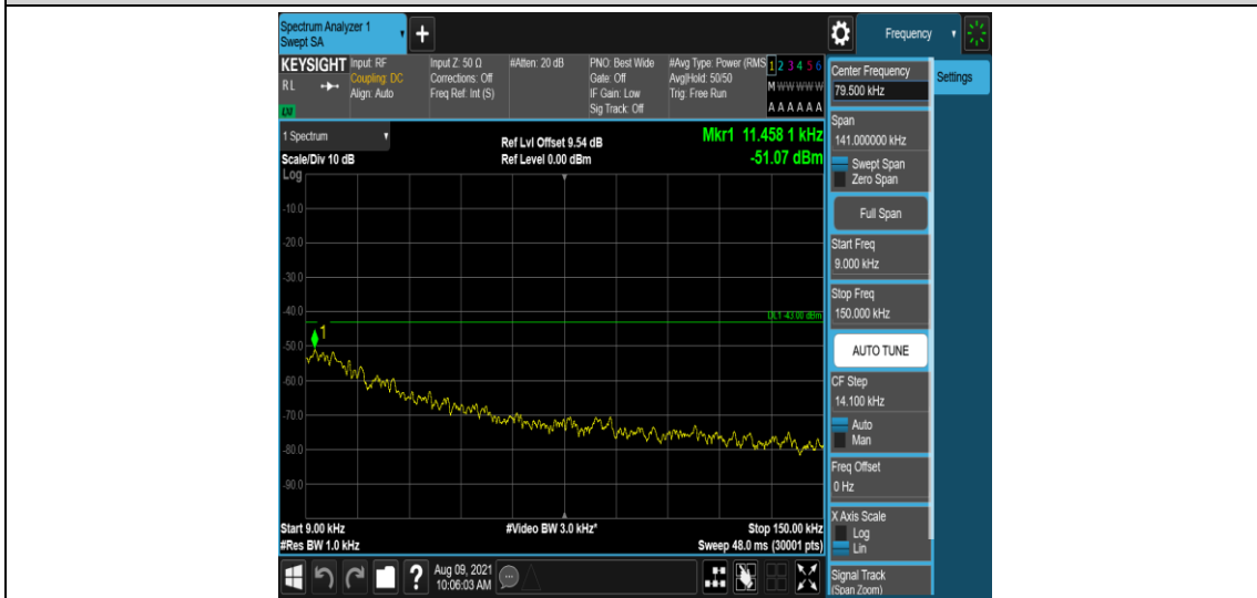
Band25-1.4MHz-16QAM-26683-1-0-High-0.009-0.15--51.07-PASS
