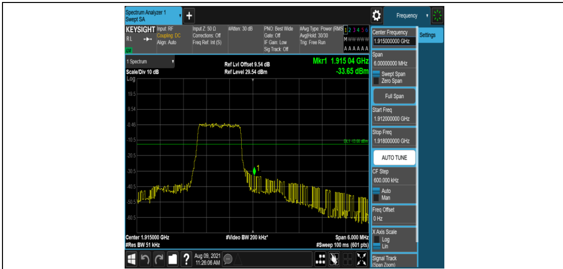
Band25-3MHz-QPSK-26675-6-0-High--33.65-PASS
