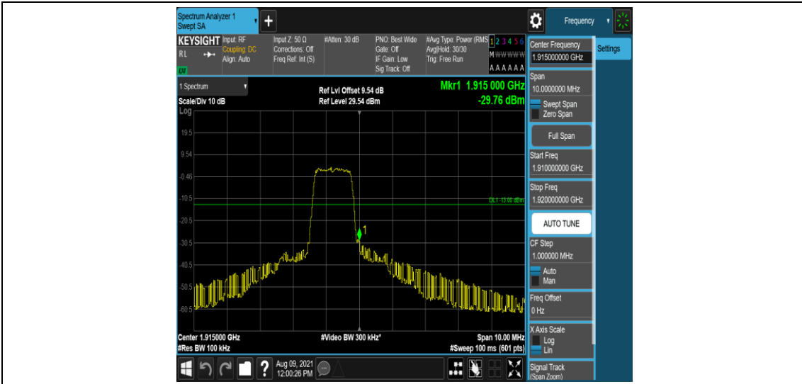
Band25-5MHz-16QAM-26665-6-0-High--29.76-PASS
