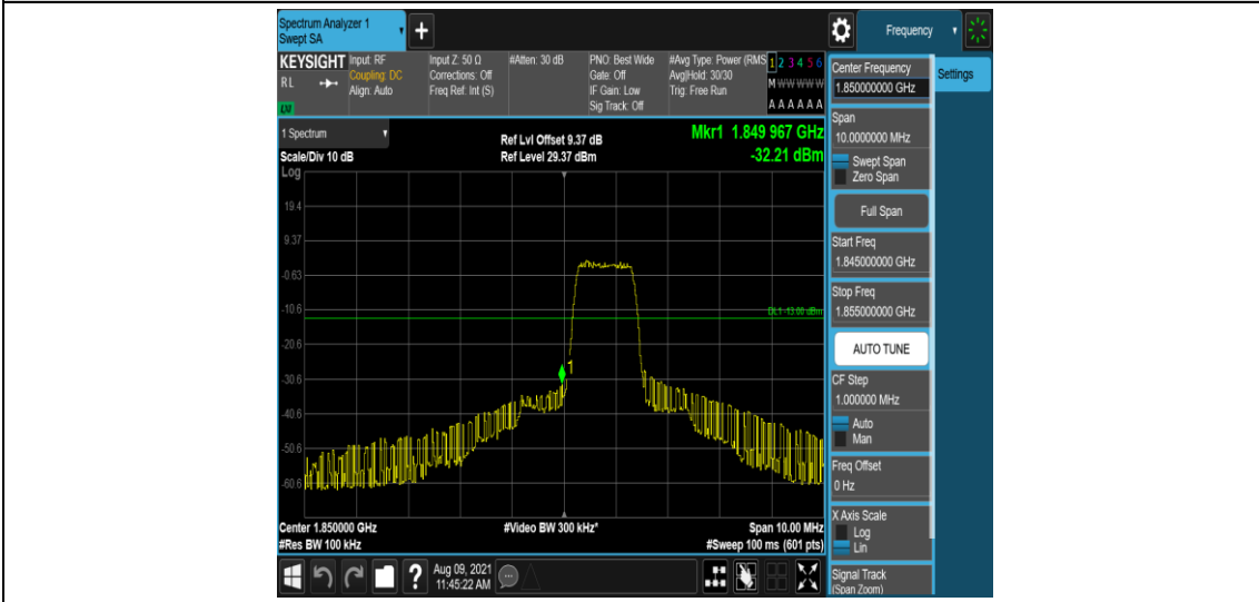
Band25-5MHz-16QAM-26065-6-0-Low--32.21-PASS
