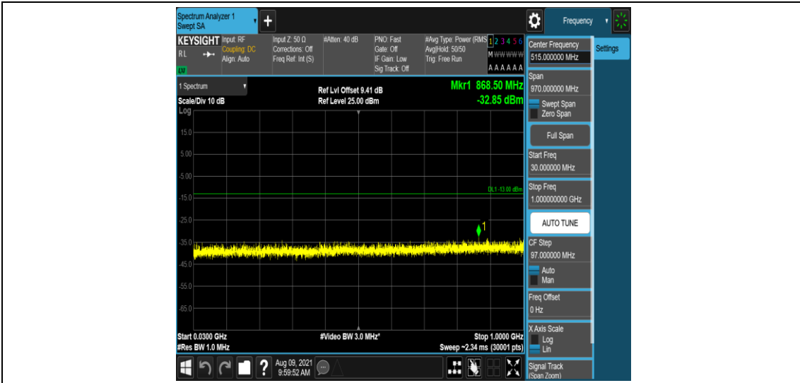
Band25-1.4MHz-QPSK-26365-1-0-Low-30-1000--32.85-PASS
