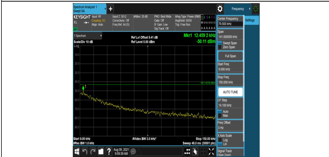
Band25-1.4MHz-QPSK-26365-1-0-Low-0.009-0.15--50.11-PASS
