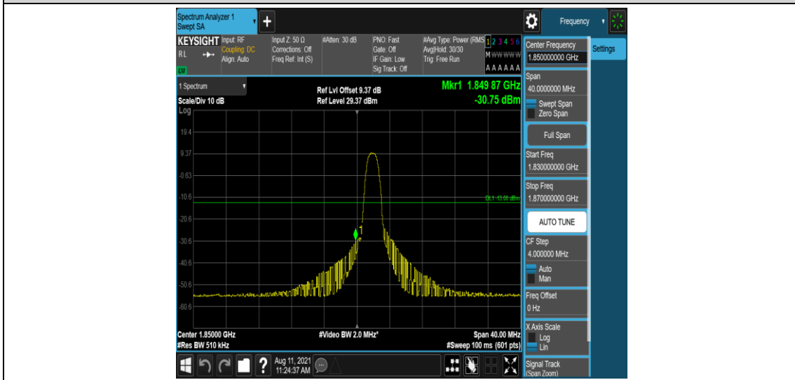
Band25-20MHz-16QAM-26140-6-0-Low--30.75-PASS
