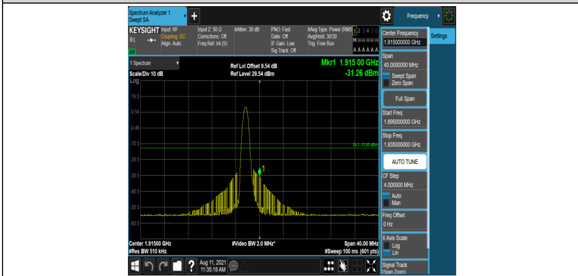
Band25-20MHz-16QAM-26590-1-0-High--31.26-PASS
