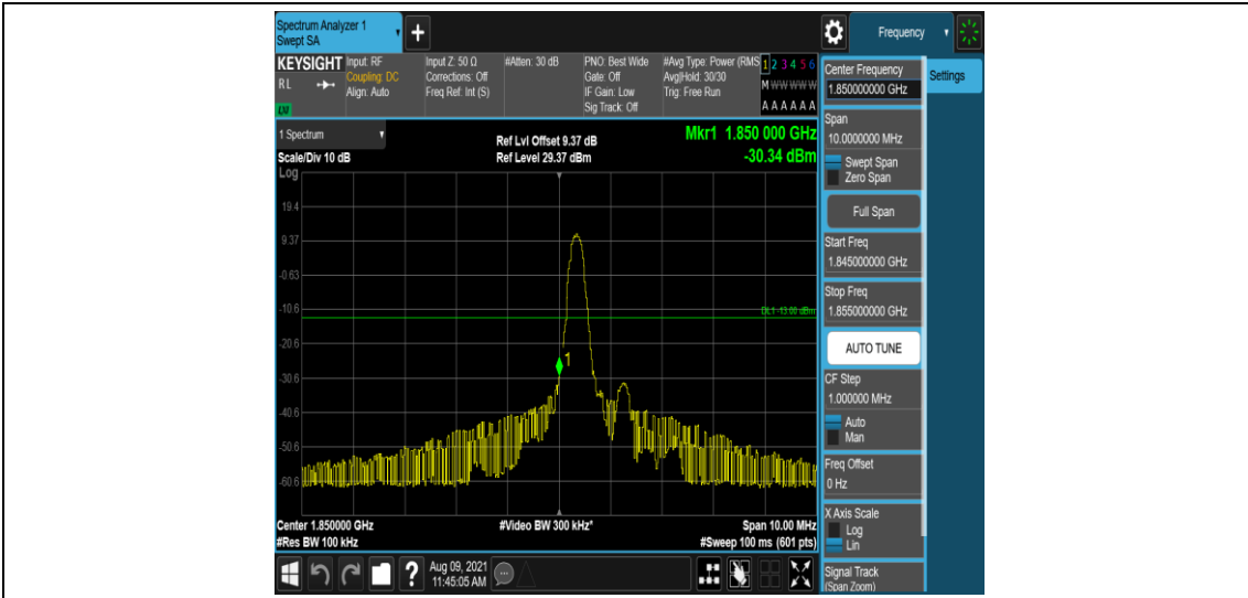
Band25-5MHz-16QAM-26065-1-0-Low--30.34-PASS
