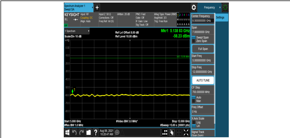
Band12-10MHz-QPSK-23095-1-0-Low-5000-12000--58.23-PASS
