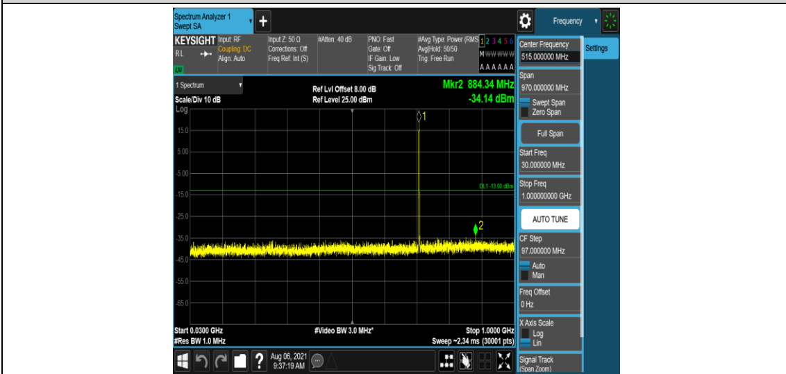
Band12-5MHz-QPSK-23155-1-0-High-30-1000--34.14-PASS
