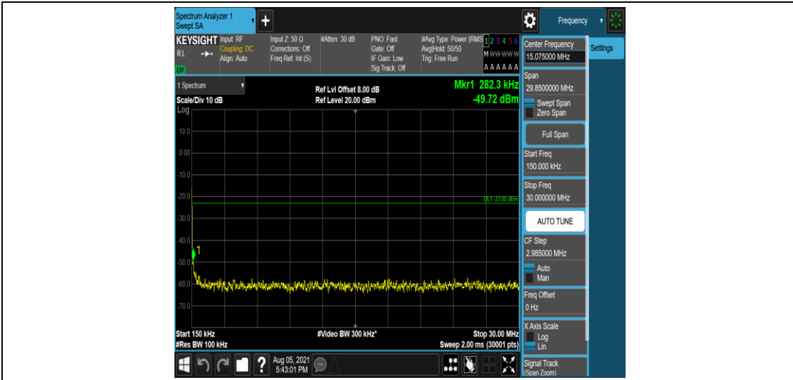
Band12-3MHz-16QAM-23165-1-0-High-0.15-30--49.72-PASS
