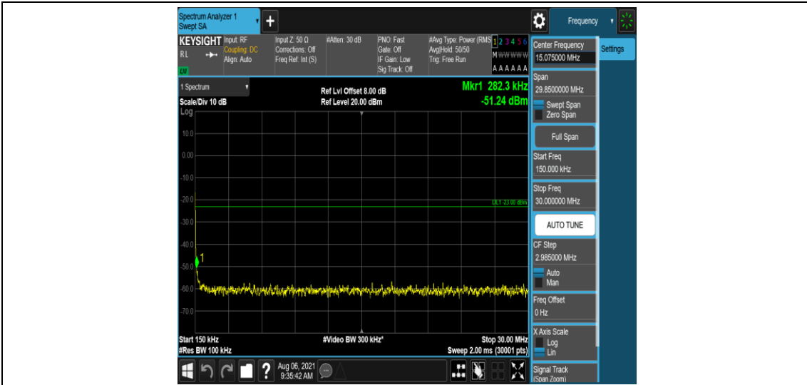
Band12-5MHz-16QAM-23095-1-0-Low-0.15-30--51.24-PASS
