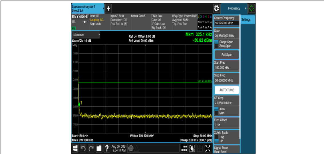
Band12-5MHz-QPSK-23095-1-0-Low-0.15-30--50.82-PASS
