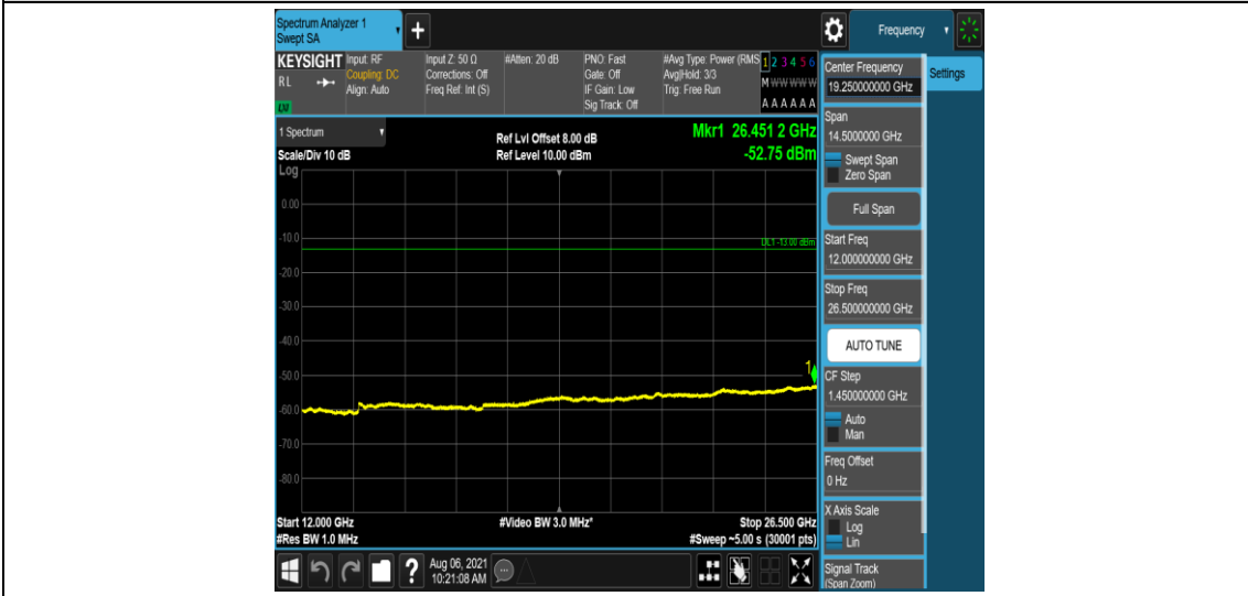
Band12-10MHz-QPSK-23095-1-0-Low-12000-26500--52.75-PASS
