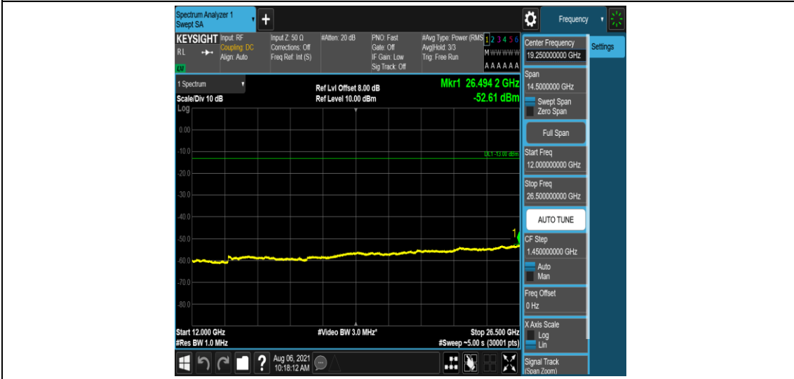
Band12-10MHz-QPSK-23060-1-0-Low-12000-26500--52.61-PASS
