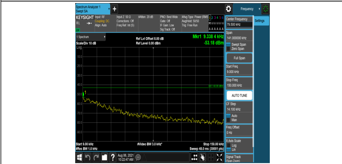
Band12-10MHz-QPSK-23130-1-0-High-0.009-0.15--53.18-PASS
