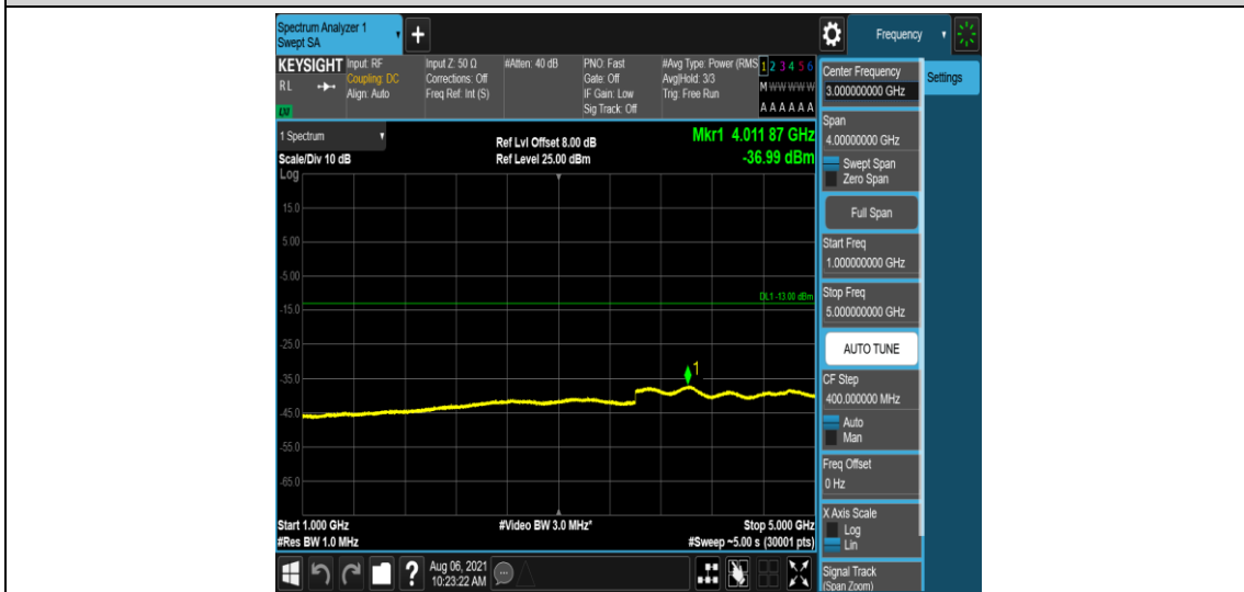
Band12-10MHz-QPSK-23130-1-0-High-1000-5000--36.99-PASS
