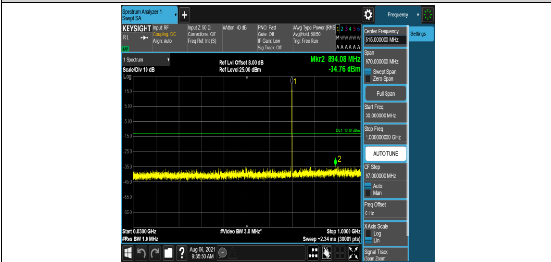
Band12-5MHz-16QAM-23095-1-0-Low-30-1000--34.77-PASS
