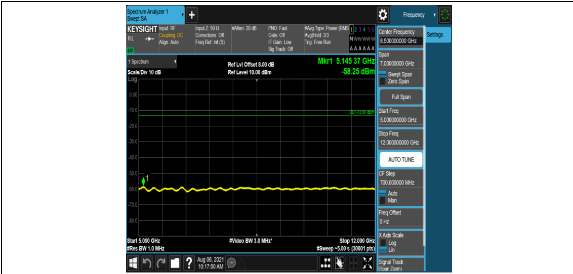
Band12-10MHz-QPSK-23060-1-0-Low-5000-12000--58.25-PASS
