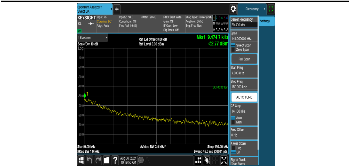
Band12-10MHz-QPSK-23095-1-0-Low-0.009-0.15--52.77-PASS
