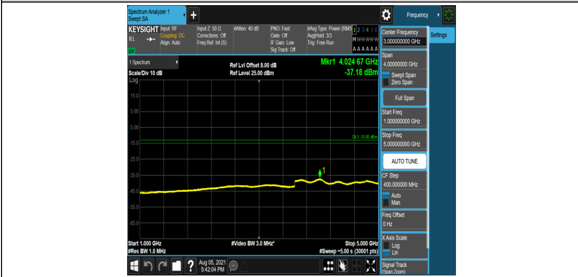
Band12-3MHz-QPSK-23165-1-0-High-1000-5000--37.18-PASS
