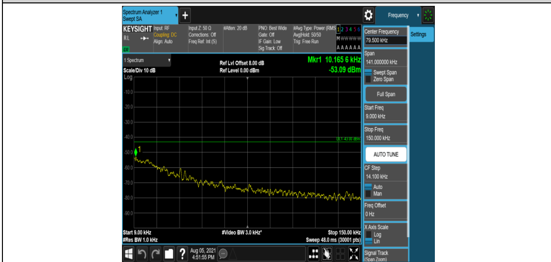
Band12-1.4MHz-16QAM-23095-1-0-Low-0.009-0.15--53.09-PASS
