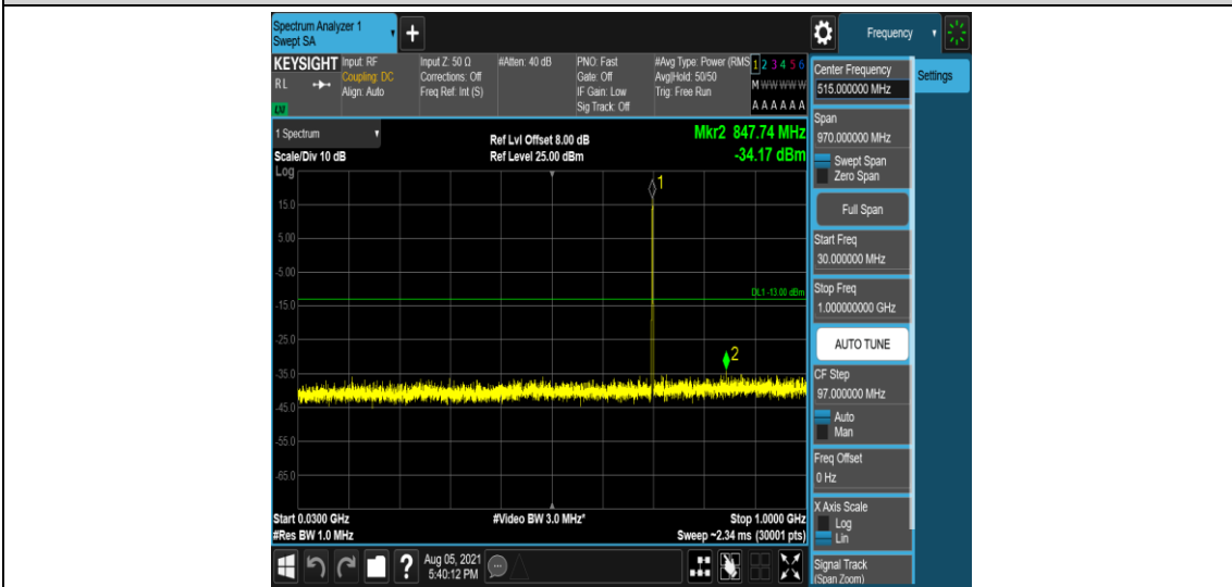
Band12-3MHz-16QAM-23095-1-0-Low-30-1000--34.17-PASS
