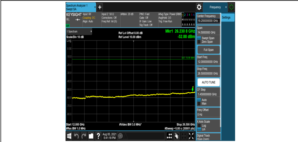
Band12-3MHz-16QAM-23095-1-0-Low-12000-26500--52.88-PASS
