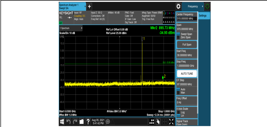
Band12-3MHz-QPSK-23165-1-0-High-30-1000--34.95-PASS
