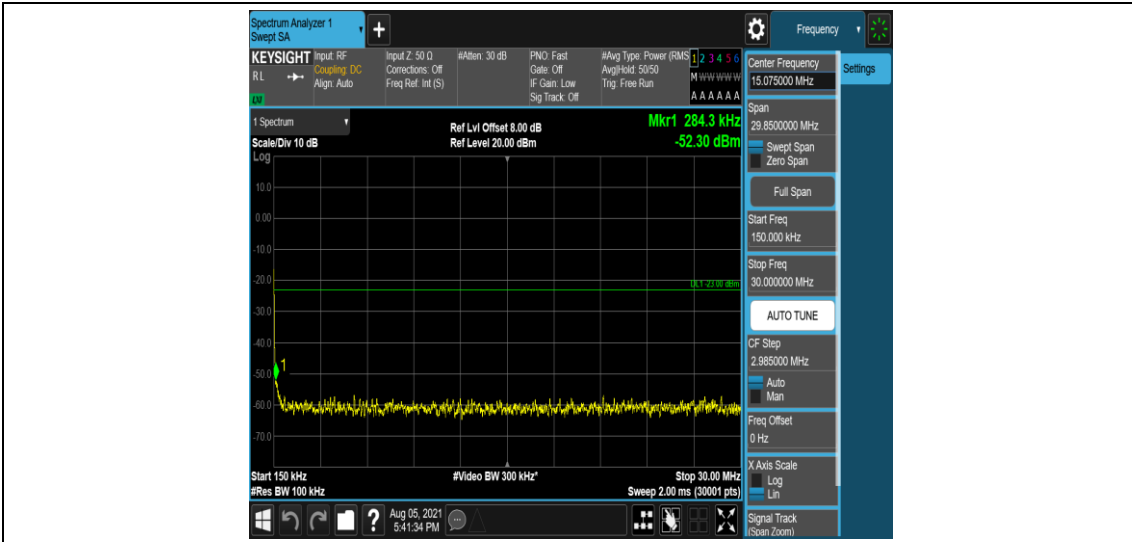
Band12-3MHz-QPSK-23165-1-0-High-0.15-30--52.3-PASS
