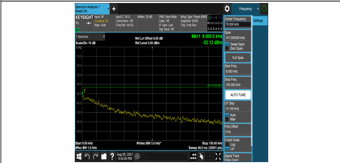
Band12-3MHz-16QAM-23165-1-0-High-0.009-0.15--52.12-PASS
