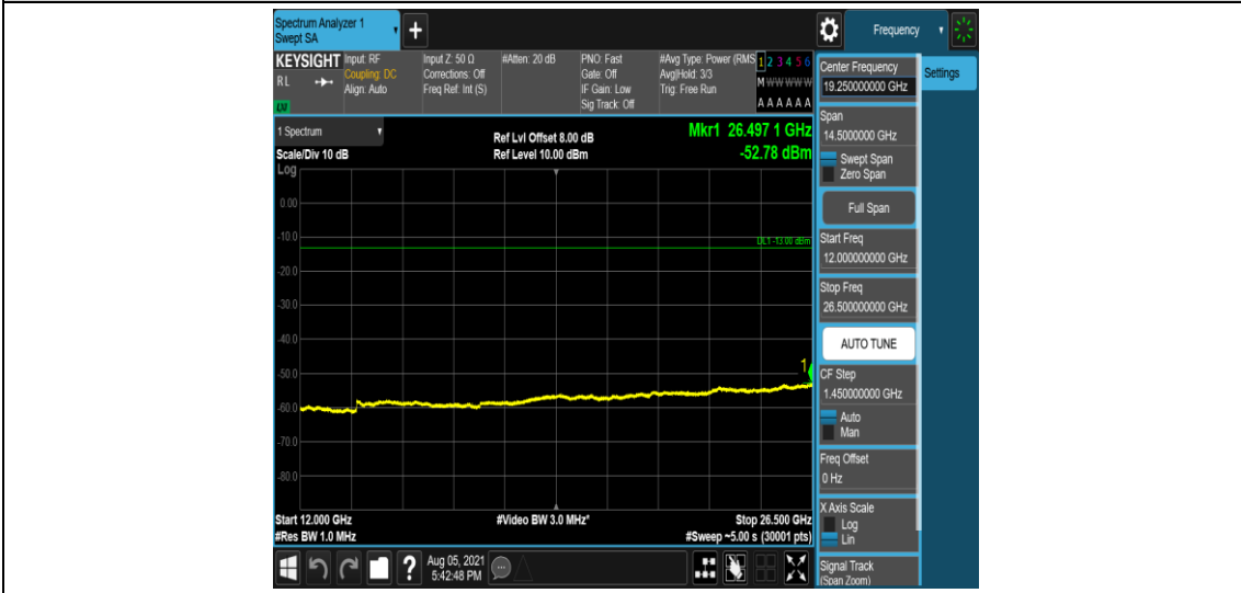
Band12-3MHz-QPSK-23165-1-0-High-12000-26500--52.78-PASS
