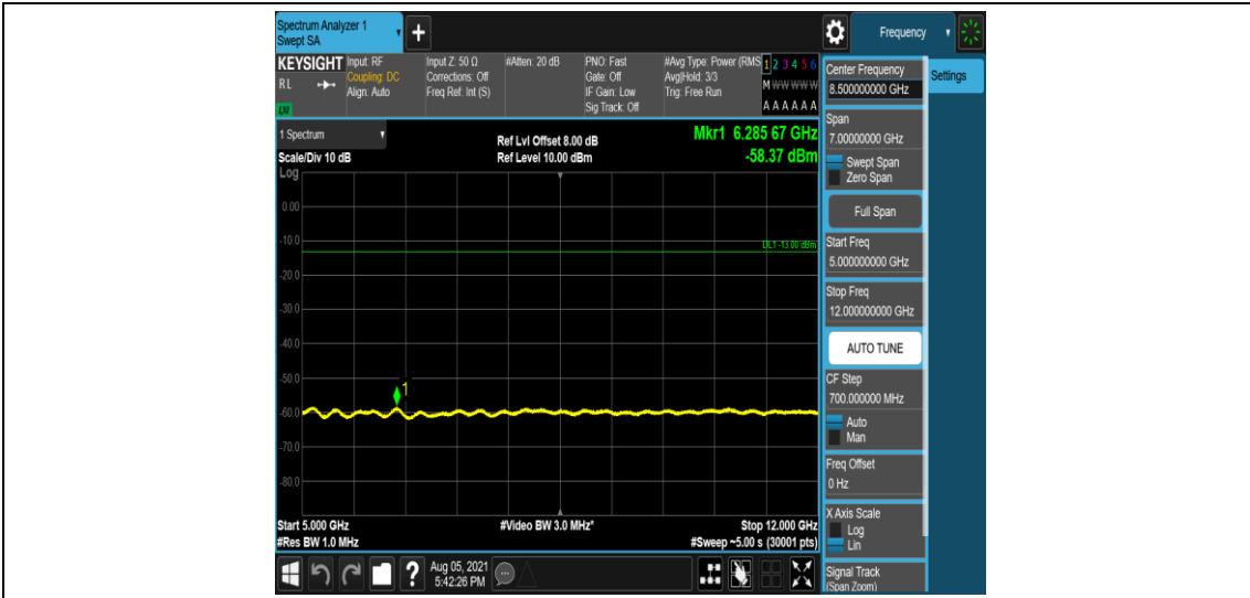
Band12-3MHz-QPSK-23165-1-0-High-5000-12000--58.37-PASS
