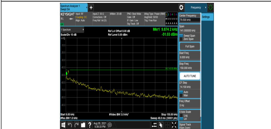
Band12-3MHz-QPSK-23095-1-0-Low-0.009-0.15--51.03-PASS
