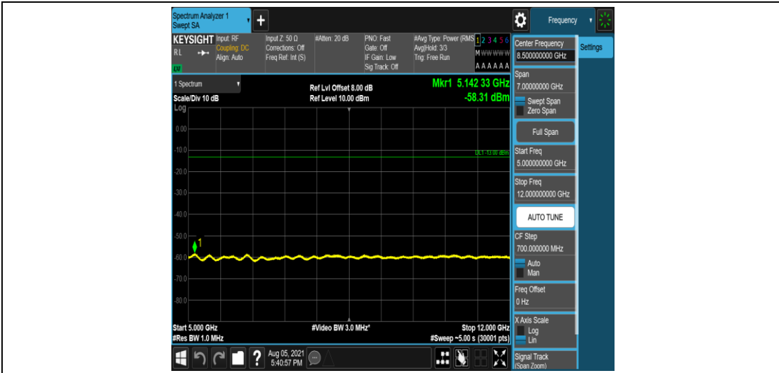
Band12-3MHz-16QAM-23095-1-0-Low-5000-12000--58.31-PASS
