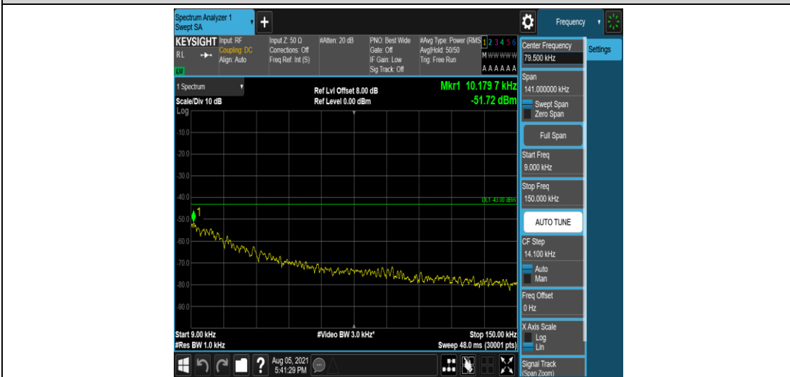
Band12-3MHz-QPSK-23165-1-0-High-0.009-0.15--51.73-PASS
