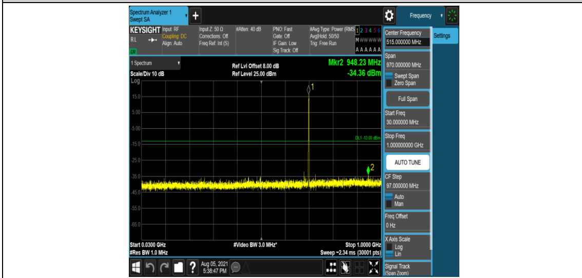
Band12-3MHz-QPSK-23095-1-0-Low-30-1000--34.36-PASS
