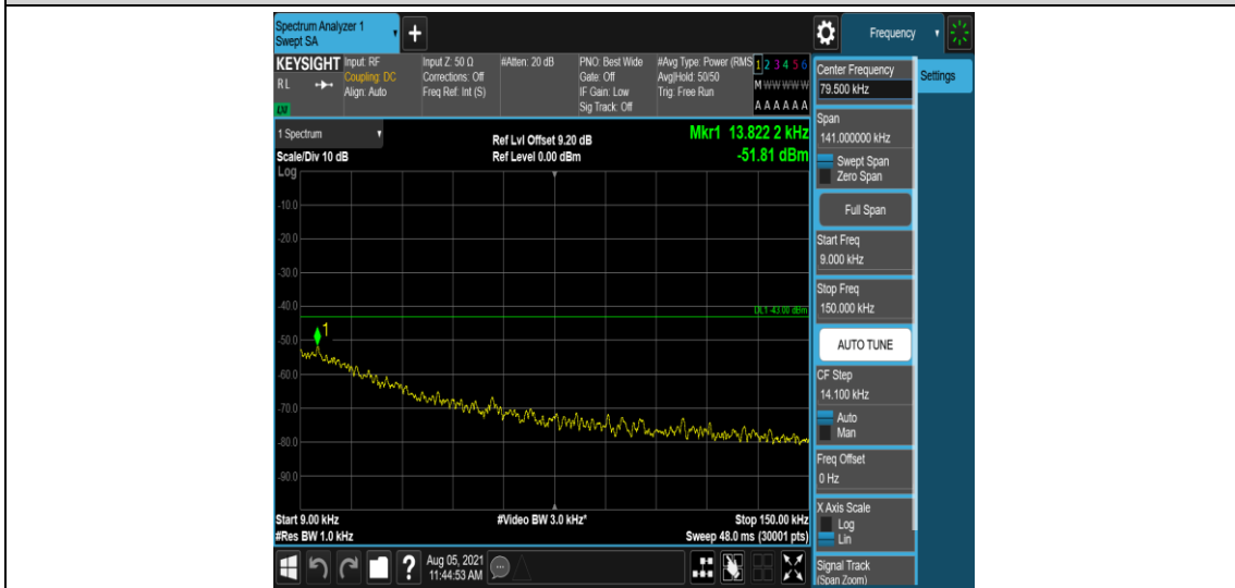
Band4-15MHz-QPSK-20175-1-0-Low-0.009-0.15--51.81-PASS
