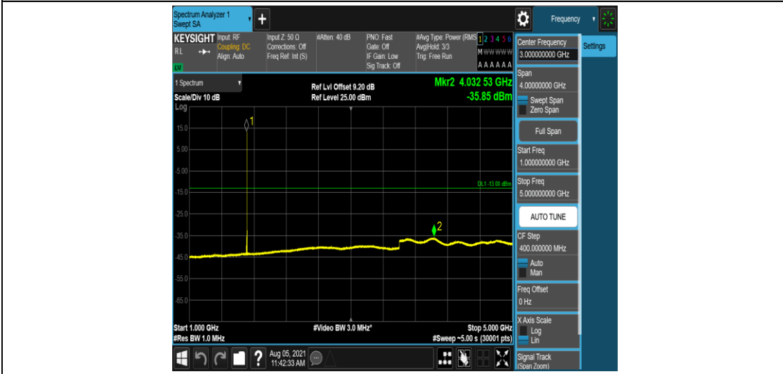
Band4-15MHz-QPSK-2025-1-0-Low-1000-5000--35.85-PASS
