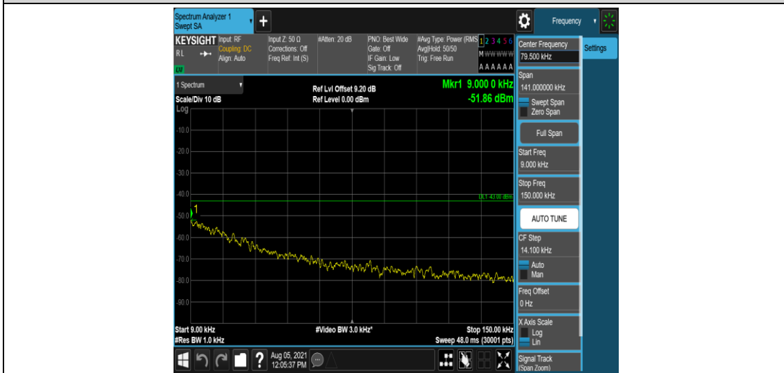
Band4-20MHz-QPSK-20175-1-0-Low-0.009-0.15--51.87-PASS
