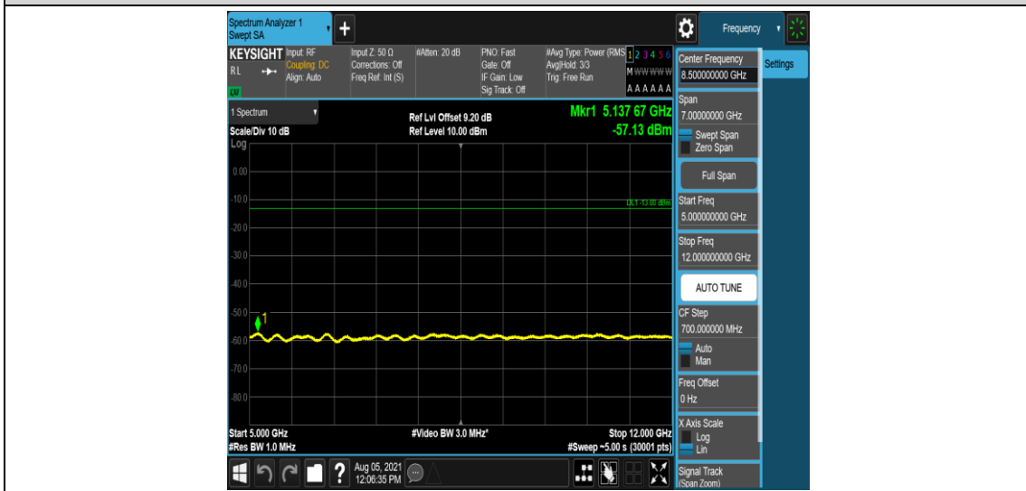
Band4-20MHz-QPSK-20175-1-0-Low-5000-12000--57.13-PASS
