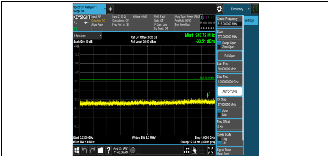
Band4-15MHz-QPSK-20175-1-0-Low-30-1000--33.51-PASS
