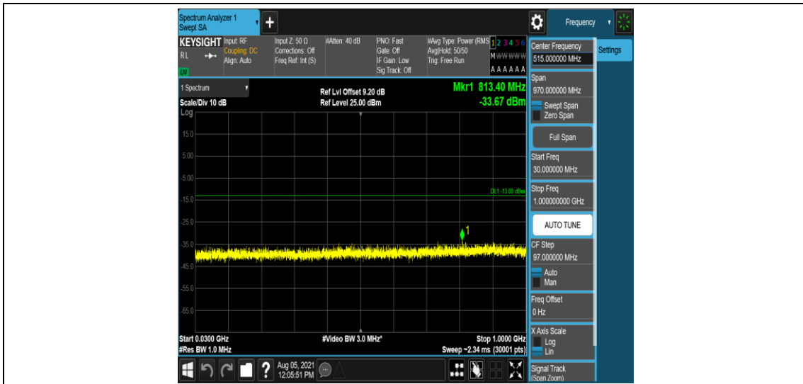
Band4-20MHz-QPSK-20175-1-0-Low-30-1000--33.67-PASS
