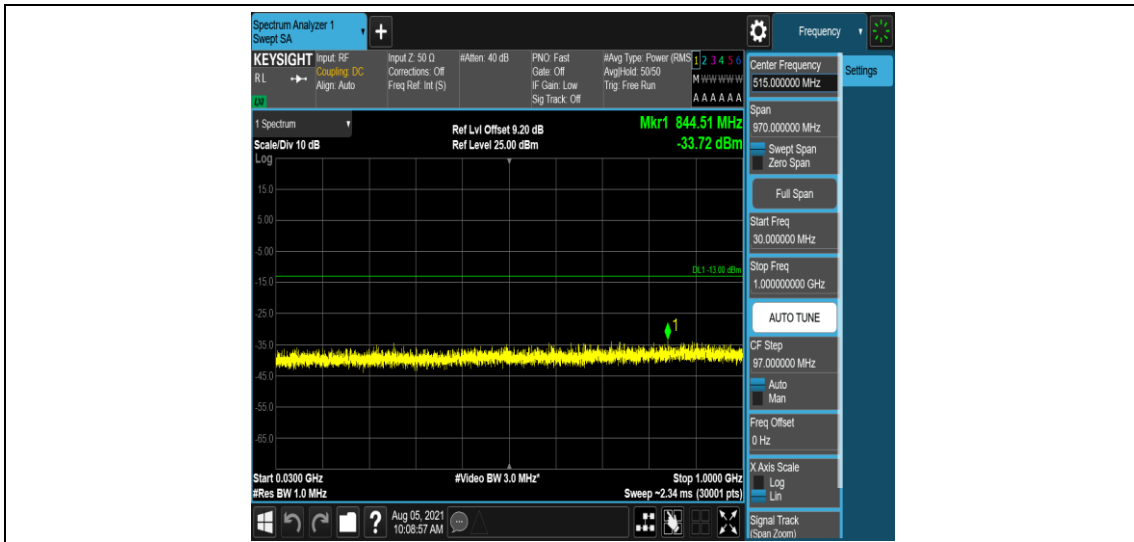
Band4-10MHz-16QAM-20175-1-0-Low-30-1000--33.72-PASS
