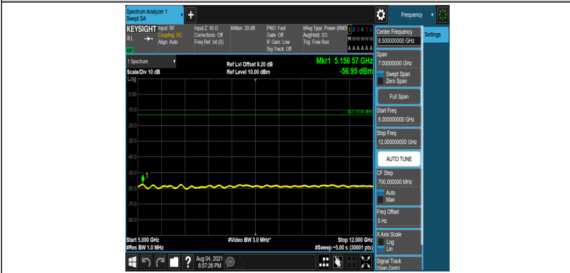
Band4-5MHz-QPSK-20175-1-0-Low-5000-12000--56.95-PASS
