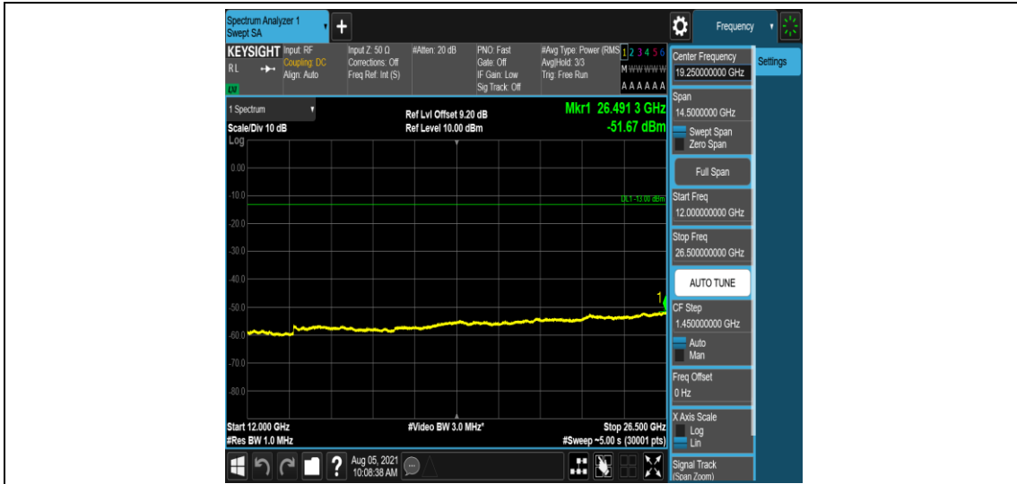
Band4-10MHz-QPSK-20175-1-0-Low-12000-26500--51.67-PASS
