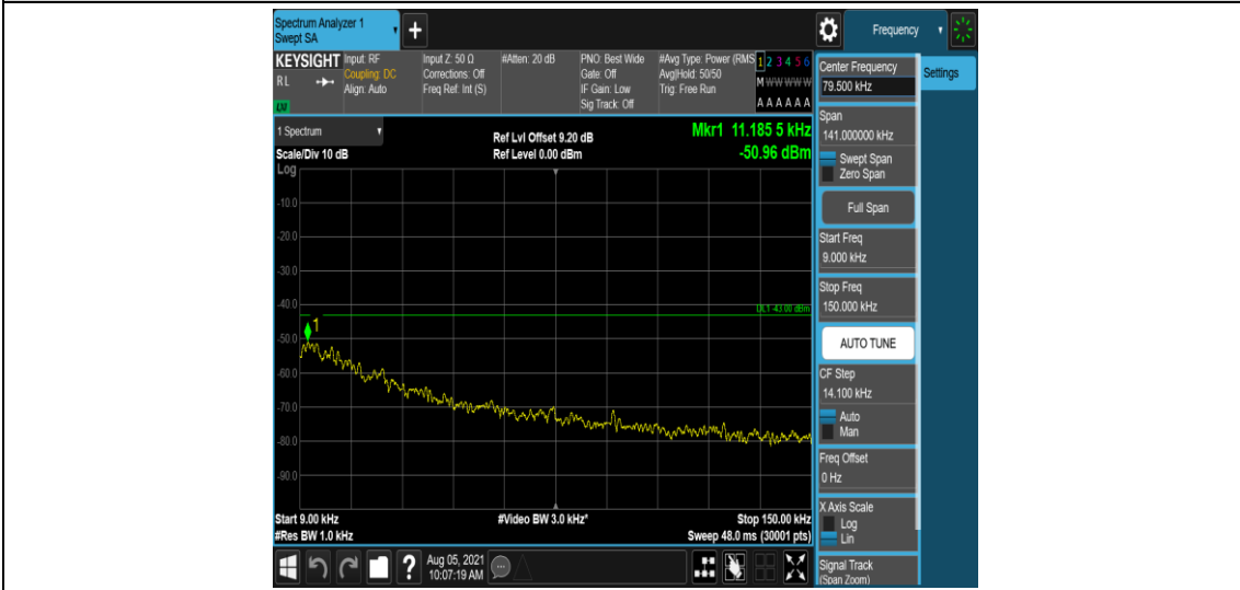
Band4-10MHz-QPSK-20175-1-0-Low-0.009-0.15--50.96-PASS
