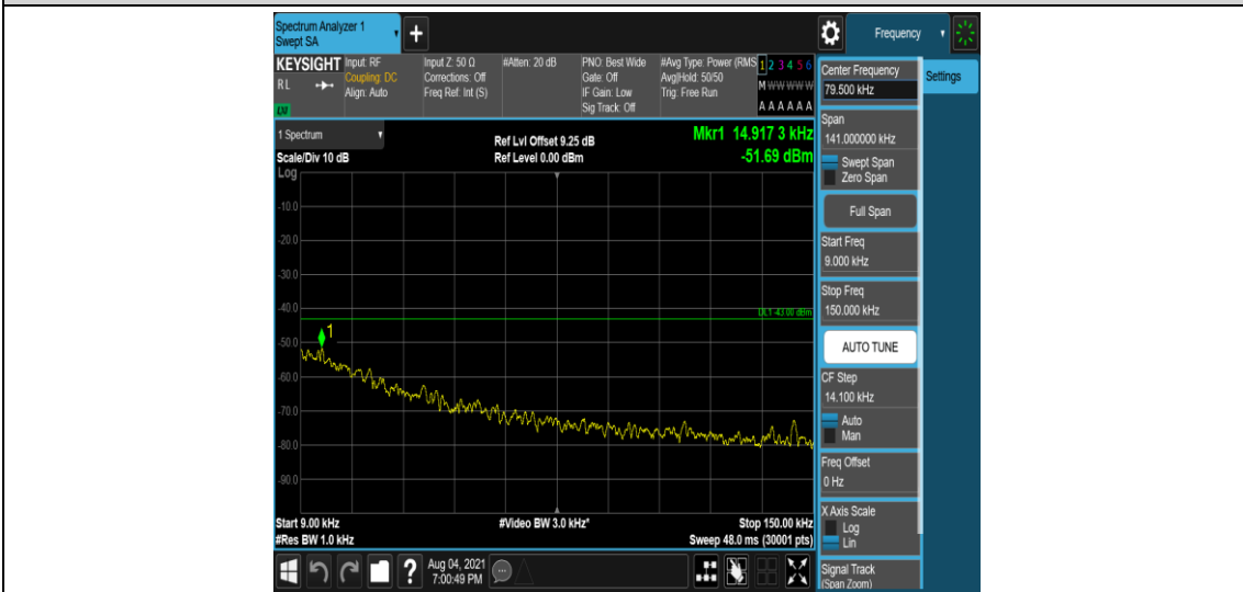
Band4-5MHz-16QAM-20375-1-0-High-0.009-0.15--51.69-PASS
