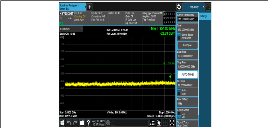
Band4-10MHz-QPSK-20175-1-0-Low-30-1000--32.29-PASS
