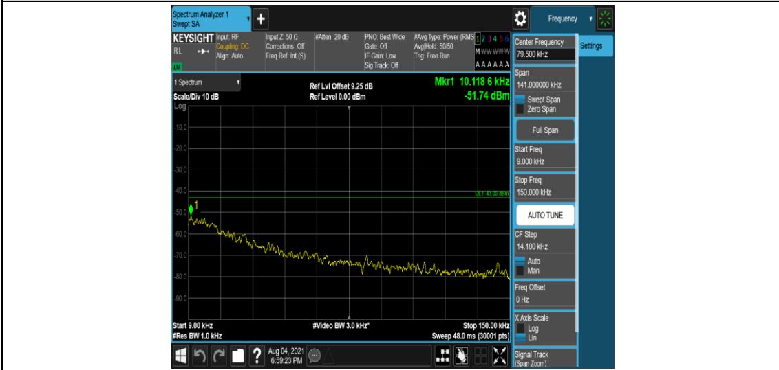
Band4-5MHz-QPSK-20375-1-0-High-0.009-0.15--51.75-PASS
