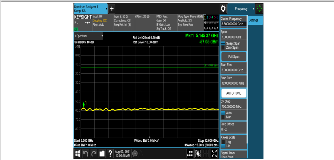
Band4-10MHz-16QAM-20000-1-0-Low-5000-12000--57.05-PASS
