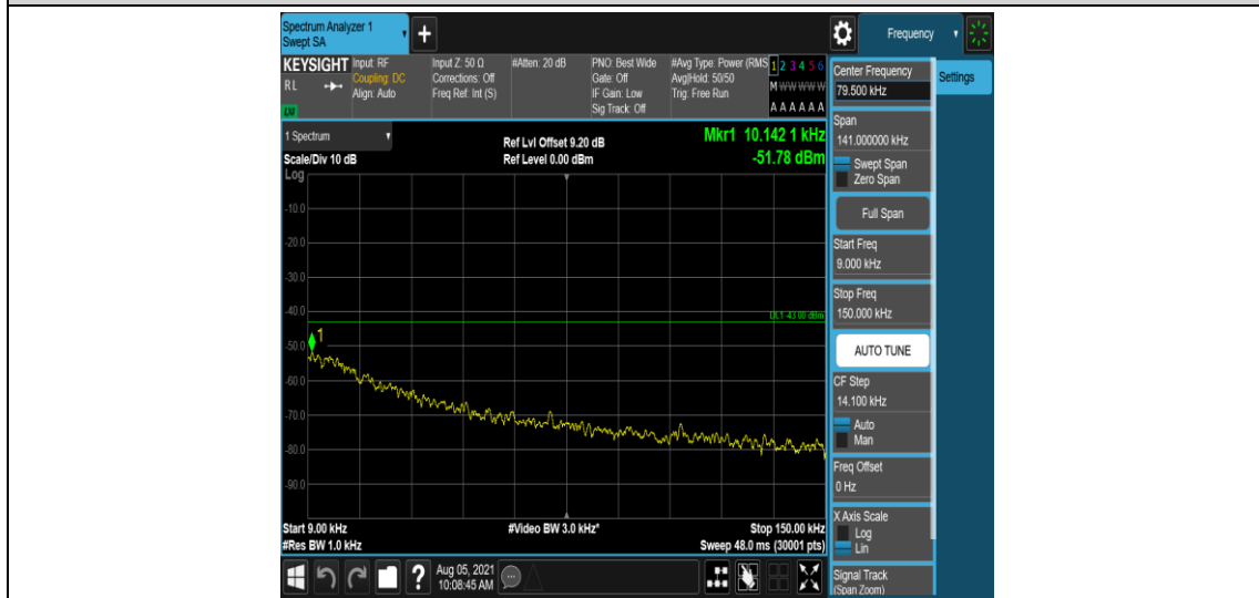
Band4-10MHz-16QAM-20175-1-0-Low-0.009-0.15--51.78-PASS
