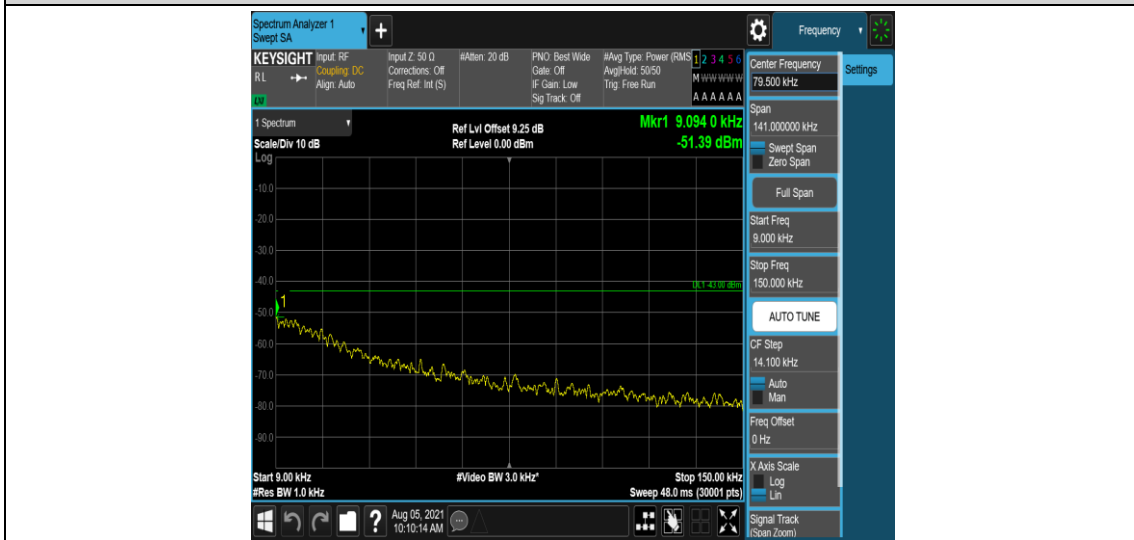
Band4-10MHz-QPSK-20350-1-0-High-0.009-0.15--51.39-PASS
