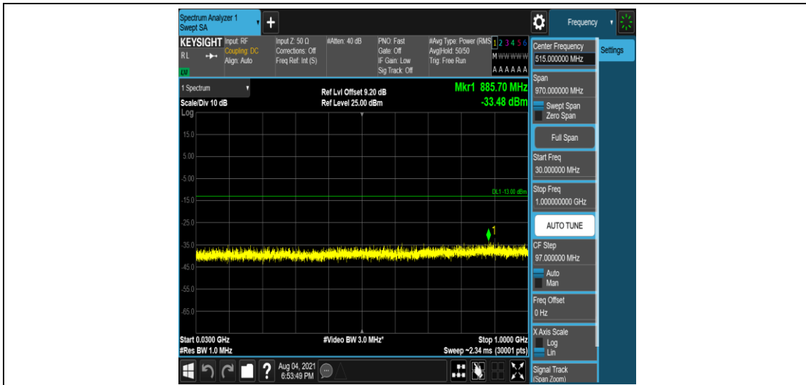
Band4-5MHz-QPSK-19975-1-0-Low-30-1000--33.48-PASS
