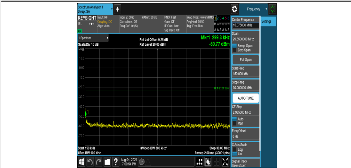
Band4-5MHz-16QAM-20375-1-0-High-0.15-30--50.77-PASS
