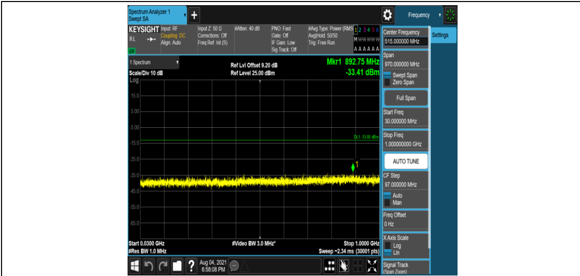
Band4-5MHz-16QAM-20175-1-0-Low-30-1000--33.41-PASS
