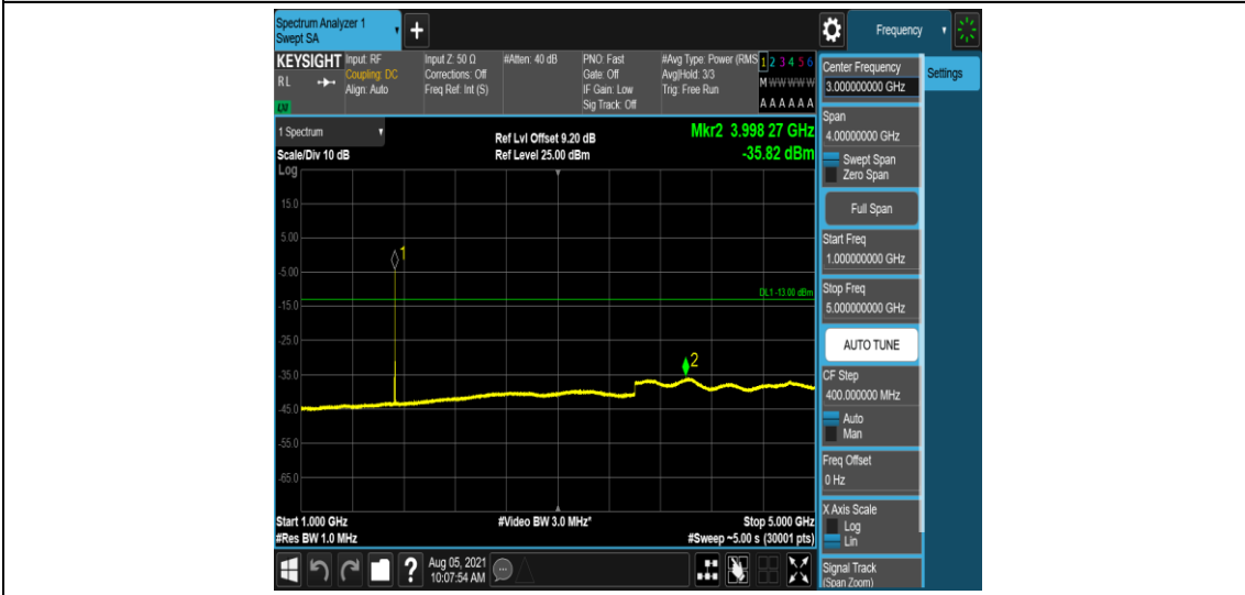
Band4-10MHz-QPSK-20175-1-0-Low-1000-5000--35.82-PASS
