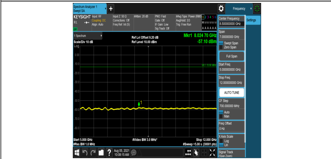
Band4-10MHz-QPSK-20175-1-0-Low-5000-12000--57.1-PASS
