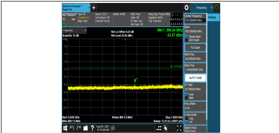
Band4-10MHz-QPSK-20350-1-0-High-30-1000--32.68-PASS
