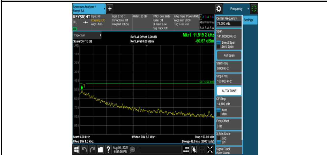
Band4-5MHz-16QAM-20175-1-0-Low-0.009-0.15--50.67-PASS
