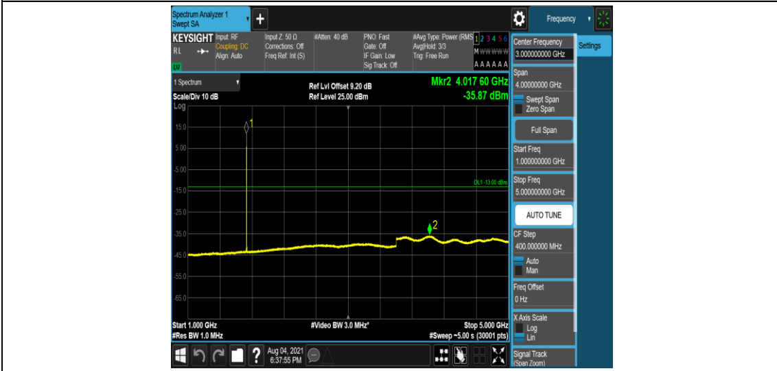
Band4-3MHz-QPSK-20175-1-0-Low-1000-5000--35.87-PASS
