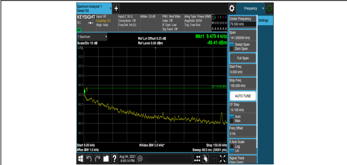
Band4-3MHz-QPSK-20385-1-0-High-0.009-0.15--49.41-PASS
