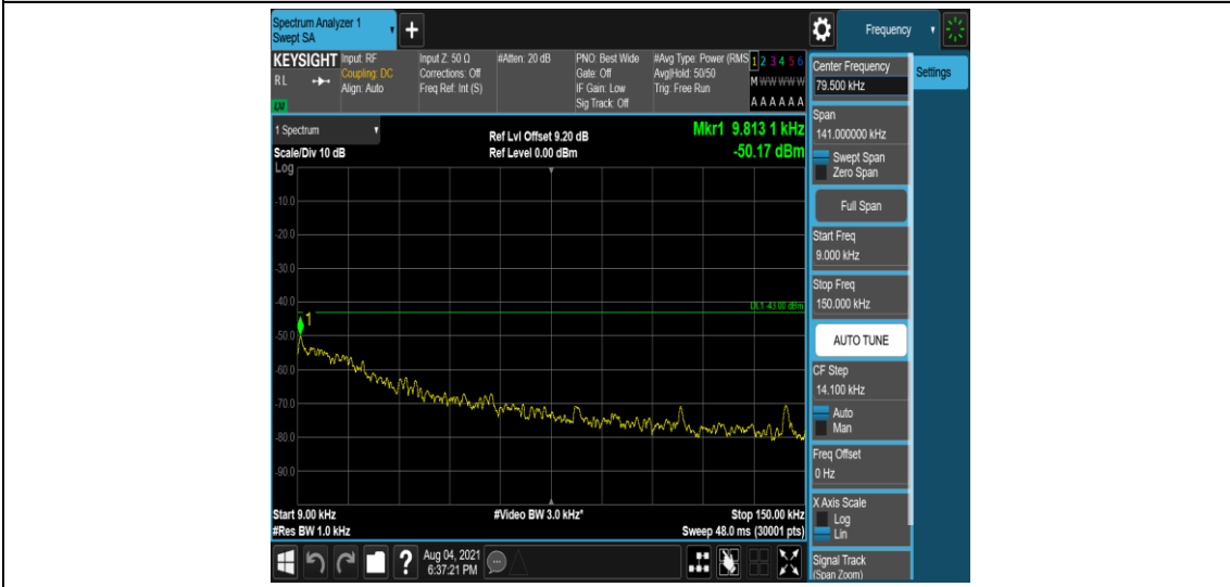
Band4-3MHz-QPSK-20175-1-0-Low-0.009-0.15--50.17-PASS
