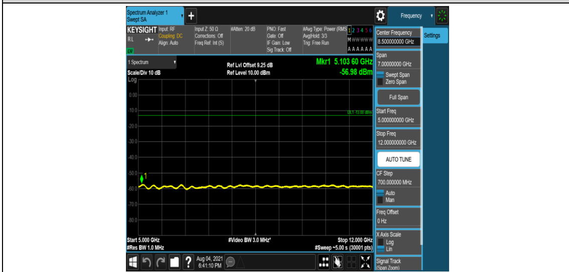
Band4-3MHz-QPSK-20385-1-0-High-5000-12000--56.98-PASS
