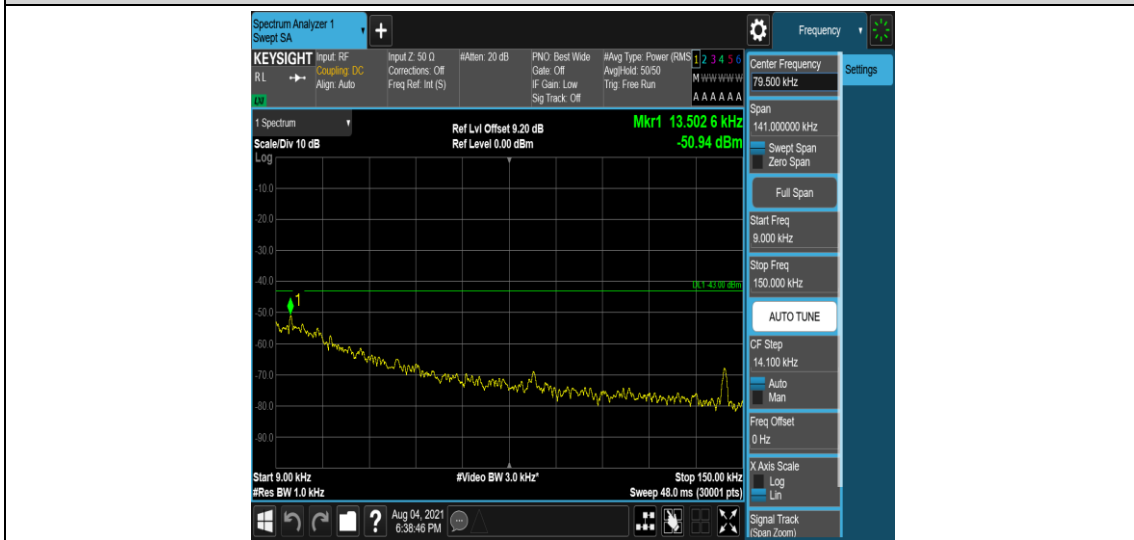
Band4-3MHz-16QAM-20175-1-0-Low-0.009-0.15--50.94-PASS
