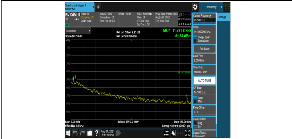
Band4-3MHz-16QAM-20385-1-0-High-0.009-0.15--51.84-PASS
