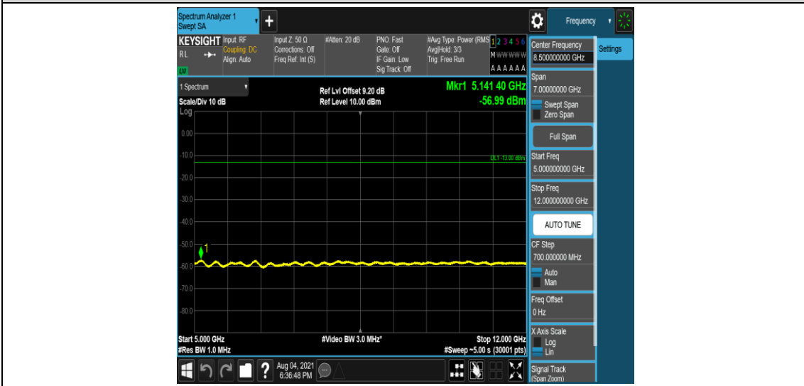
Band4-3MHz-16QAM-19965-1-0-Low-5000-12000--56.99-PASS
