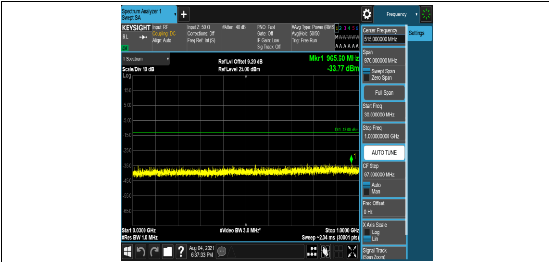
Band4-3MHz-QPSK-20175-1-0-Low-30-1000--33.77-PASS
