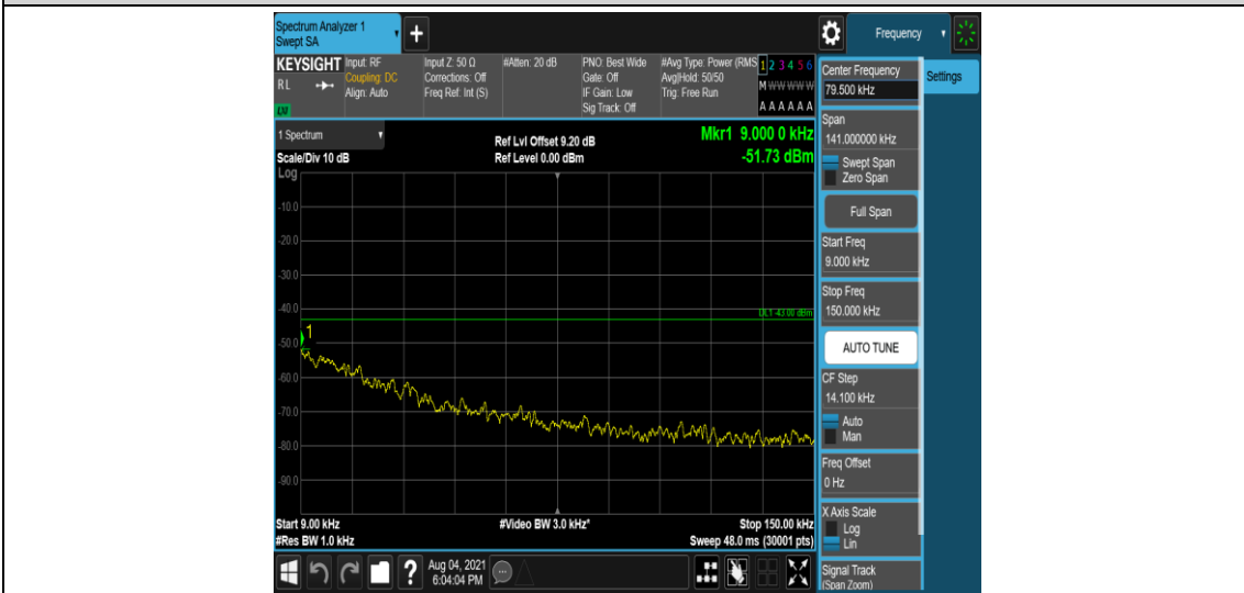
Band4-1.4MHz-16QAM-20175-1-0-Low-0.009-0.15--51.73-PASS
