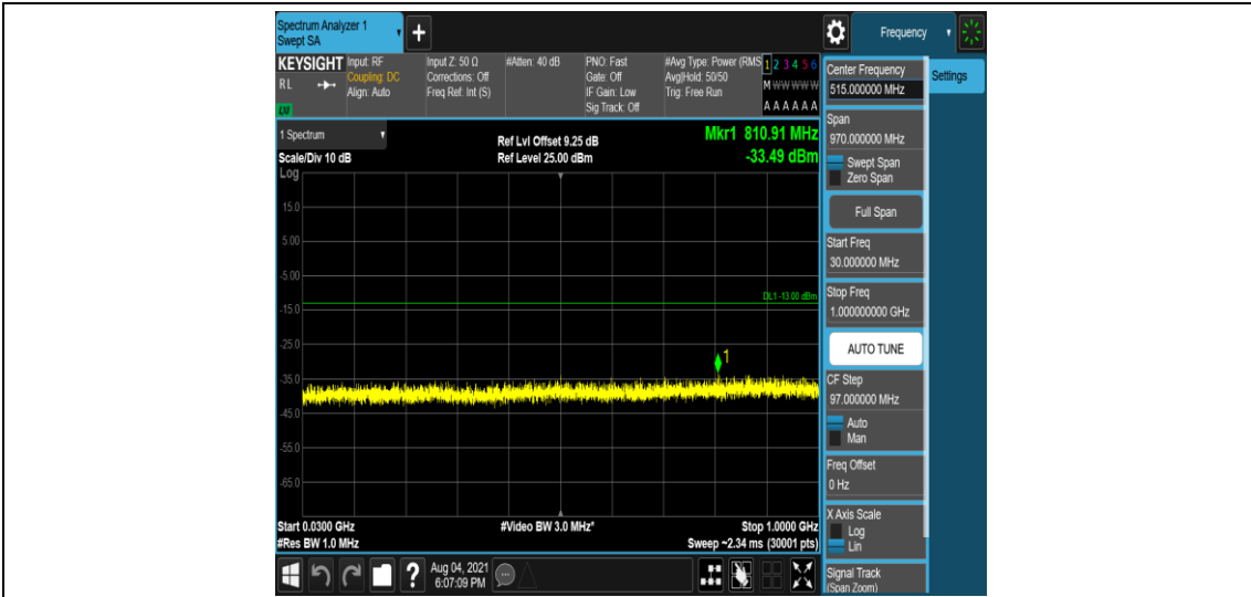
Band4-1.4MHz-16QAM-20393-1-0-High-30-1000--33.49-PASS
