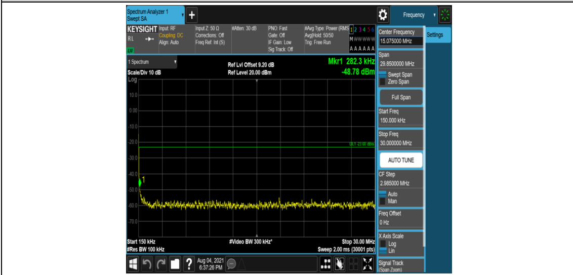
Band4-3MHz-QPSK-20175-1-0-Low-0.15-30--48.78-PASS
