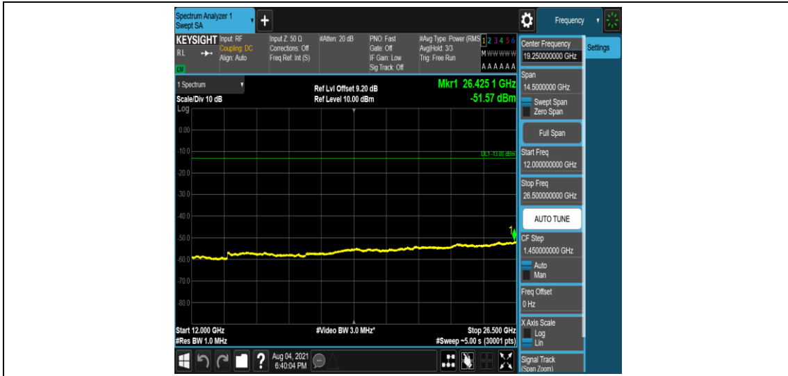
Band4-3MHz-16QAM-20175-1-0-Low-12000-26500--51.57-PASS
