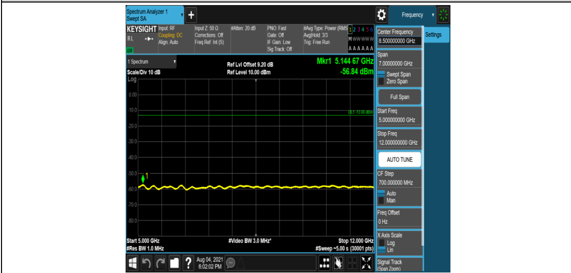
Band4-1.4MHz-16QAM-19957-1-0-Low-5000-12000--56.84-PASS
