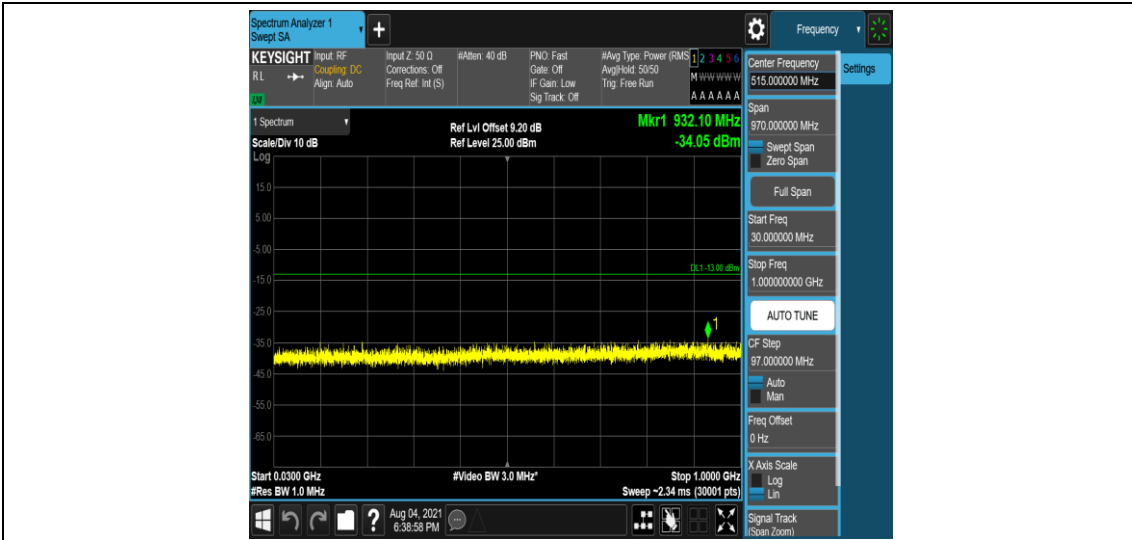
Band4-3MHz-16QAM-20175-1-0-Low-30-1000--34.05-PASS
