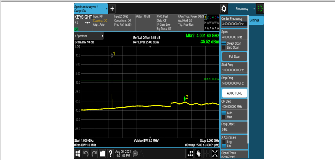
Band2-15MHz-16QAM-19125-6-0-Low-1000-5000--35.52-PASS
