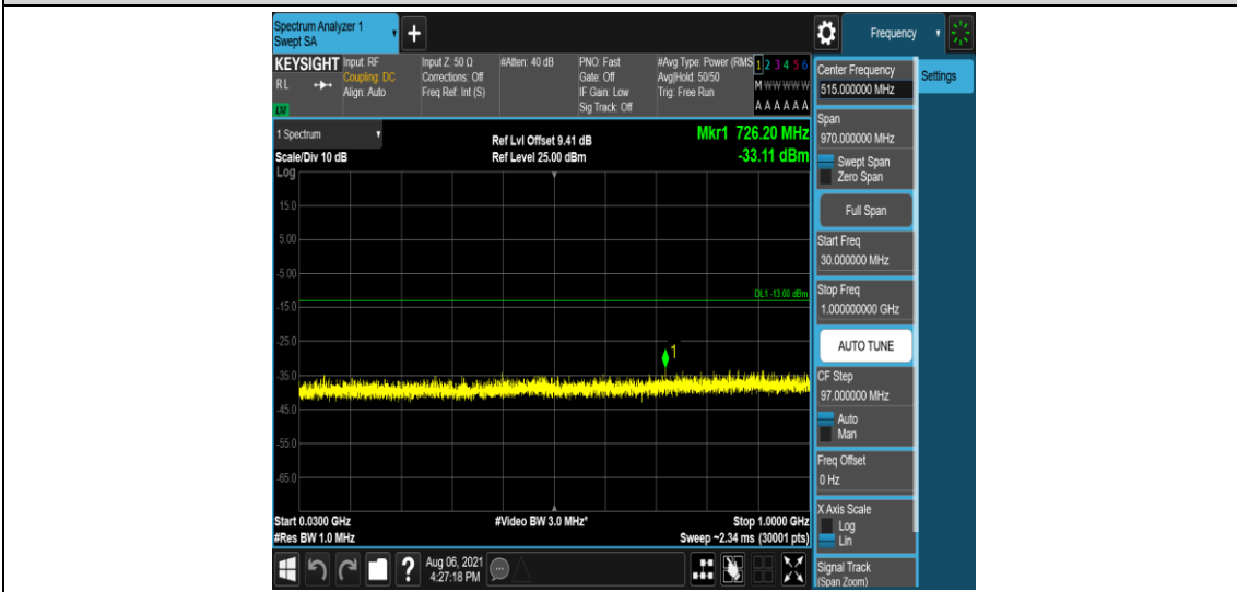
Band2-20MHz-QPSK-18700-6-0-Low-30-1000--33.11-PASS
