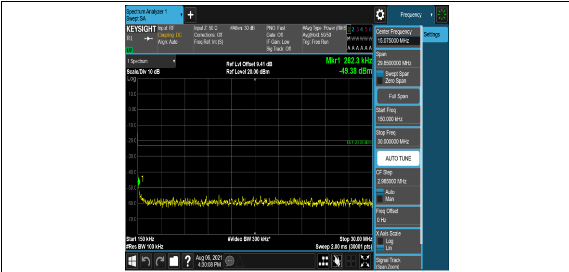
Band2-20MHz-QPSK-18900-1-5-Low-0.15-30--49.38-PASS
