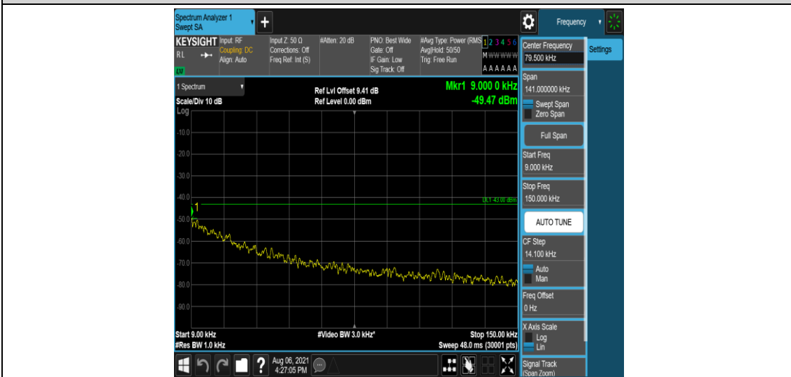
Band2-20MHz-QPSK-18700-6-0-Low-0.009-0.15--49.47-PASS
