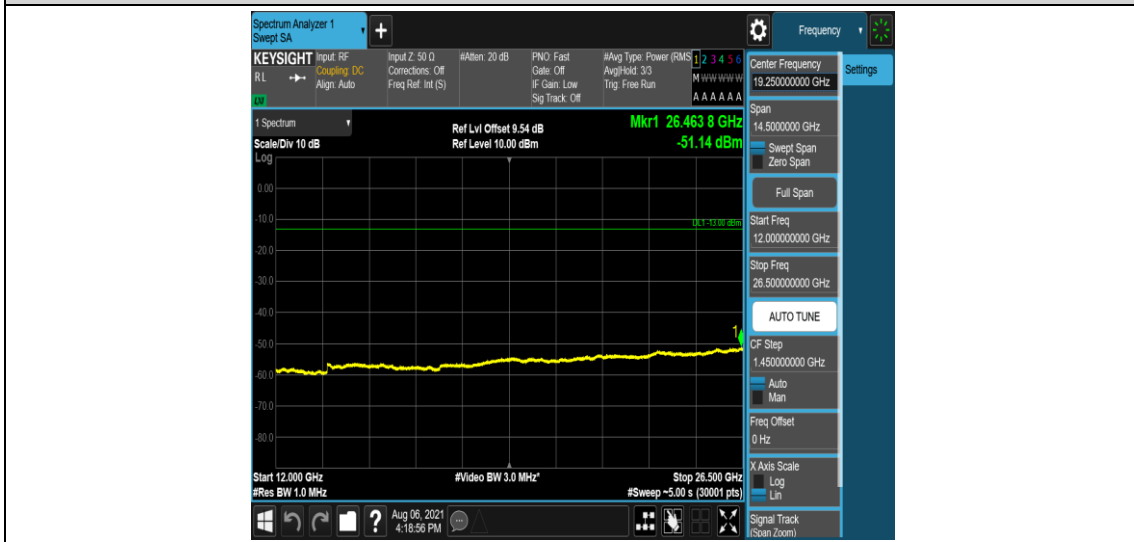
Band2-15MHz-16QAM-19125-1-0-Low-12000-26500--51.14-PASS
