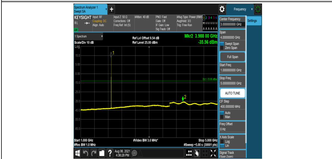
Band2-20MHz-QPSK-19100-1-0-Low-1000-5000--35.56-PASS
