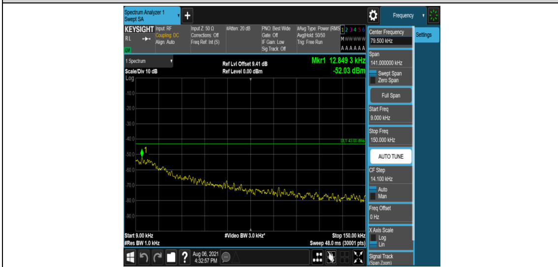
Band2-20MHz-QPSK-18900-6-0-Low-0.009-0.15--52.03-PASS
