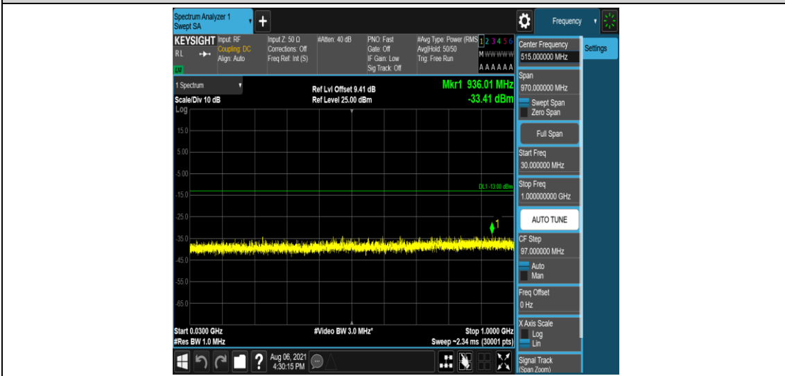
Band2-20MHz-QPSK-18900-1-5-Low-30-1000--33.41-PASS
