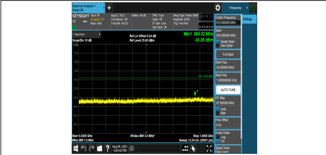
Band2-15MHz-16QAM-19125-6-0-Low-30-1000--33.29-PASS
