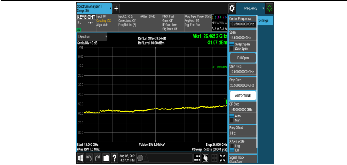
Band2-20MHz-QPSK-19100-1-0-Low-12000-26500--51.07-PASS
