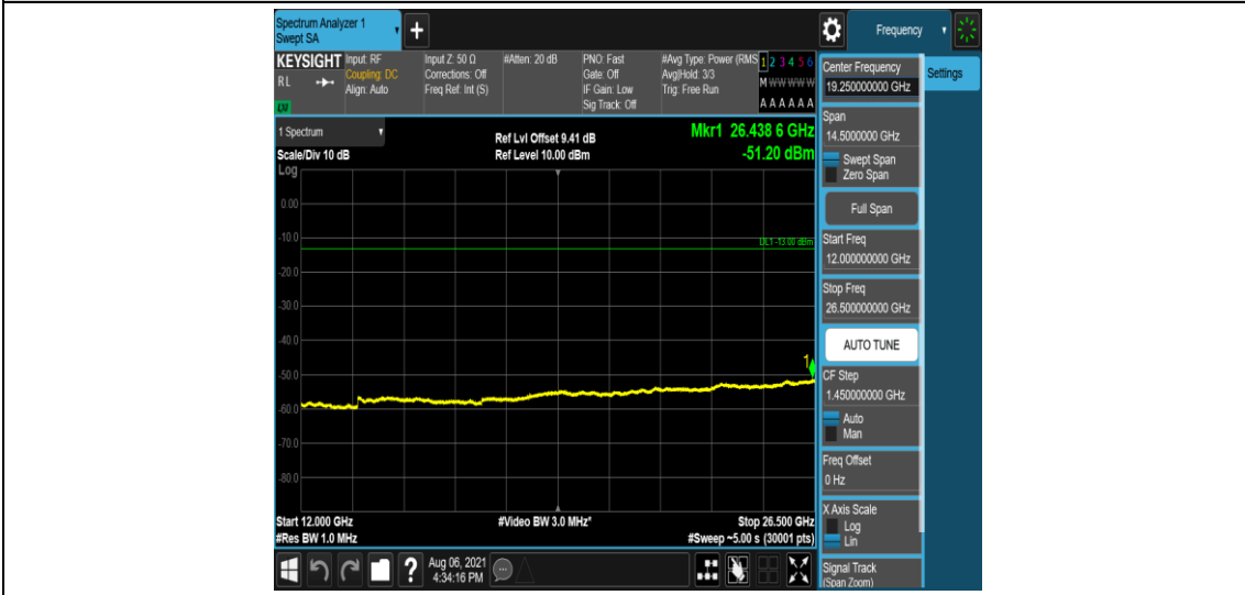
Band2-20MHz-QPSK-18900-6-0-Low-12000-26500--51.2-PASS
