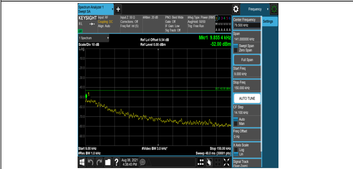
Band2-20MHz-QPSK-19100-6-0-Low-0.009-0.15--52-PASS
