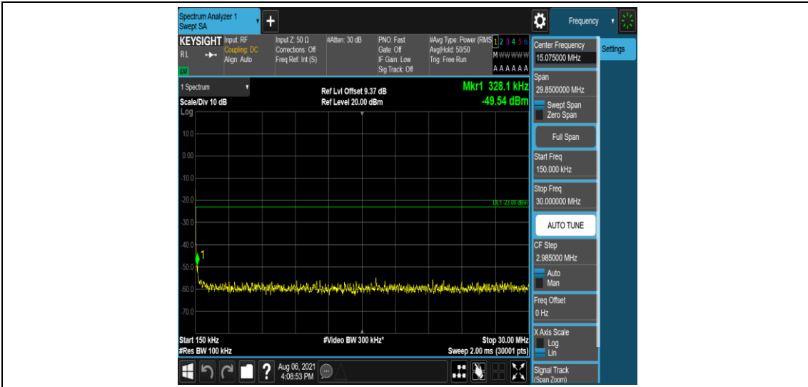
Band2-15MHz-16QAM-18675-6-0-Low-0.15-30--49.54-PASS
