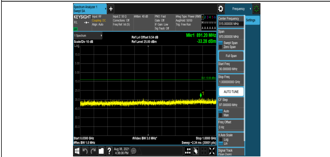
Band2-20MHz-QPSK-19100-1-0-Low-30-1000--33.29-PASS
