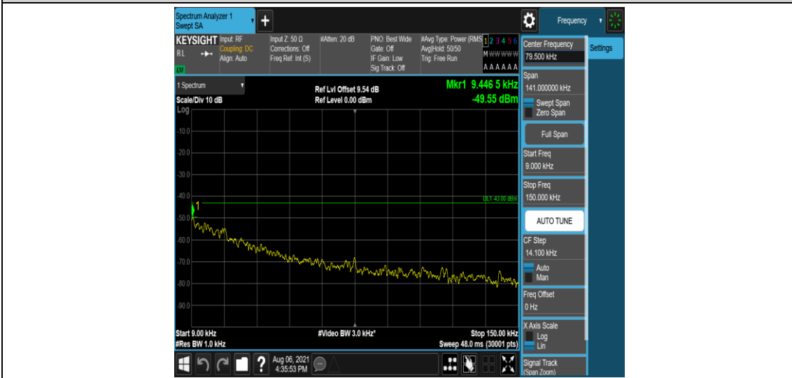
Band2-20MHz-QPSK-19100-1-0-Low-0.009-0.15--49.55-PASS
