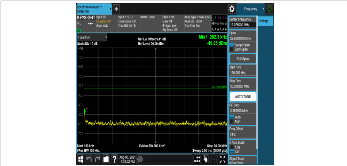
Band2-20MHz-QPSK-18900-6-0-Low-0.15-30--49.85-PASS
