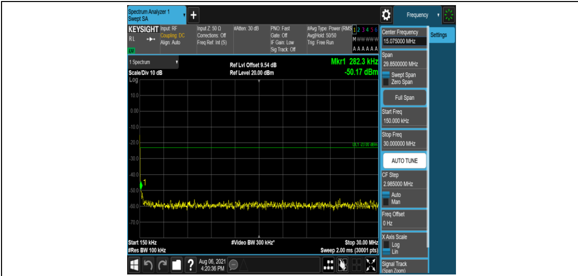
Band2-15MHz-16QAM-19125-6-0-Low-0.15-30--50.17-PASS
