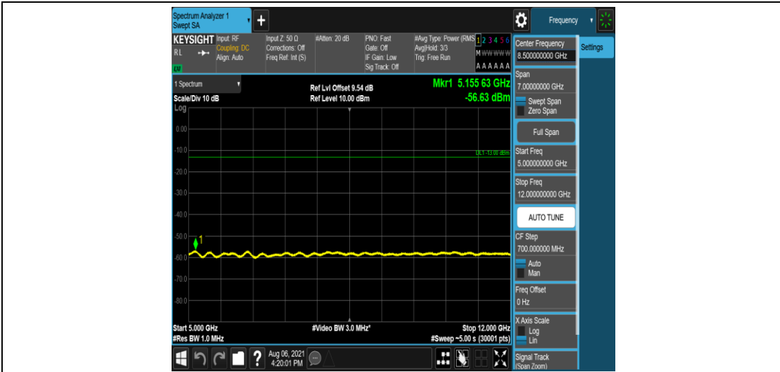
Band2-15MHz-QPSK-19125-6-0-Low-5000-12000--56.63-PASS
