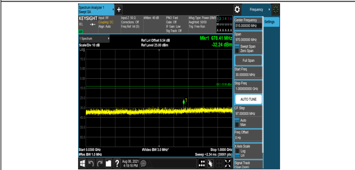
Band2-15MHz-QPSK-19125-6-0-Low-30-1000--32.24-PASS
