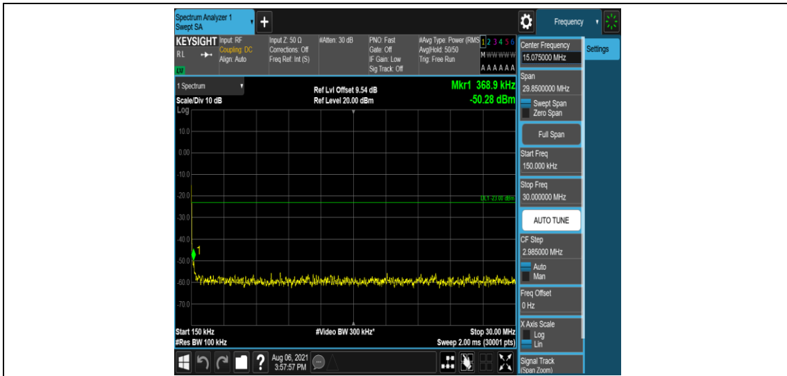
Band2-10MHz-16QAM-19150-1-0-Low-0.15-30--50.28-PASS
