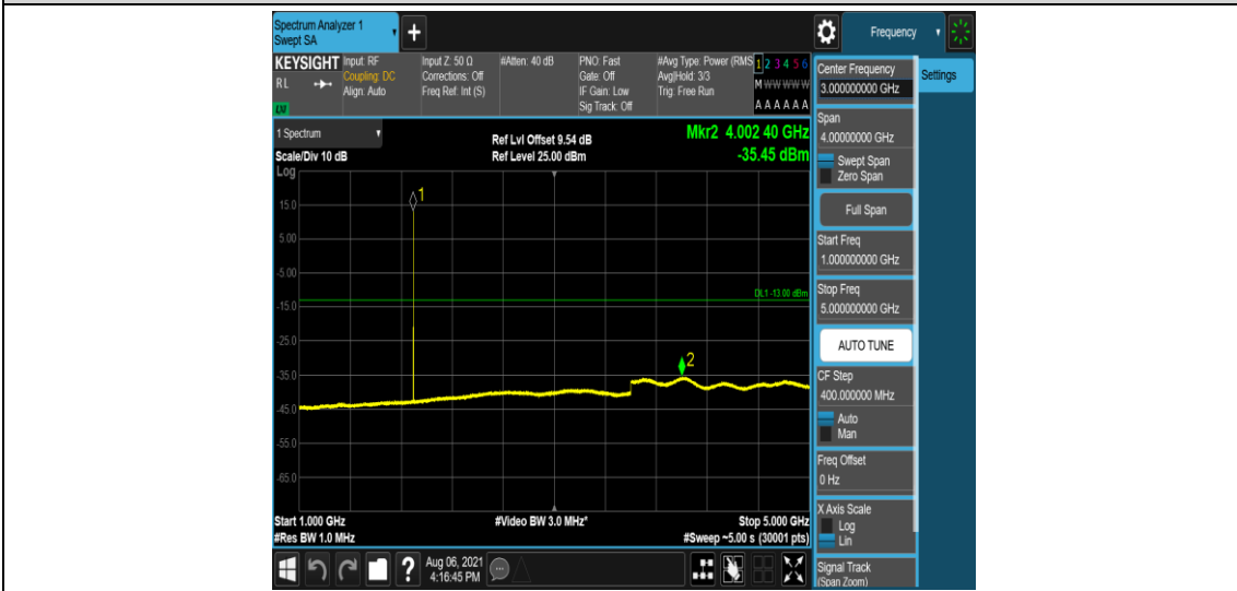
Band2-15MHz-QPSK-19125-1-0-Low-1000-5000--35.45-PASS
