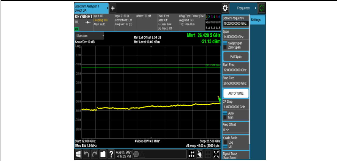
Band2-15MHz-QPSK-19125-1-0-Low-12000-26500--51.15-PASS
