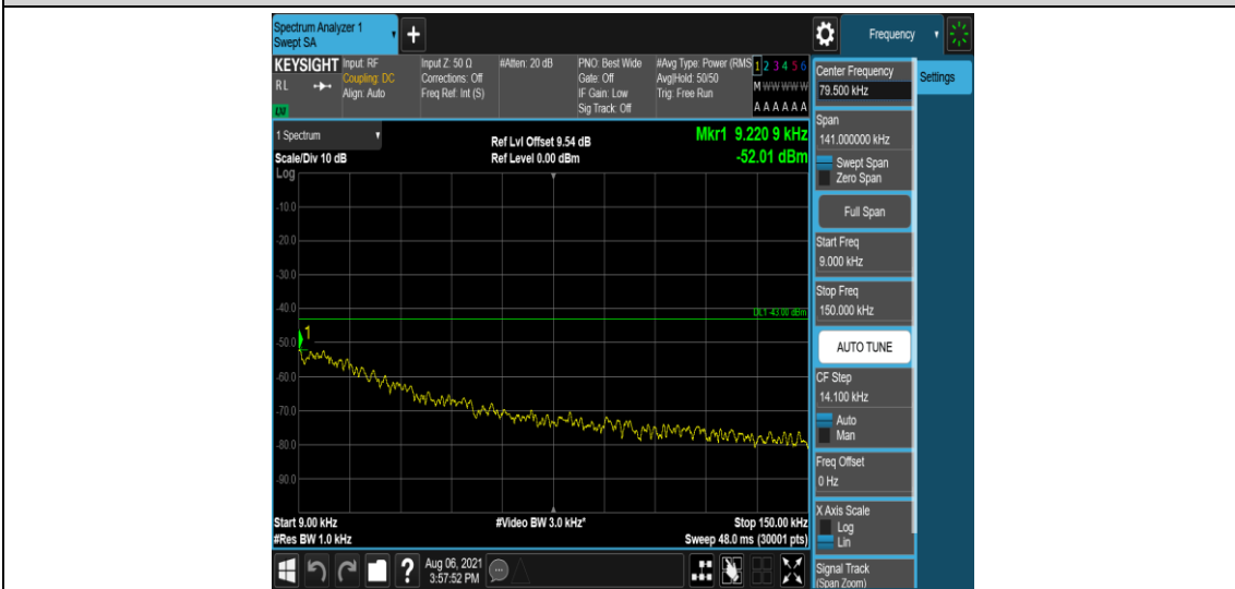
Band2-10MHz-16QAM-19150-1-0-Low-0.009-0.15--52.01-PASS
