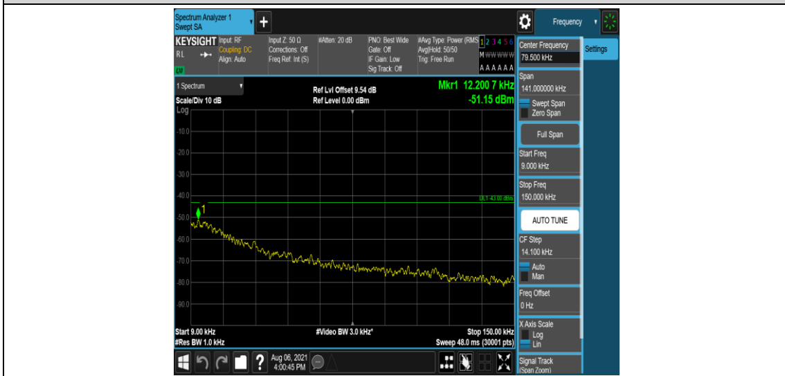
Band2-10MHz-16QAM-19150-6-0-Low-0.009-0.15--51.15-PASS
