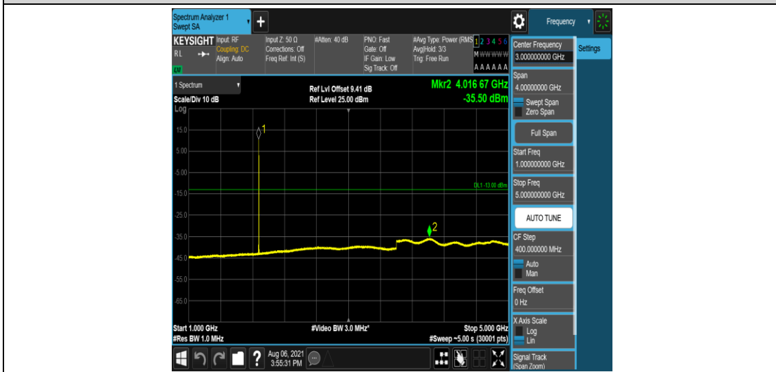
Band2-10MHz-16QAM-18900-6-0-Low-1000-5000--35.5-PASS
