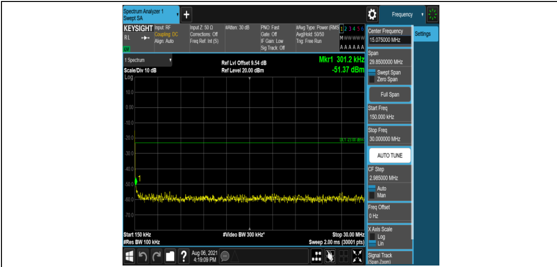
Band2-15MHz-QPSK-19125-6-0-Low-0.15-30--51.38-PASS
