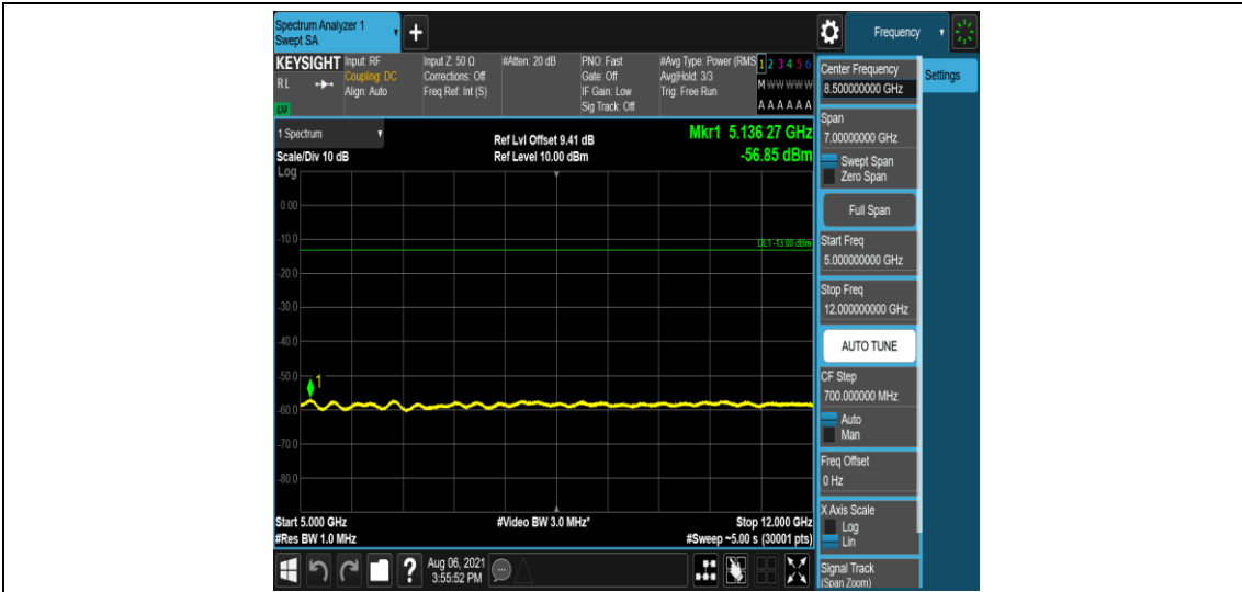
Band2-10MHz-16QAM-18900-6-0-Low-5000-12000--56.85-PASS
