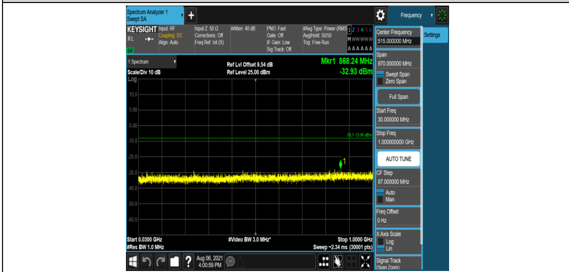
Band2-10MHz-16QAM-19150-6-0-Low-30-1000--32.93-PASS
