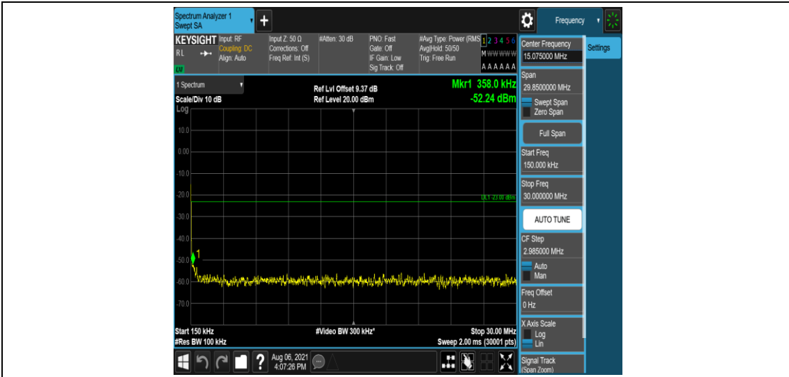
Band2-15MHz-QPSK-18675-6-0-Low-0.15-30--52.24-PASS
