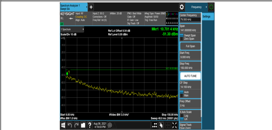
Band2-15MHz-QPSK-19125-6-0-Low-0.009-0.15--51.3-PASS
