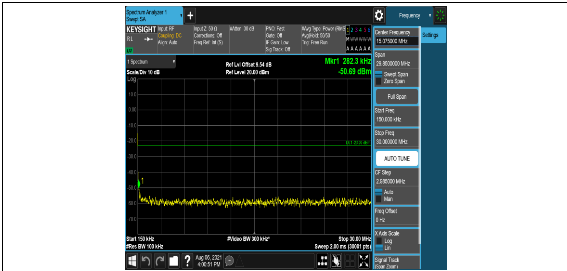
Band2-10MHz-16QAM-19150-6-0-Low-0.15-30--50.69-PASS
