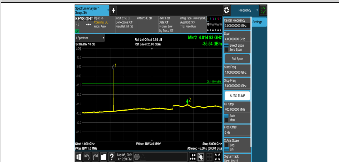
Band2-15MHz-QPSK-19125-6-0-Low-1000-5000--35.54-PASS
