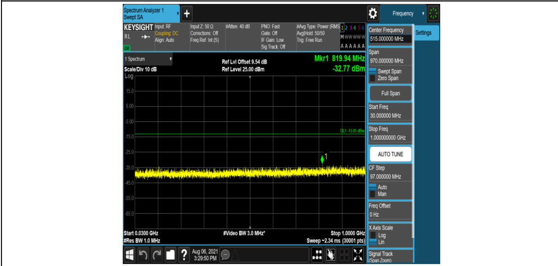
Band2-5MHz-16QAM-19175-6-0-Low-30-1000--32.77-PASS
