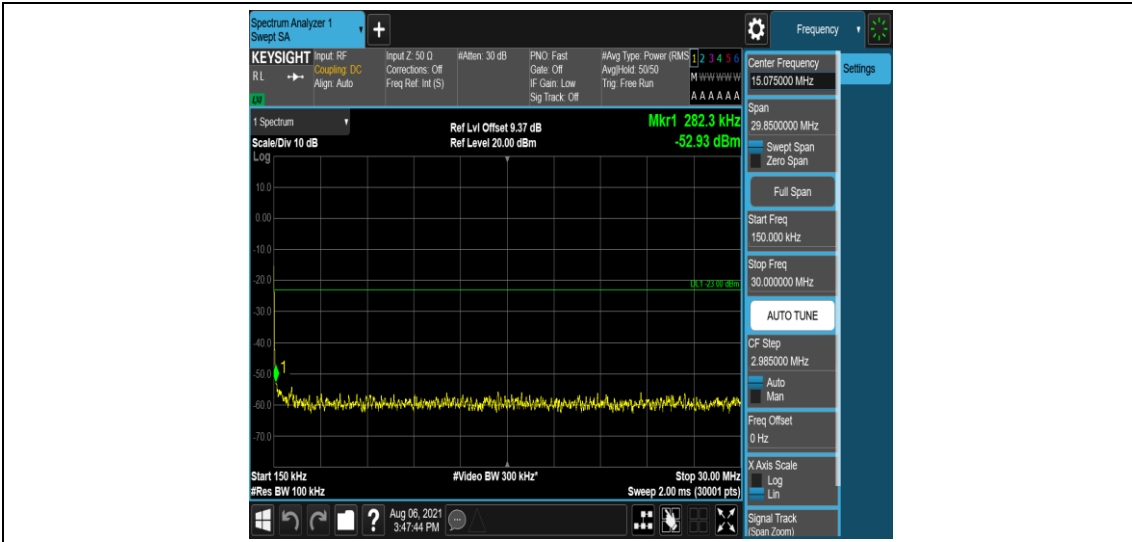
Band2-10MHz-QPSK-18650-6-0-Low-0.15-30--52.93-PASS
