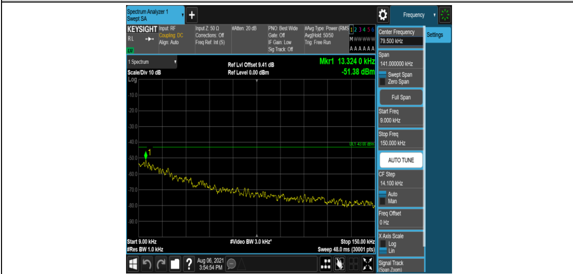
Band2-10MHz-16QAM-18900-6-0-Low-0.009-0.15--51.38-PASS
