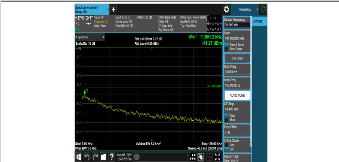
Band2-10MHz-16QAM-18650-1-0-Low-0.009-0.15--51.27-PASS
