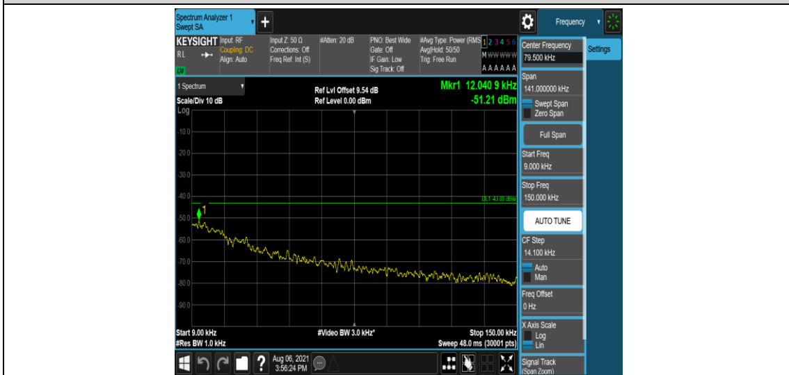
Band2-10MHz-QPSK-19150-1-0-Low-0.009-0.15--51.21-PASS
