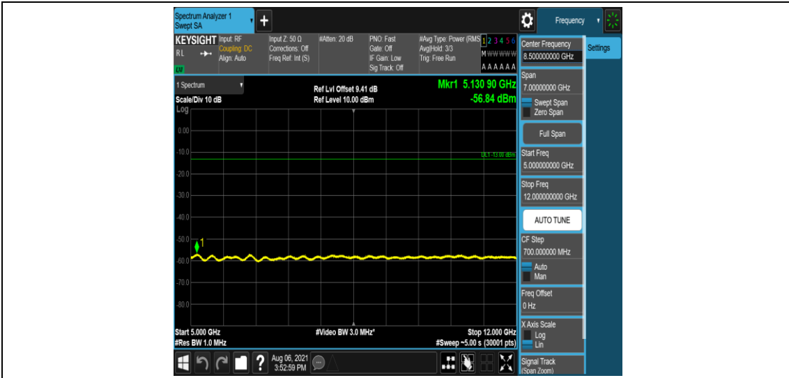
Band2-10MHz-16QAM-18900-1-5-Low-5000-12000--56.84-PASS
