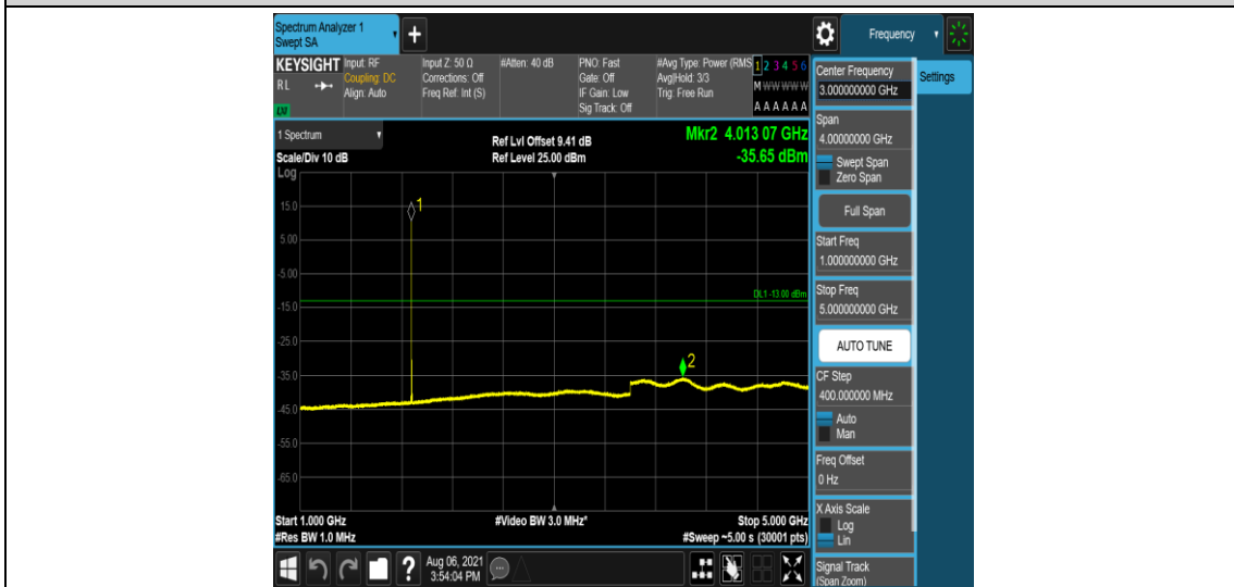
Band2-10MHz-QPSK-18900-6-0-Low-1000-5000--35.65-PASS
