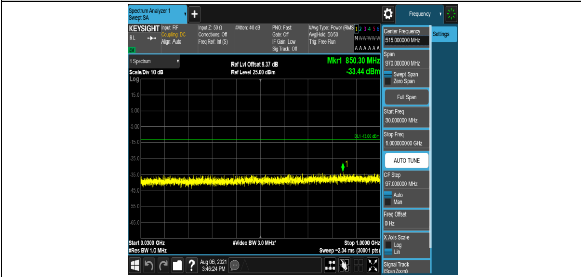
Band2-10MHz-16QAM-18650-1-0-Low-30-1000--33.44-PASS
