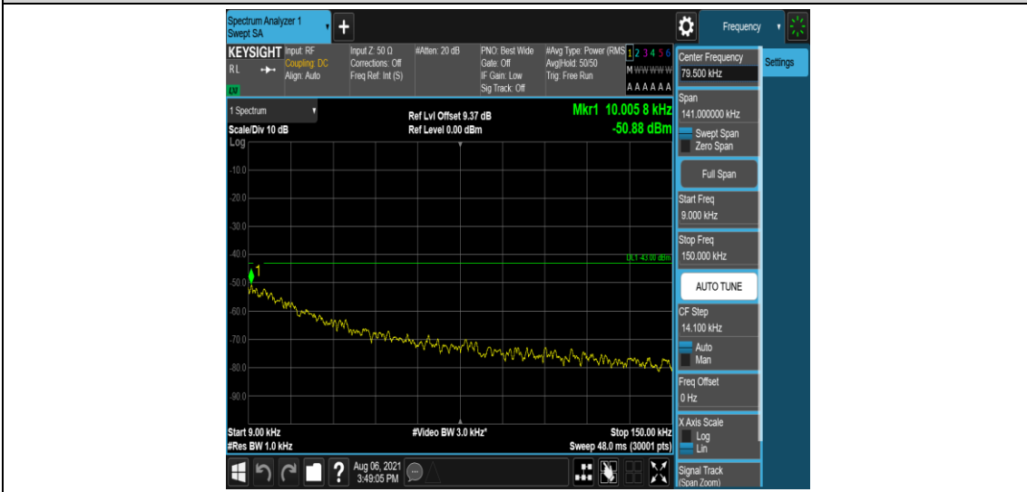
Band2-10MHz-16QAM-18650-6-0-Low-0.009-0.15--50.88-PASS
