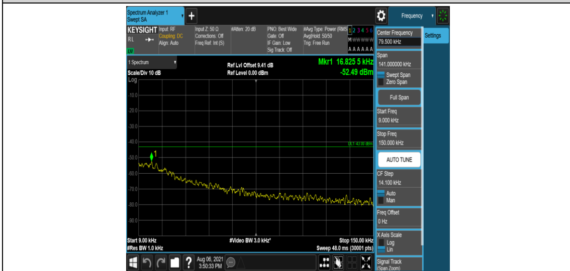
Band2-10MHz-QPSK-18900-1-5-Low-0.009-0.15--52.49-PASS
