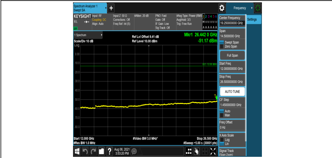
Band2-10MHz-16QAM-18900-1-5-Low-12000-26500--51.17-PASS
