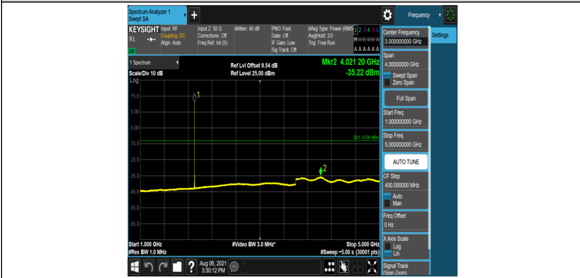
Band2-5MHz-16QAM-19175-6-0-Low-1000-5000--35.22-PASS
