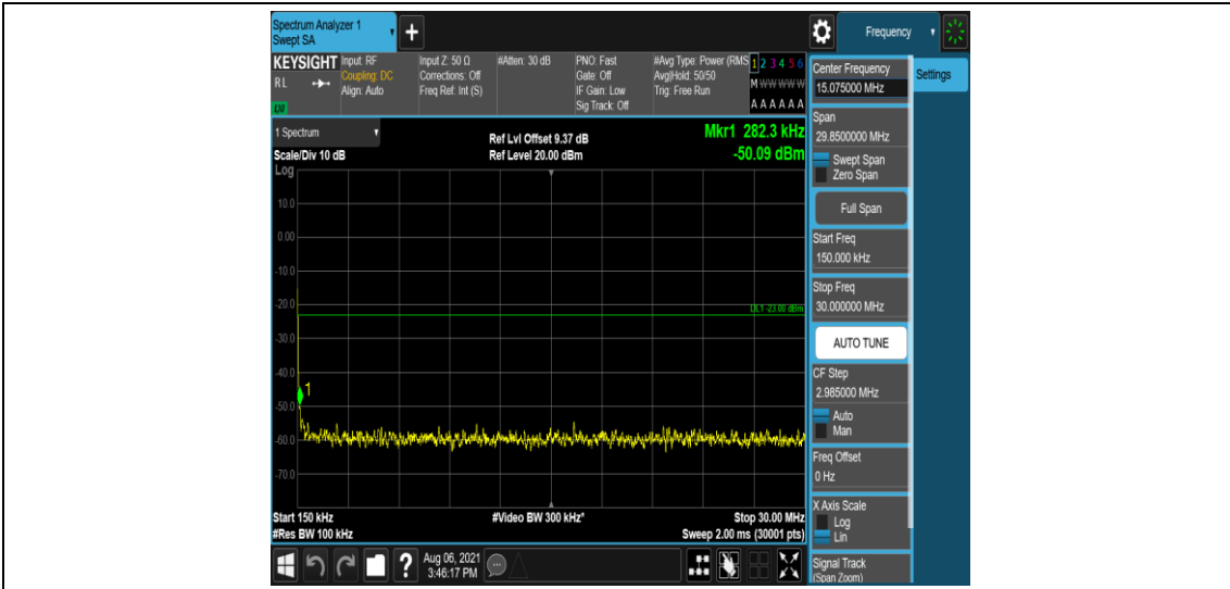
Band2-10MHz-16QAM-18650-1-0-Low-0.15-30--50.09-PASS
