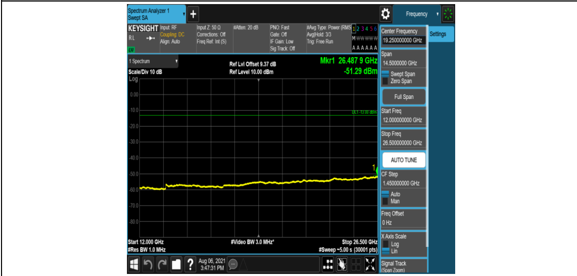
Band2-10MHz-16QAM-18650-1-0-Low-12000-26500--51.29-PASS
