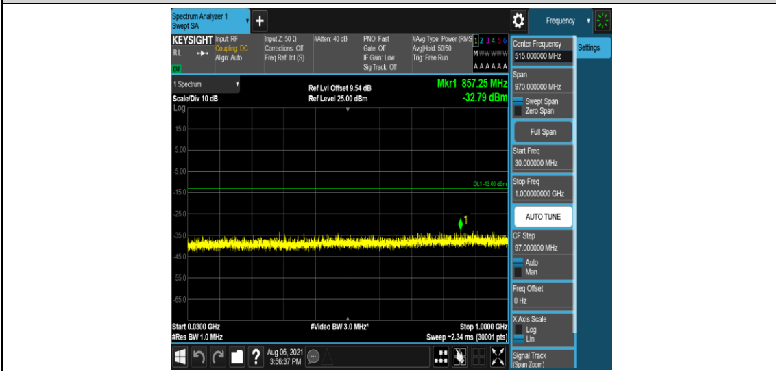
Band2-10MHz-QPSK-19150-1-0-Low-30-1000--32.79-PASS
