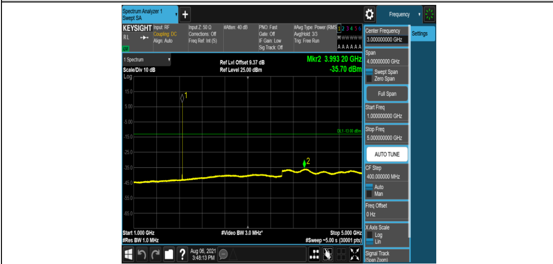
Band2-10MHz-QPSK-18650-6-0-Low-1000-5000--35.7-PASS
