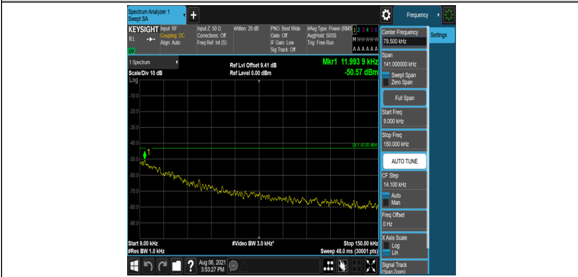
Band2-10MHz-QPSK-18900-6-0-Low-0.009-0.15--50.57-PASS
