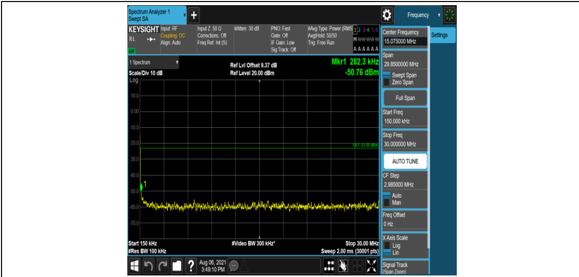
Band2-10MHz-16QAM-18650-6-0-Low-0.15-30--50.76-PASS
