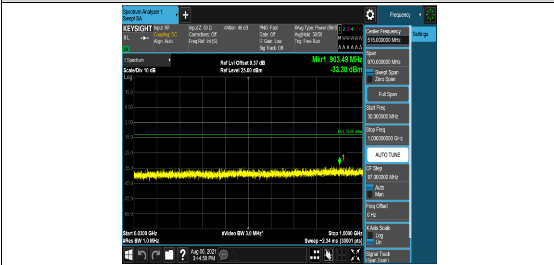
Band2-10MHz-QPSK-18650-1-0-Low-30-1000--33.3-PASS
