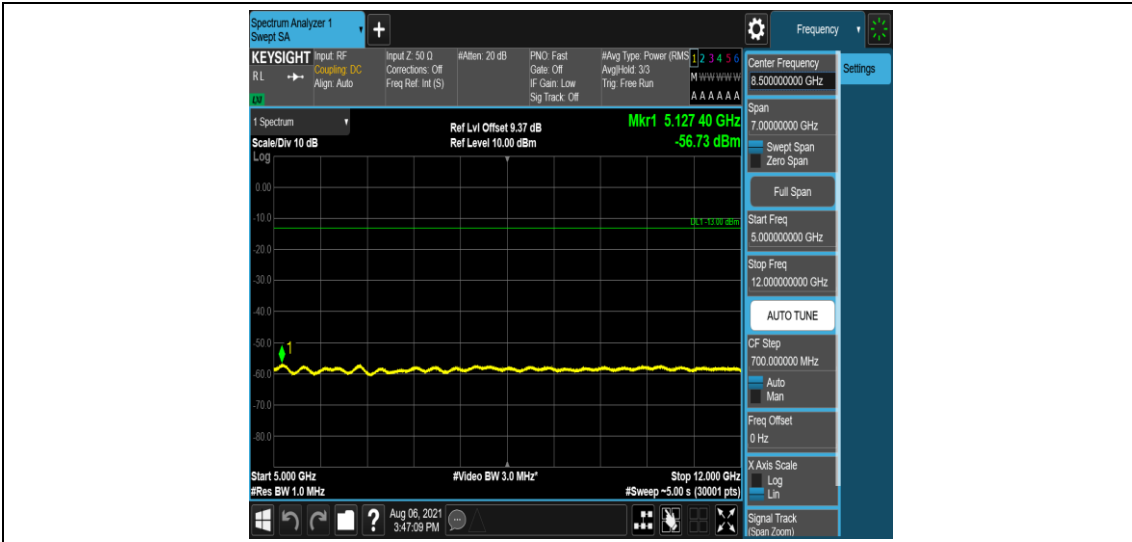
Band2-10MHz-16QAM-18650-1-0-Low-5000-12000--56.73-PASS
