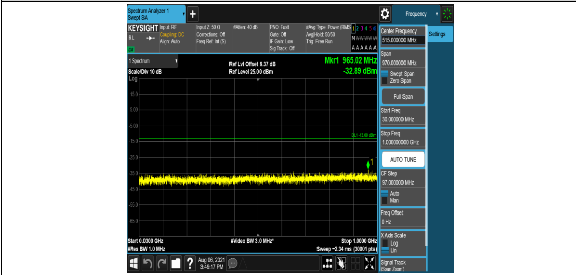
Band2-10MHz-16QAM-18650-6-0-Low-30-1000--32.89-PASS
