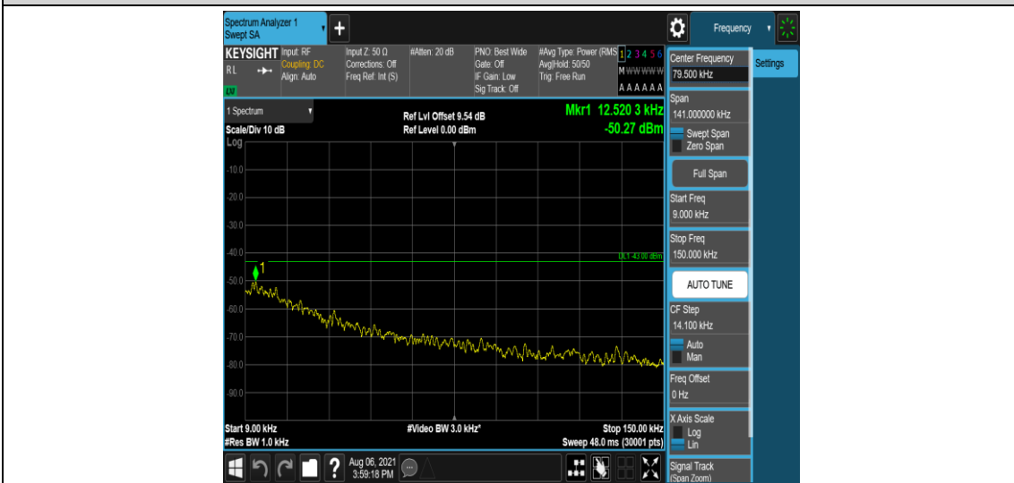
Band2-10MHz-QPSK-19150-6-0-Low-0.009-0.15--50.27-PASS
