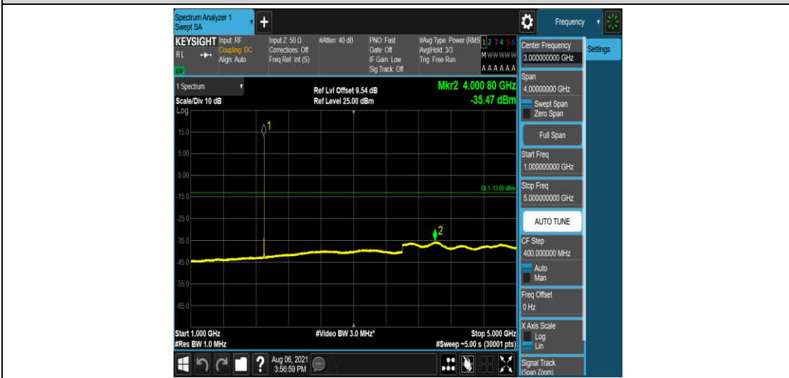
Band2-10MHz-QPSK-19150-1-0-Low-1000-5000--35.47-PASS
