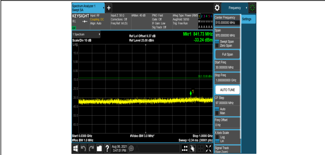
Band2-10MHz-QPSK-18650-6-0-Low-30-1000--33.24-PASS
