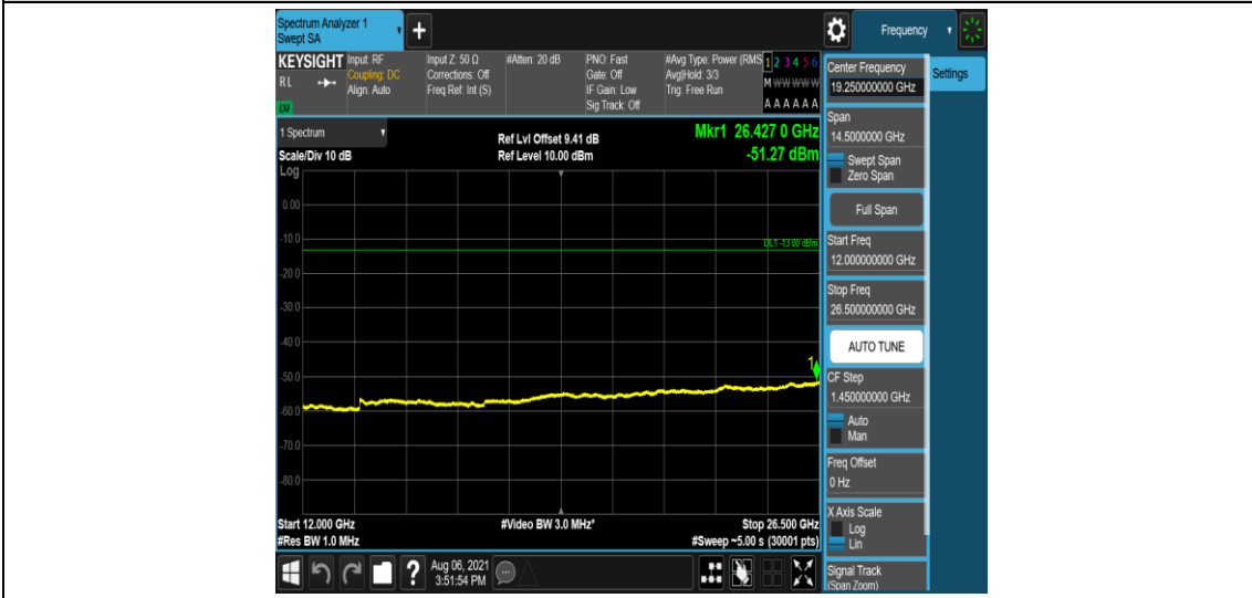
Band2-10MHz-QPSK-18900-1-5-Low-12000-26500--51.27-PASS
