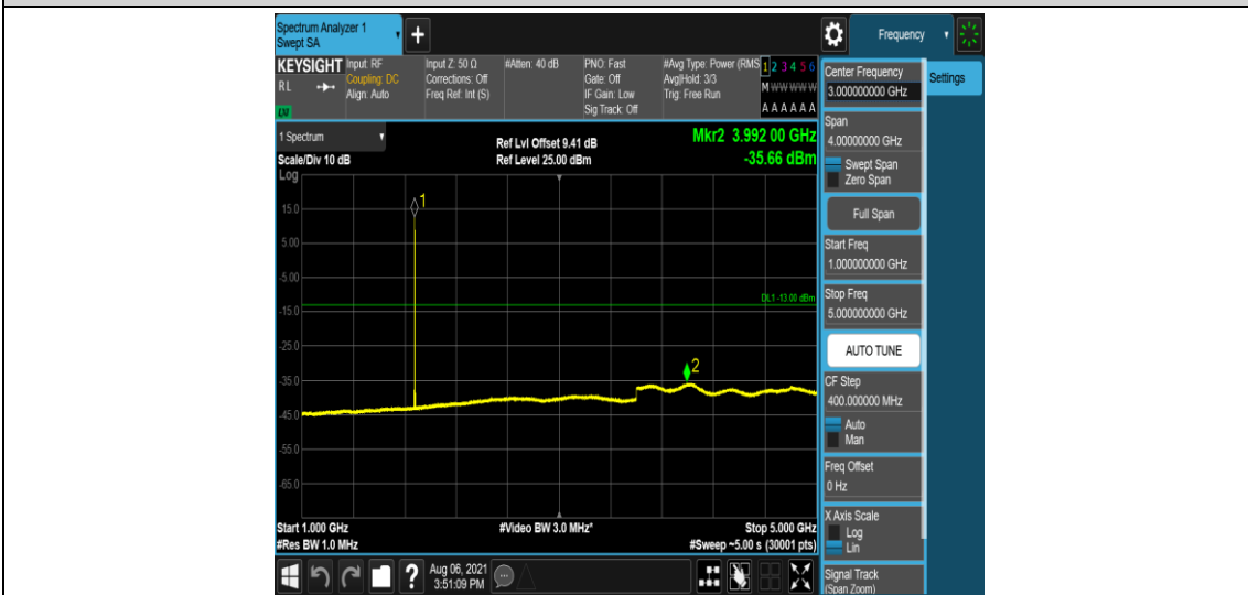
Band2-10MHz-QPSK-18900-1-5-Low-1000-5000--35.66-PASS
