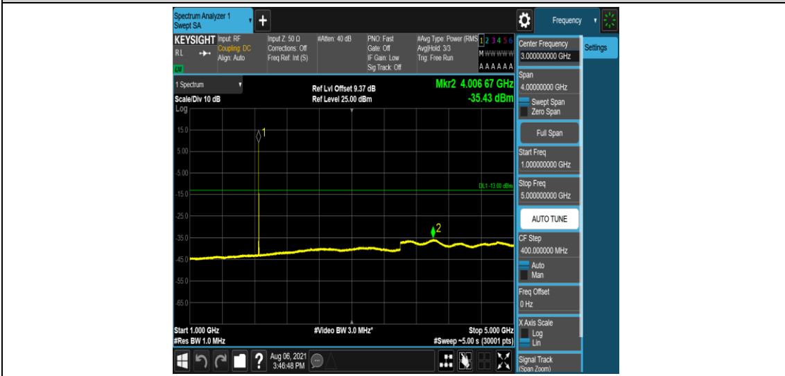
Band2-10MHz-16QAM-18650-1-0-Low-1000-5000--35.43-PASS
