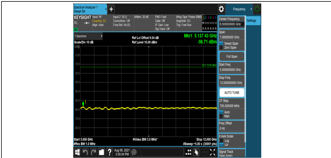
Band2-5MHz-16QAM-19175-6-0-Low-5000-12000--56.71-PASS
